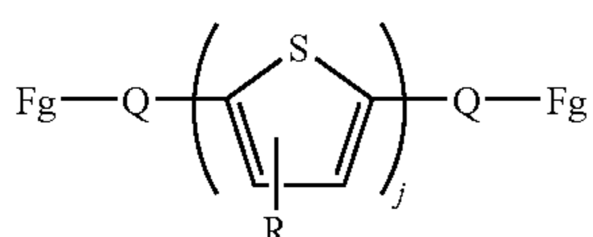
Building blocks containing an oligothiophene core
