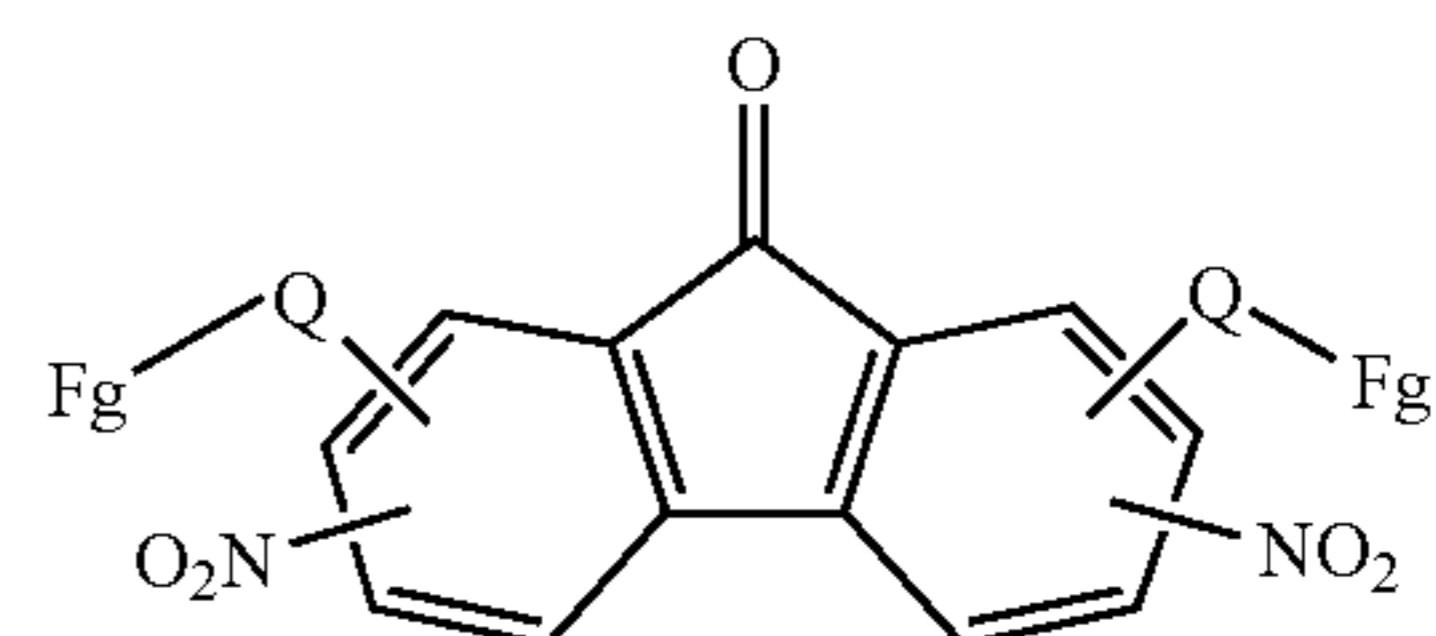
nitrofluorenones
