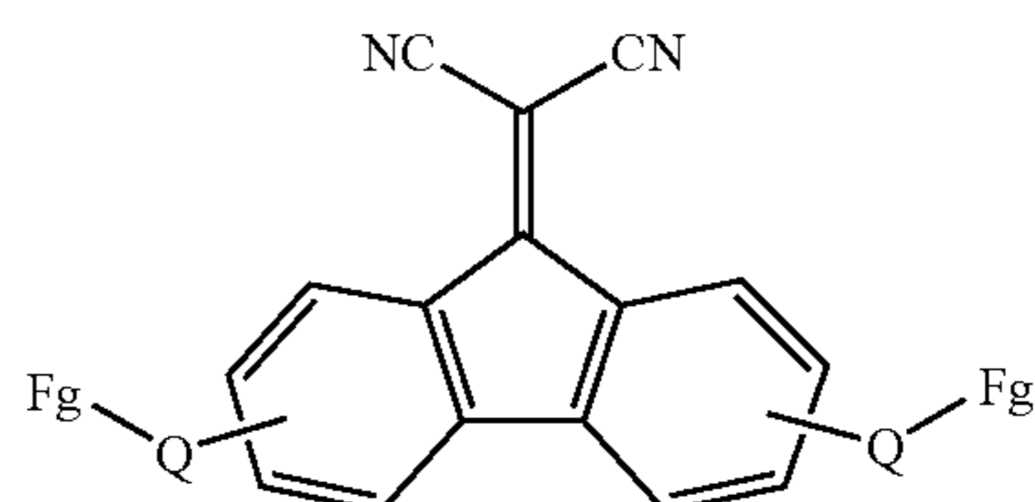
9-fluorenylidene malonitriles
