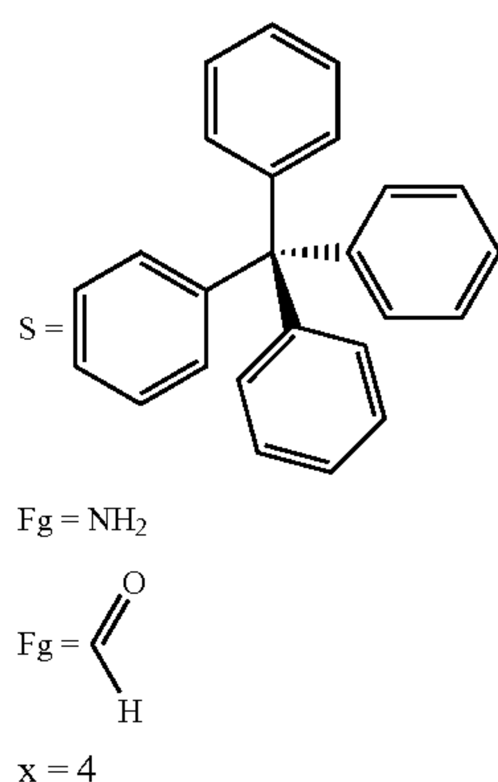
Molecular Building Block with Two Types of Functional Group.
