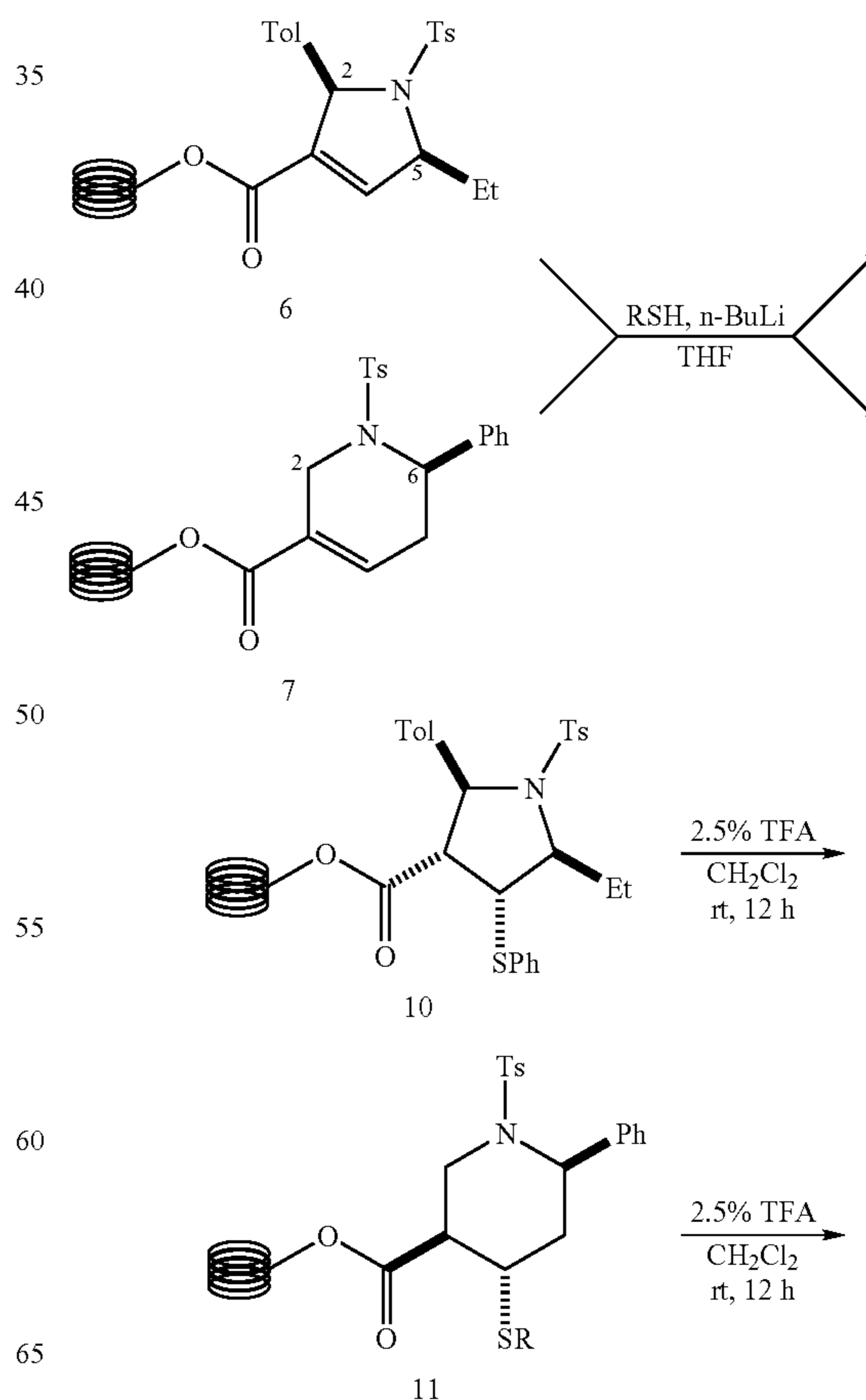
Scheme 2. Solid phase diastereoselective Michael additions.
