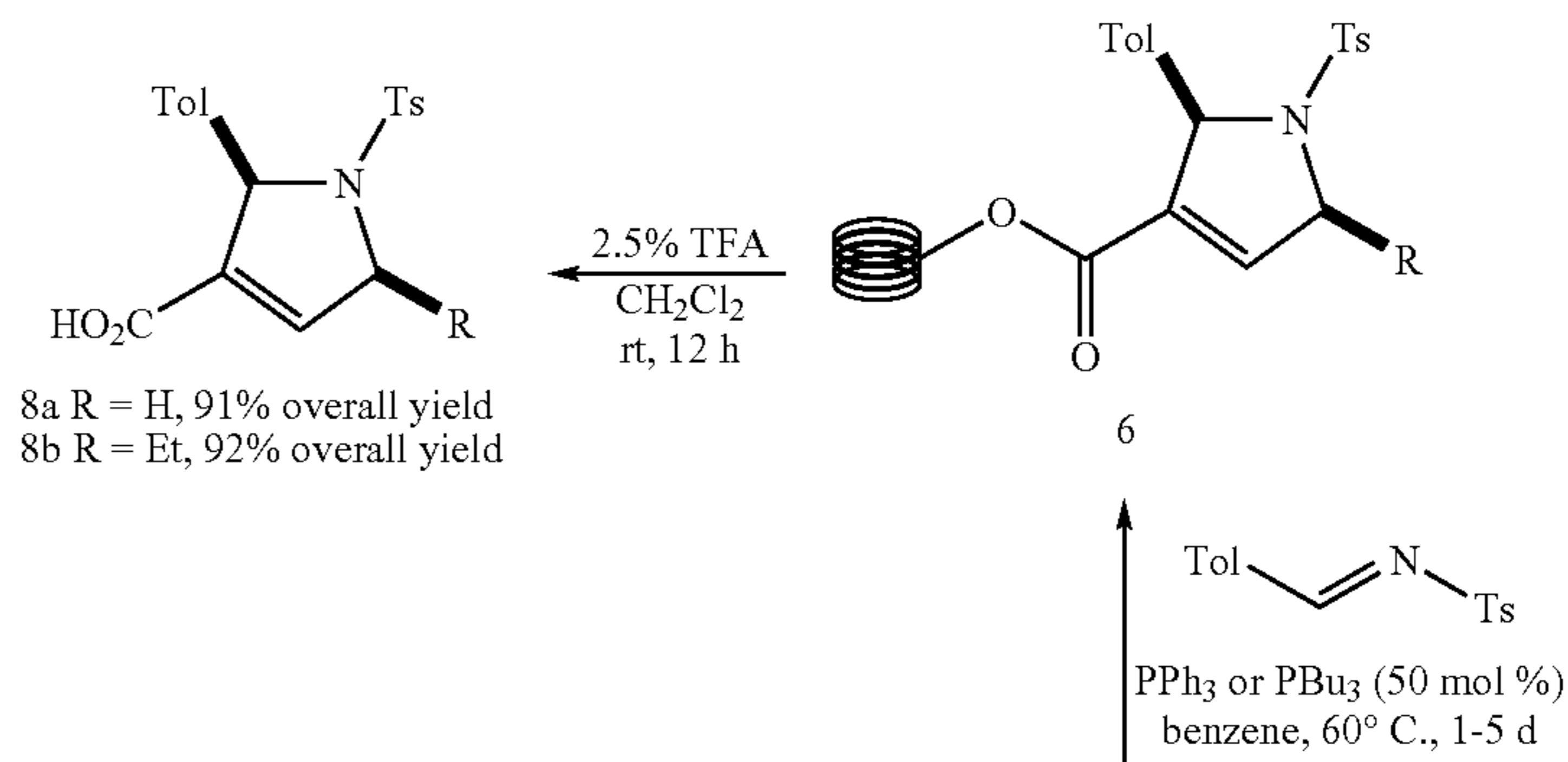
Scheme I. Solid phase syntheses of dihydropyrroles 8 and tetrahydropyridines 9.
