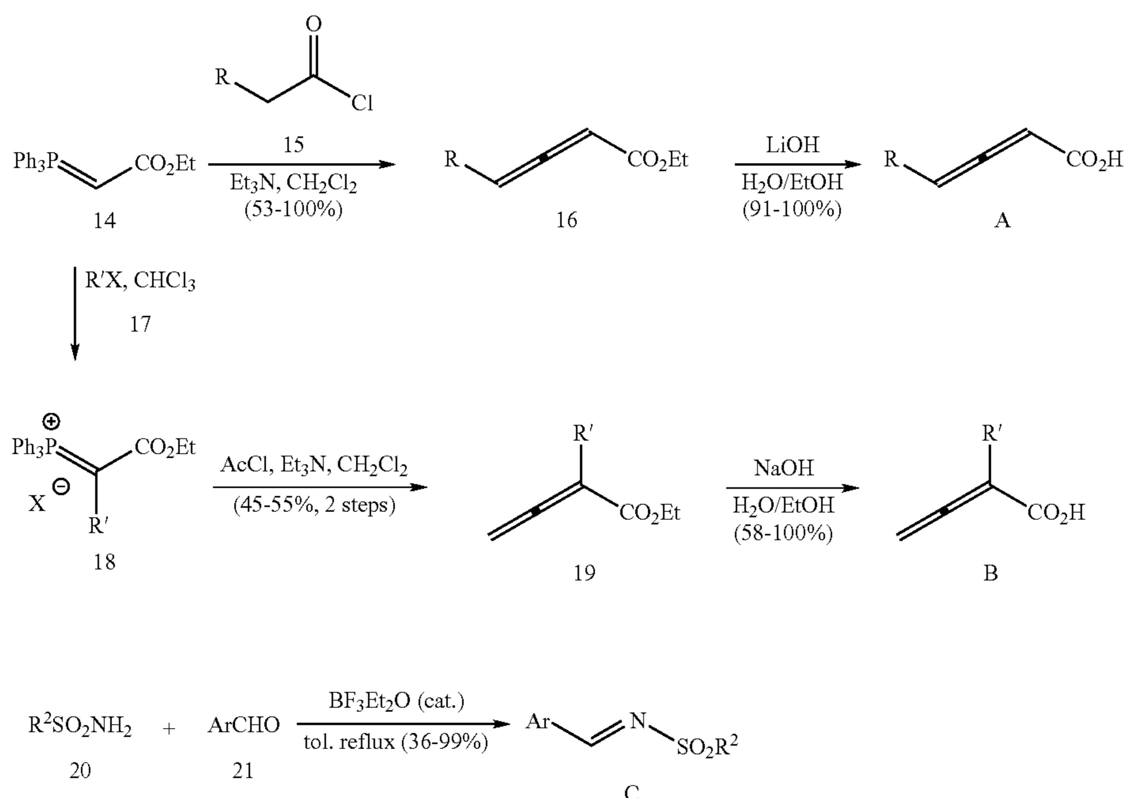
Scheme 3. Building block preparation.
