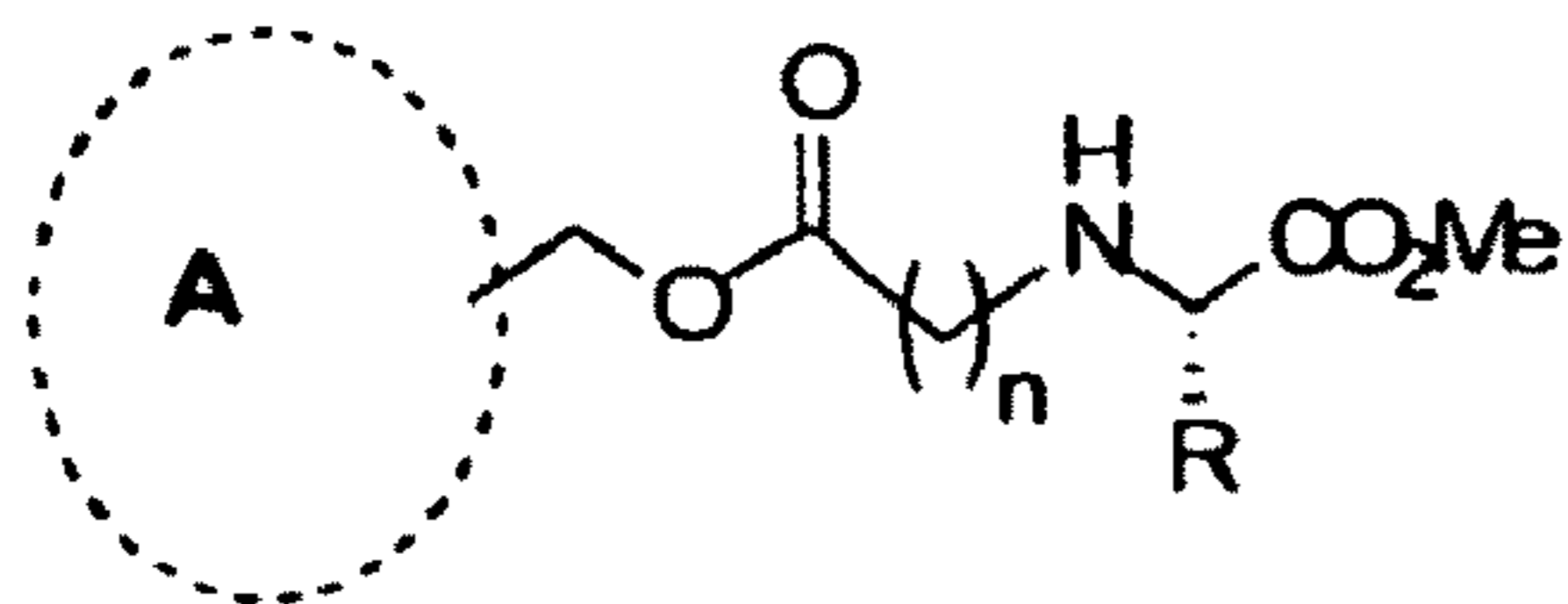
General structure of the third generation GGTLs
