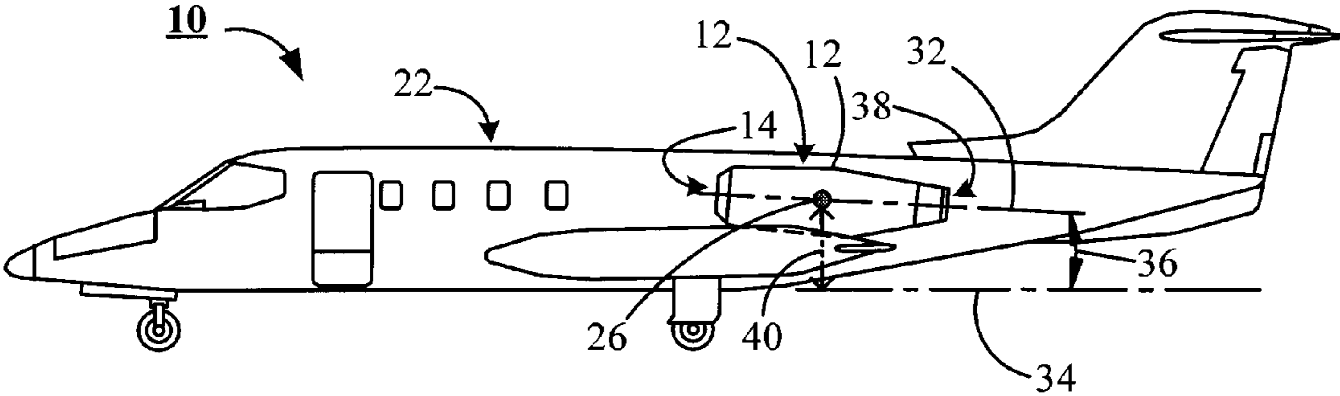
FIG. 2 PRIOR ART
