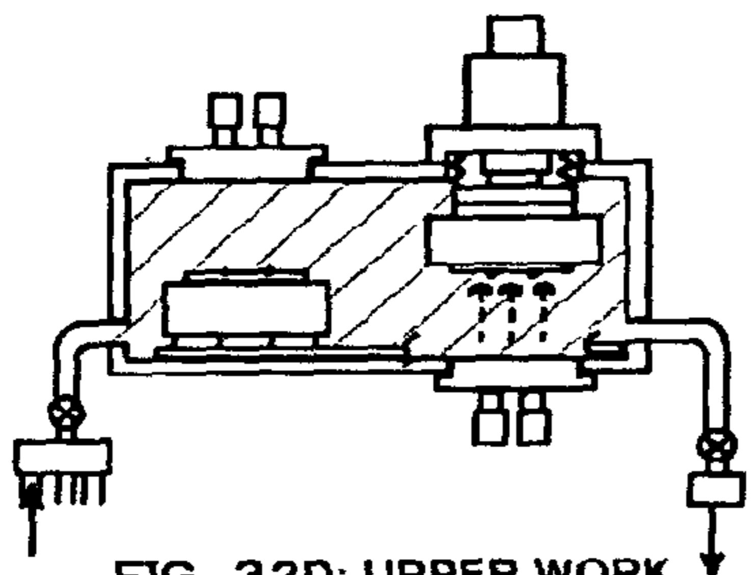
FIG. 32D: UPPER WORK PLASMA TREATMENT
