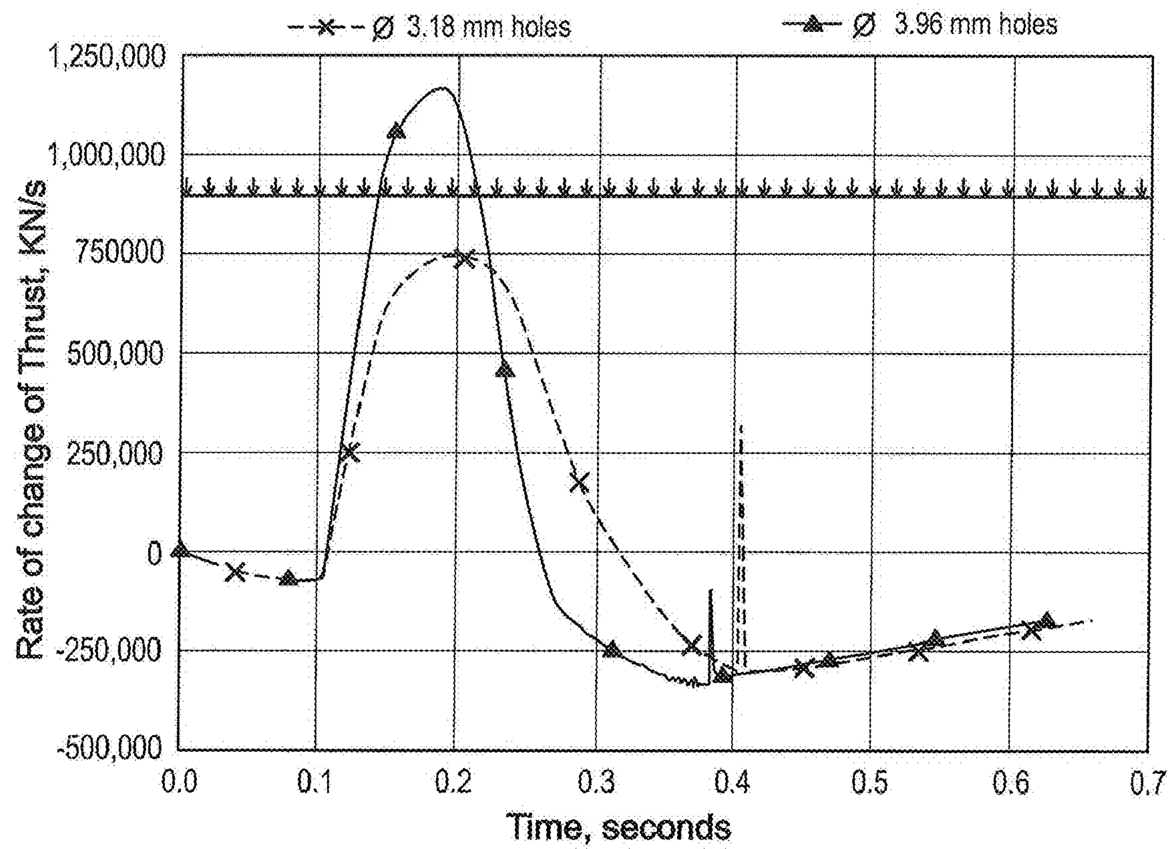
Force Rate of Change Plot
