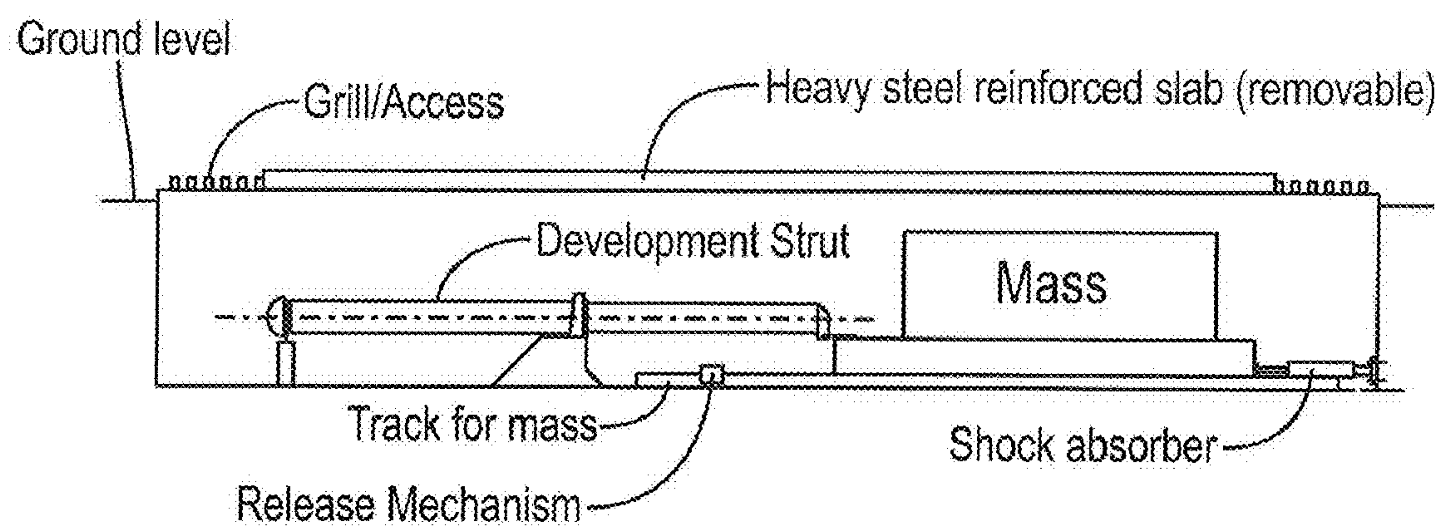
MAG Strut Performance Development Test Set-up
