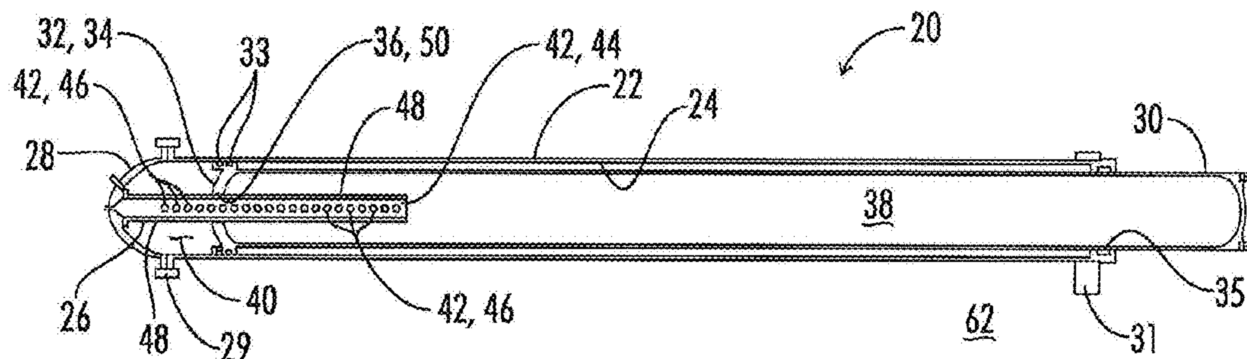
Schematic of the Proposed MAG Strut Design
