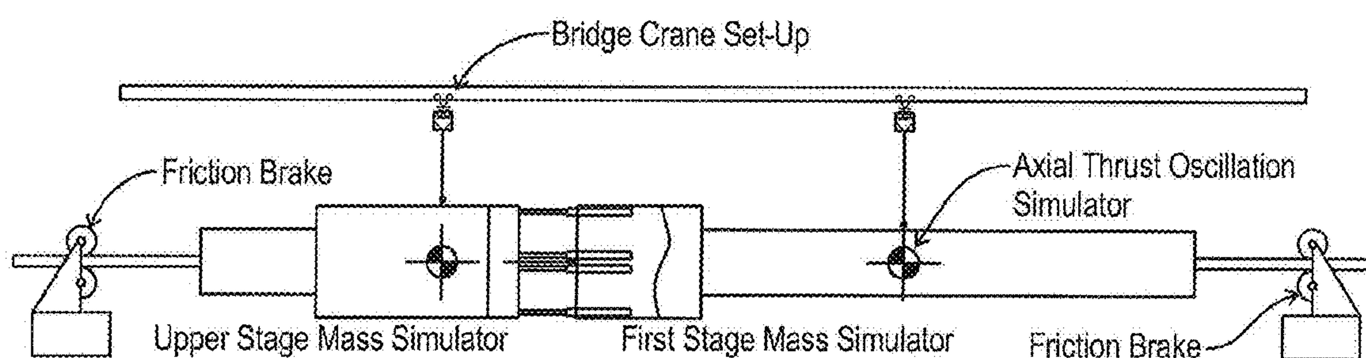
System demonstration test set up
