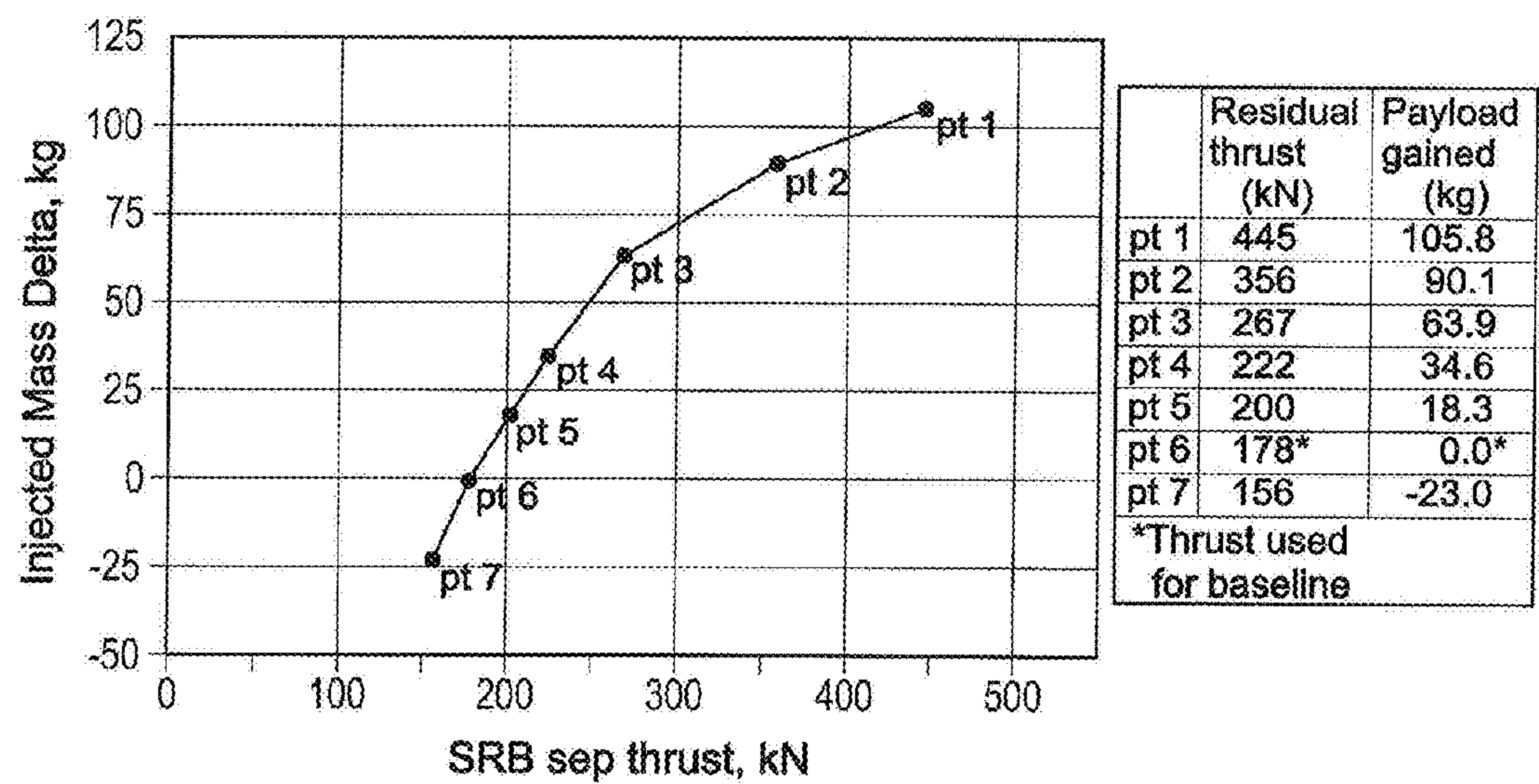
Payload Delta from Baseline vs. Separation Thrust
