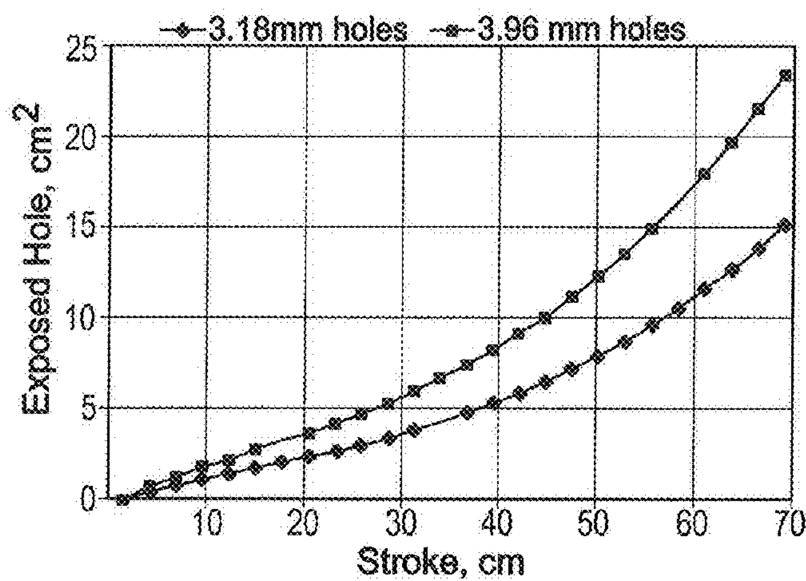
Exposed Hole Area for Two Candidate Hole-Patterns
