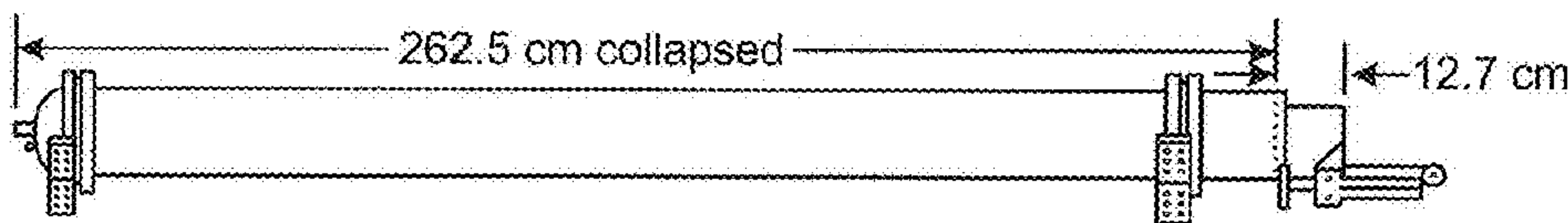
Strut Rendering (Collapsed)M
