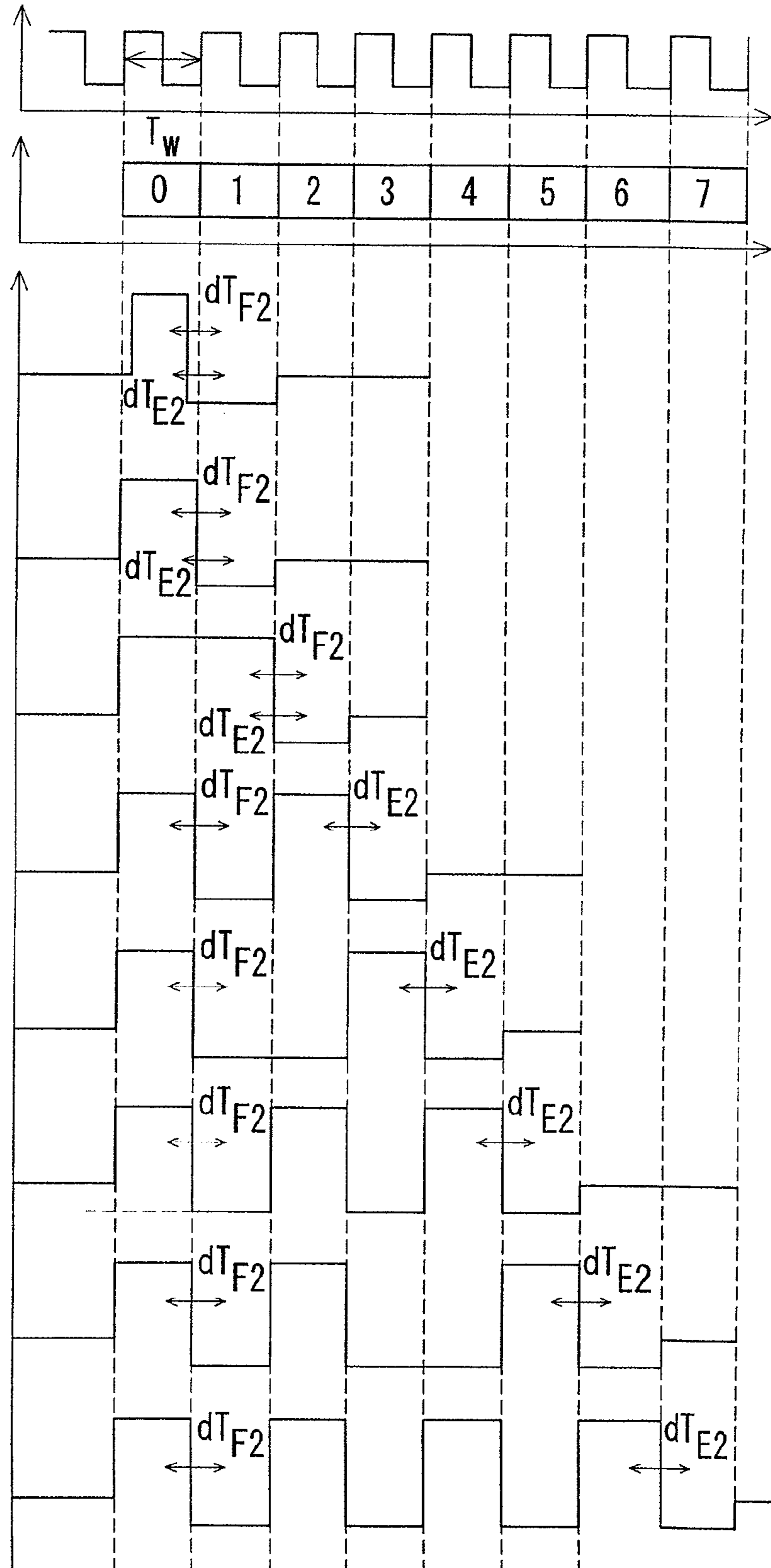
Fig. 10A 128 REFERENCE-TIME SIGNAL
