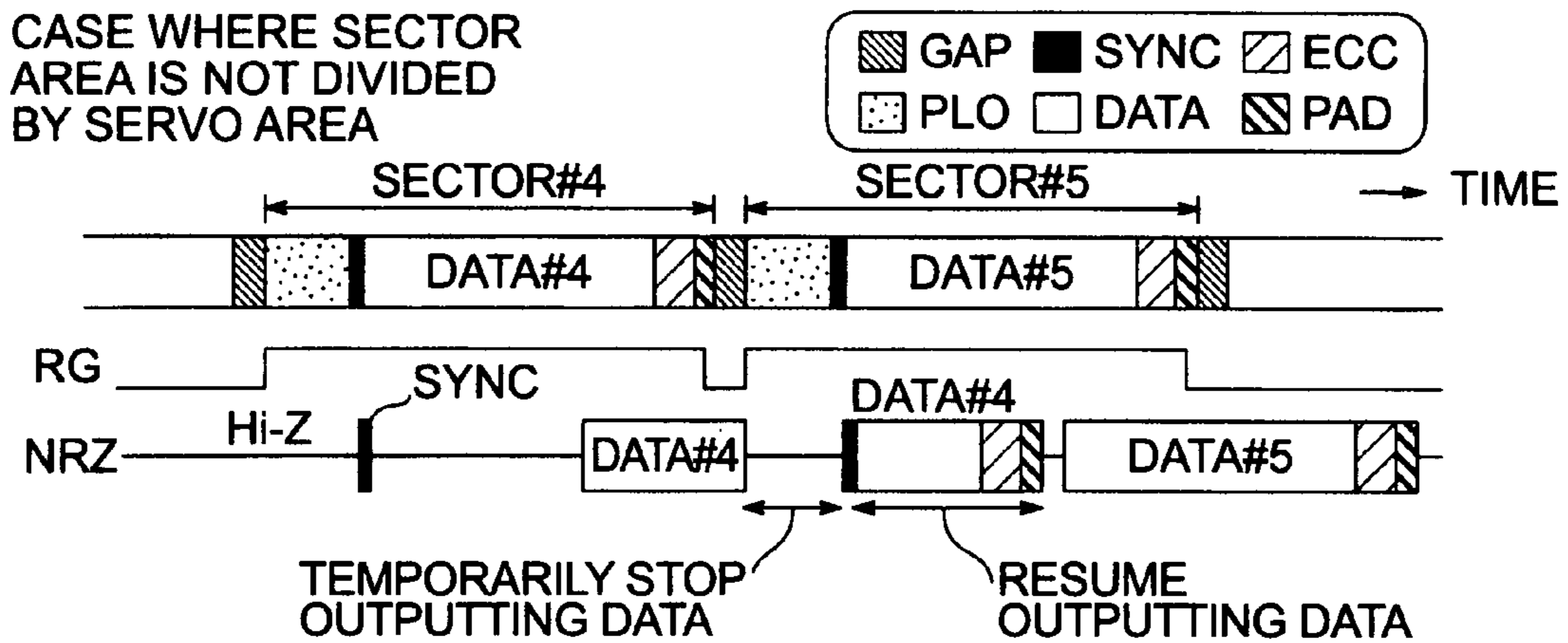
CASE WHERE SECTOR AREA IS DIVIDED BY SERVO AREA FIG. 9B
