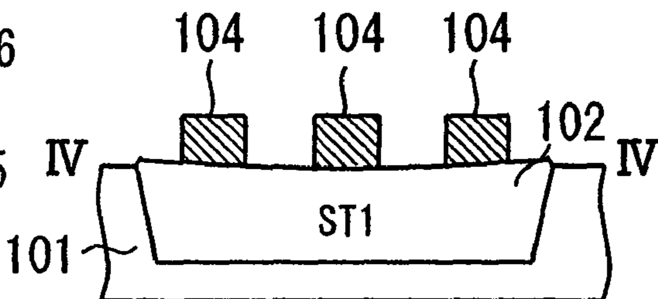
Fig. 13C (PRIOR ART)
