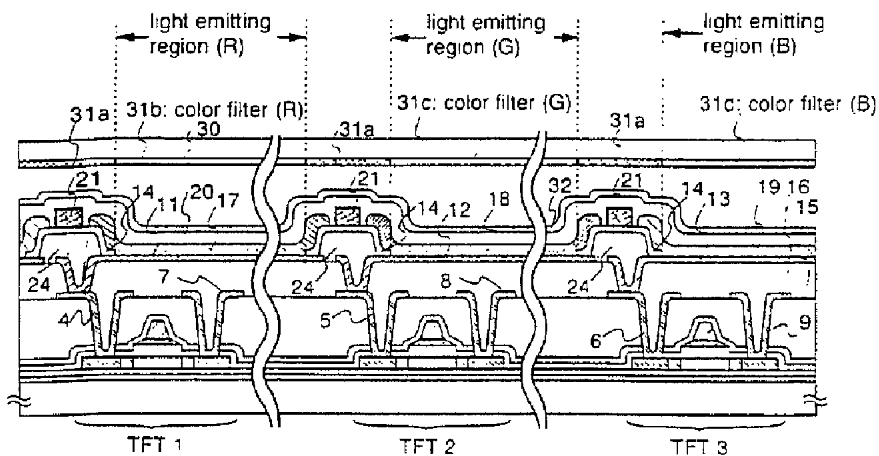
FIG. 1B sectional view of B-B'
