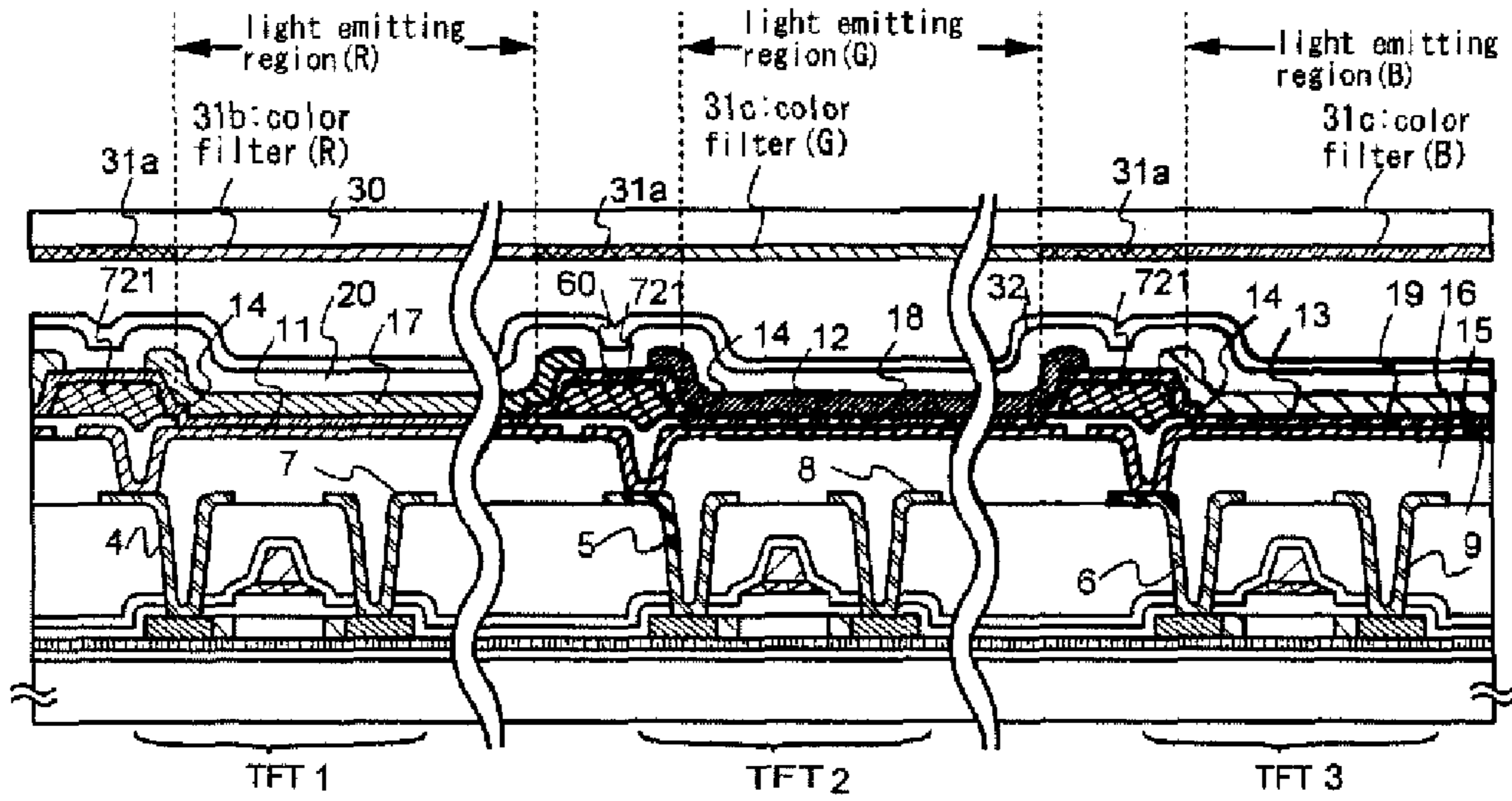
FIG.9B sectional view of B-B'
