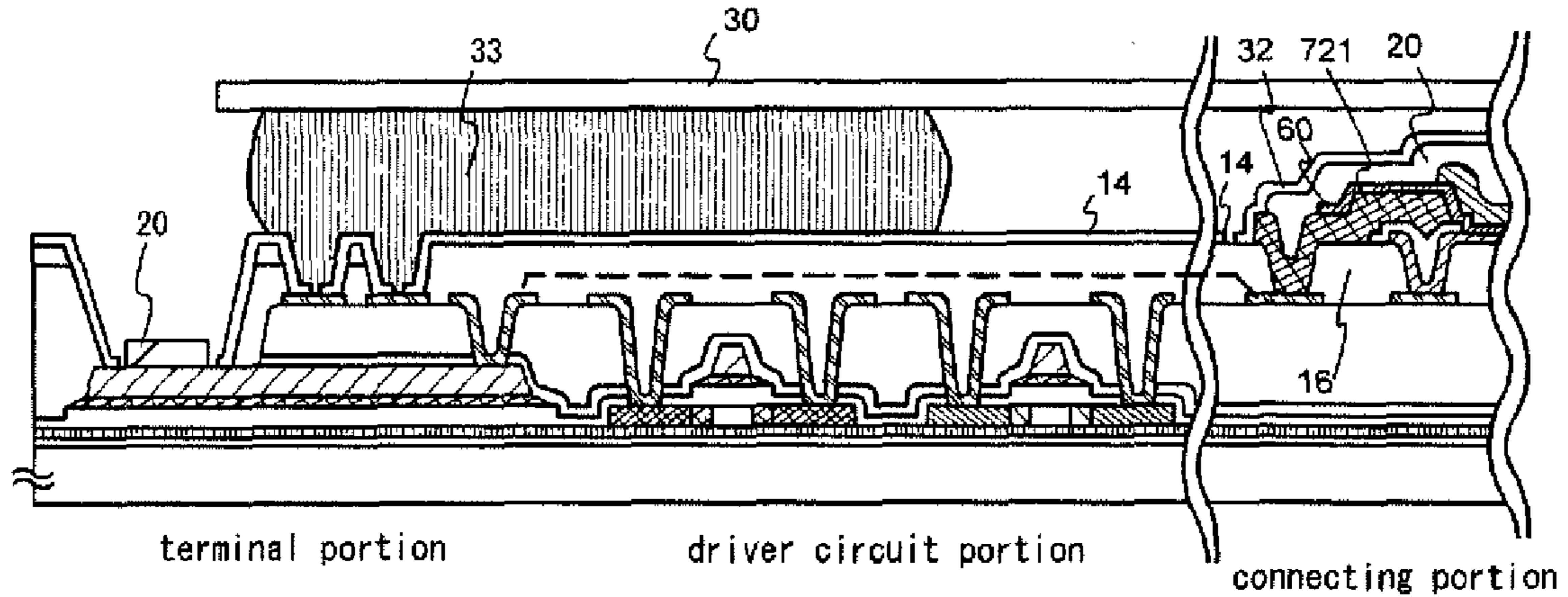
FIG.9C sectional view of C-C'
