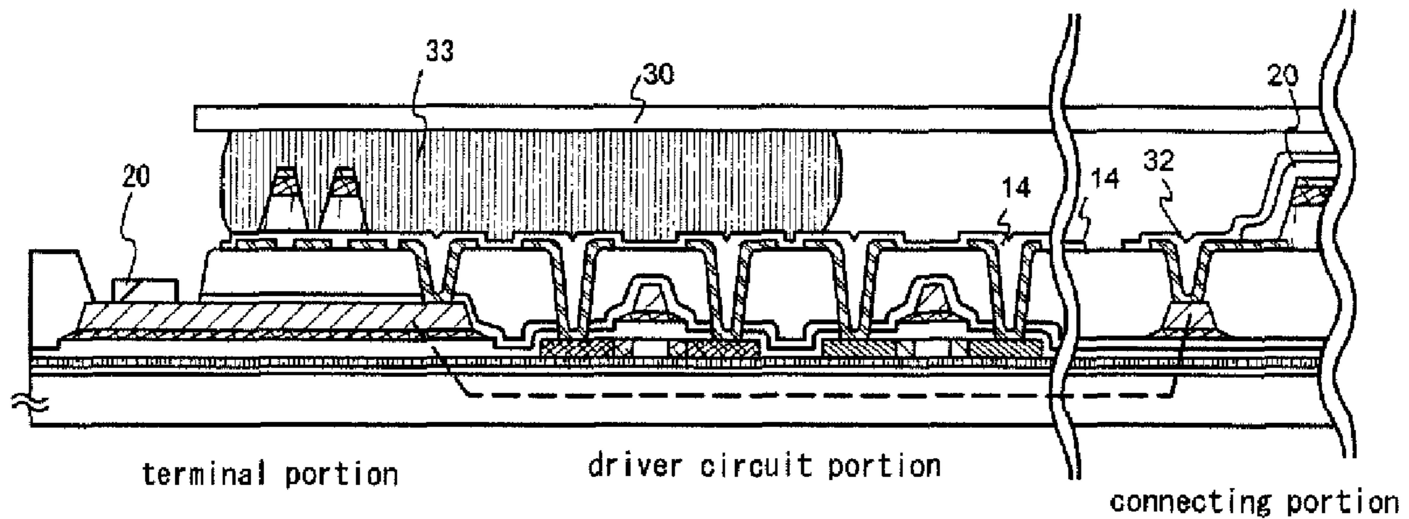
FIG.6C sectional view of C-C'
