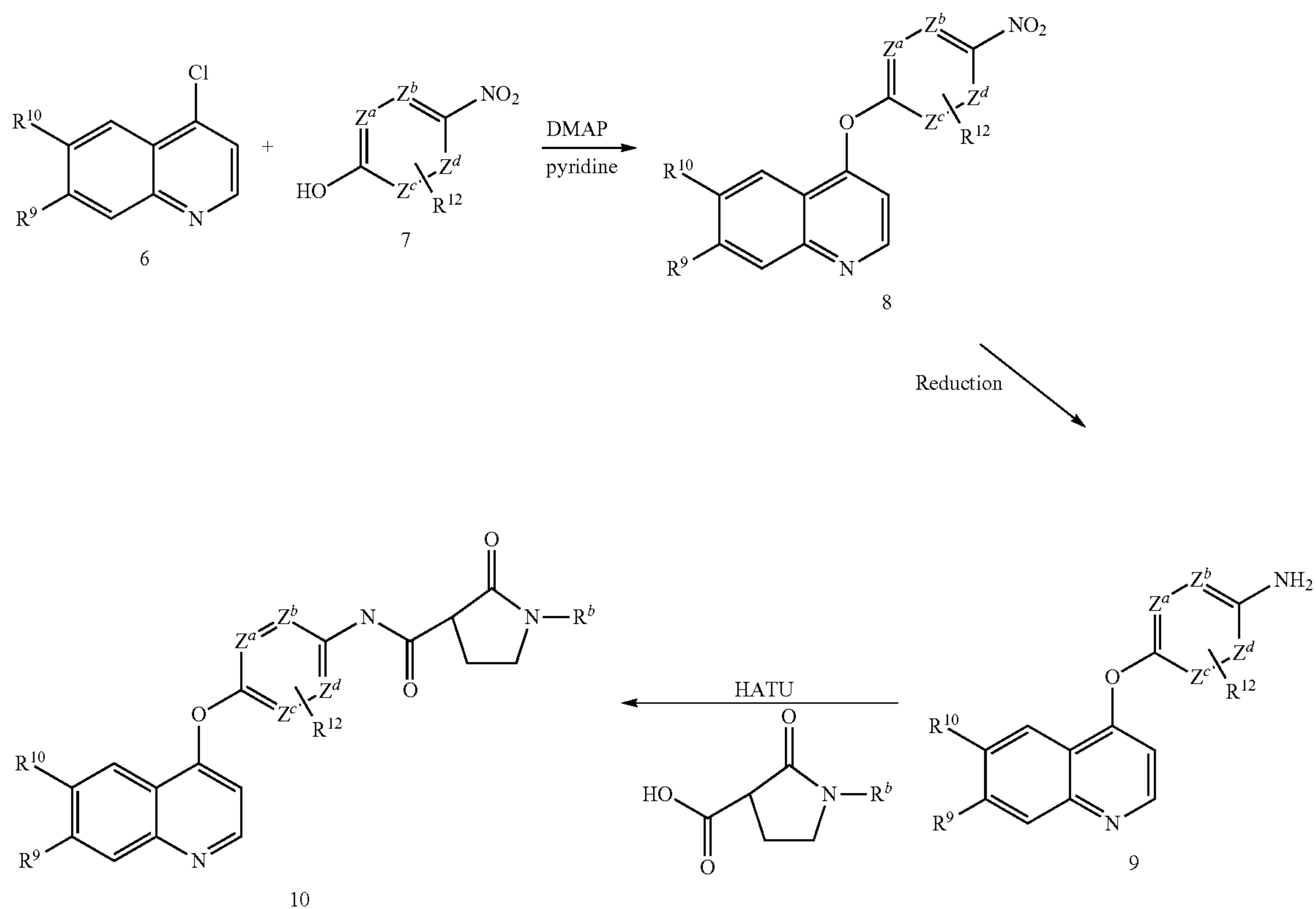
Scheme 2
