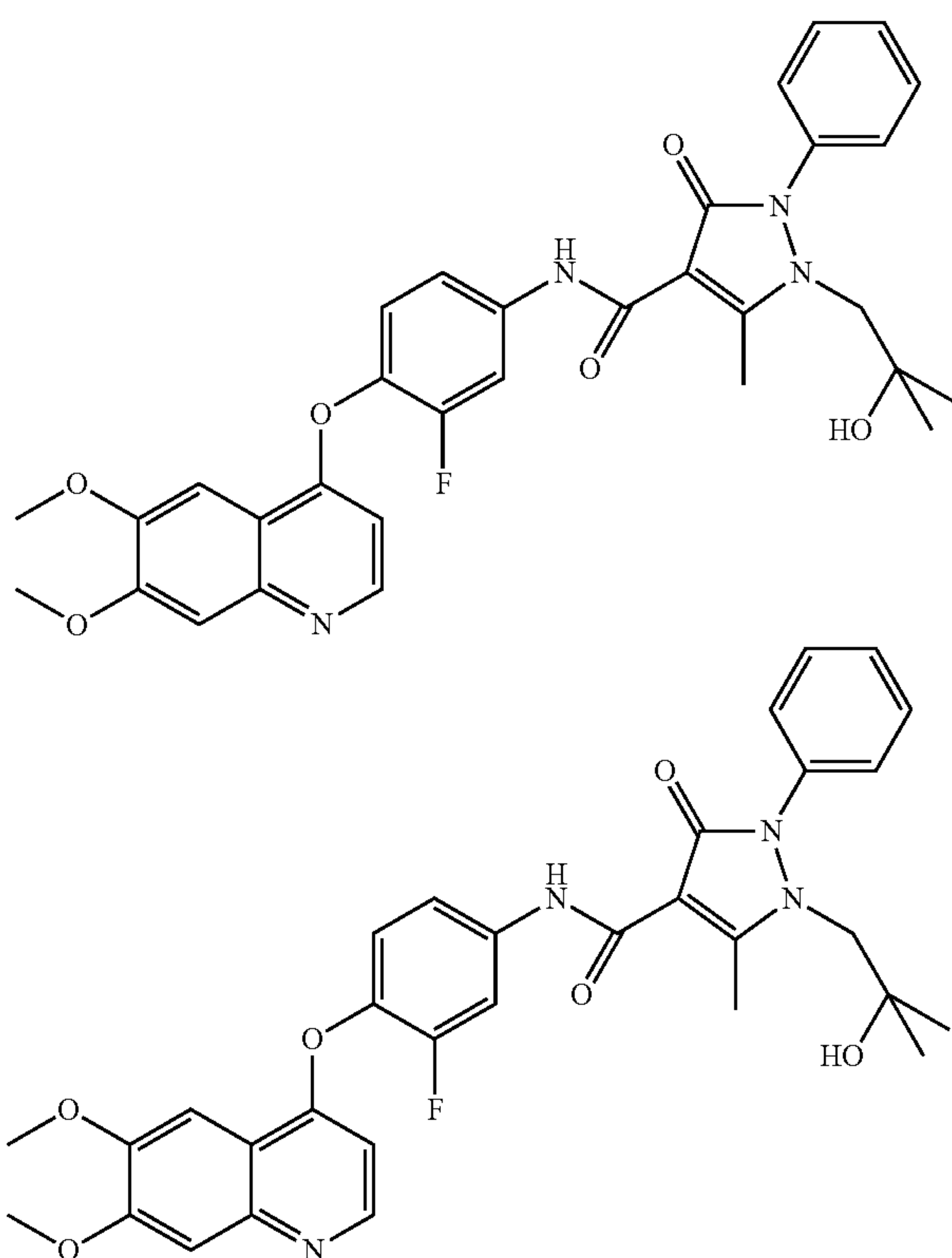
N-(4-(6,7-dimethoxyquinolin-4-yloxy)-3-fluorophenyl)-1-(2-hydroxy-2-methylpropyl)-5-methyl-3-oxo-2-phenyl-2,3-dihydro-1H-pyrazole-4-carboxamide
