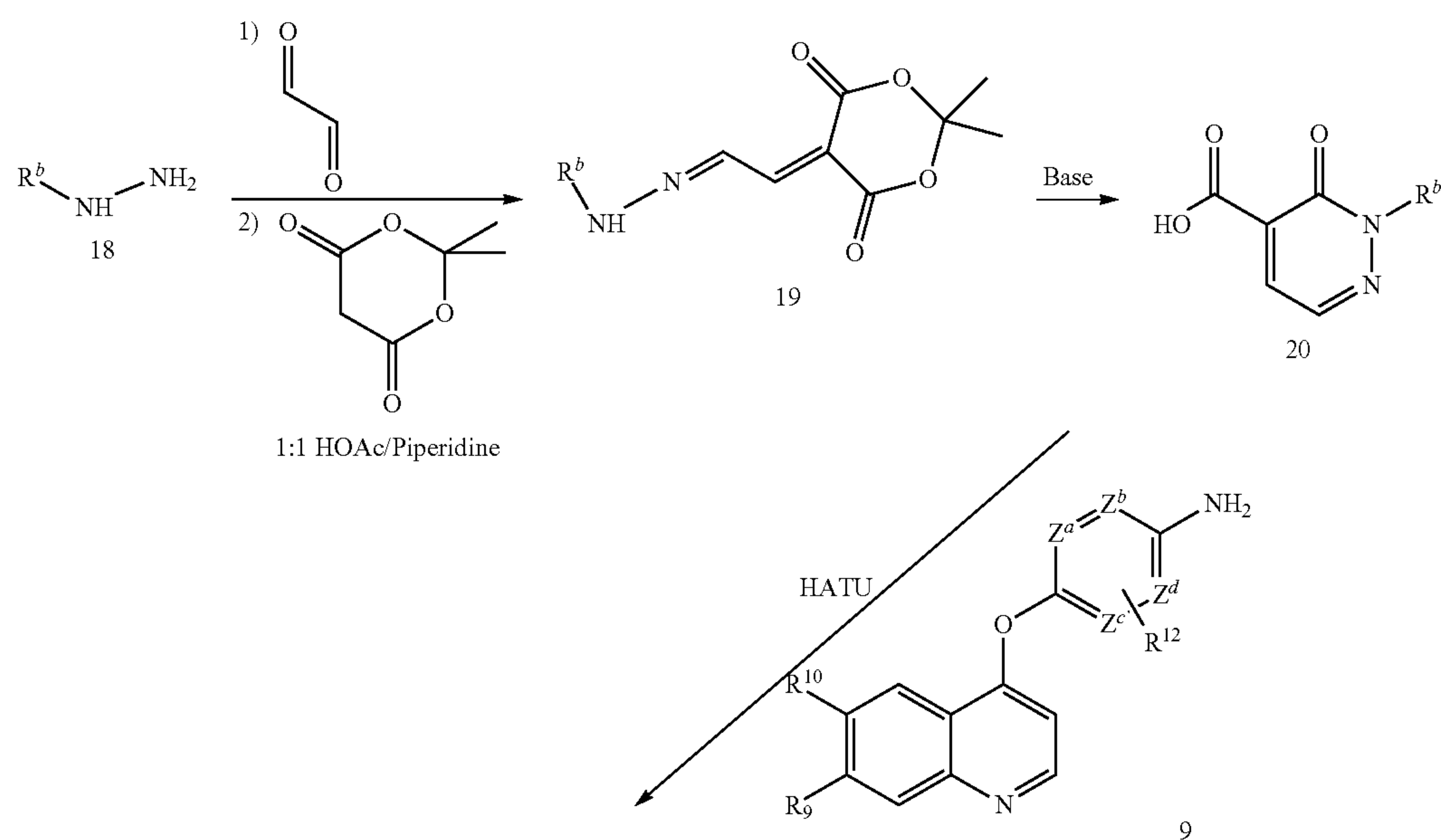
Scheme 5
