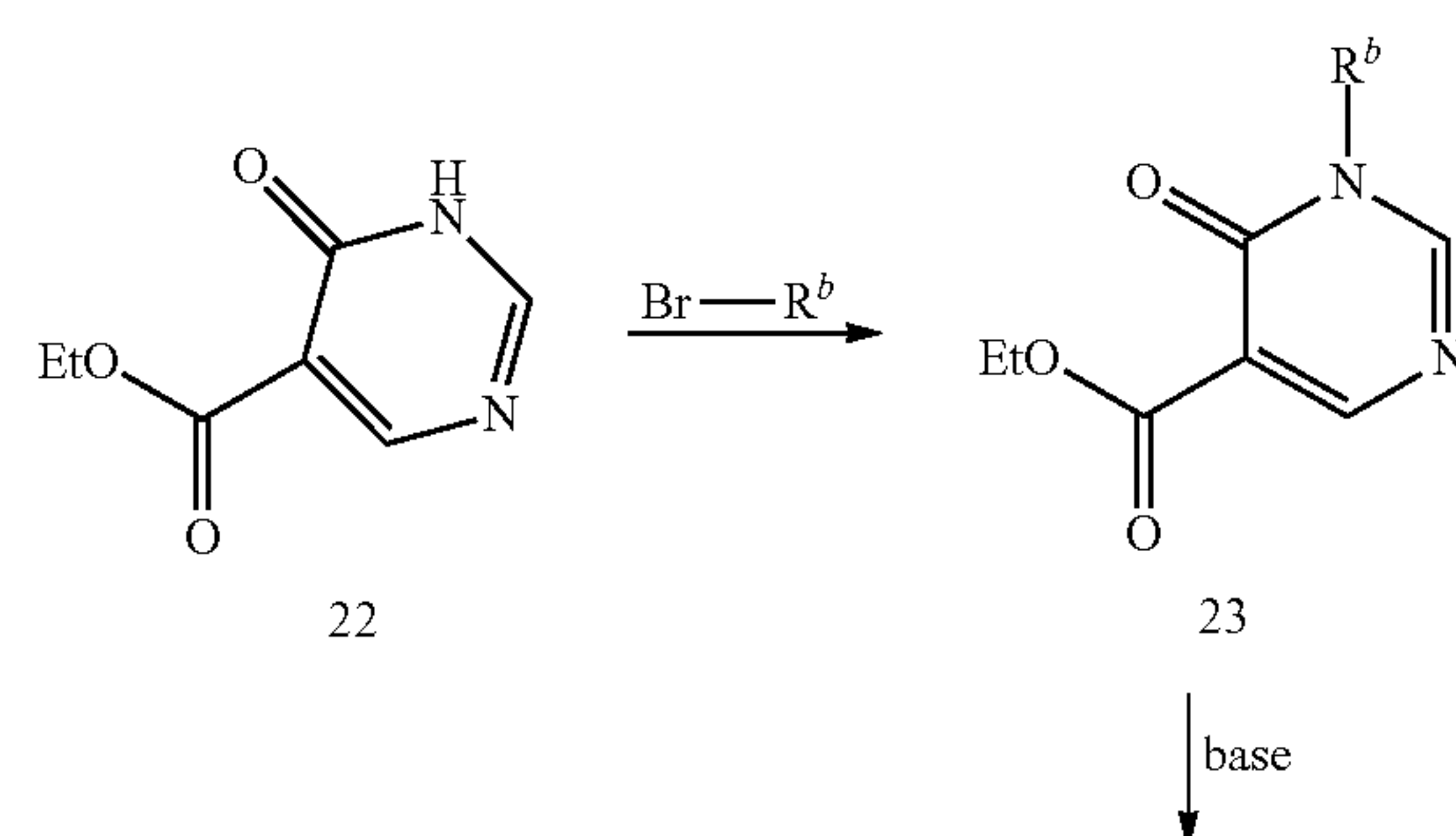
Scheme 6
