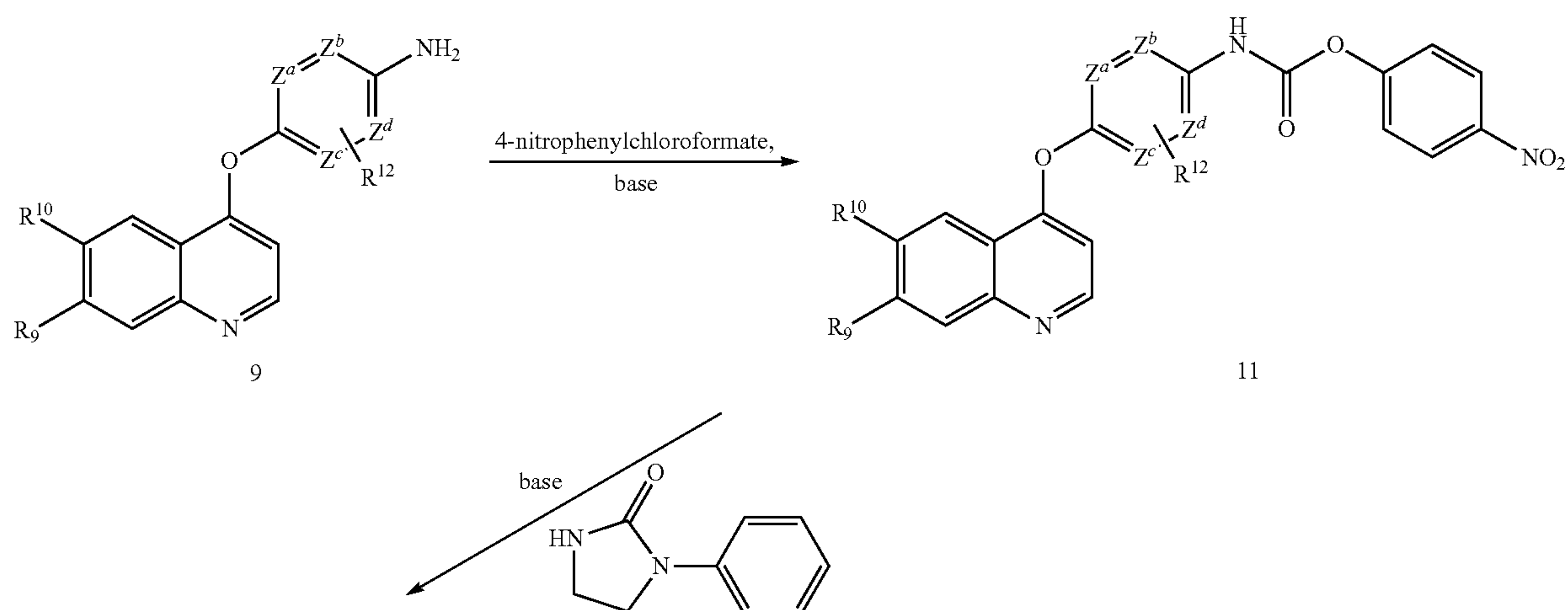
Scheme 3
