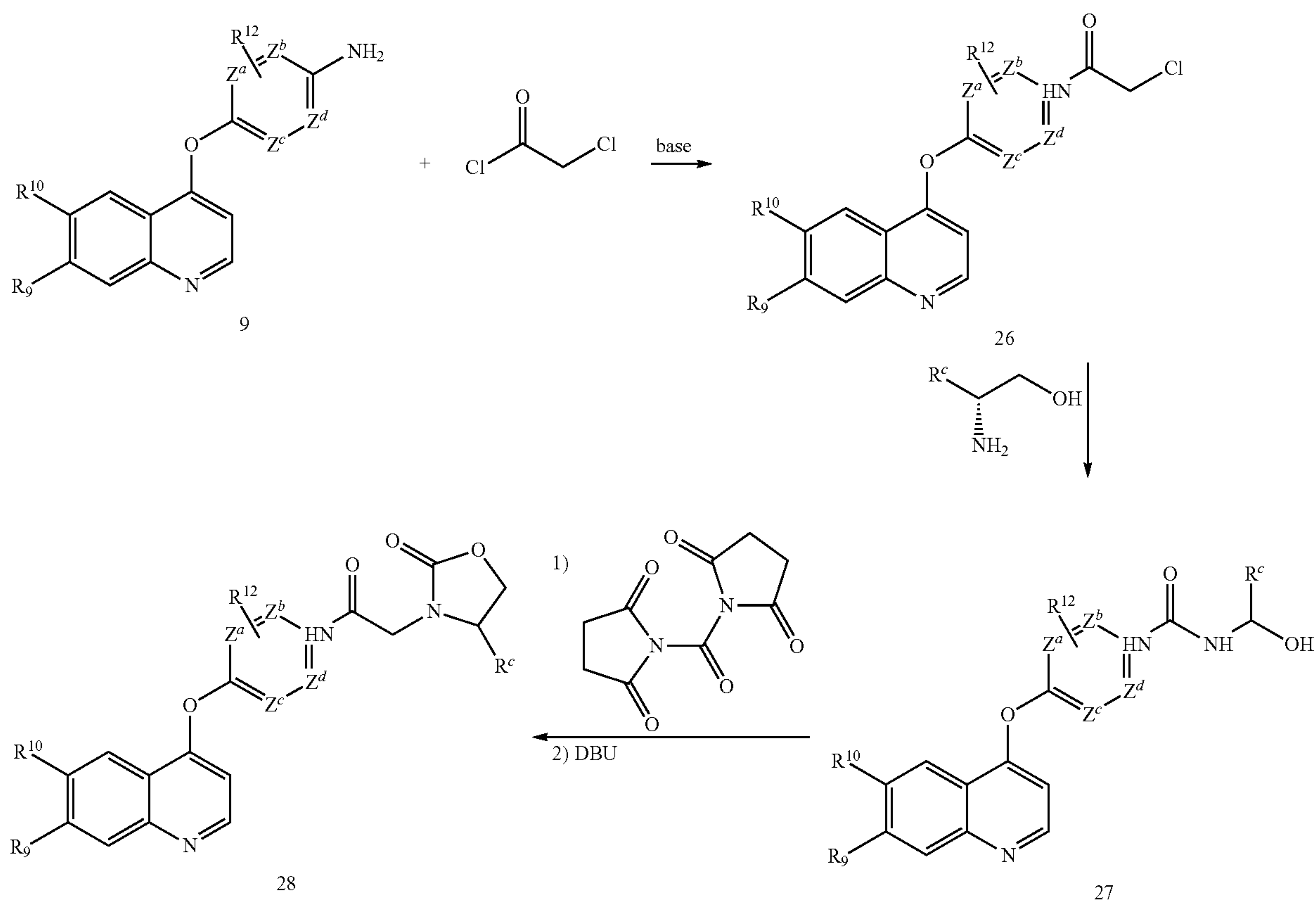
Scheme 7
