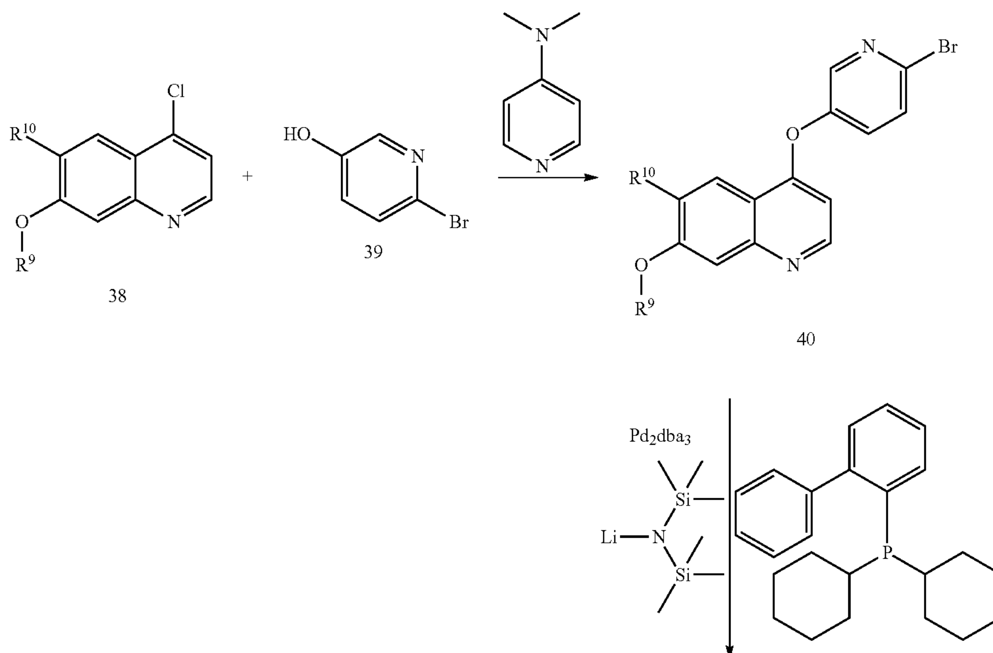
Scheme 10
