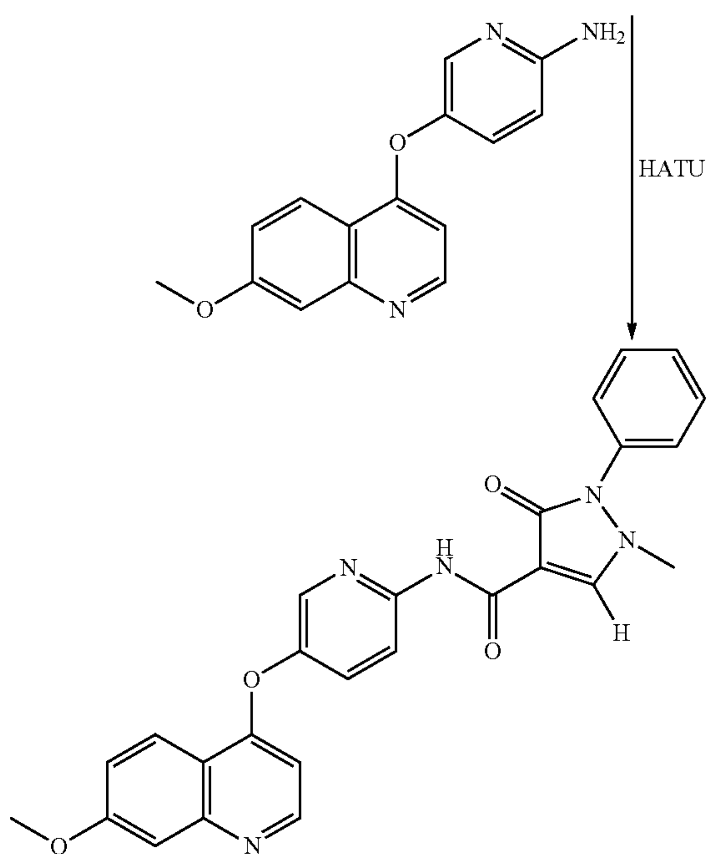
N-(5-(7-methoxyquinolin-4-yloxy)pyridin-2-yl)-1-methyl-3-oxo-2-phenyl-2,3-dihydro-1H-pyrazole-4-carboxamide
