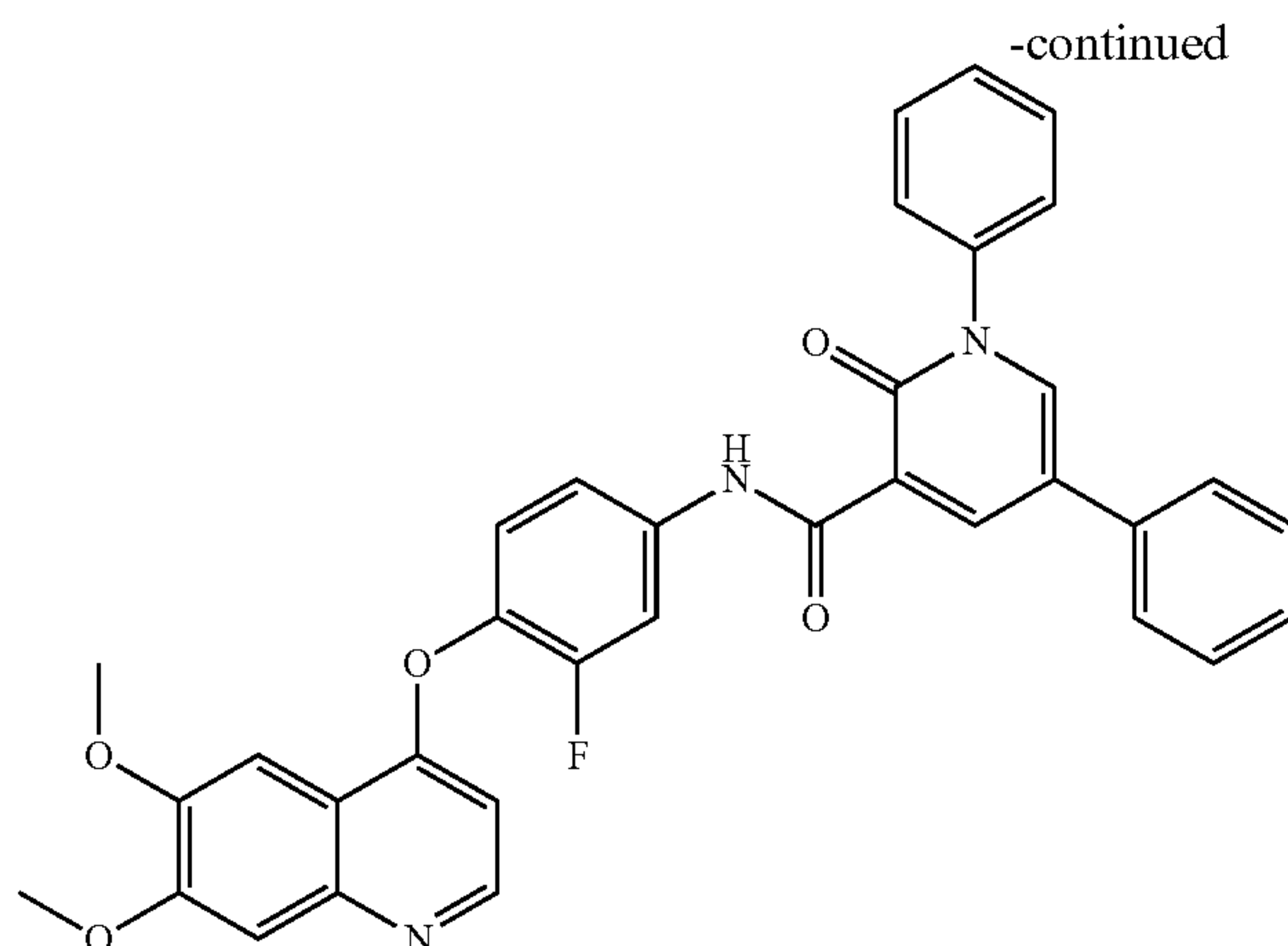
N-(4-(6,7-dimethoxyquinolin-4-yloxy)-3-fluorophenyl)-2-oxo-1,5-diphenyl-1,2-dihydropyridine-3-carboxamide
