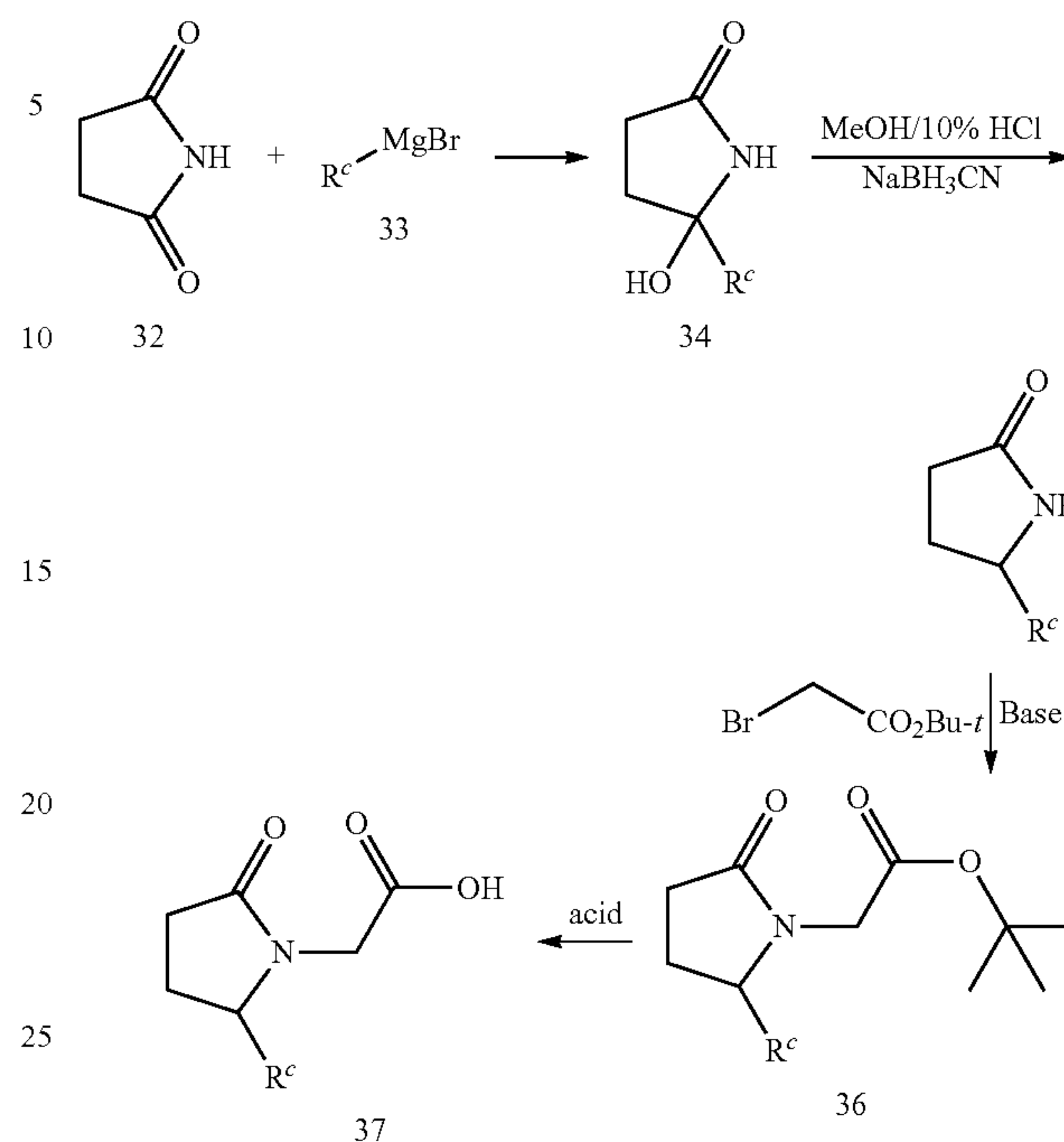
Scheme 9
