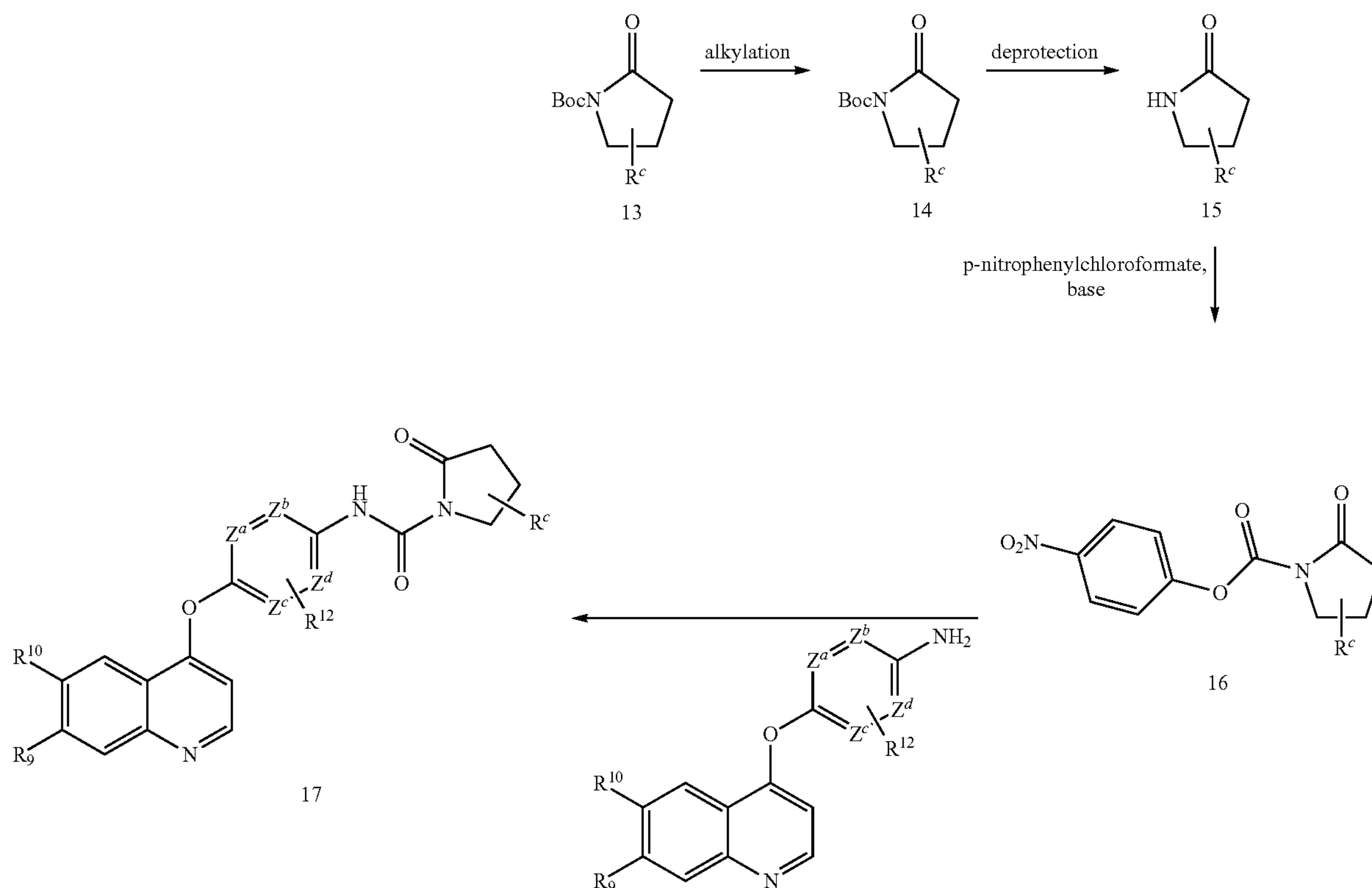
Scheme 4
