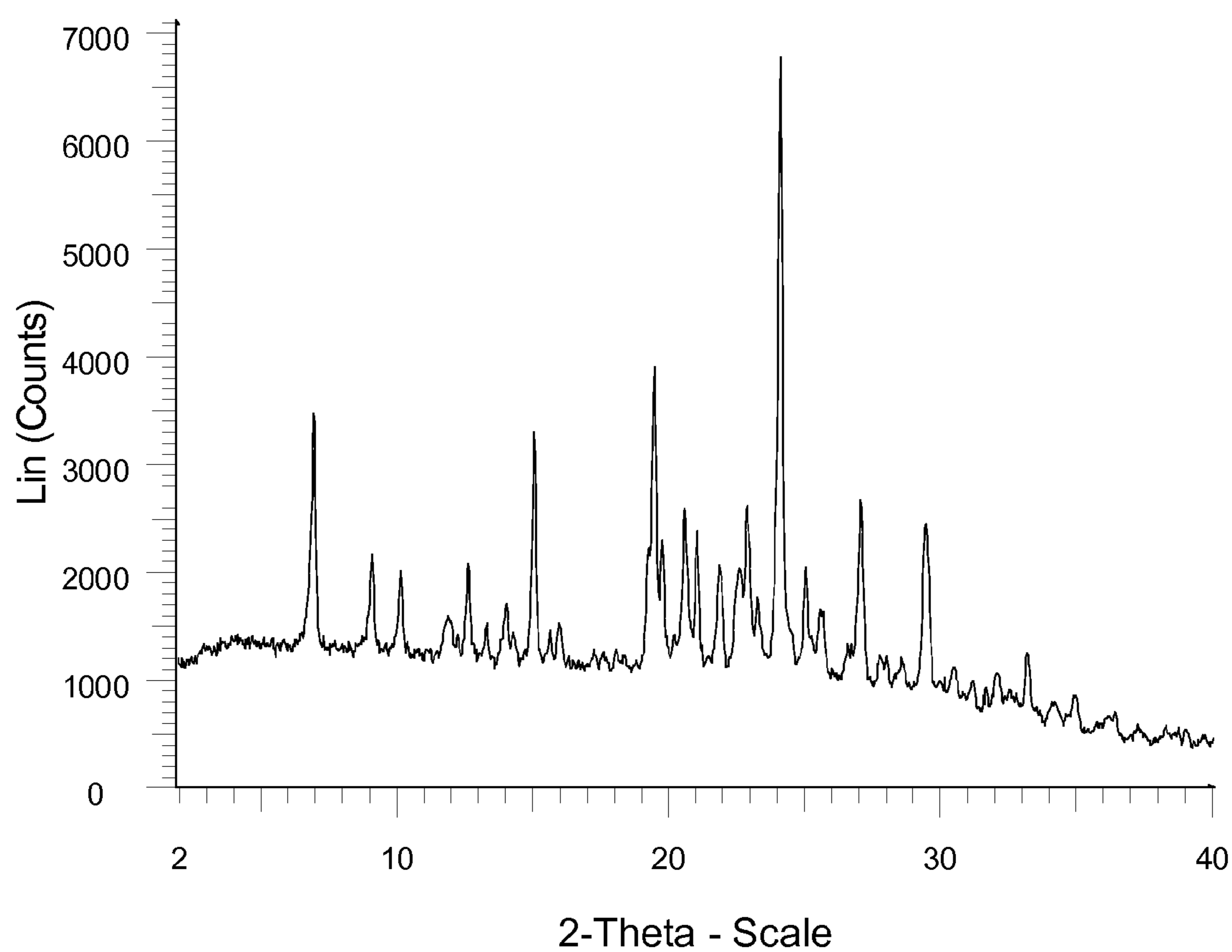
Powder X-ray diffraction pattern of Compound (I) difumarate Form C
