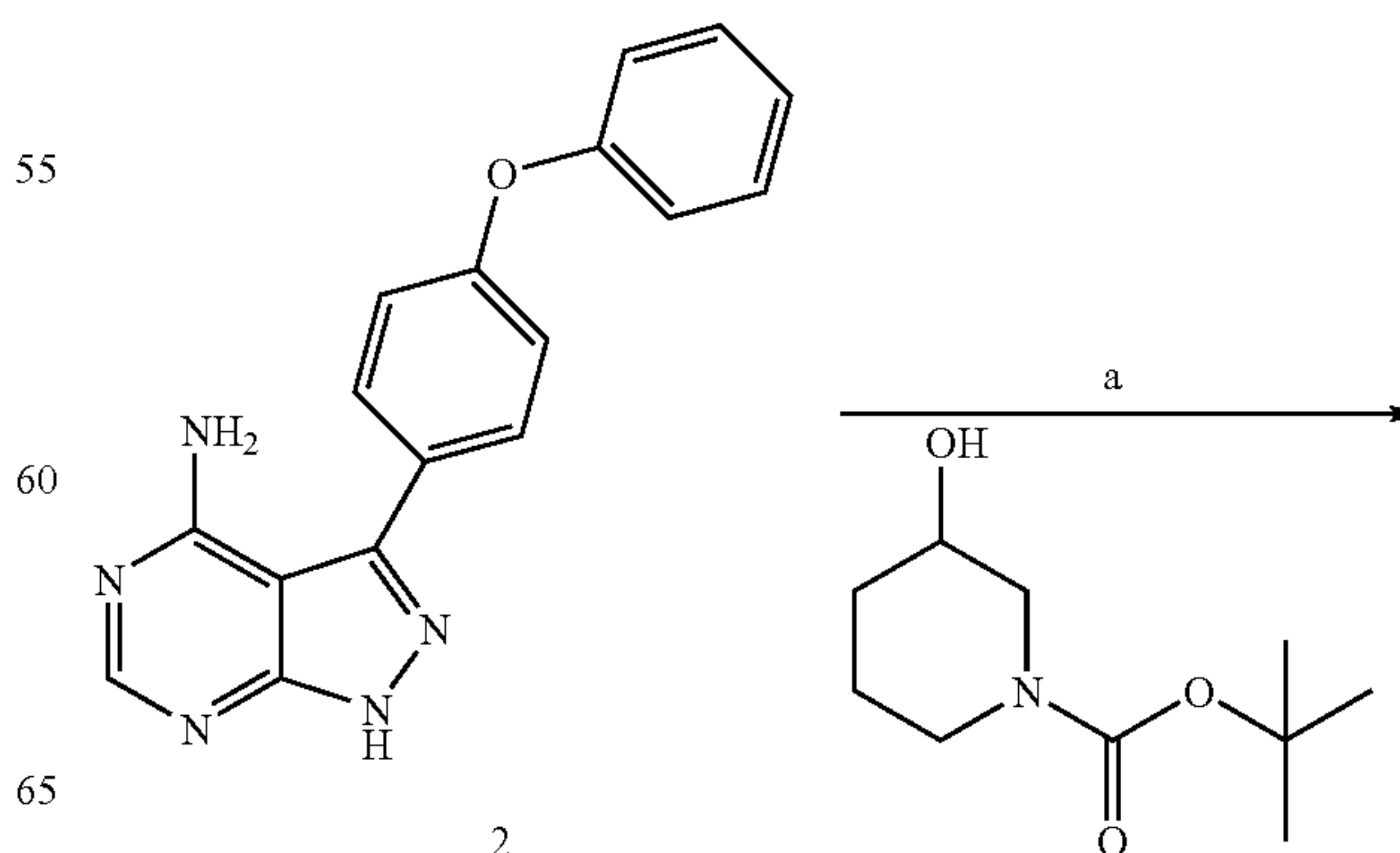
Scheme 1.
