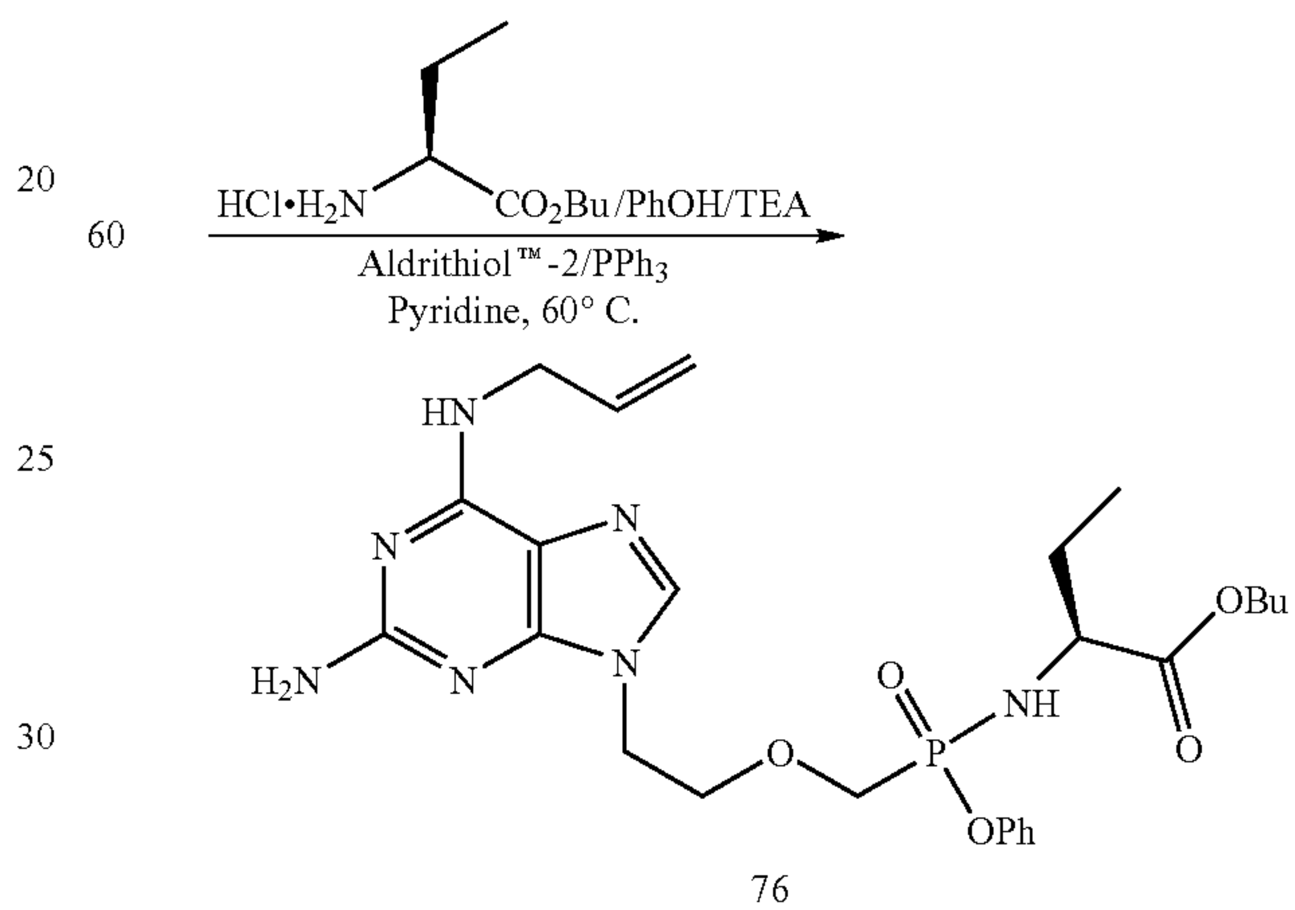
Scheme 21
