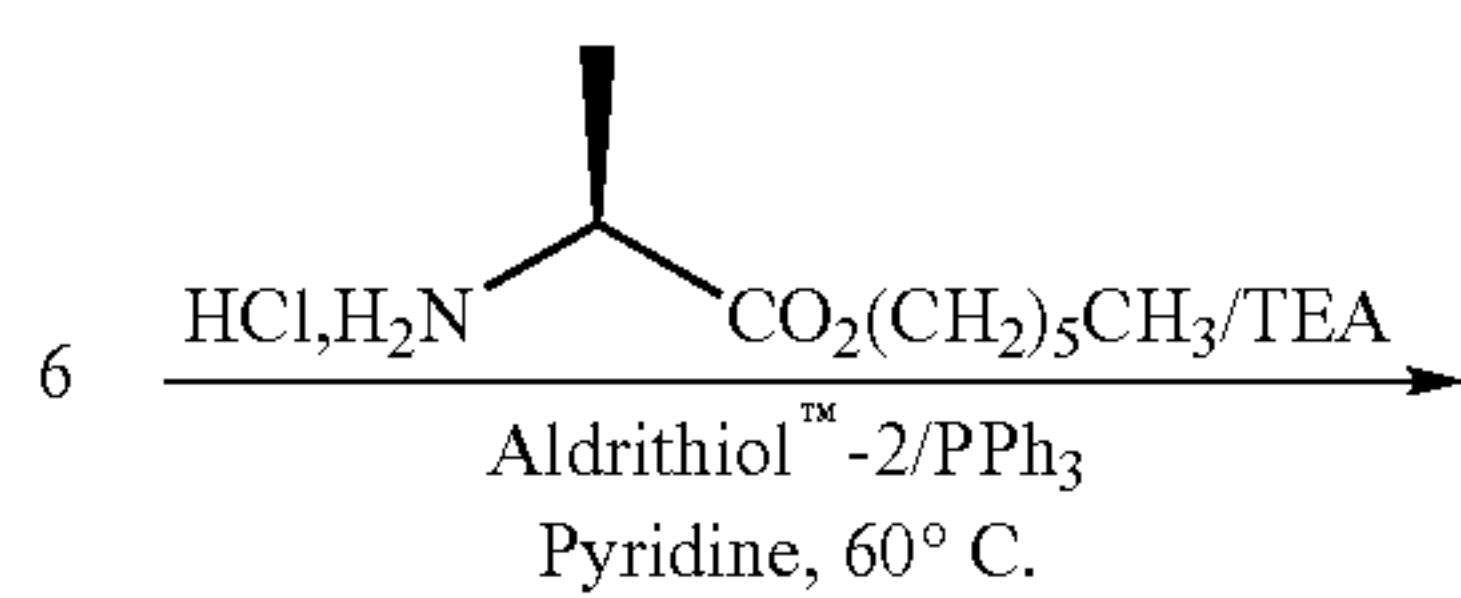
Scheme 7
