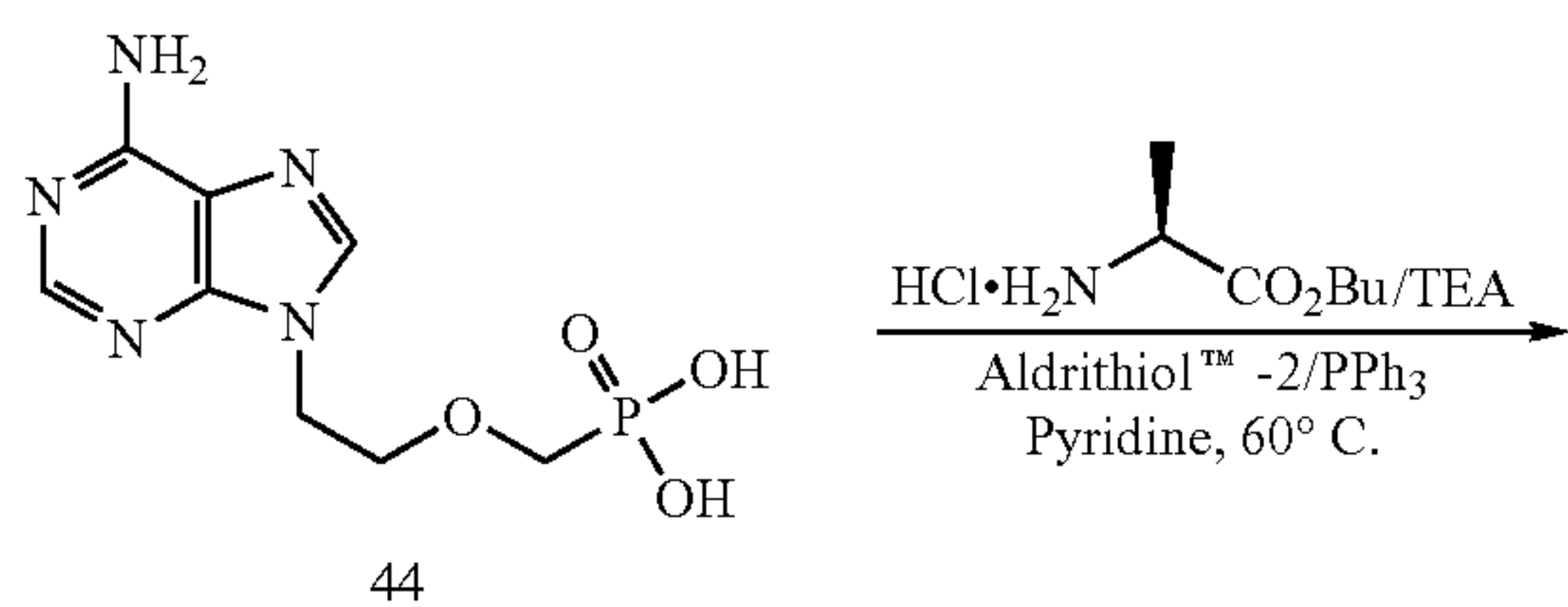
Scheme 13
