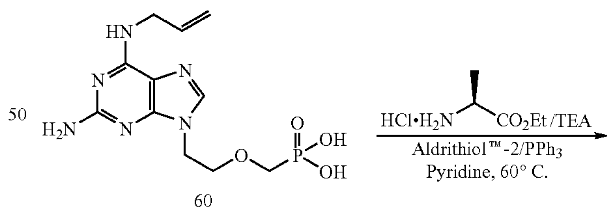
Scheme 18
