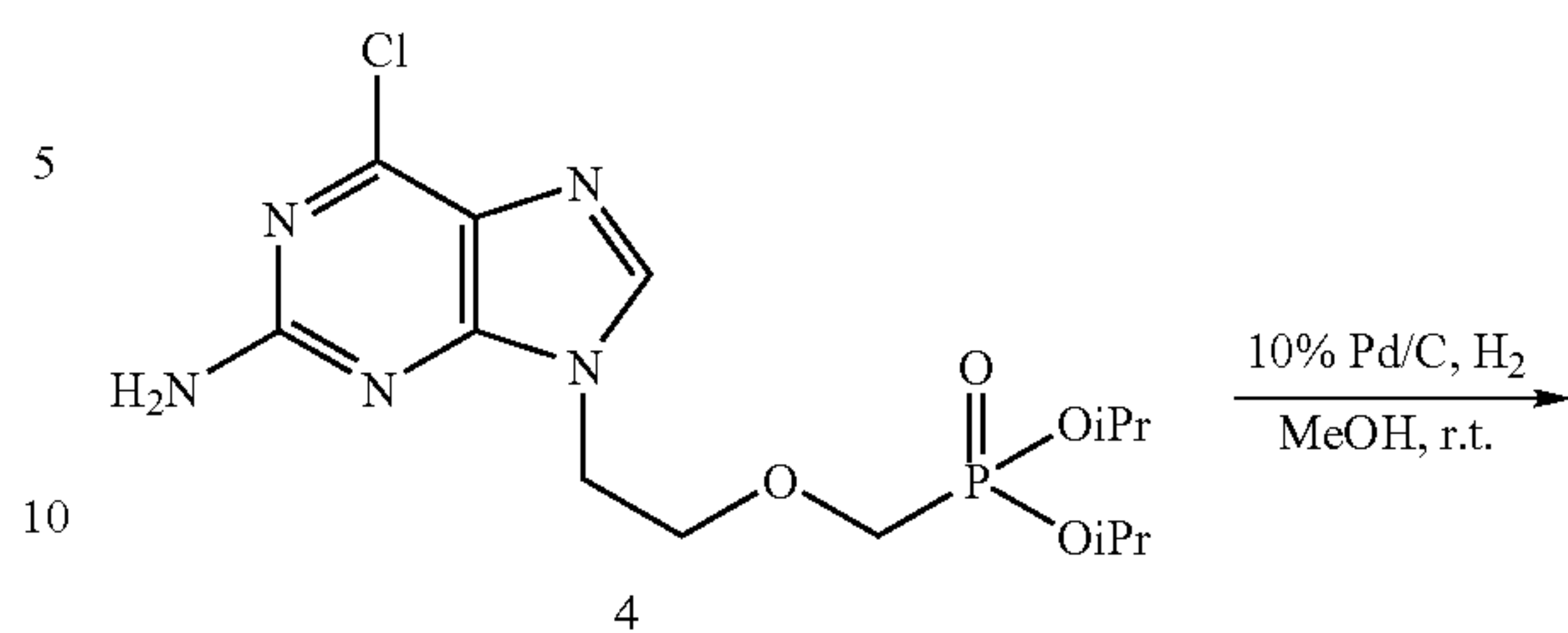
Scheme 15
