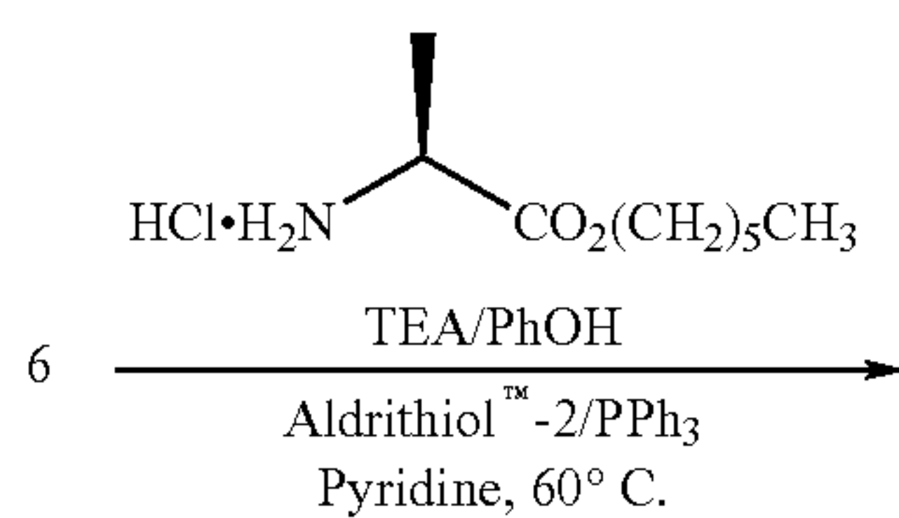
Scheme 4
