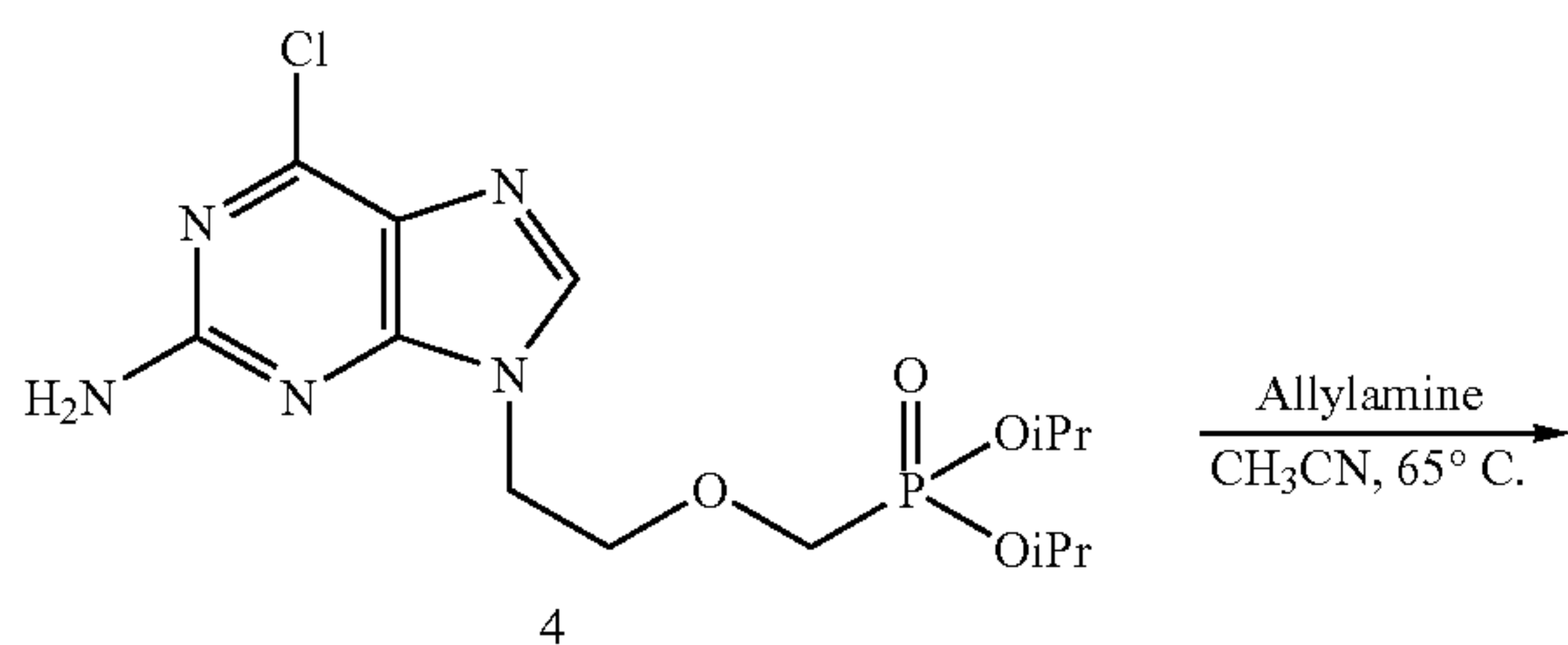
Scheme 16
