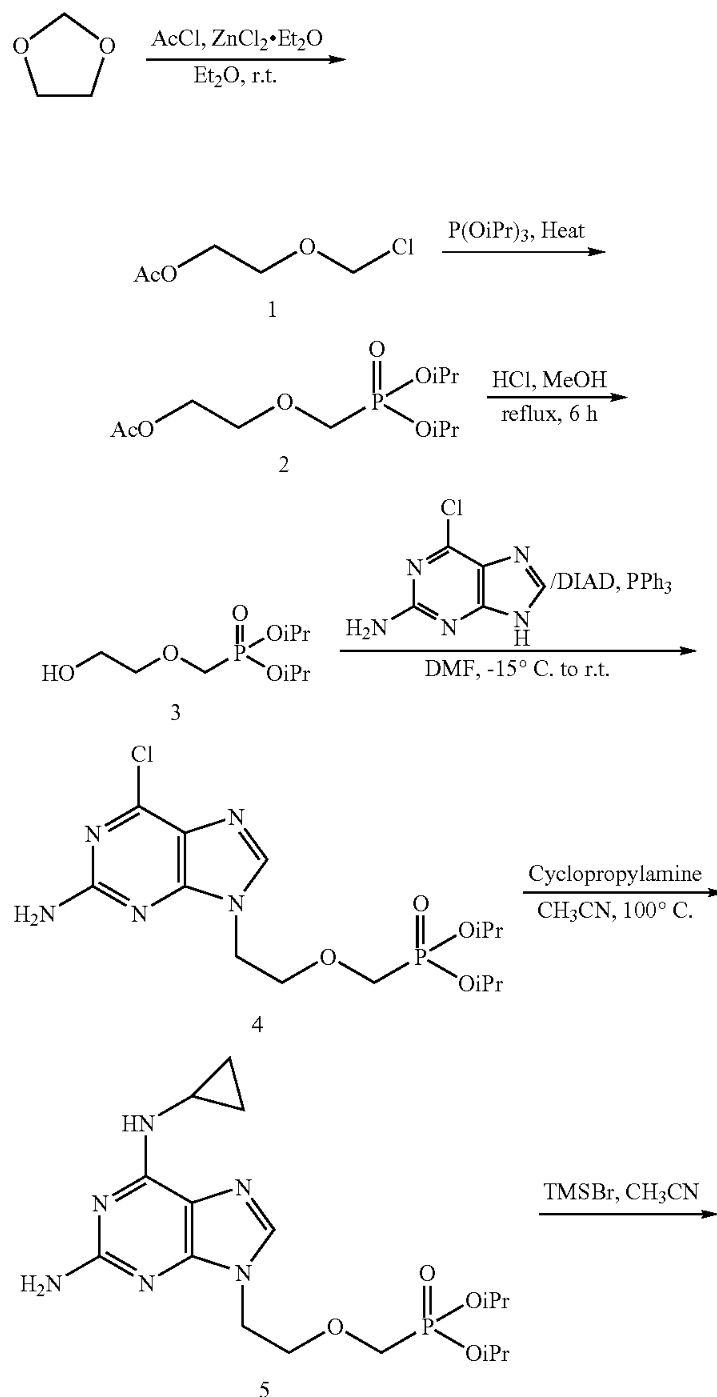
Scheme 1
