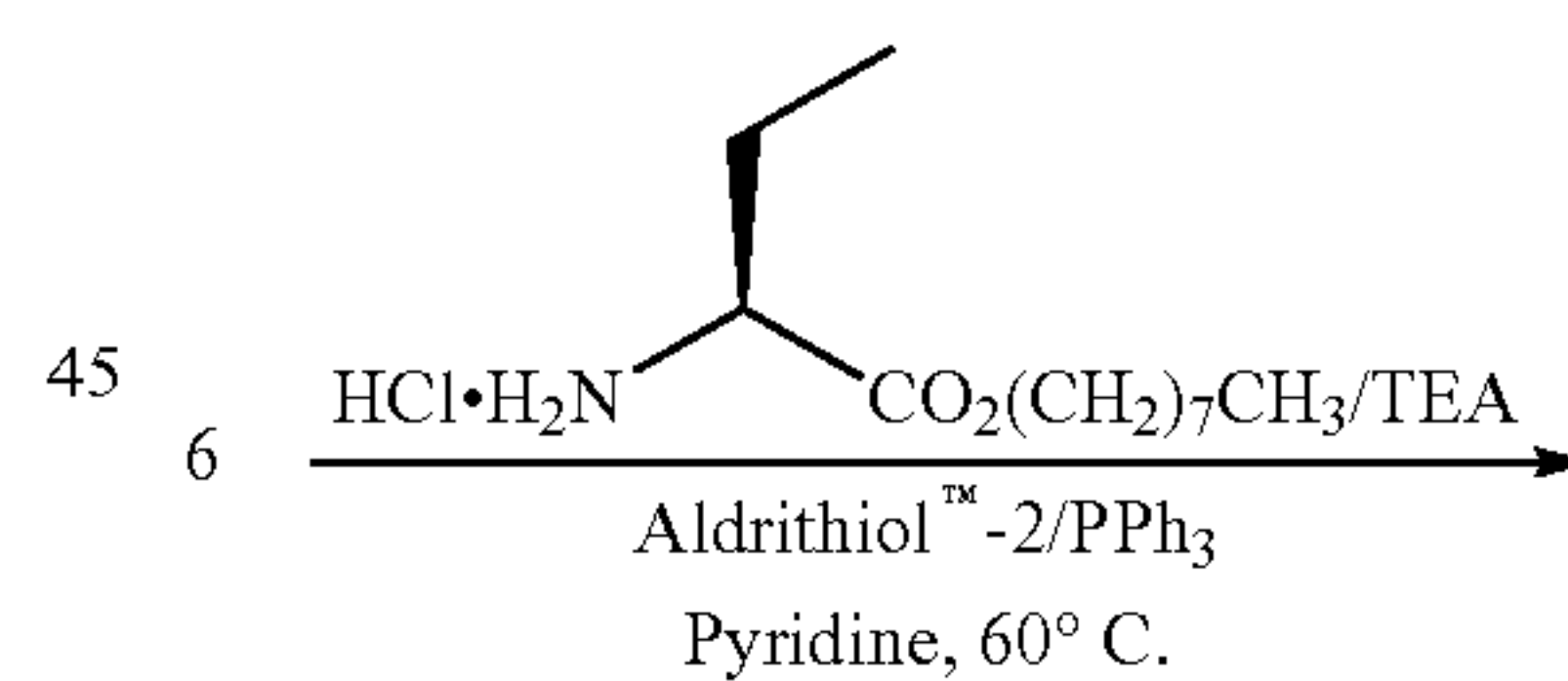
Scheme 8
