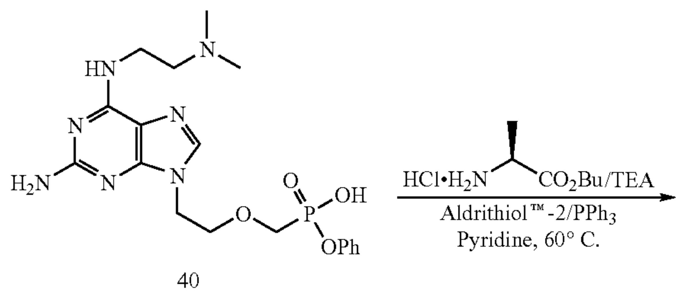
Scheme 11
