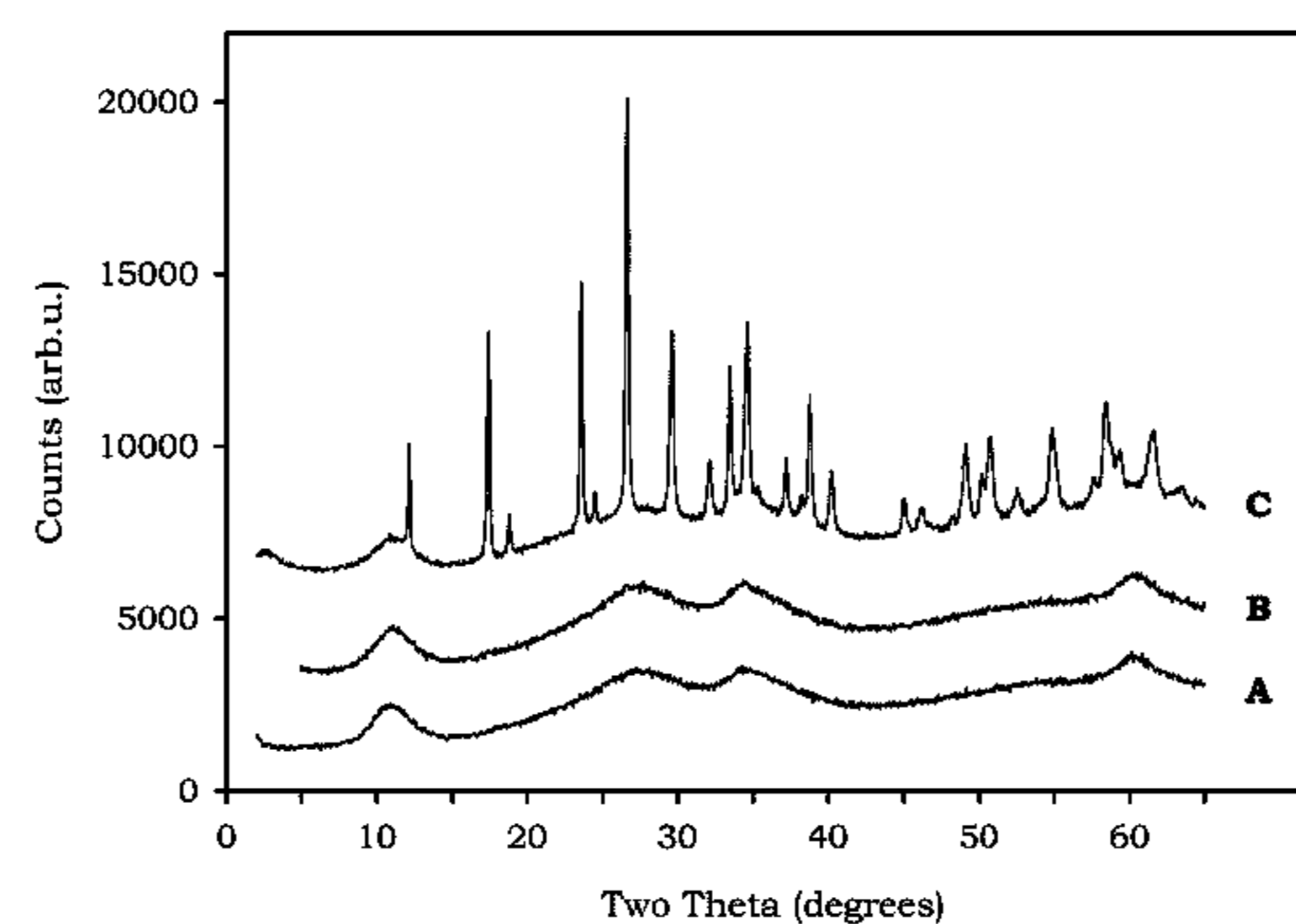
X-ray diffraction patterns of the catalyst compositions Example 1 (A), Example 3 (B) and Example 4 (C).
