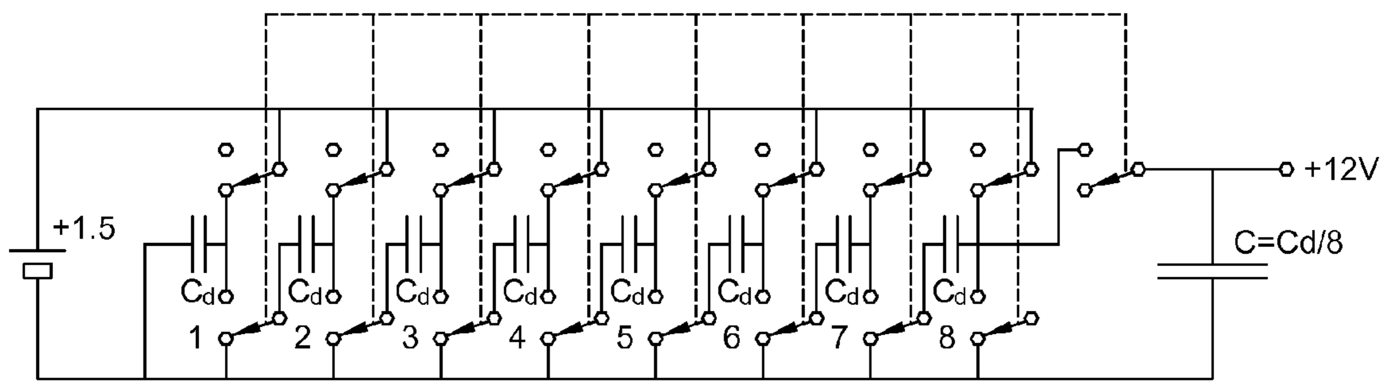
(a) PARALLEL SERIES CONVERTER
