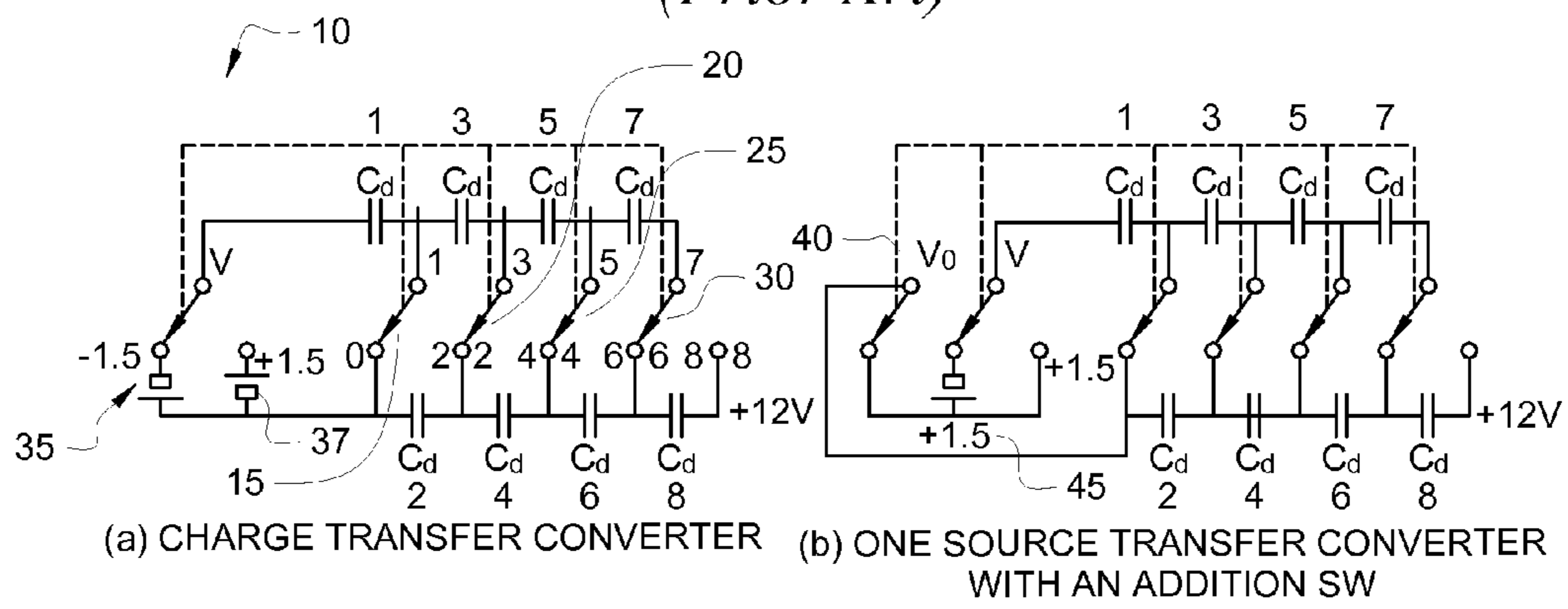
FIG. 3 (Prior Art)
