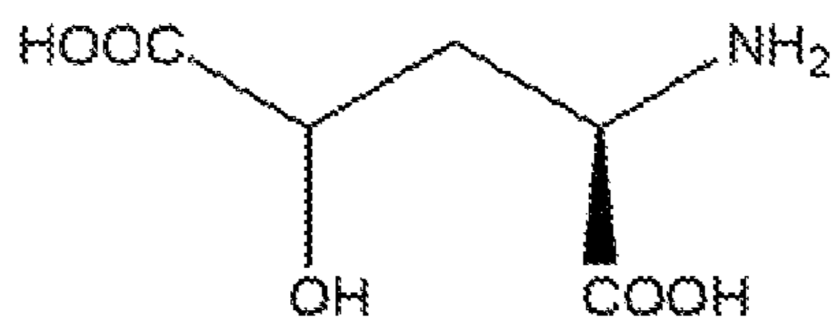
D-gamma-hydroxy glutamate
