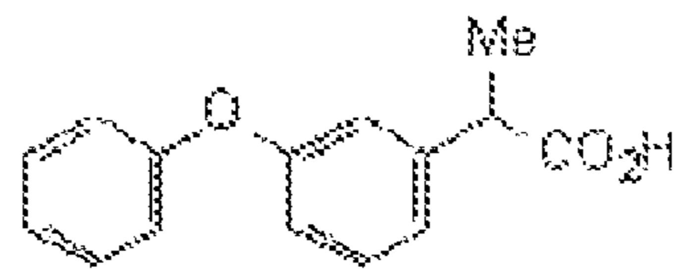
Fenoprofen
