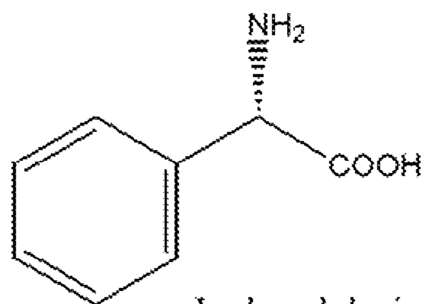
L-phenylglycine
