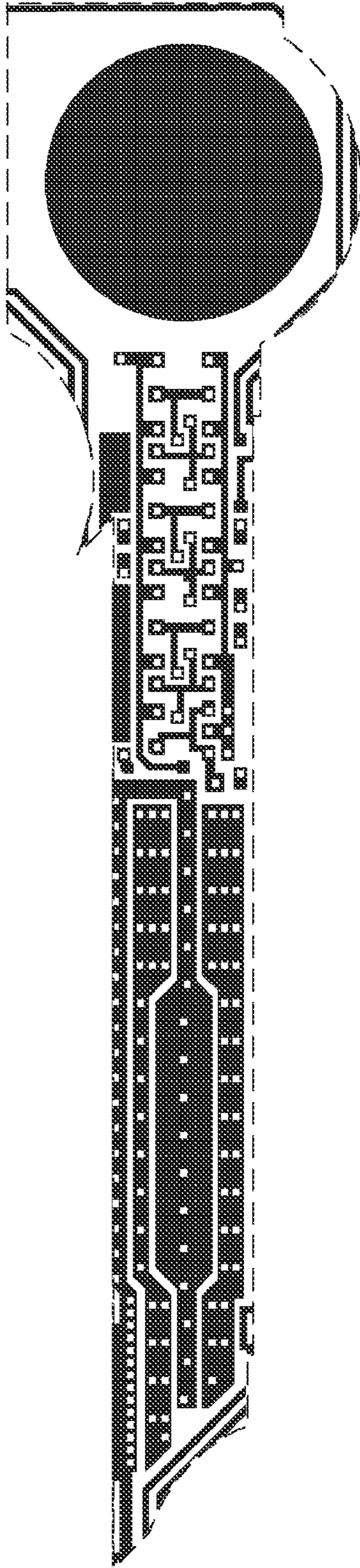
Metal 1 mask
