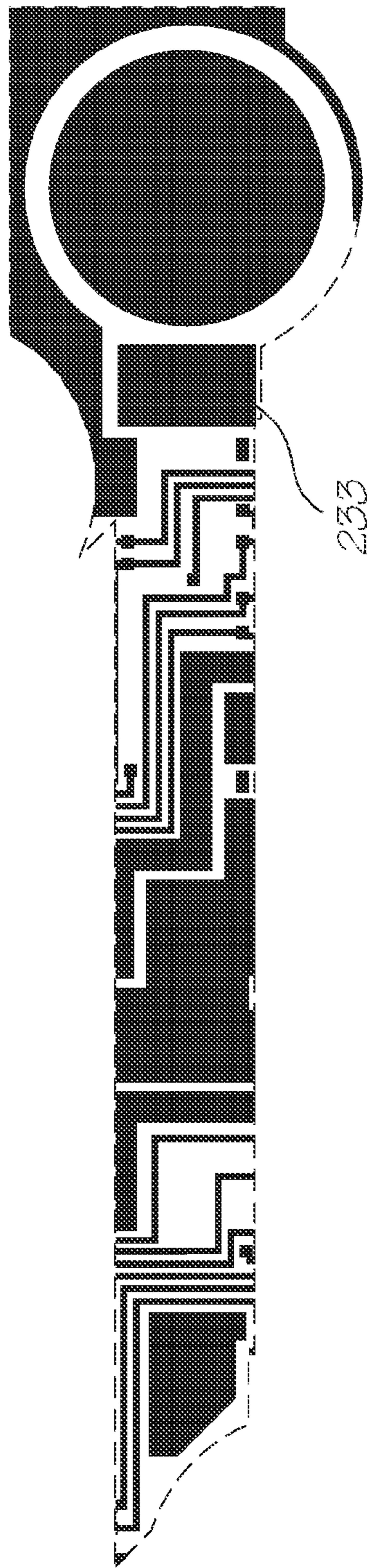
Metal 2 mask
