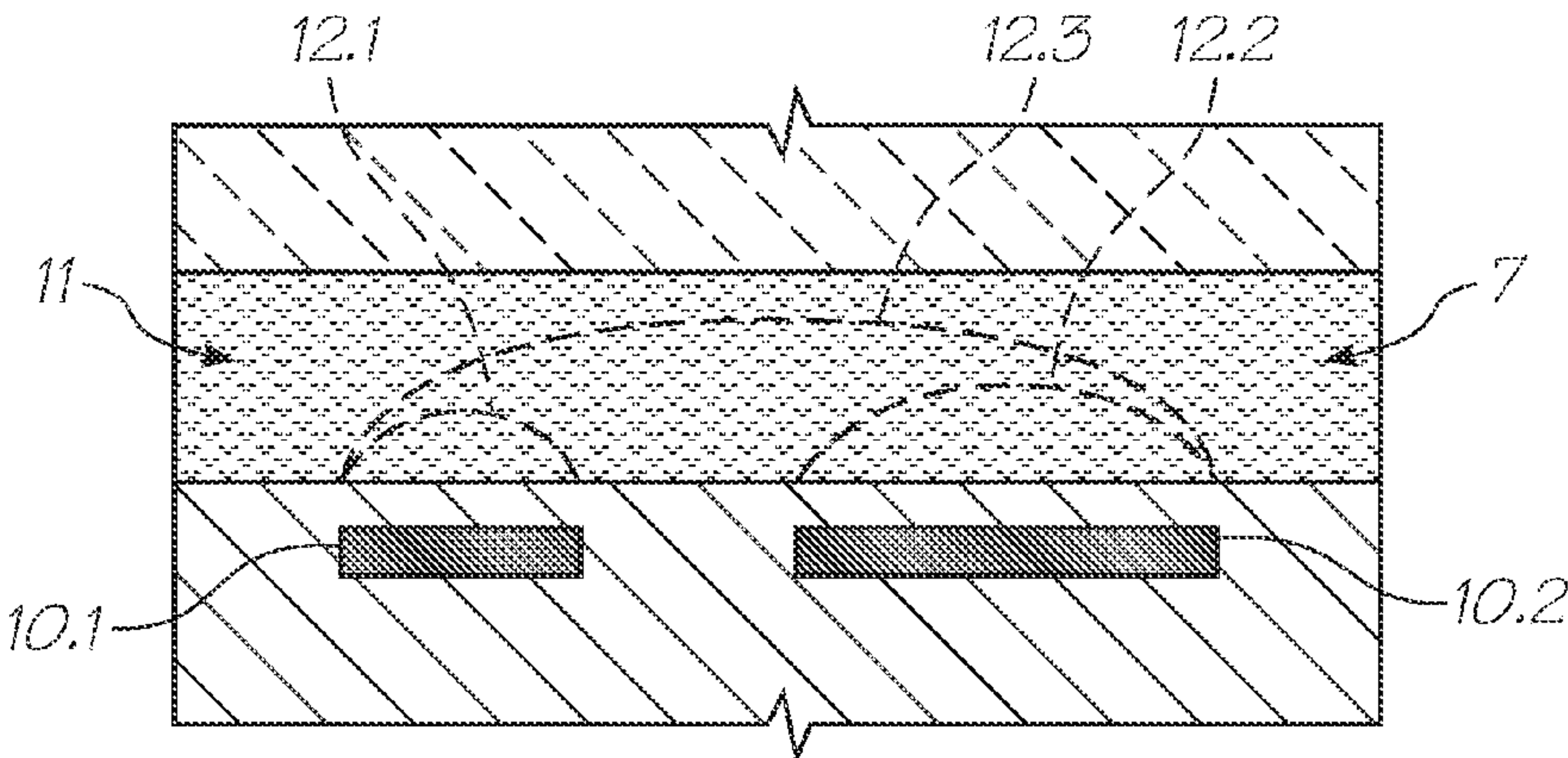
FIG. 52 (PRIOR ART)
