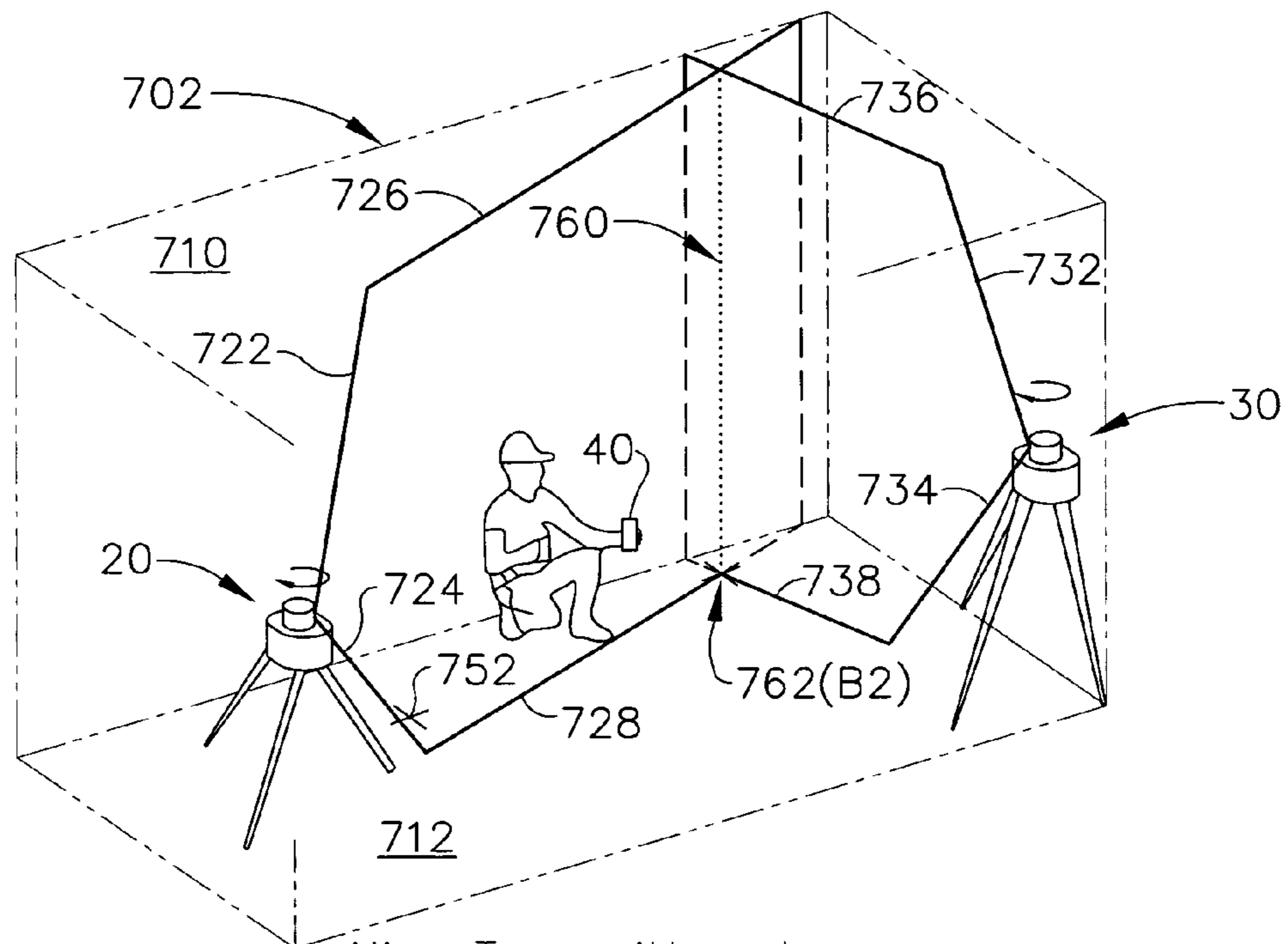
FIG. 11 Align Transmitters to Benchmark 2
