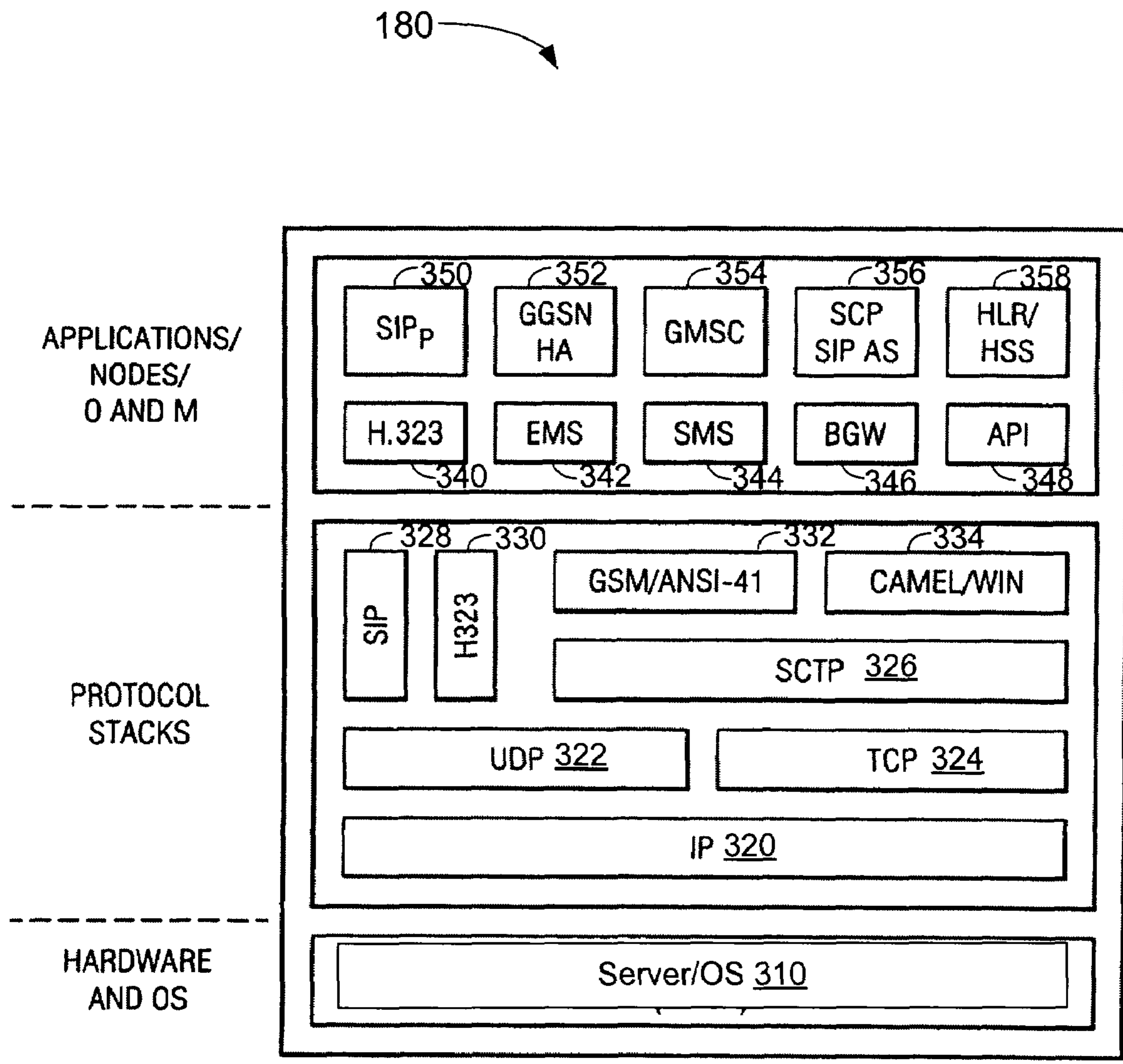
GATEWAY SERVER SYSTEM COMPONENTS
