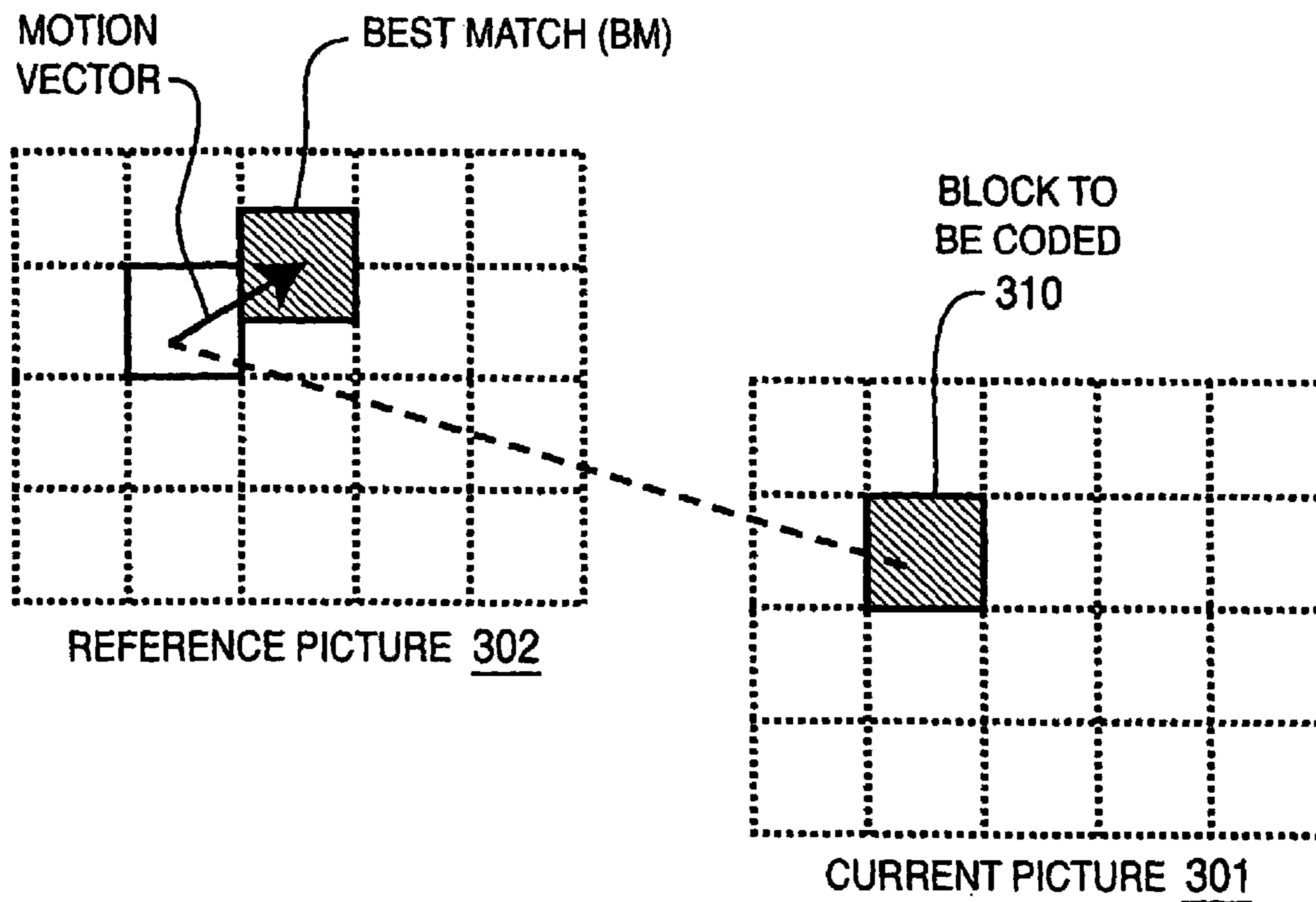
FIG. 3 PRIOR ART
