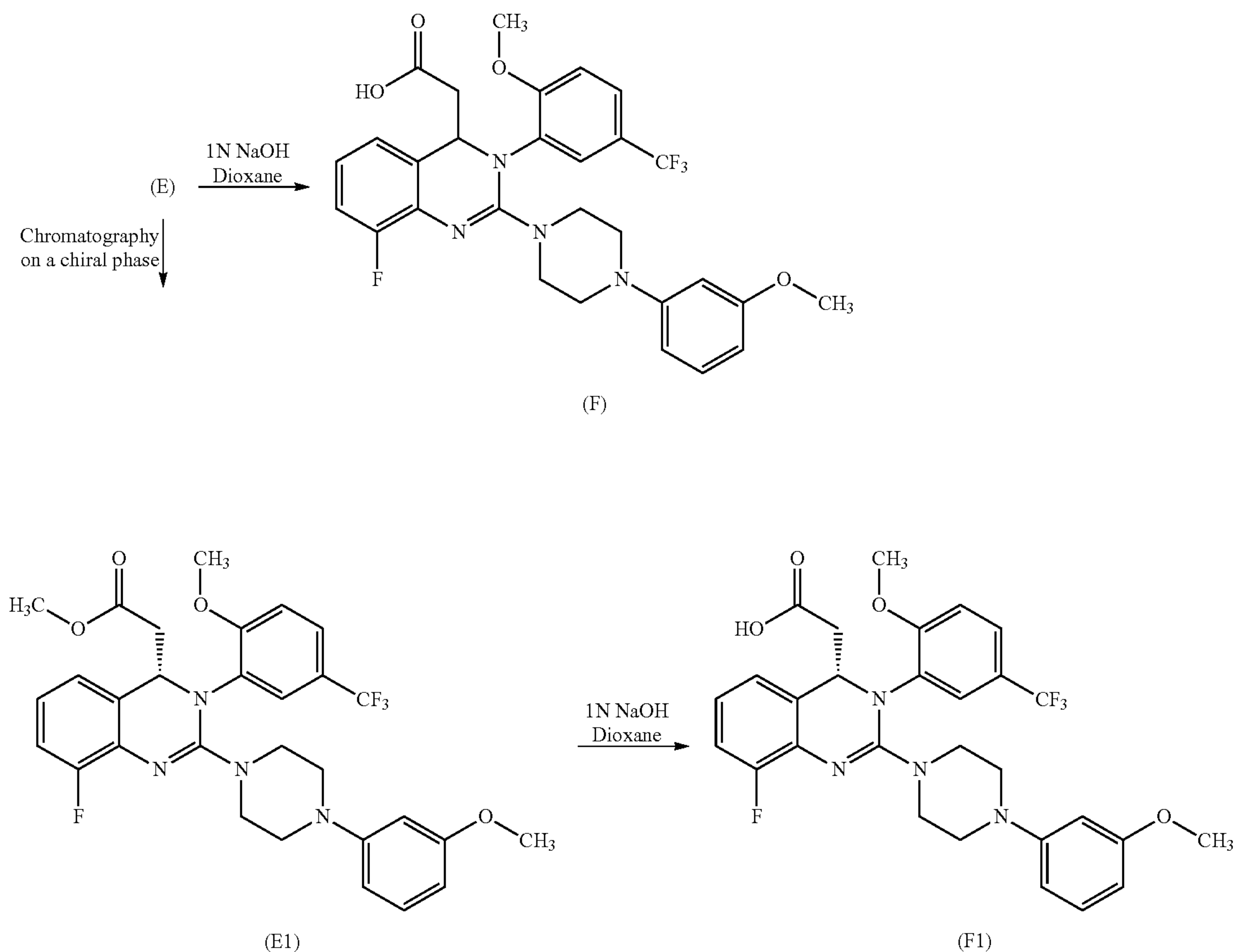
Scheme 2:
