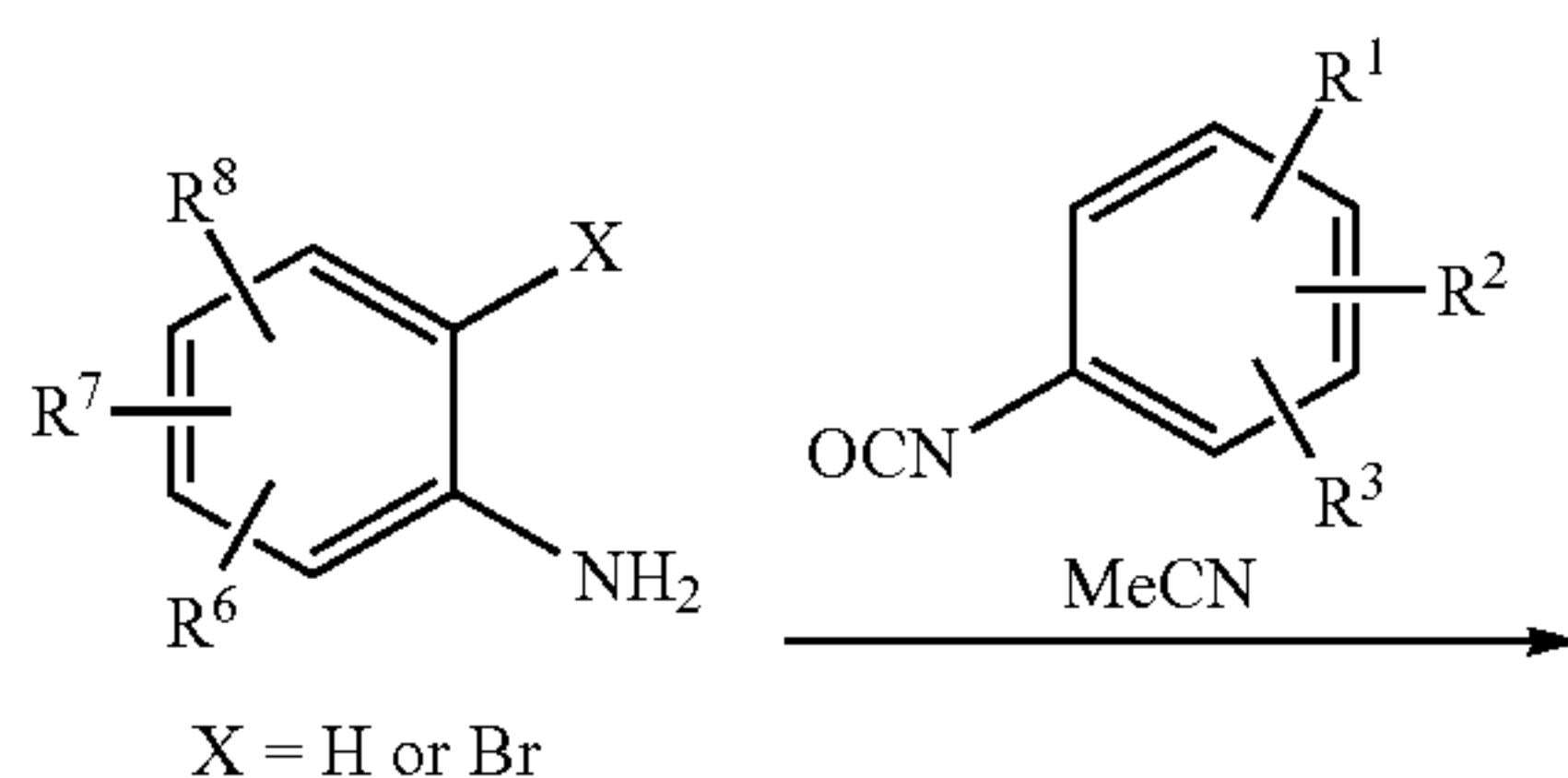
Scheme 3:
