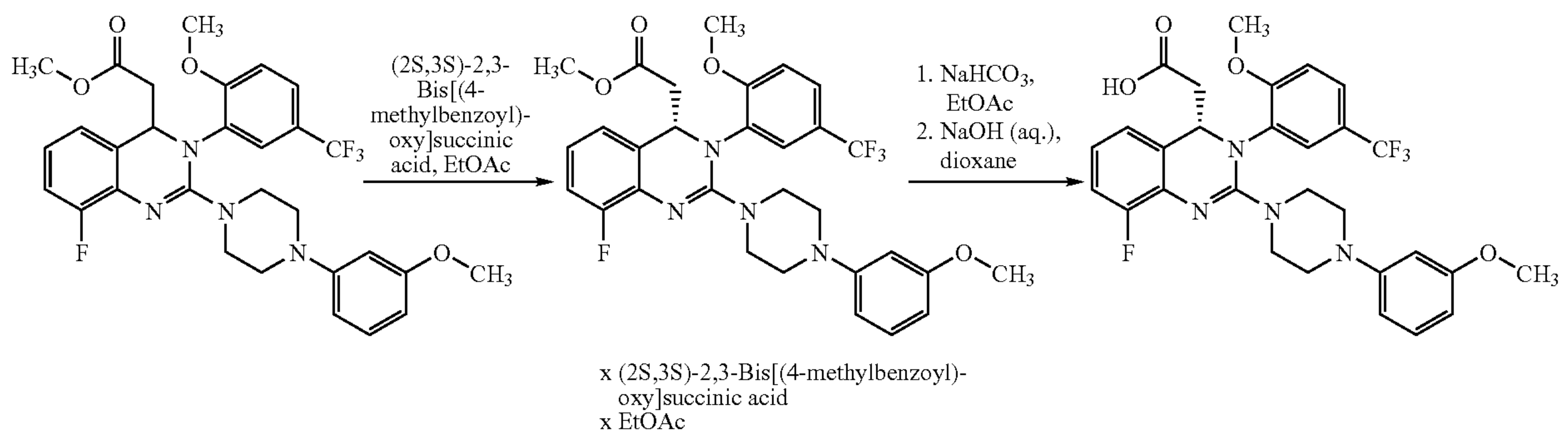
Scheme 4:
