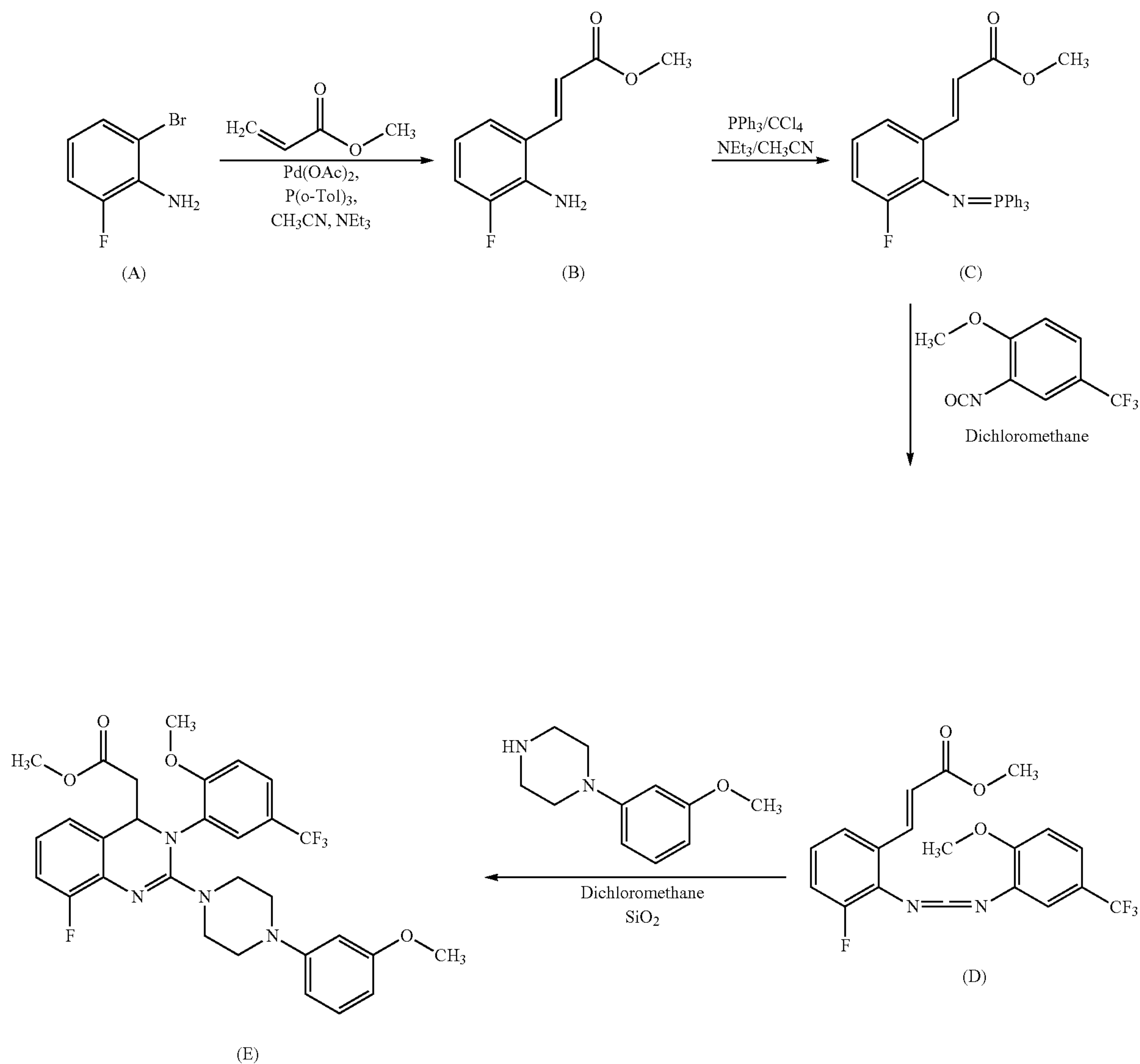
Scheme 1:
