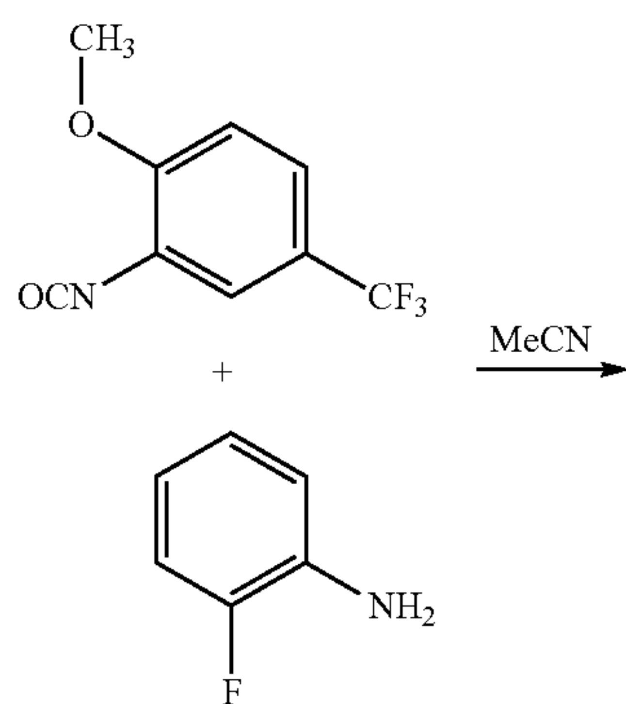
Scheme 7:
