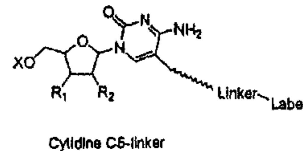
Cytidine C5-linker
