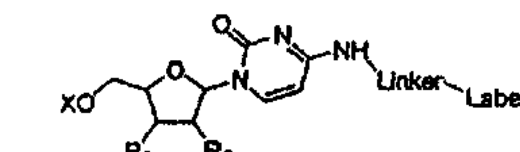
Cytidine N4-linker
