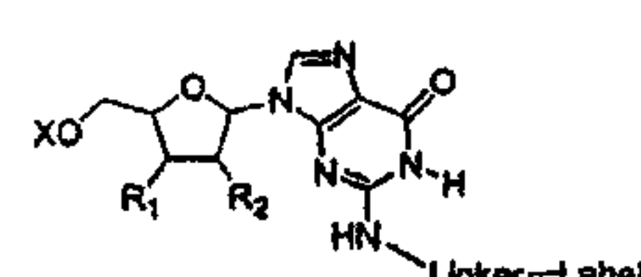
Guanosine N2-linker
