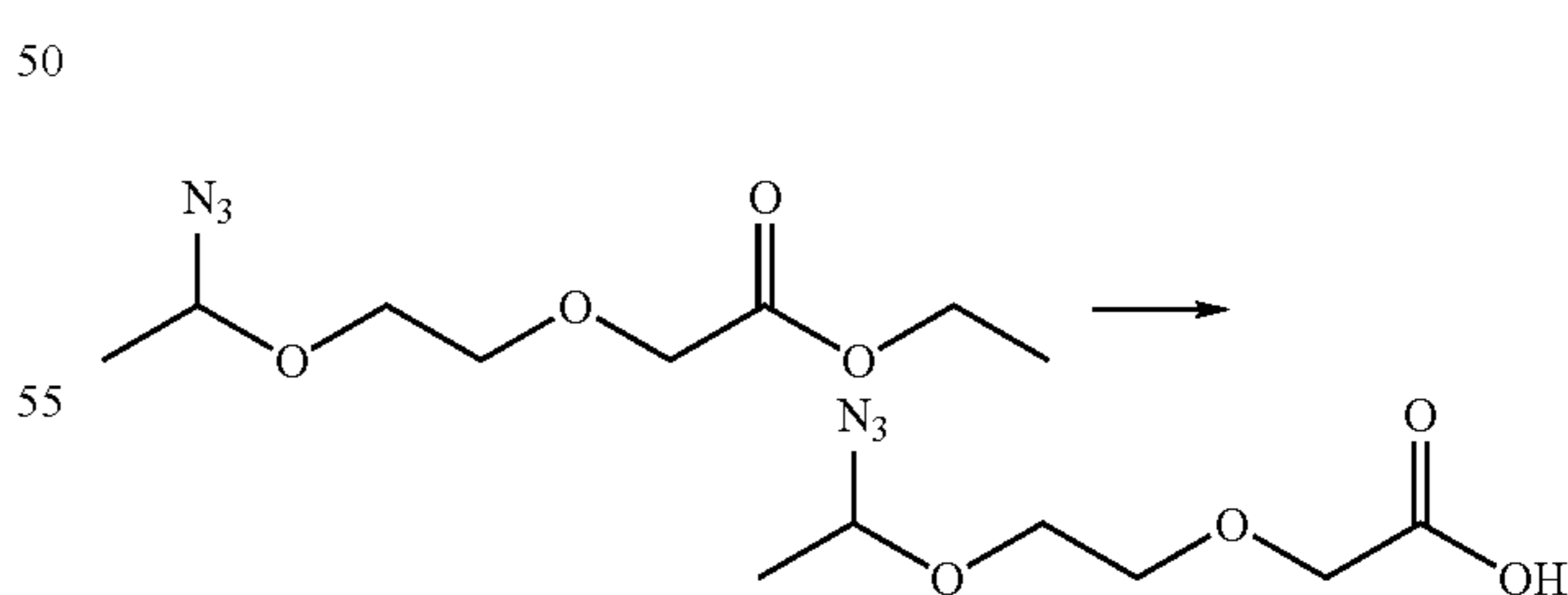
[2-(1-Azido-ethoxy)-ethoxy]-acetic acid
