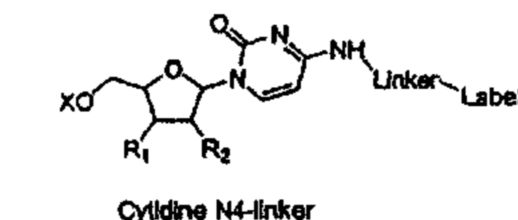
Cytidine N4-linker
