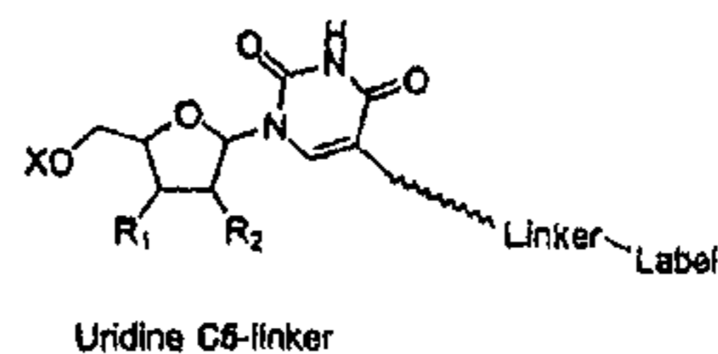
Uridine C5-linker
