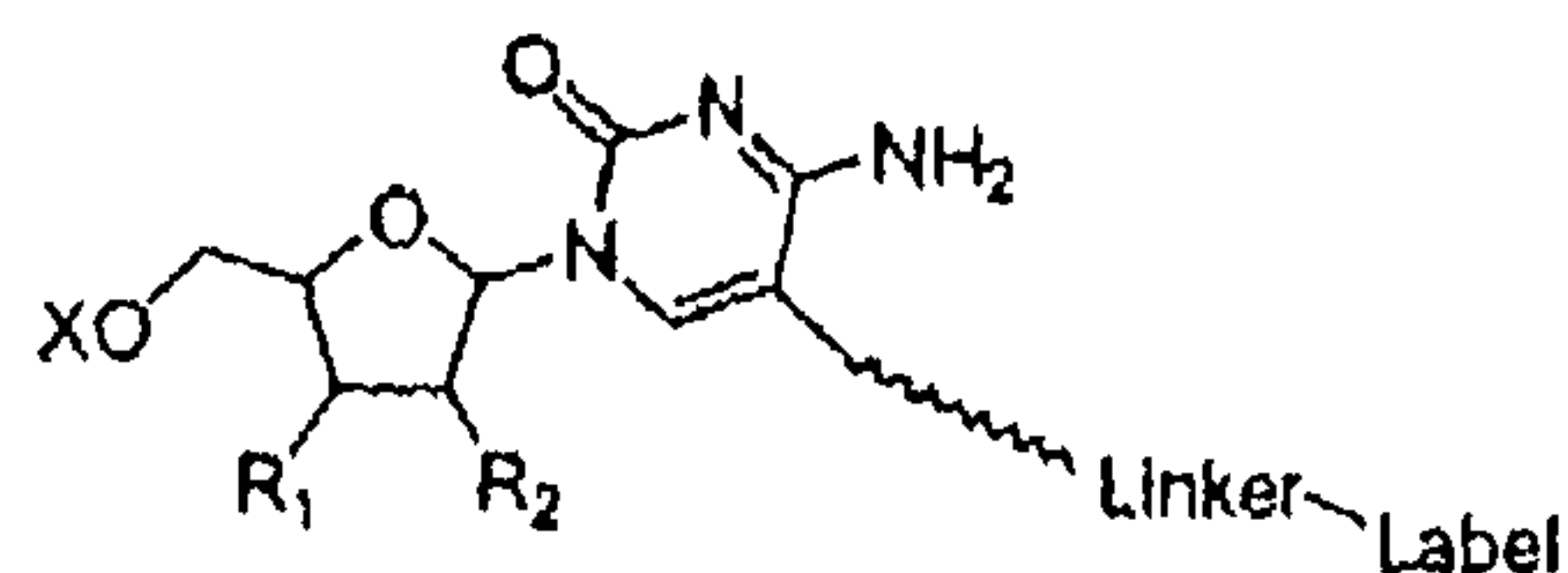
Cytidine C5-linker
