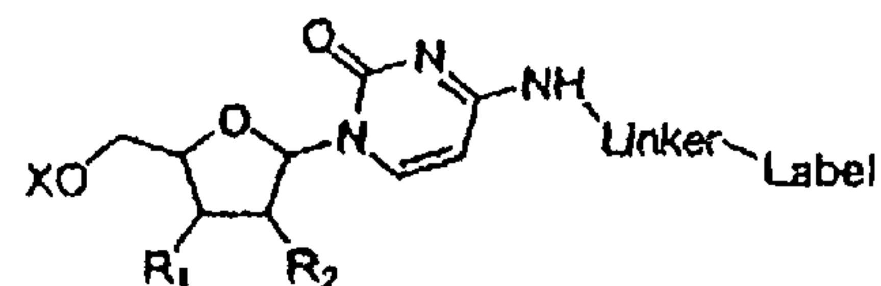
Cytidine N4-linker
