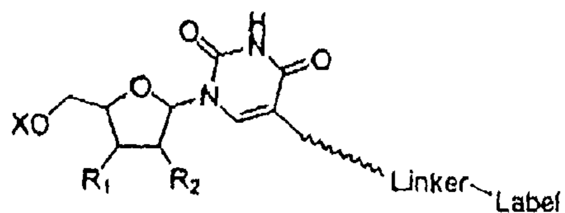
Uridine C5-linker
