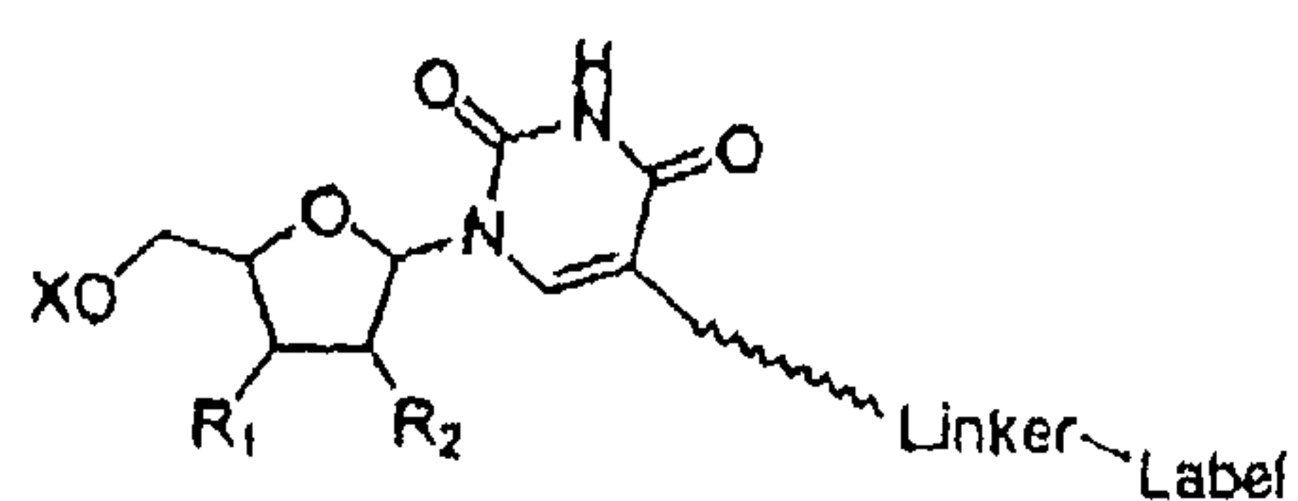
Uridine C5-linker
