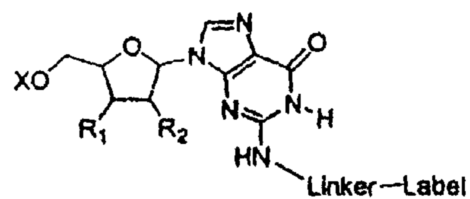
Guanosine N2-linker
