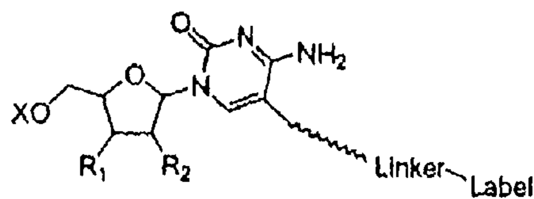
Cytidine C5-linker
