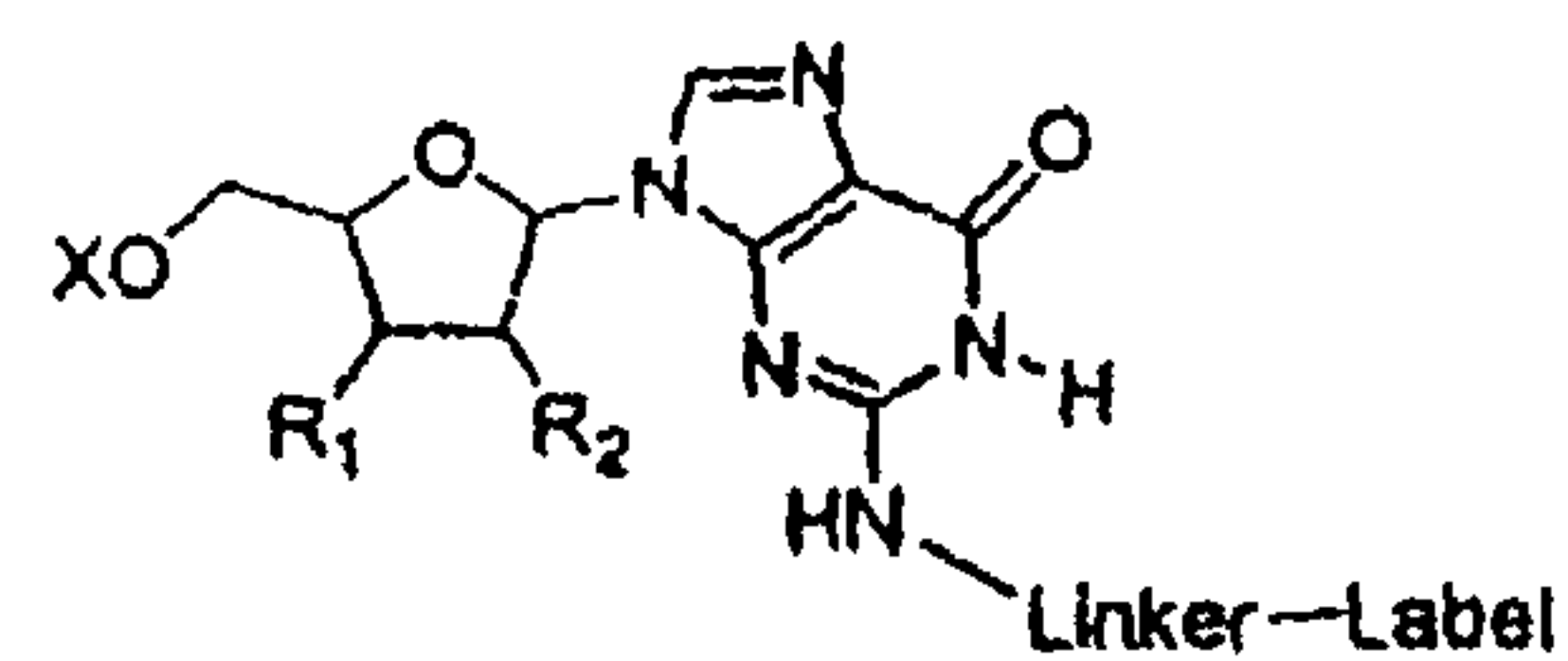
Guanosine N2-linker
