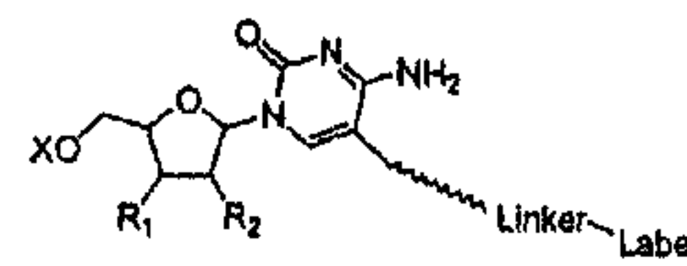
Cytidine C5-linker
