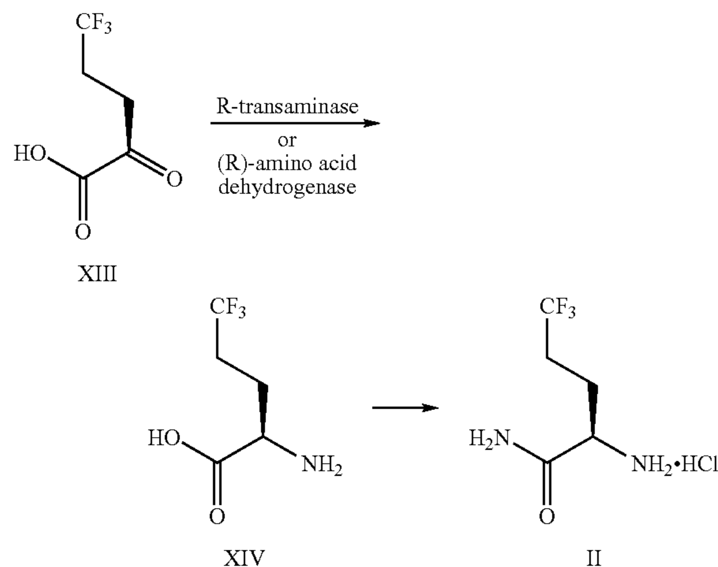
Reaction Scheme 4
