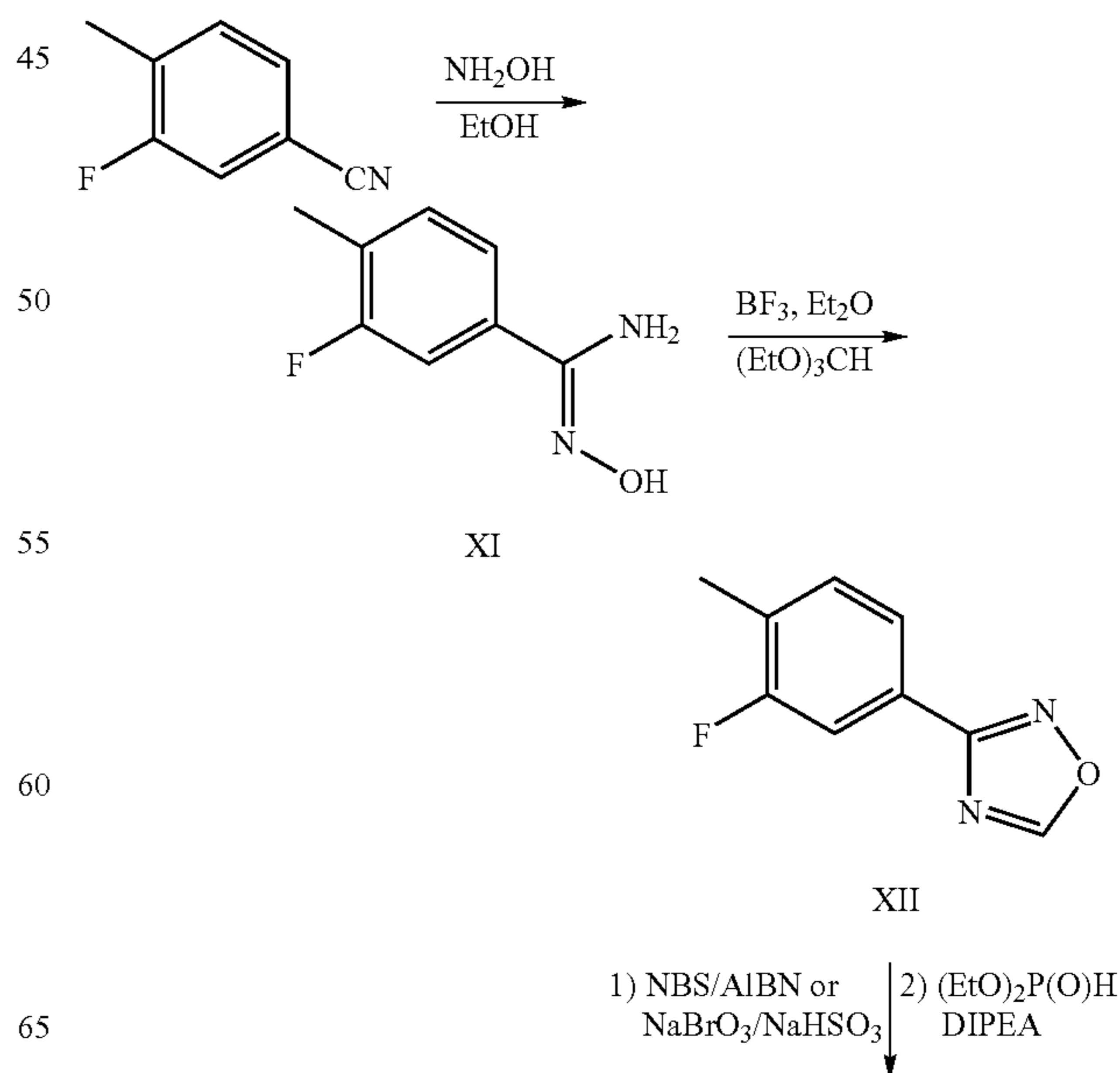
Reaction Scheme 6
