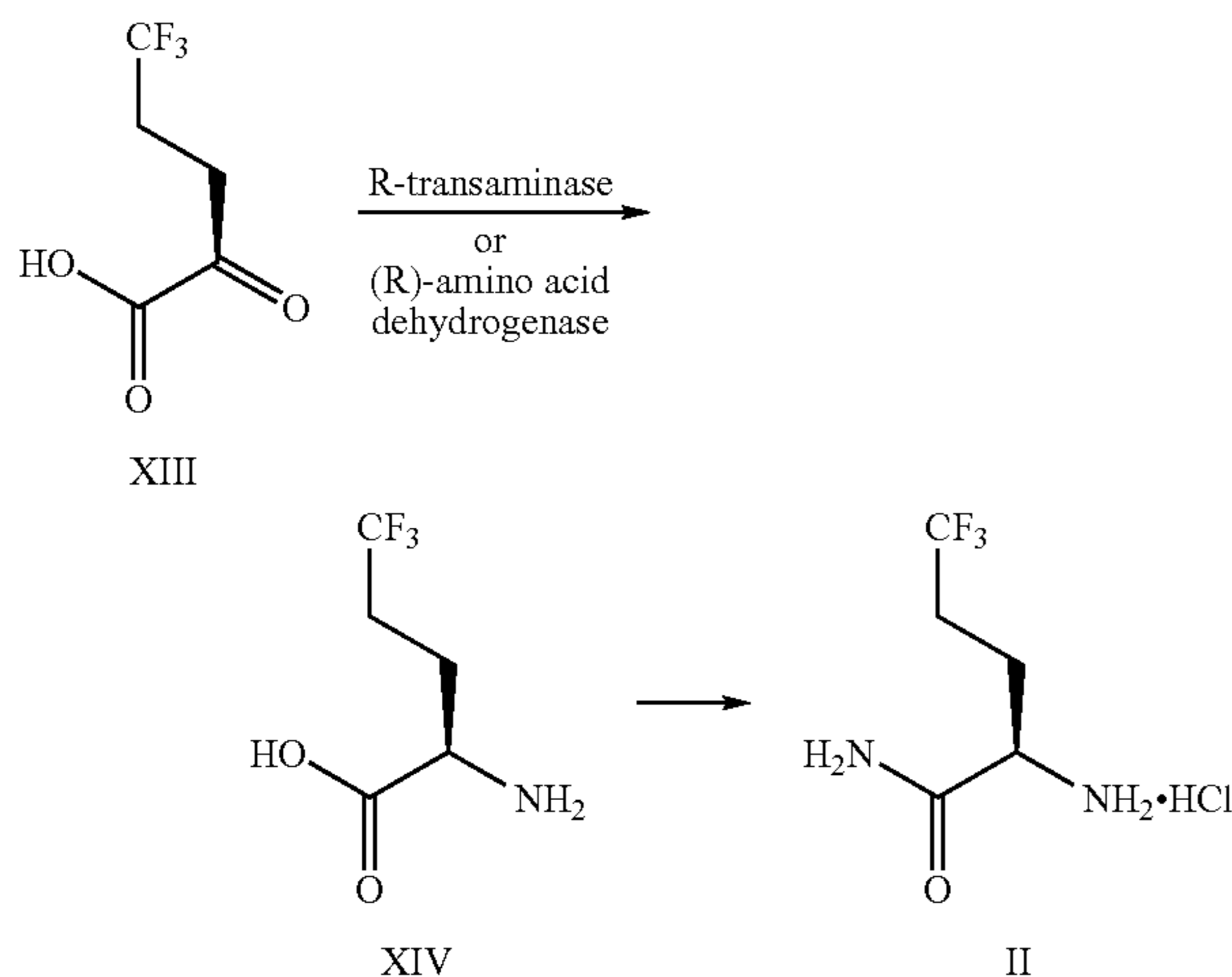
Reaction Scheme 4
