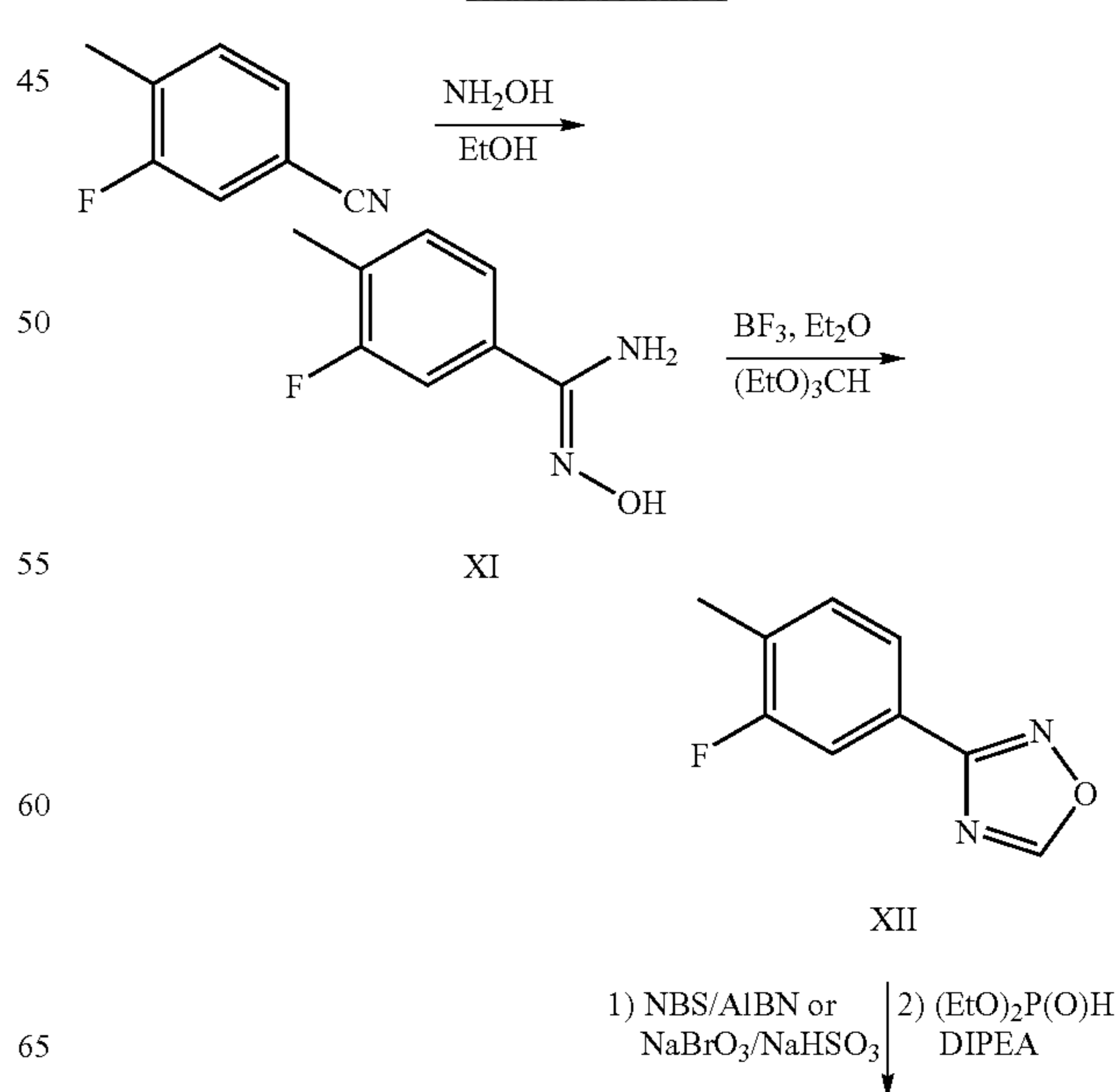
Reaction Scheme 6
