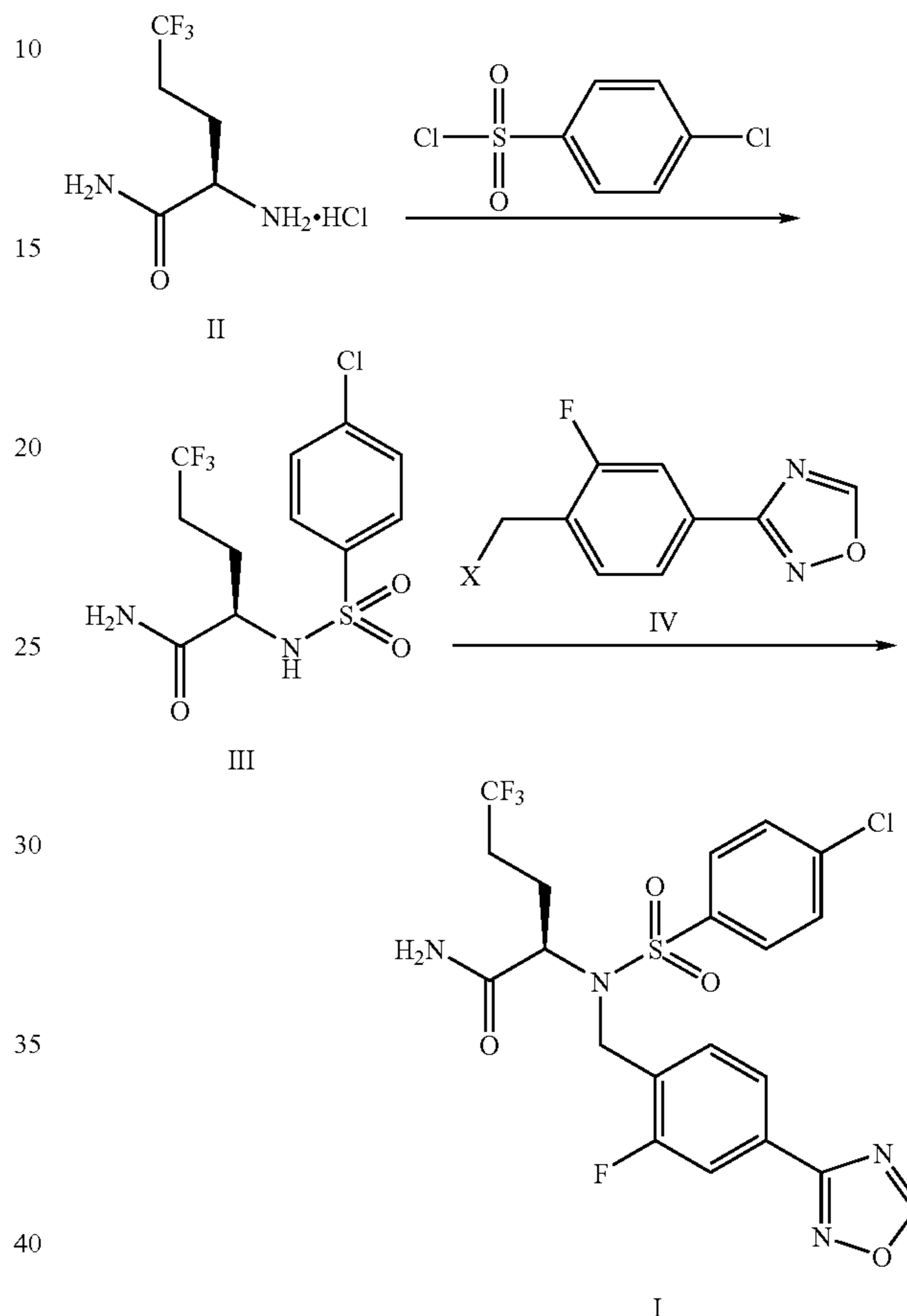
Reaction Scheme 1
