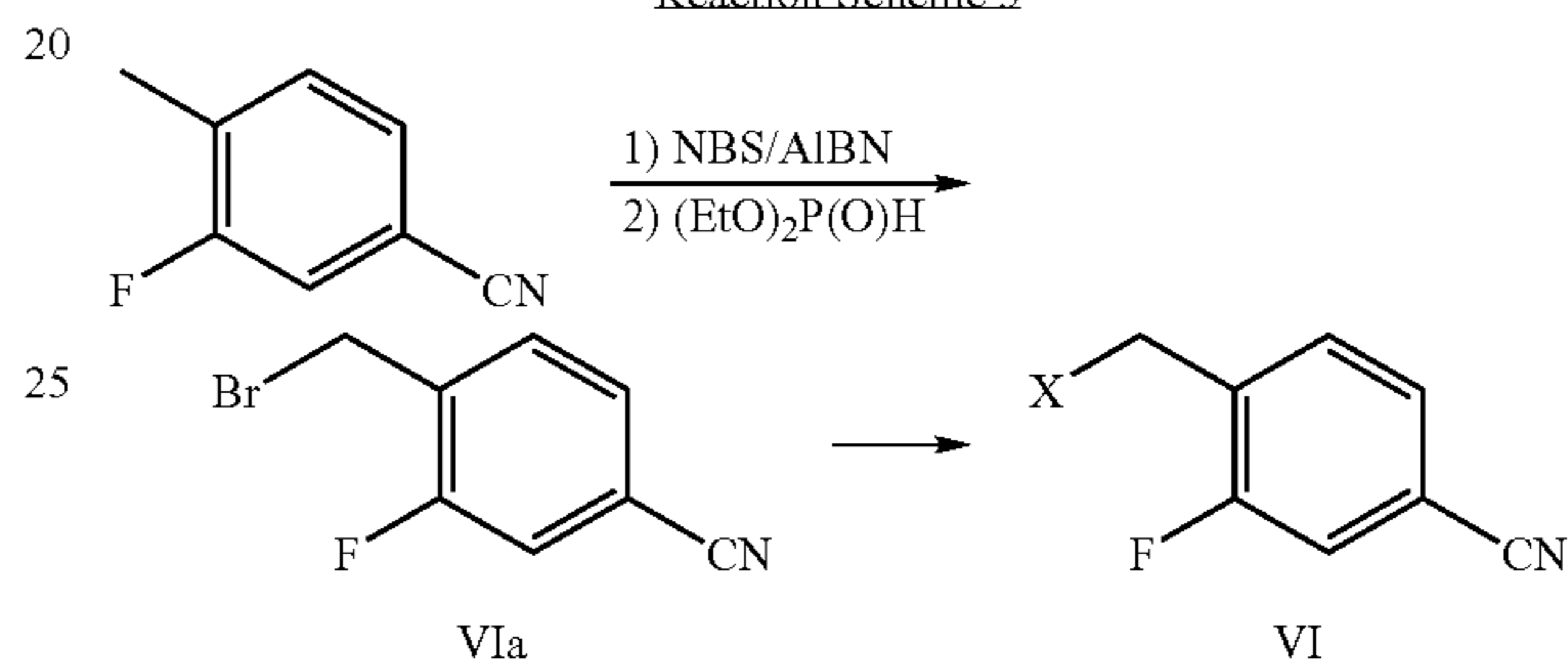
Reaction Scheme 5
