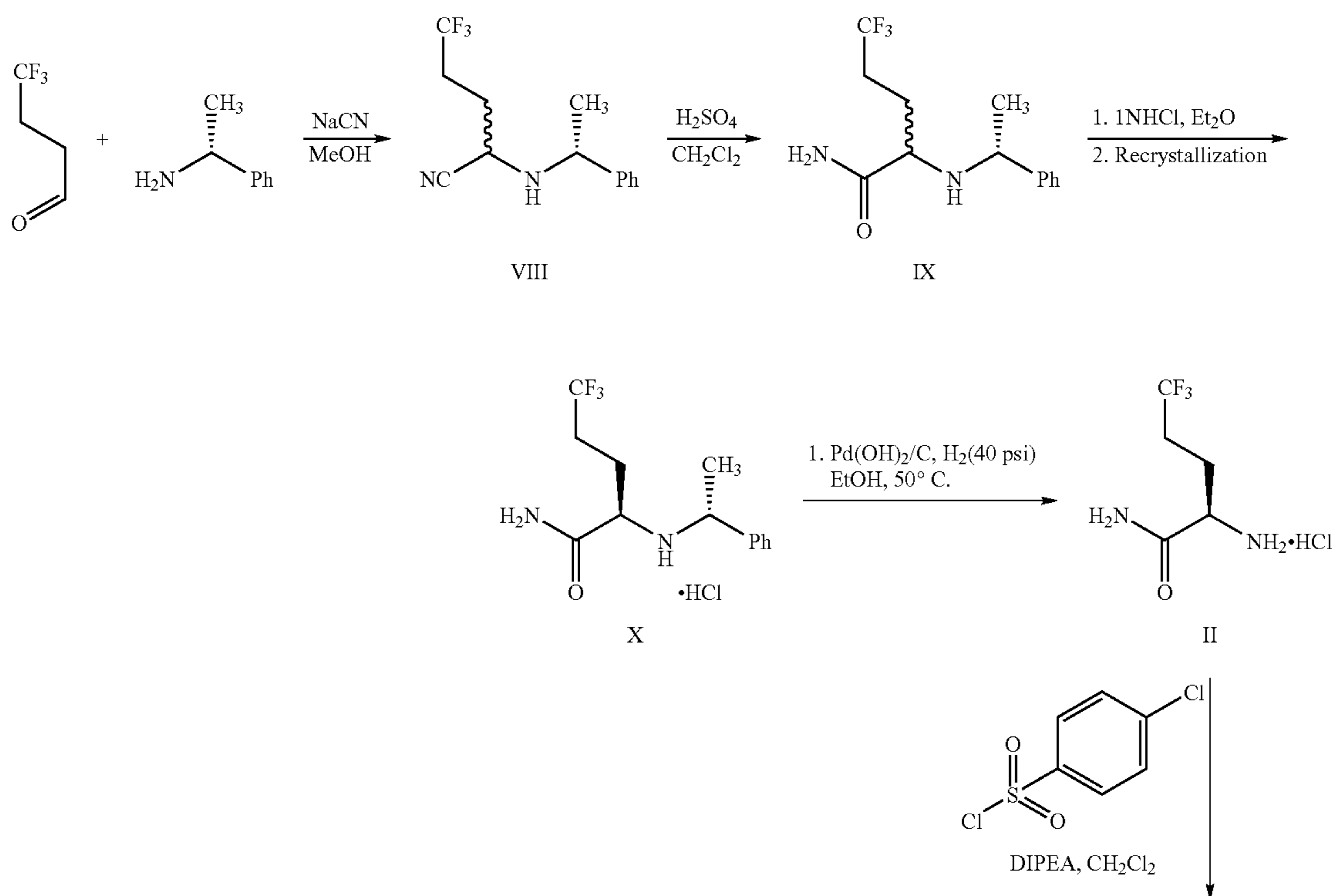
Reaction Scheme 3
