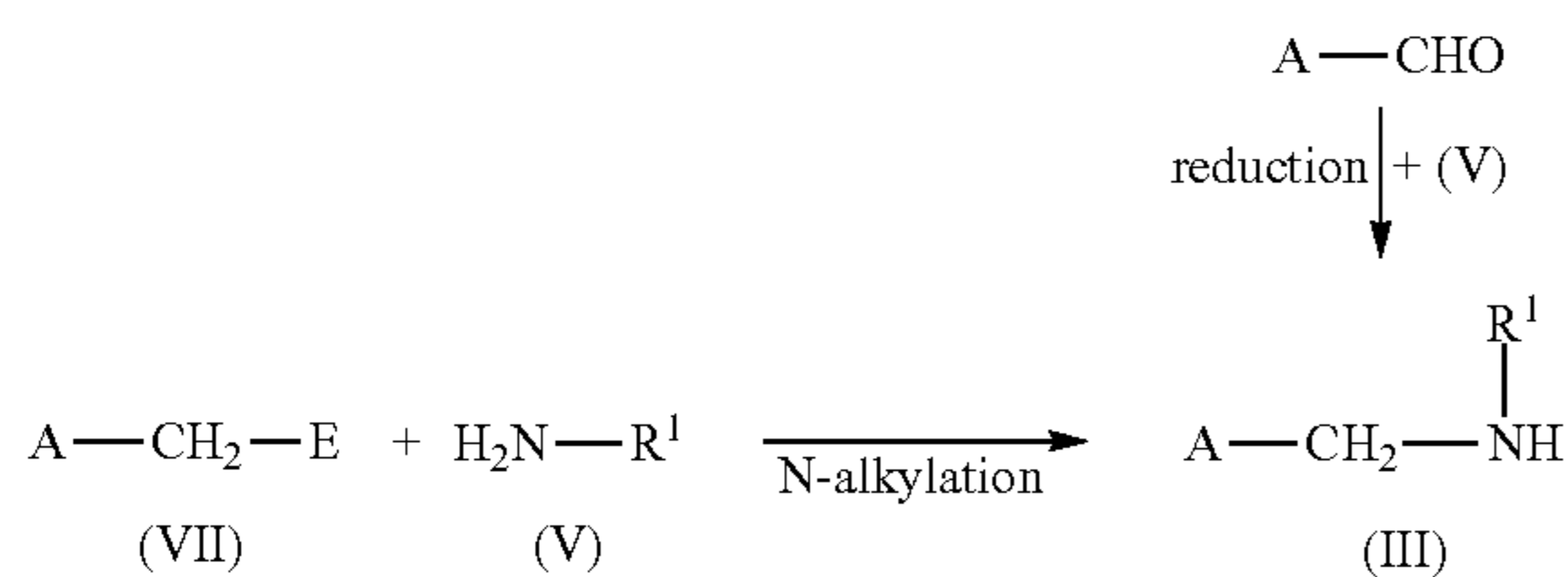
Scheme V
