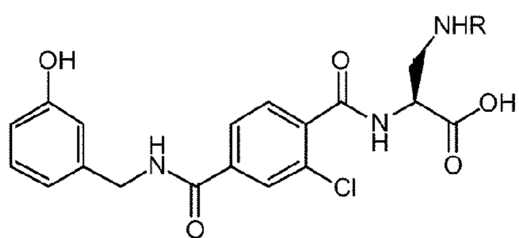
Compound 1, R = (C=S)NH-Fluorescein
