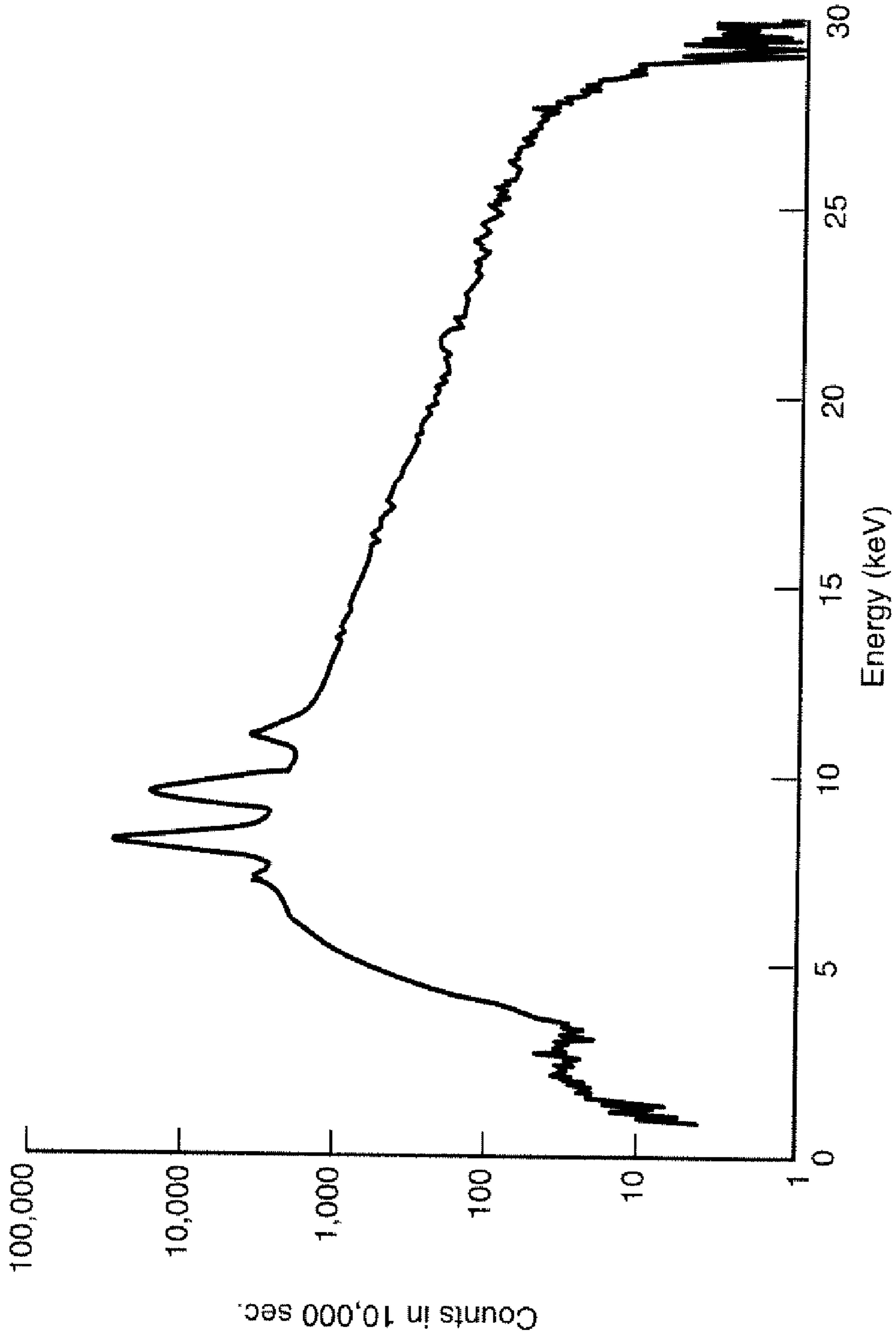
Electron Generator X-ray Tube Measured Spectrum
