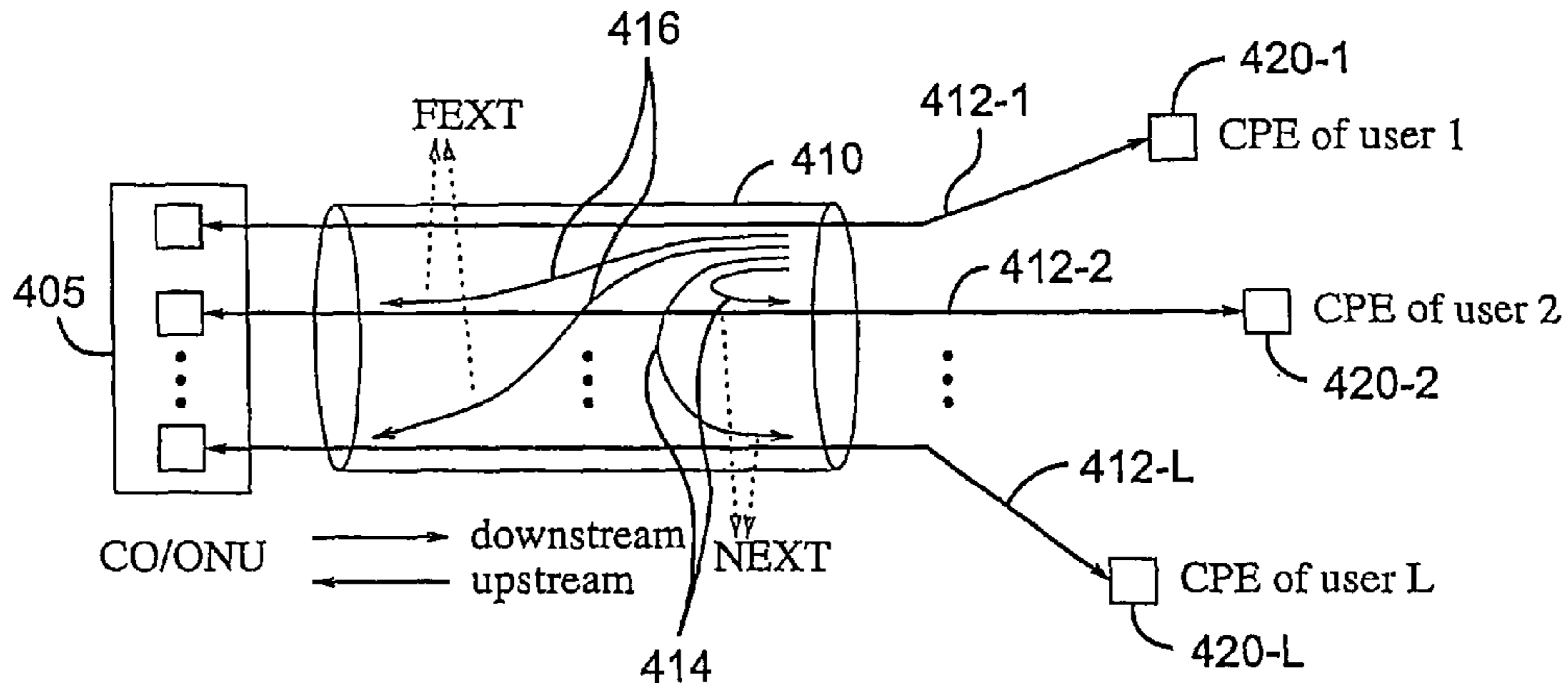
FIG. 4 Prior Art
