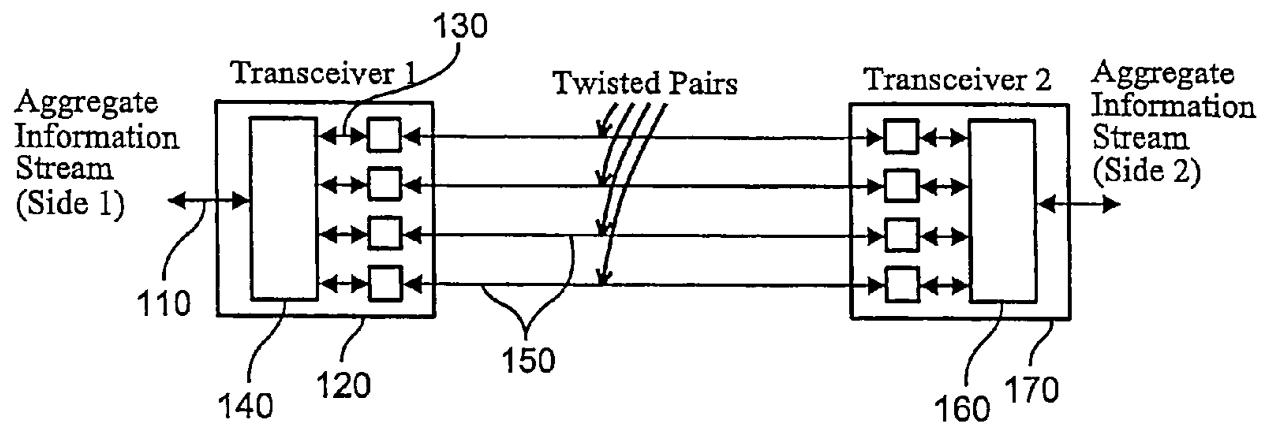
FIG. 1 Prior Art
