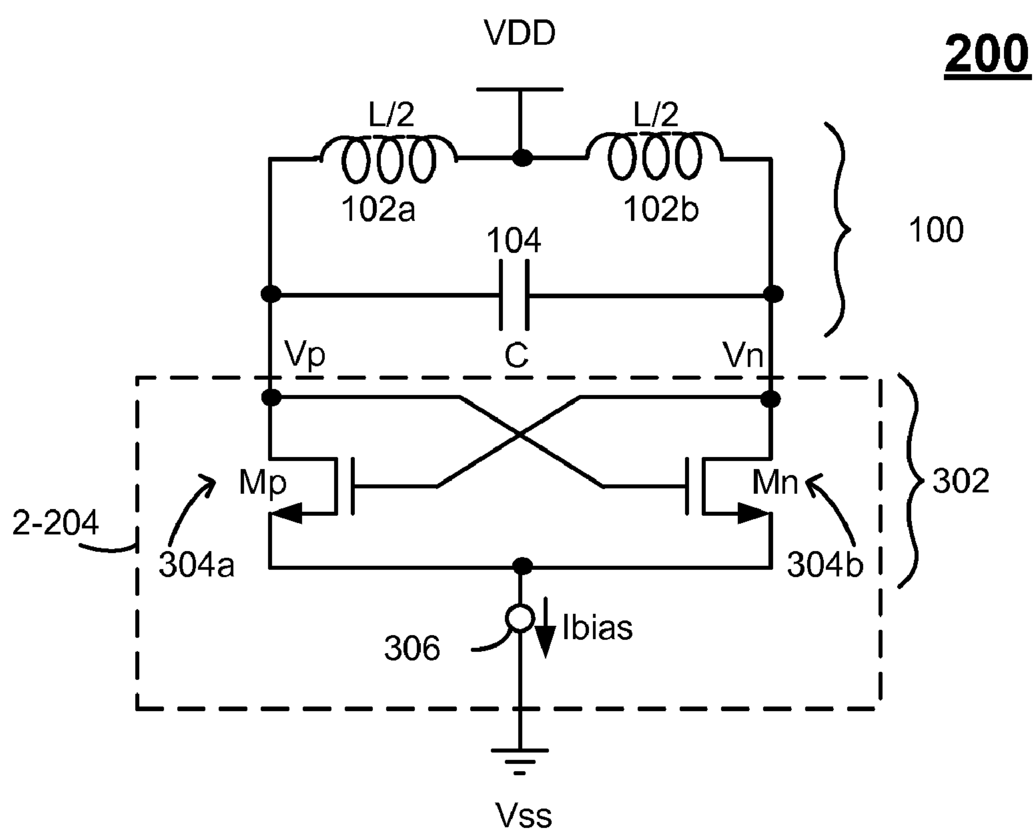
Fig. 3 (prior art)
