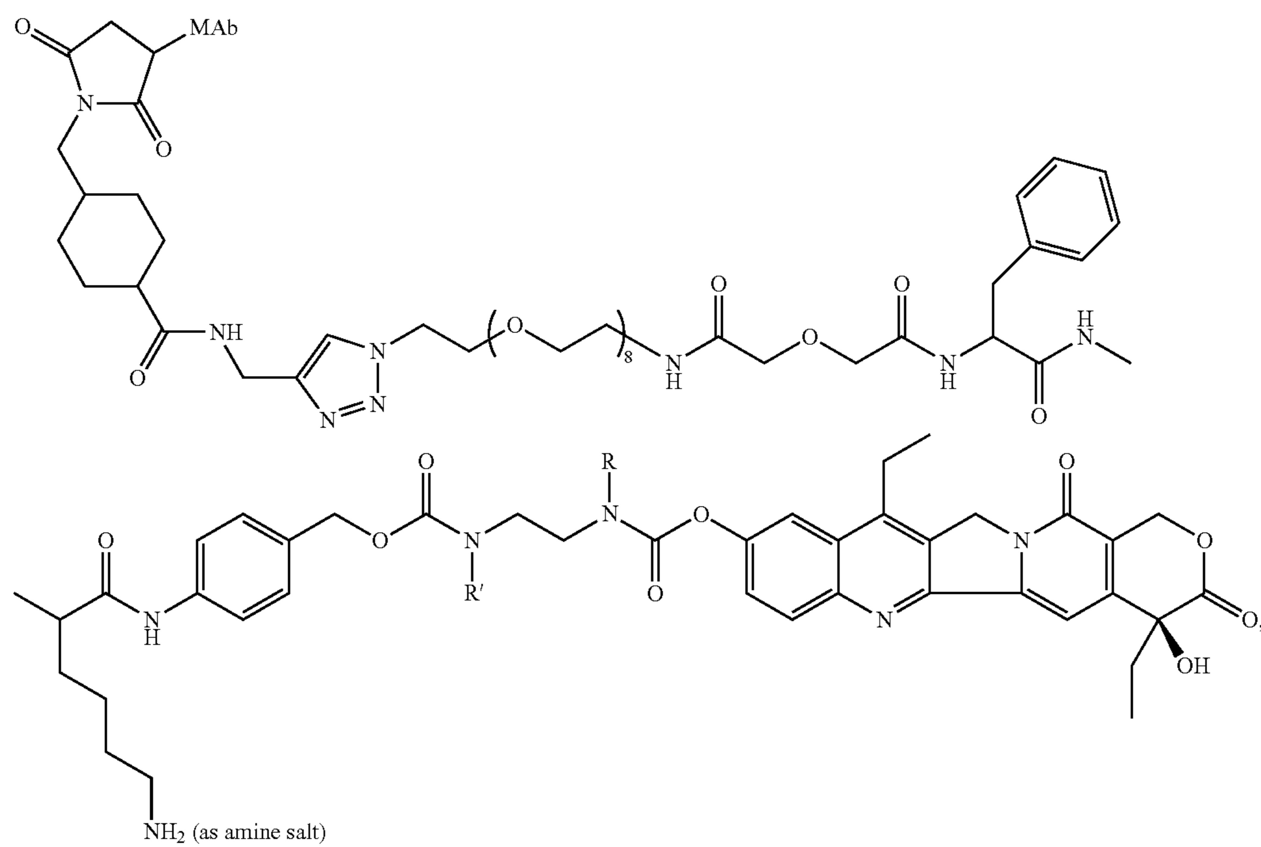
MAb-CLY-SN-38
