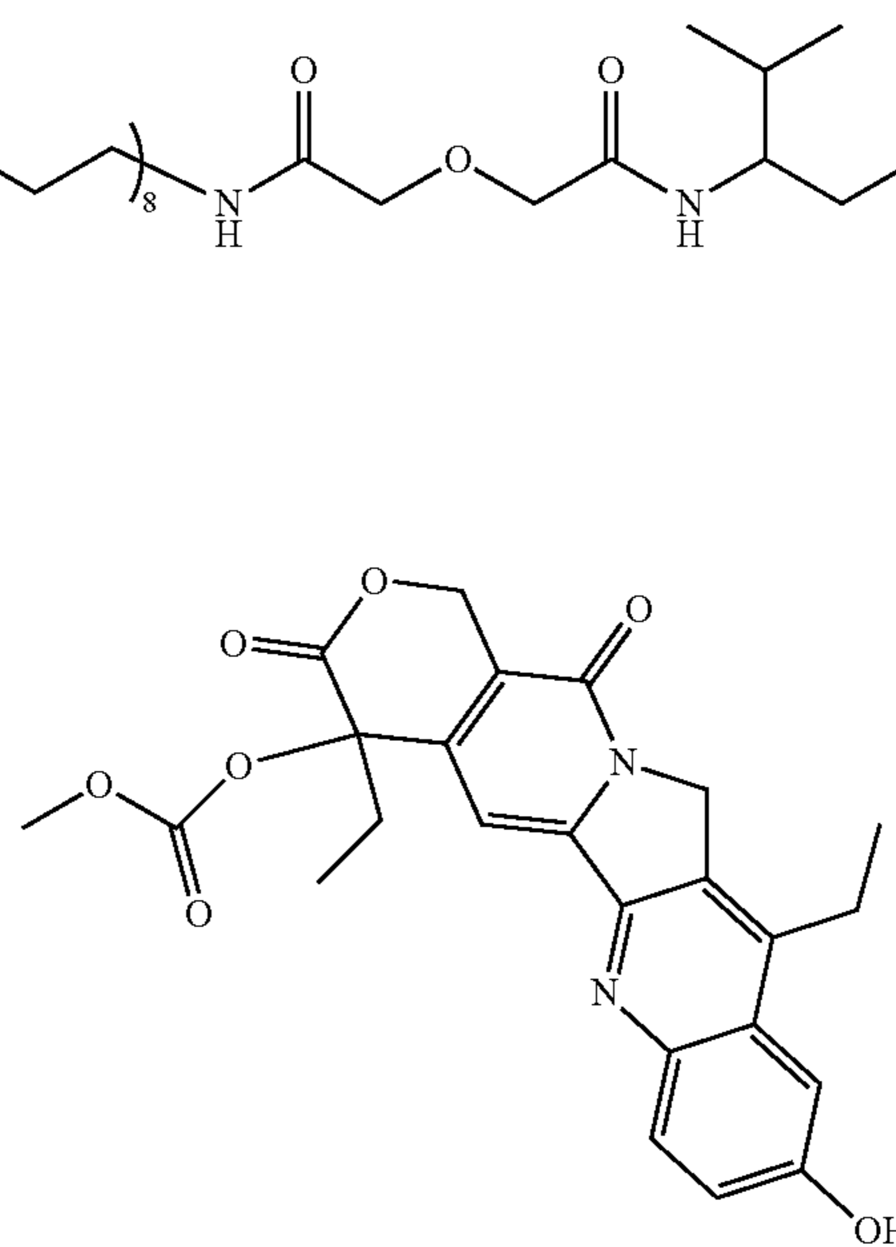
MAb-CL6-SN-38
