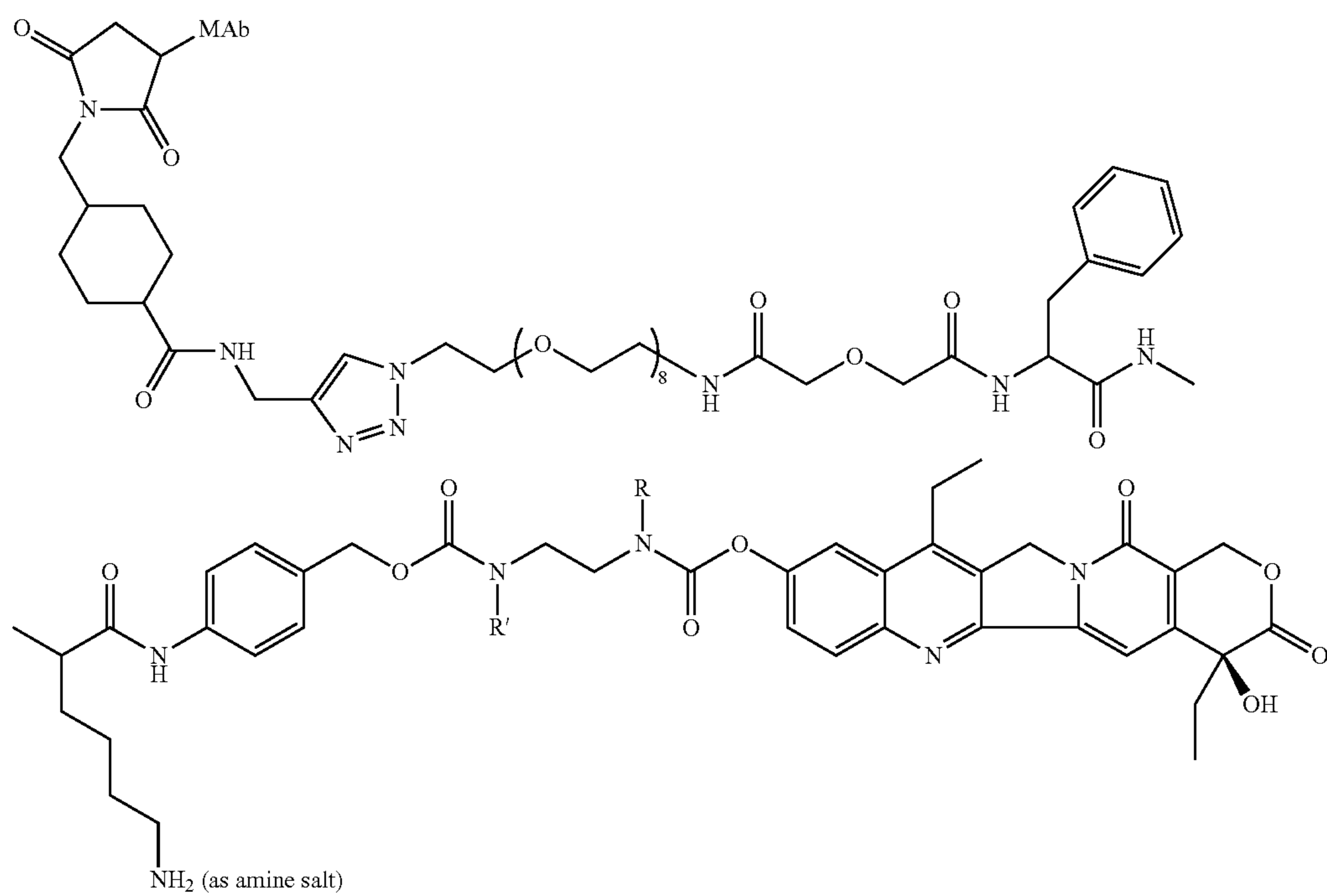
MAb-CLY-SN-38
