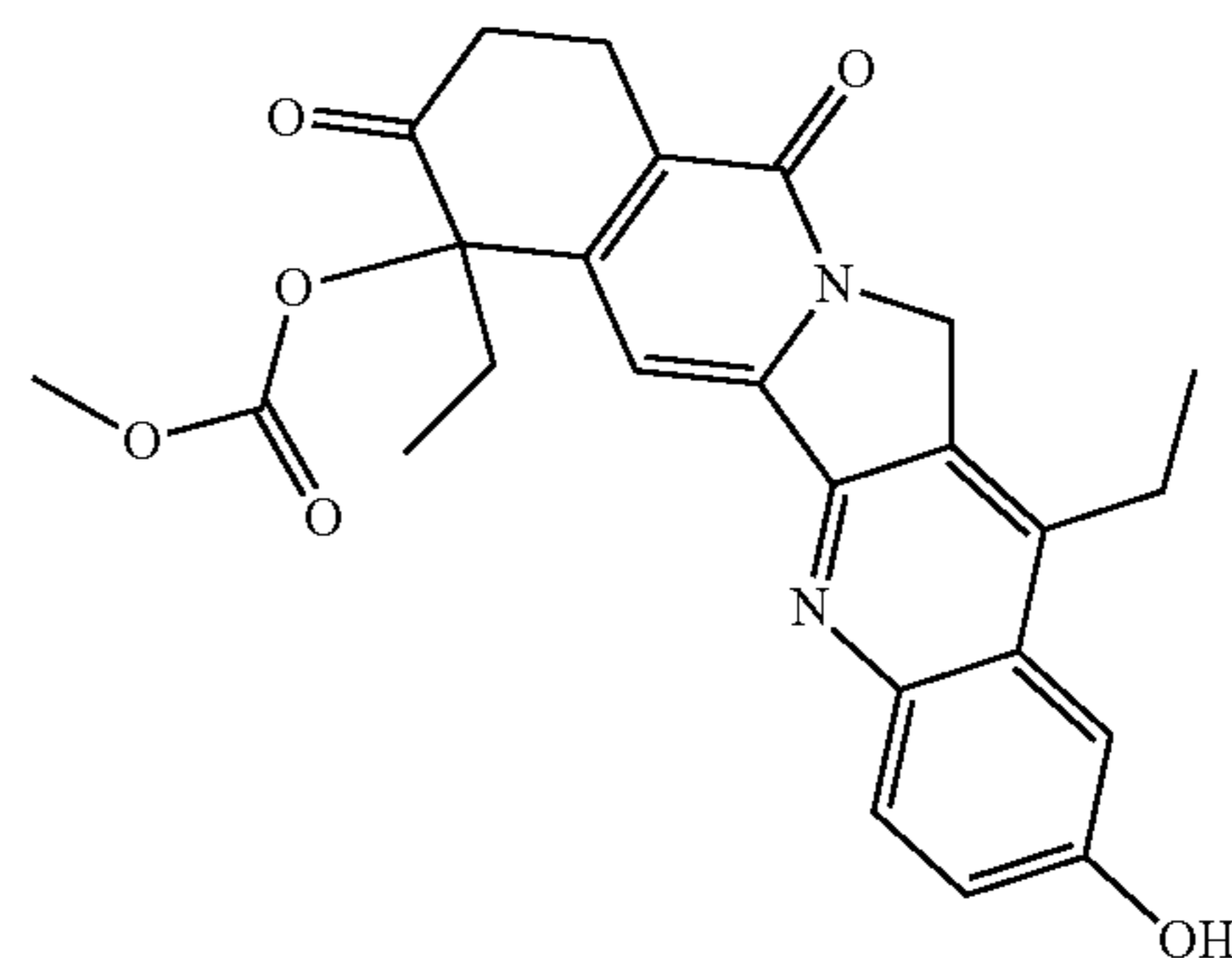
MAB-CL2A-SN-38
