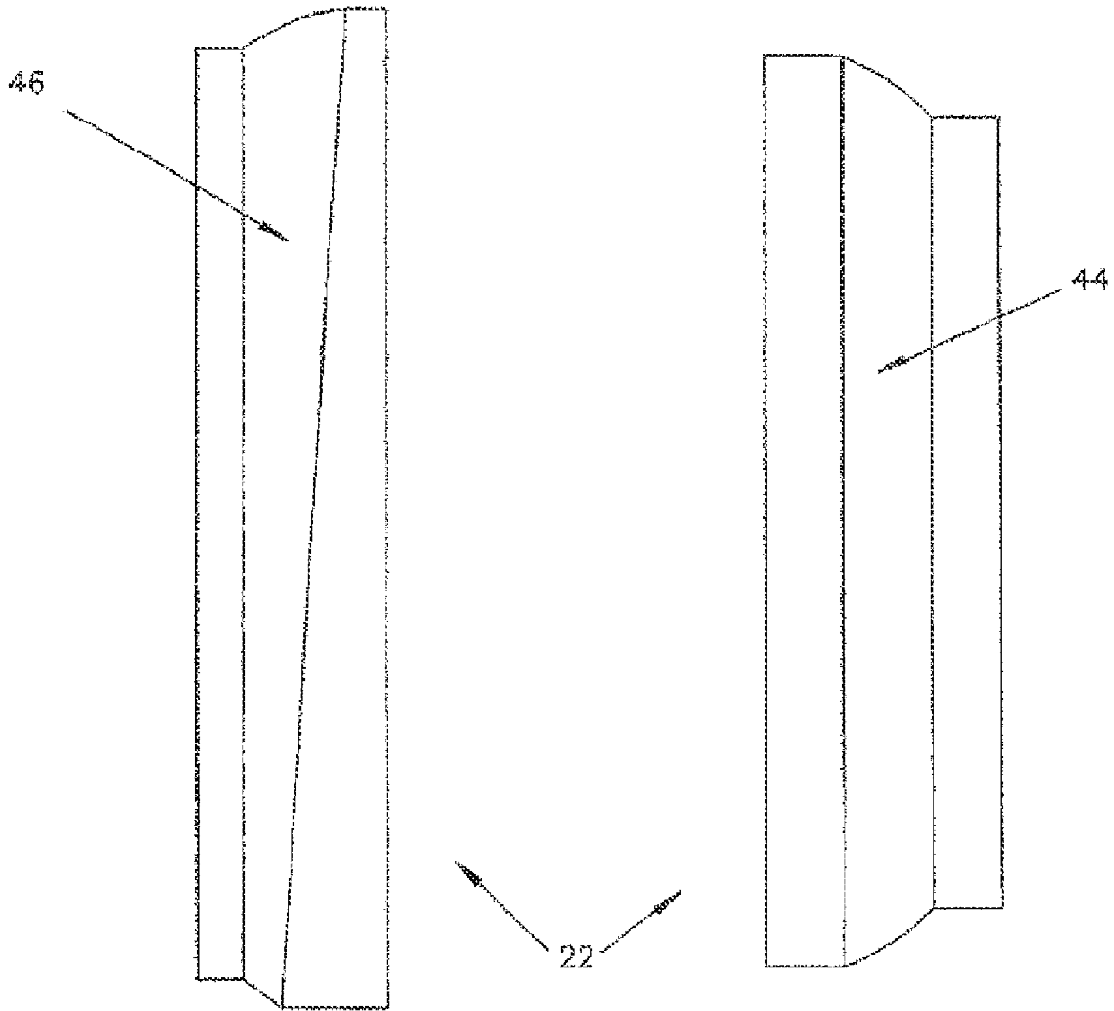
TOP VIEW
