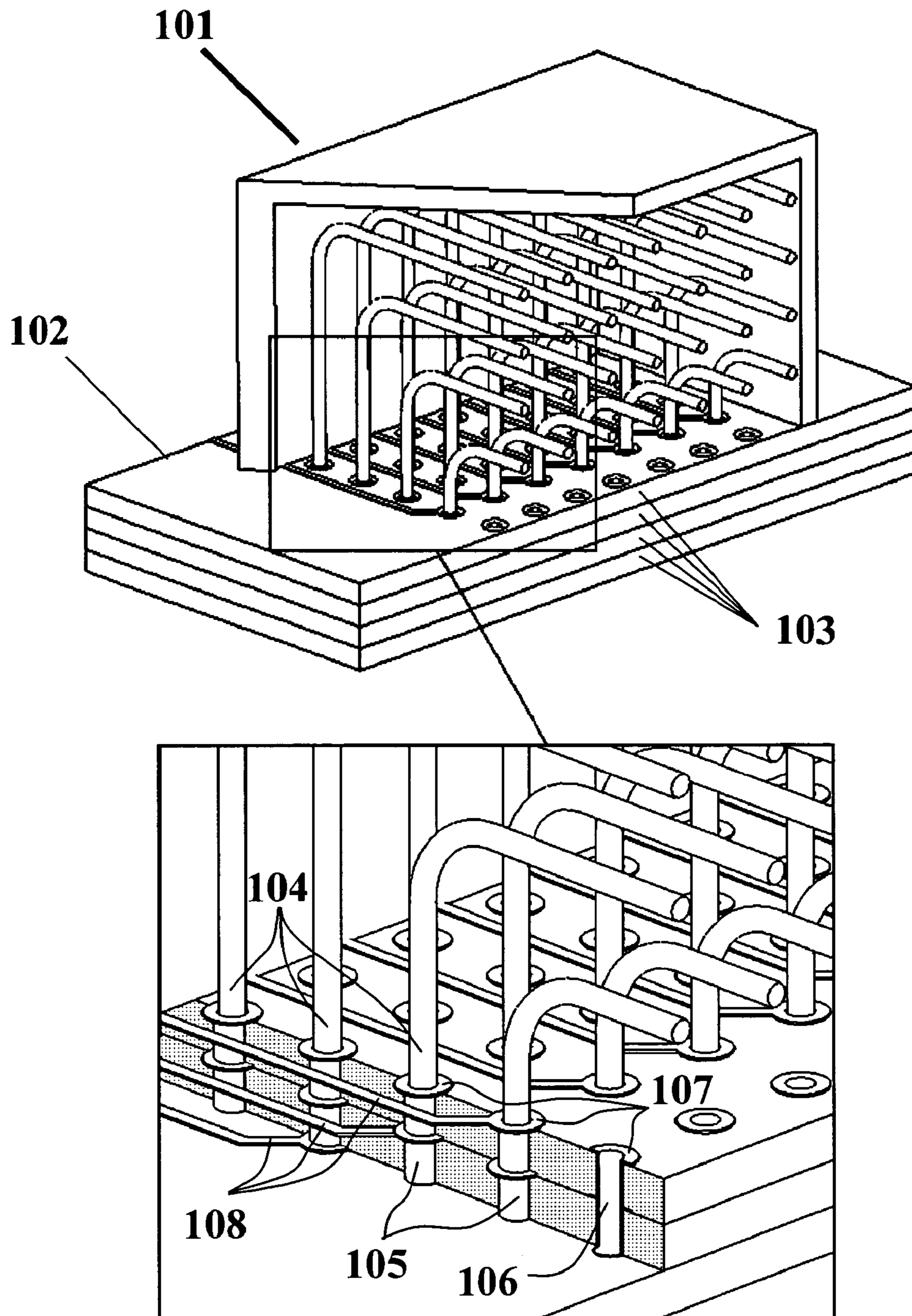
FIGURE 1 PRIOR ART
