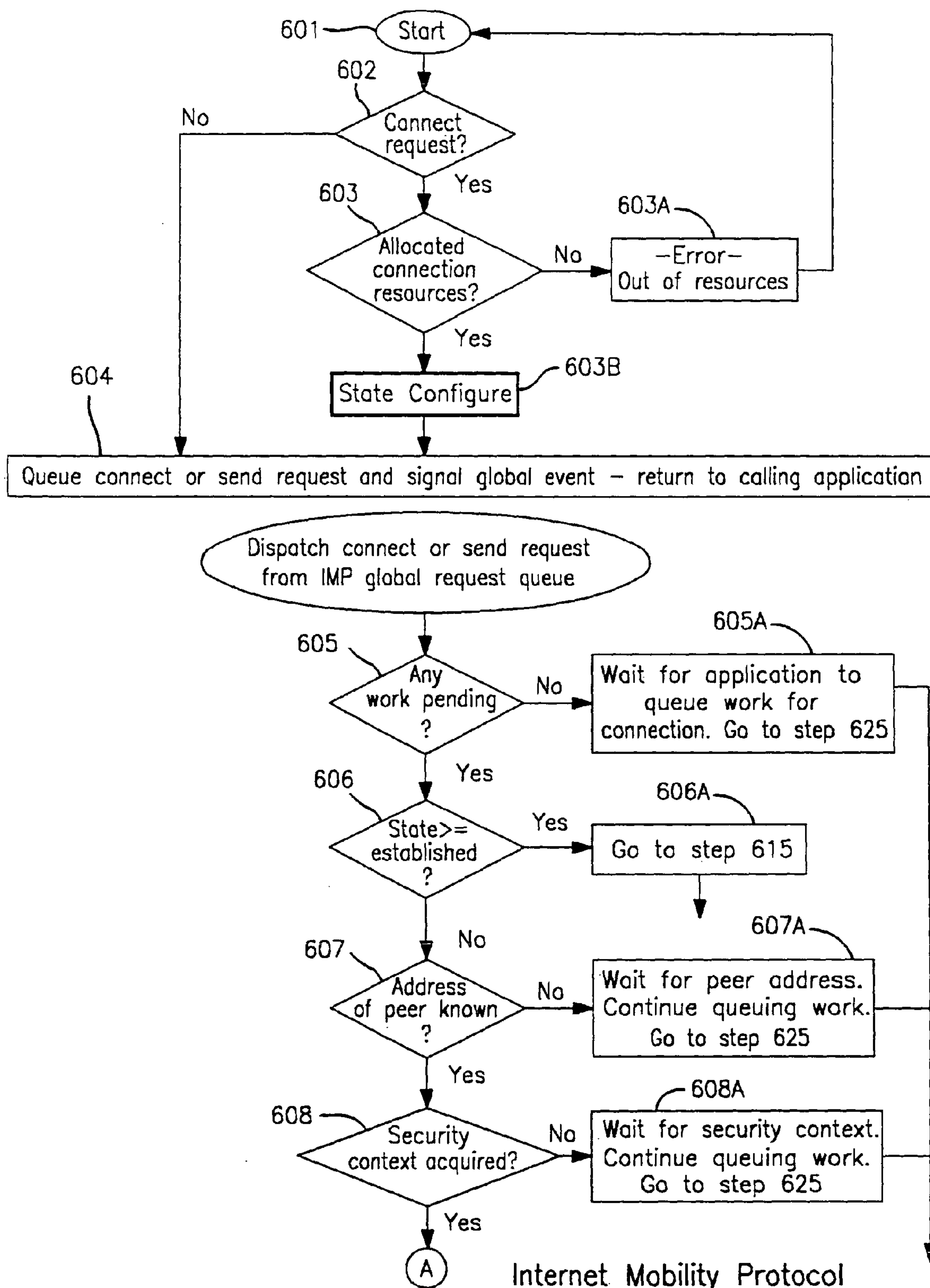
FIG. 10A Connect and Send request logic
