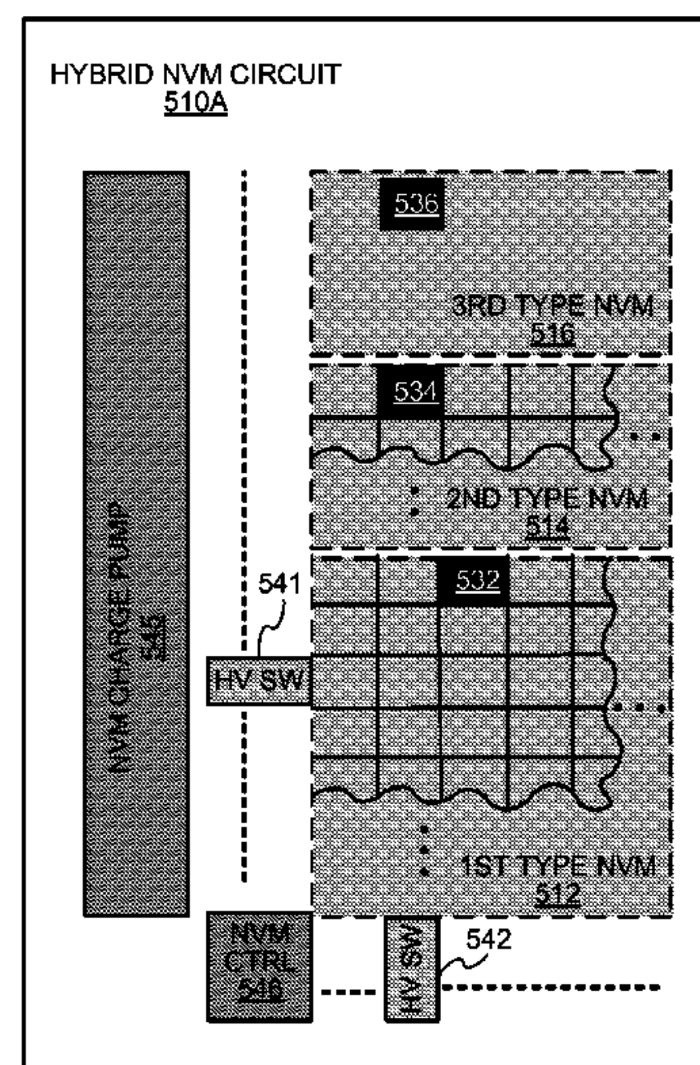
HYBRID NVM WITH HIGH VOLTAGE SWITCHES
