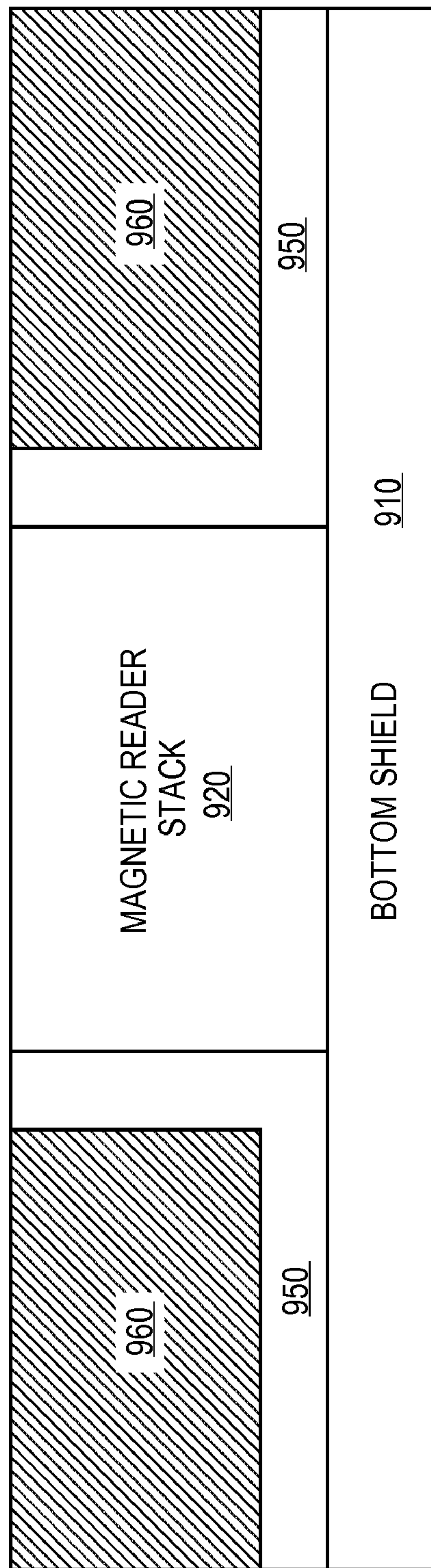
CROSS-SECTIONAL VIEW
