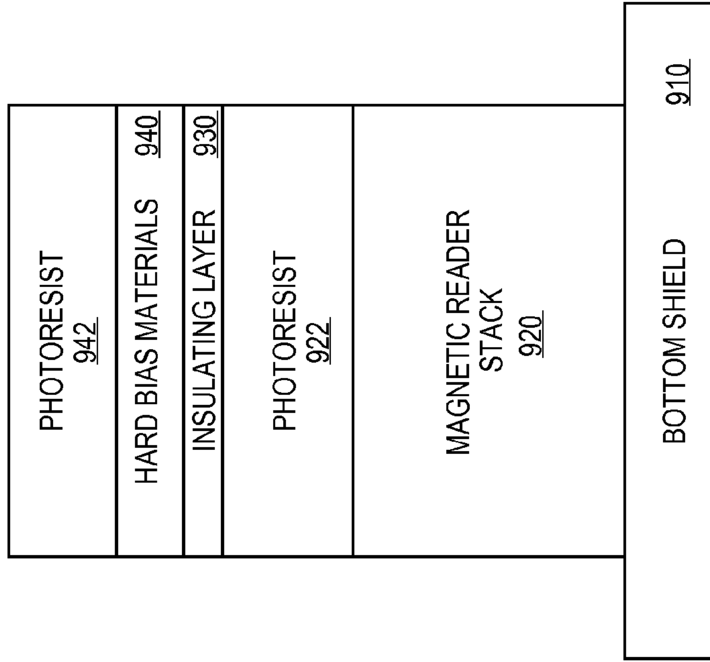
CROSS-SECTIONAL VIEW
