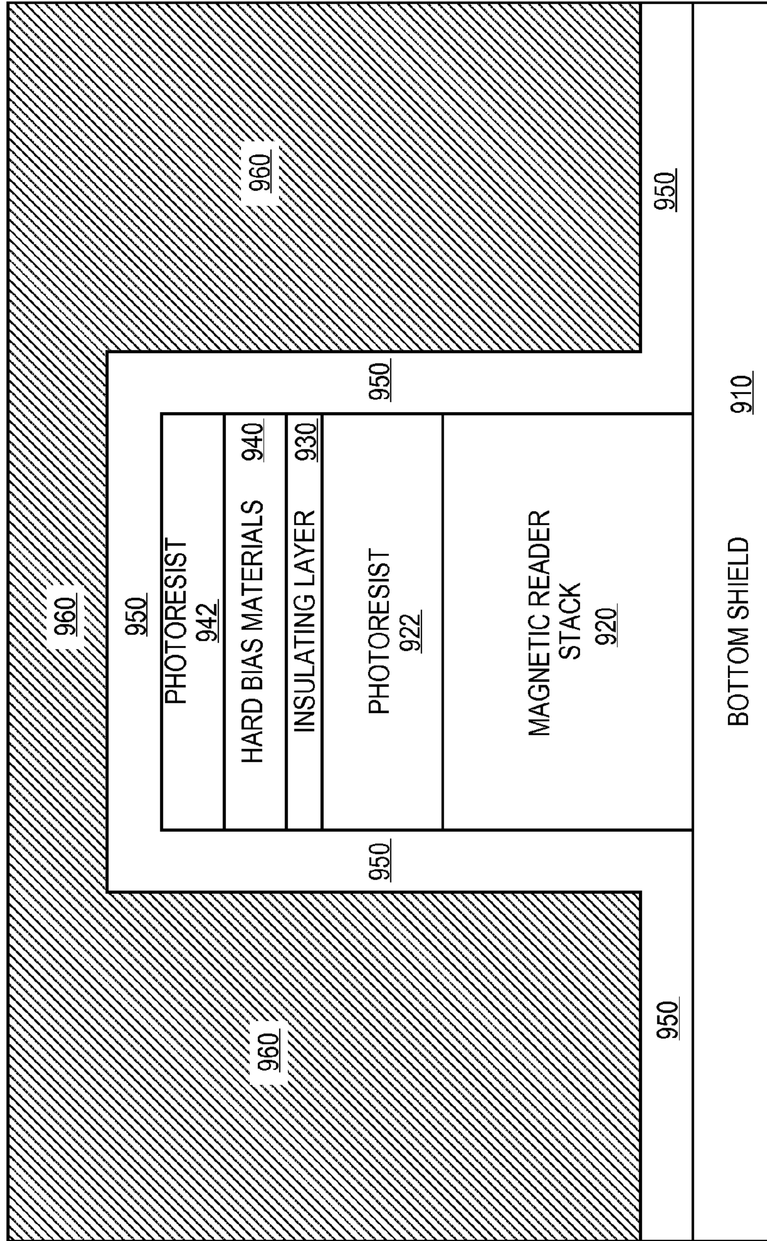
CROSS-SECTIONAL VIEW
