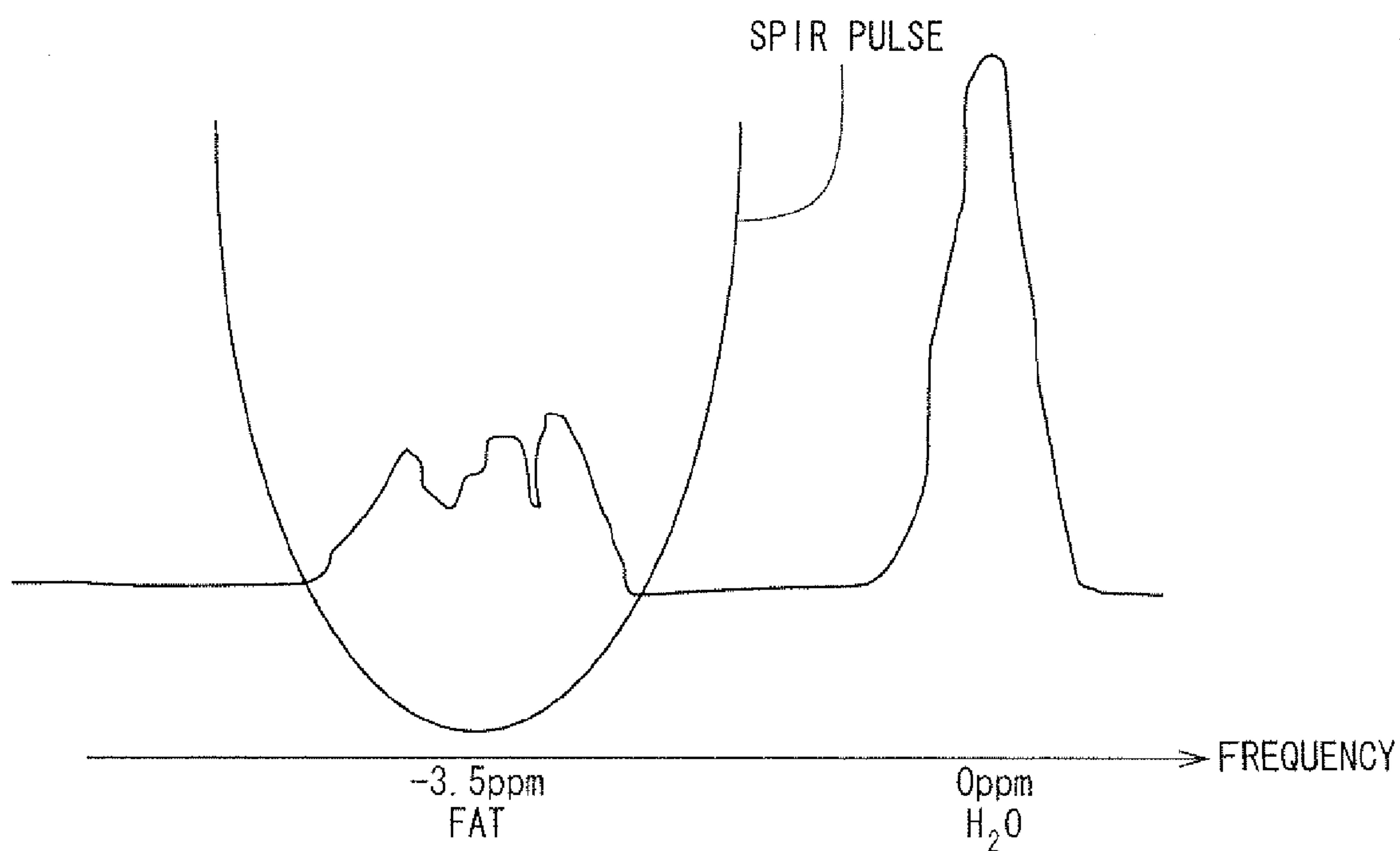
FIG. 2 PRIOR ART
