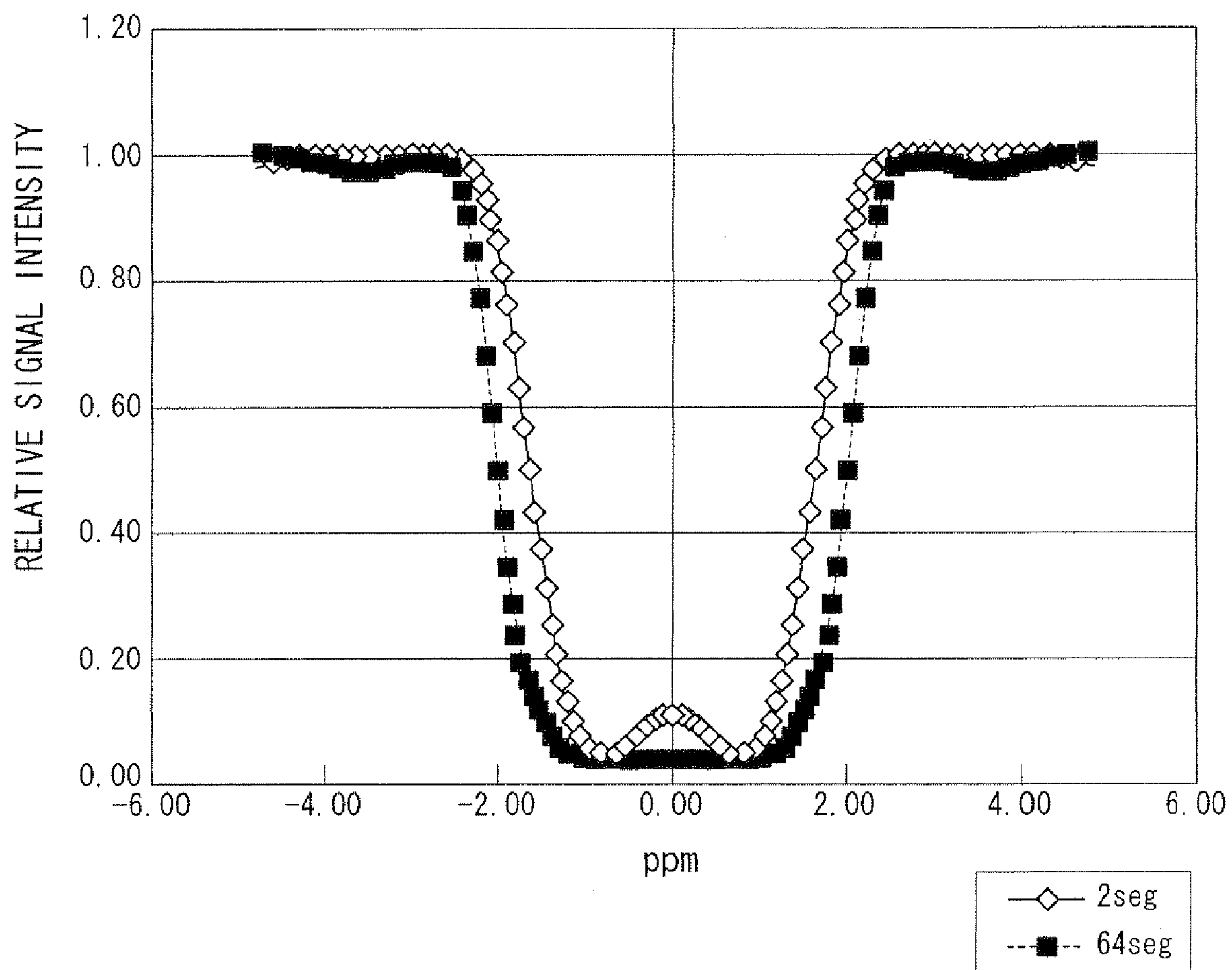
FIG. 8 PRIOR ART
