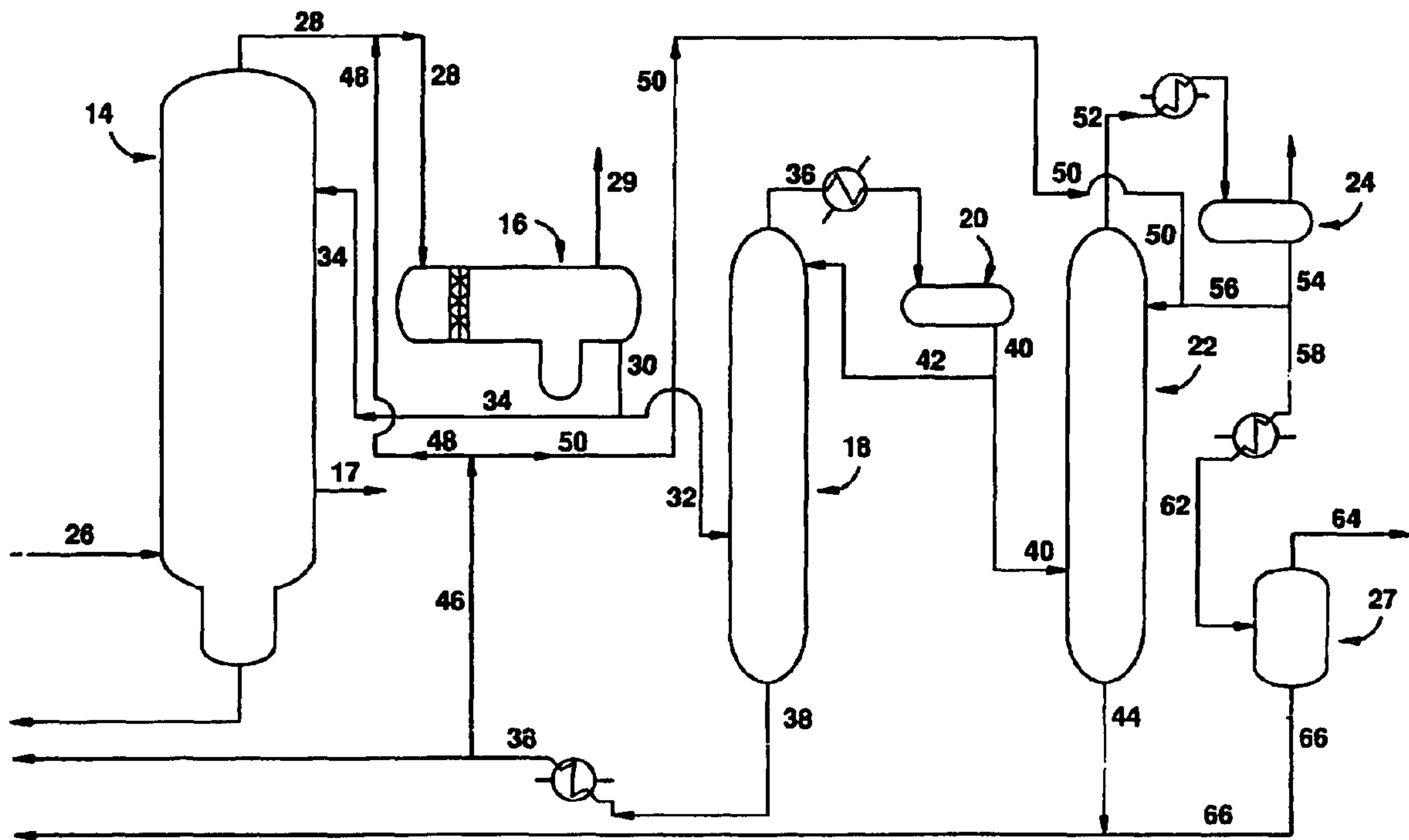
FIG.1 (PRIOR ART)
