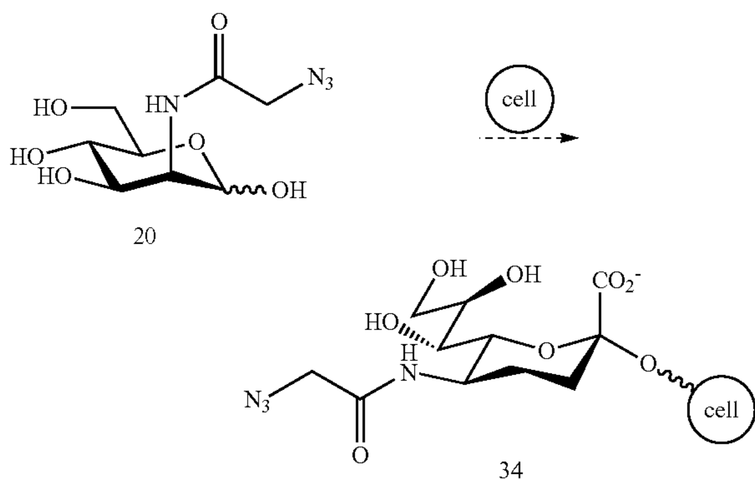
Scheme 10
