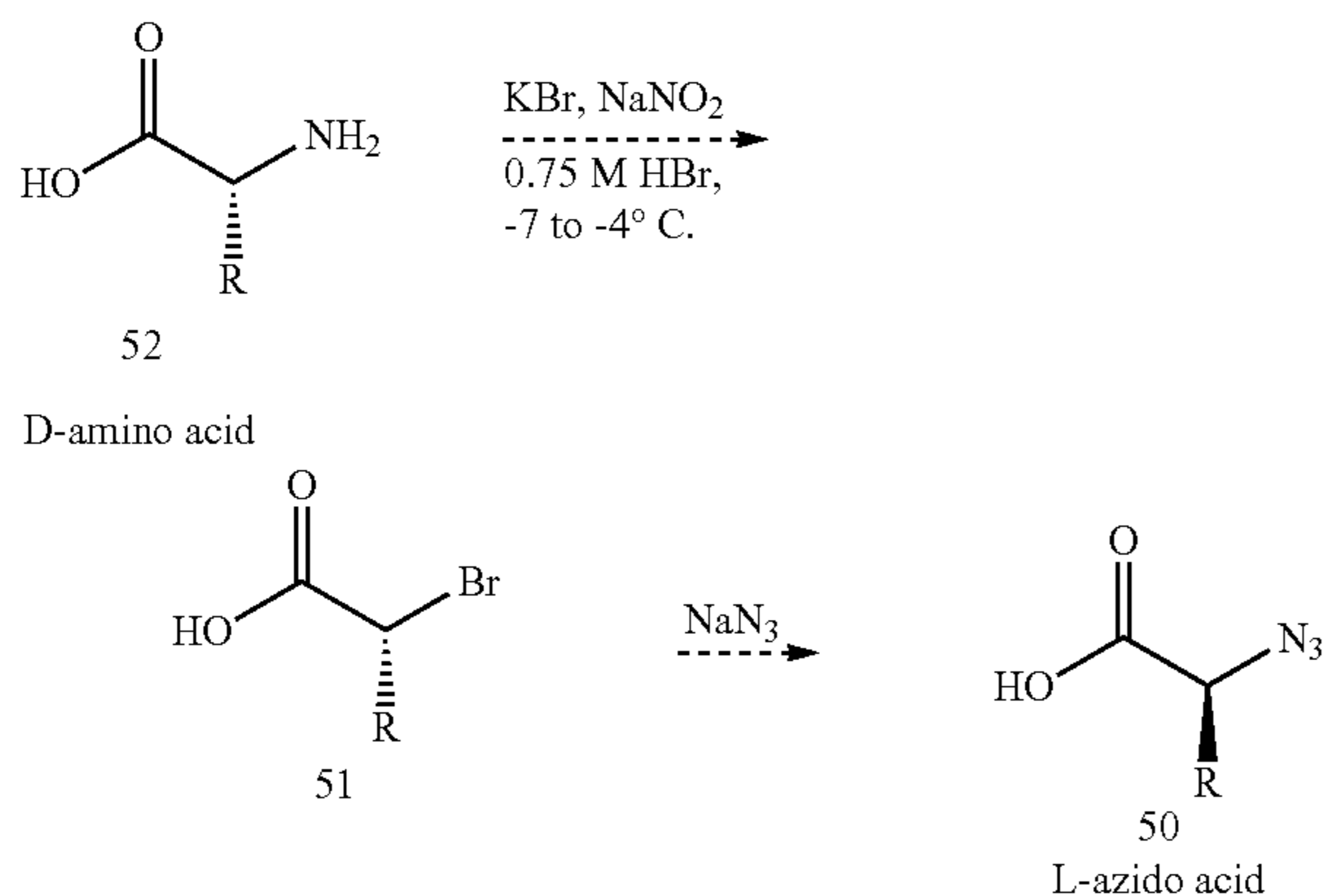
Scheme 15
