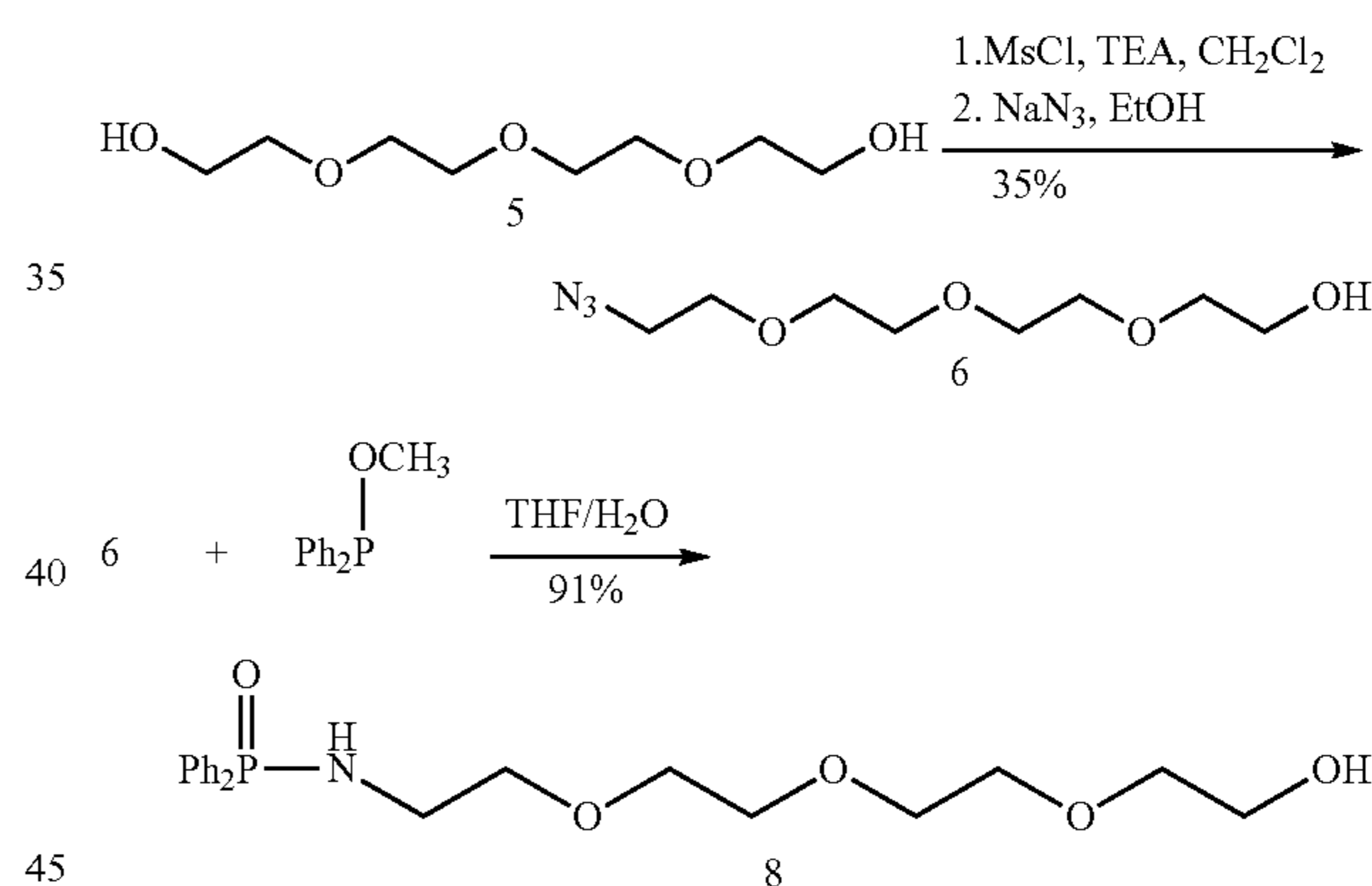
Scheme 2
