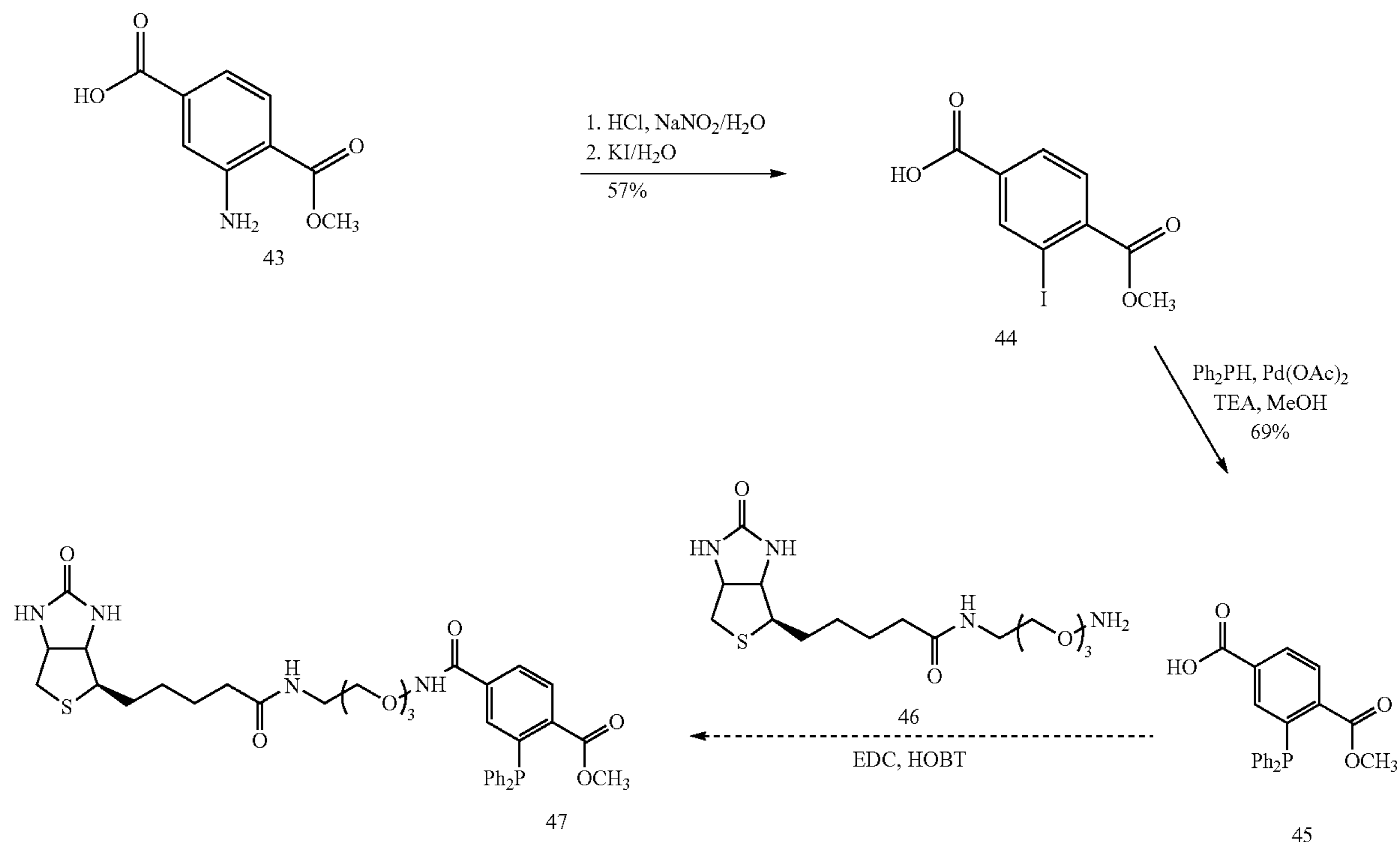
Scheme 12
