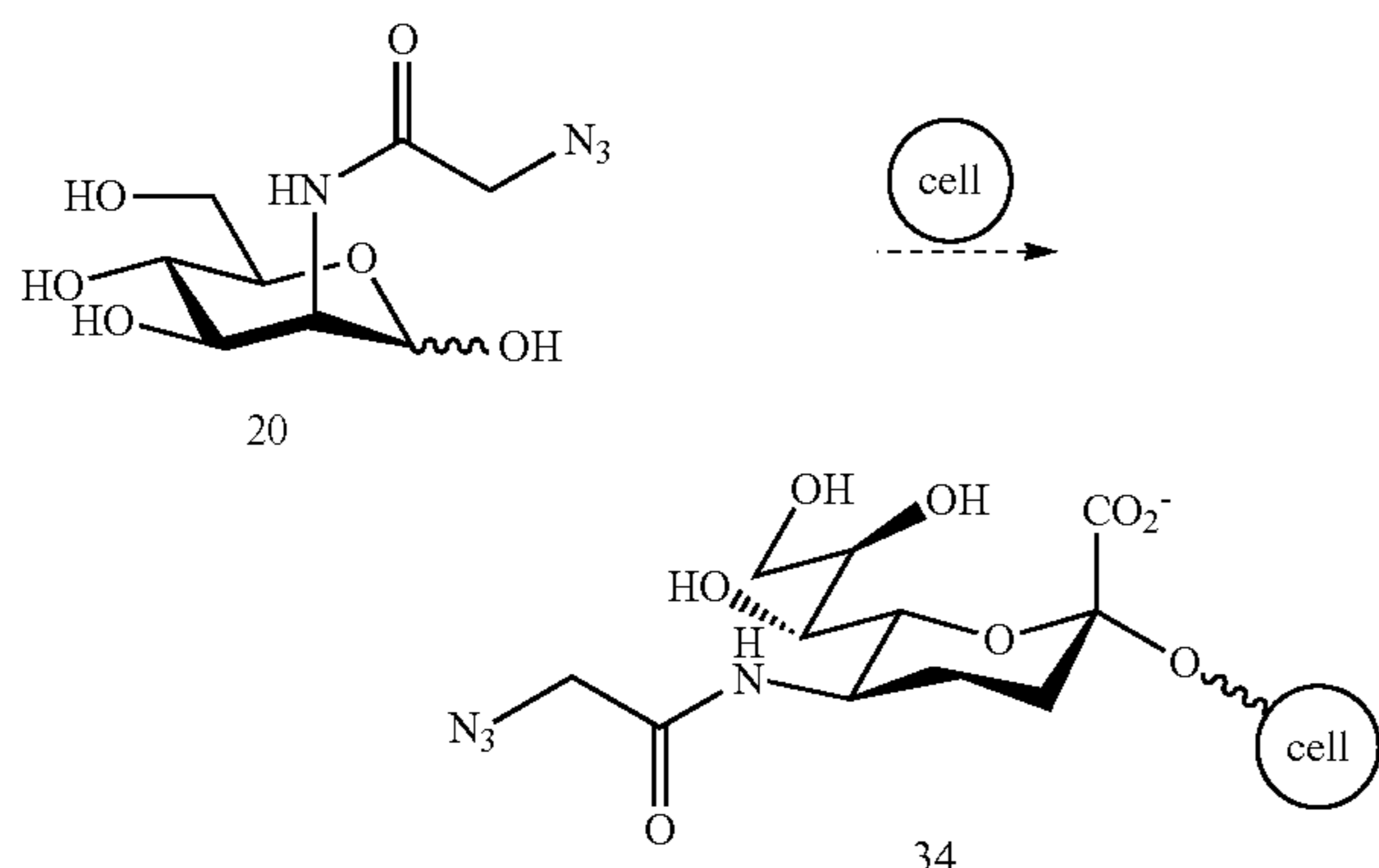
Scheme 10
