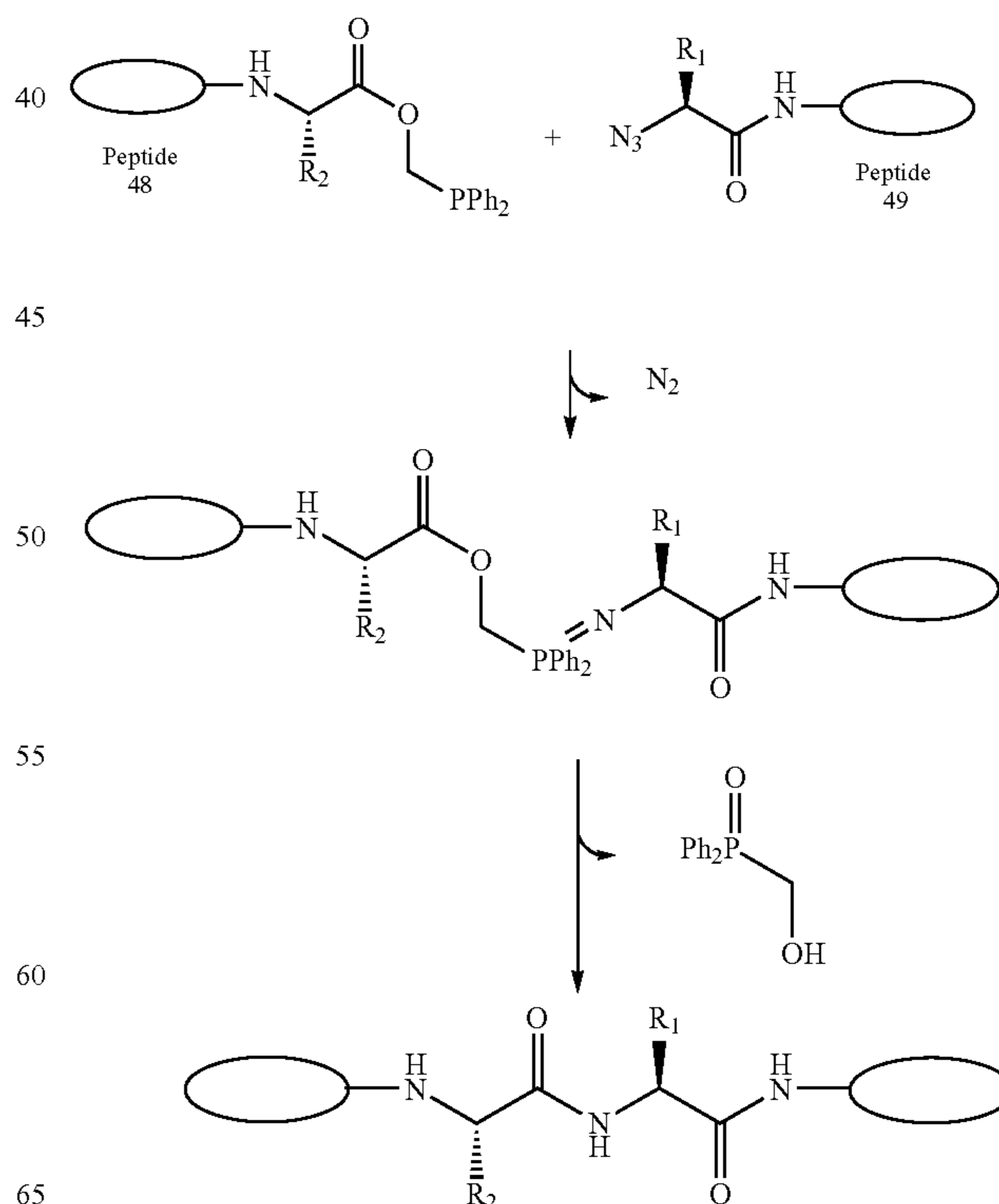
Scheme 14
