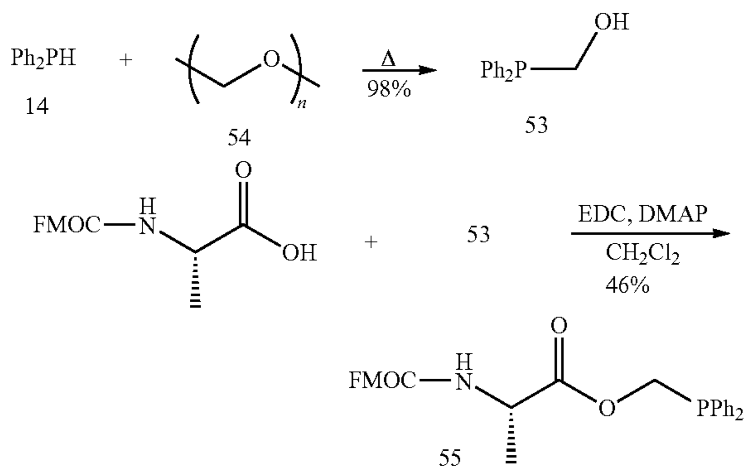
Scheme 16
