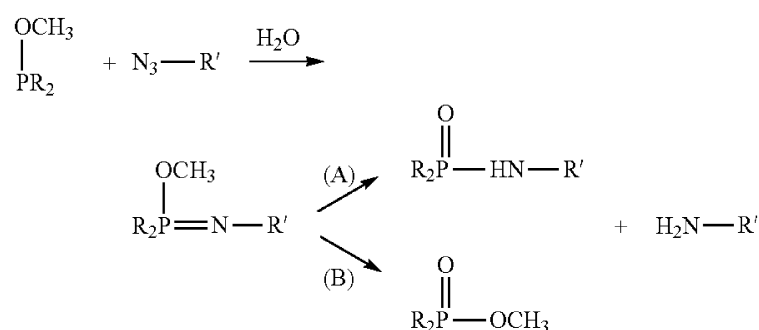
Scheme 1
