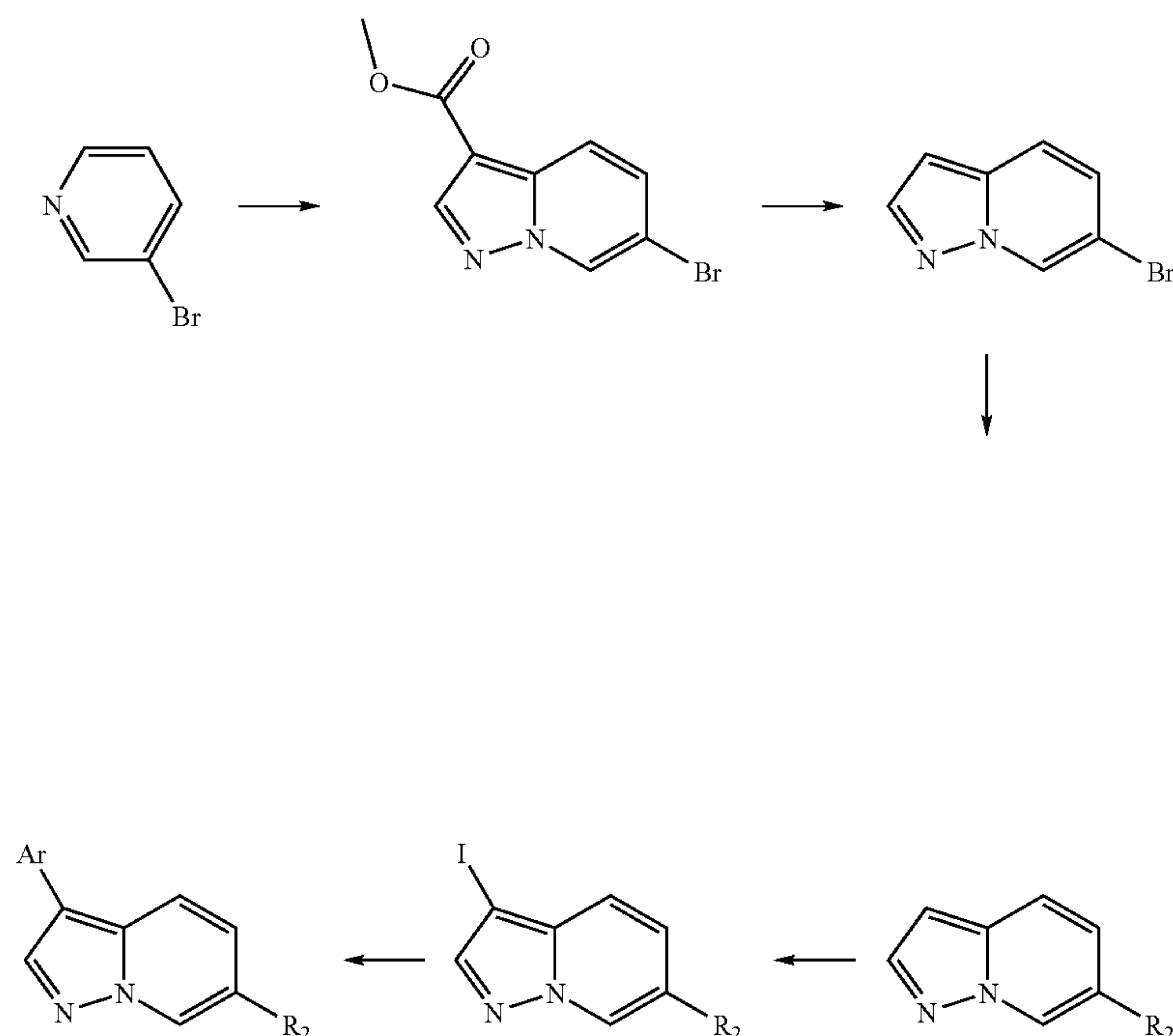
Scheme 7
