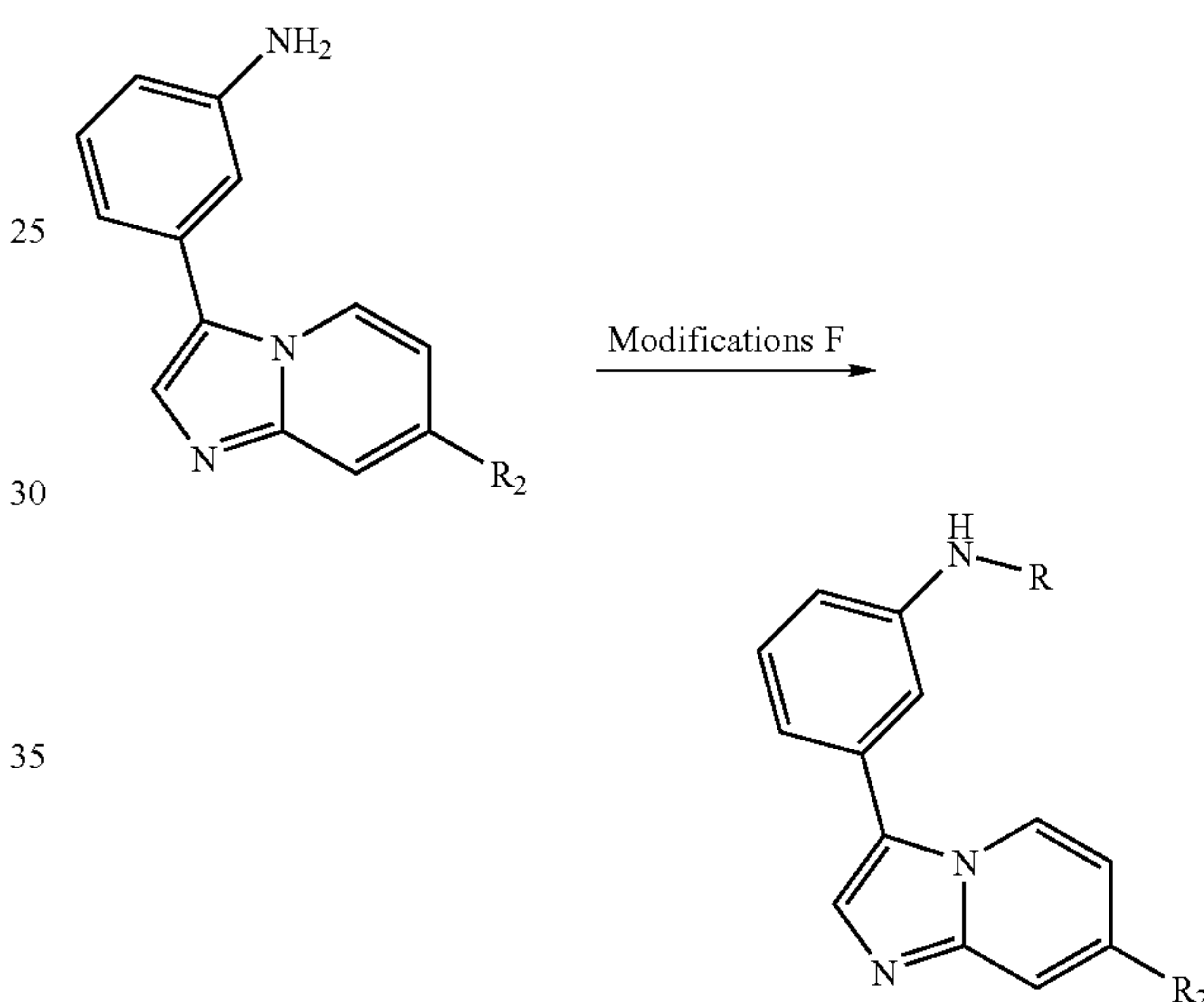
Scheme 3
