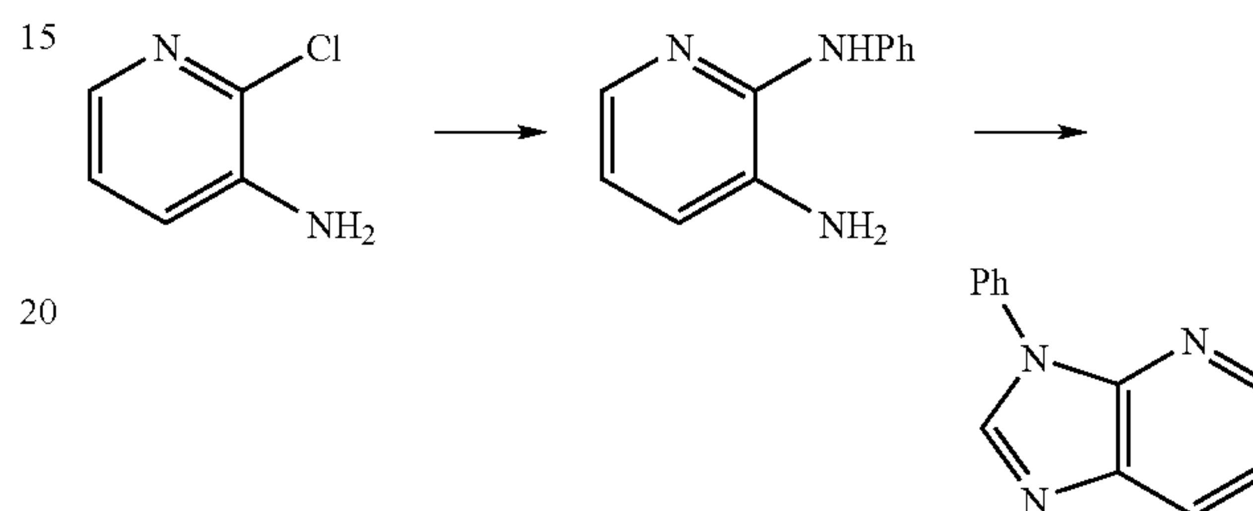
Scheme 8
