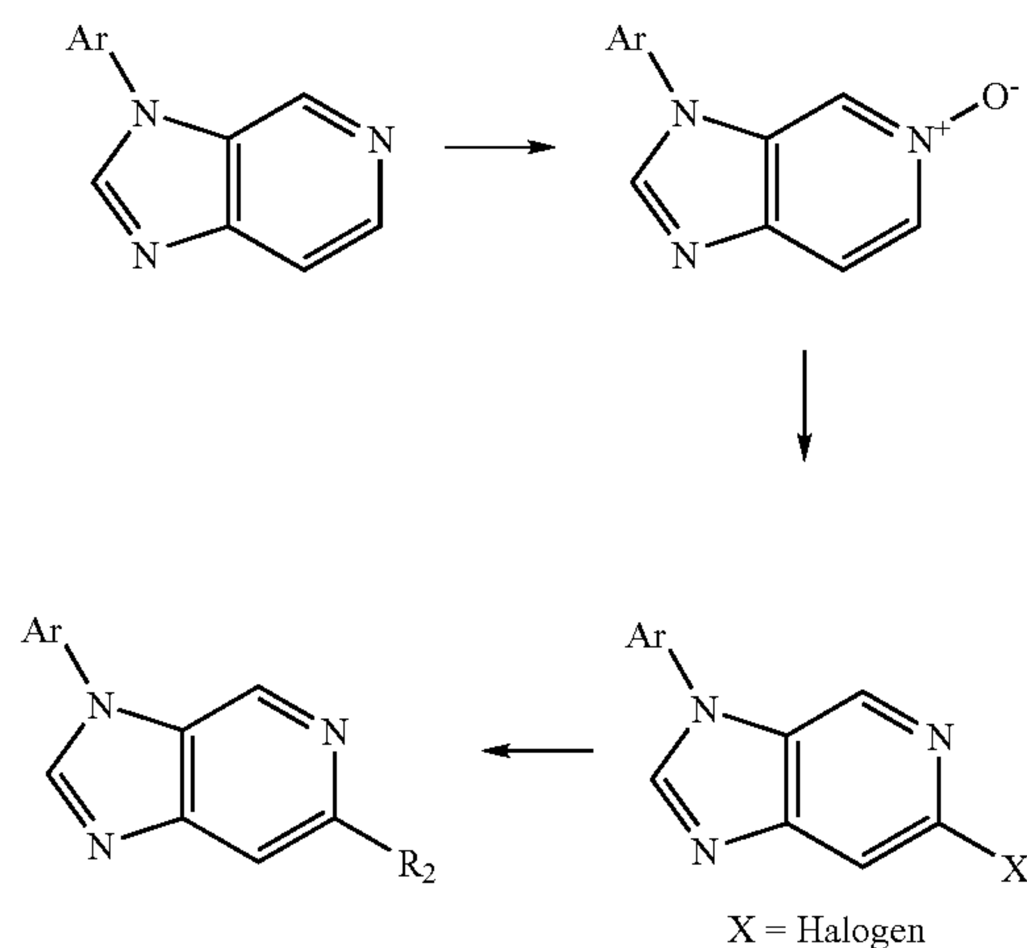
Scheme 11
