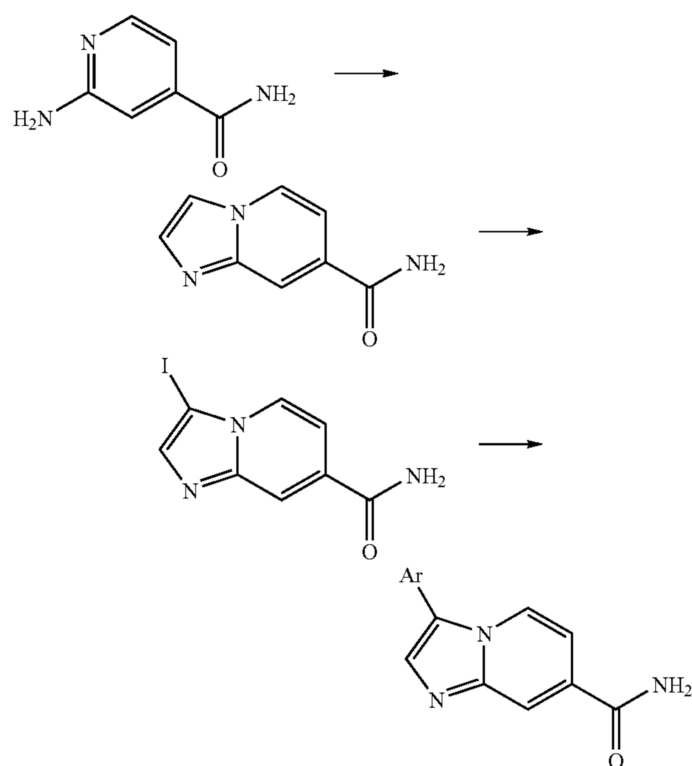
Scheme 1C
