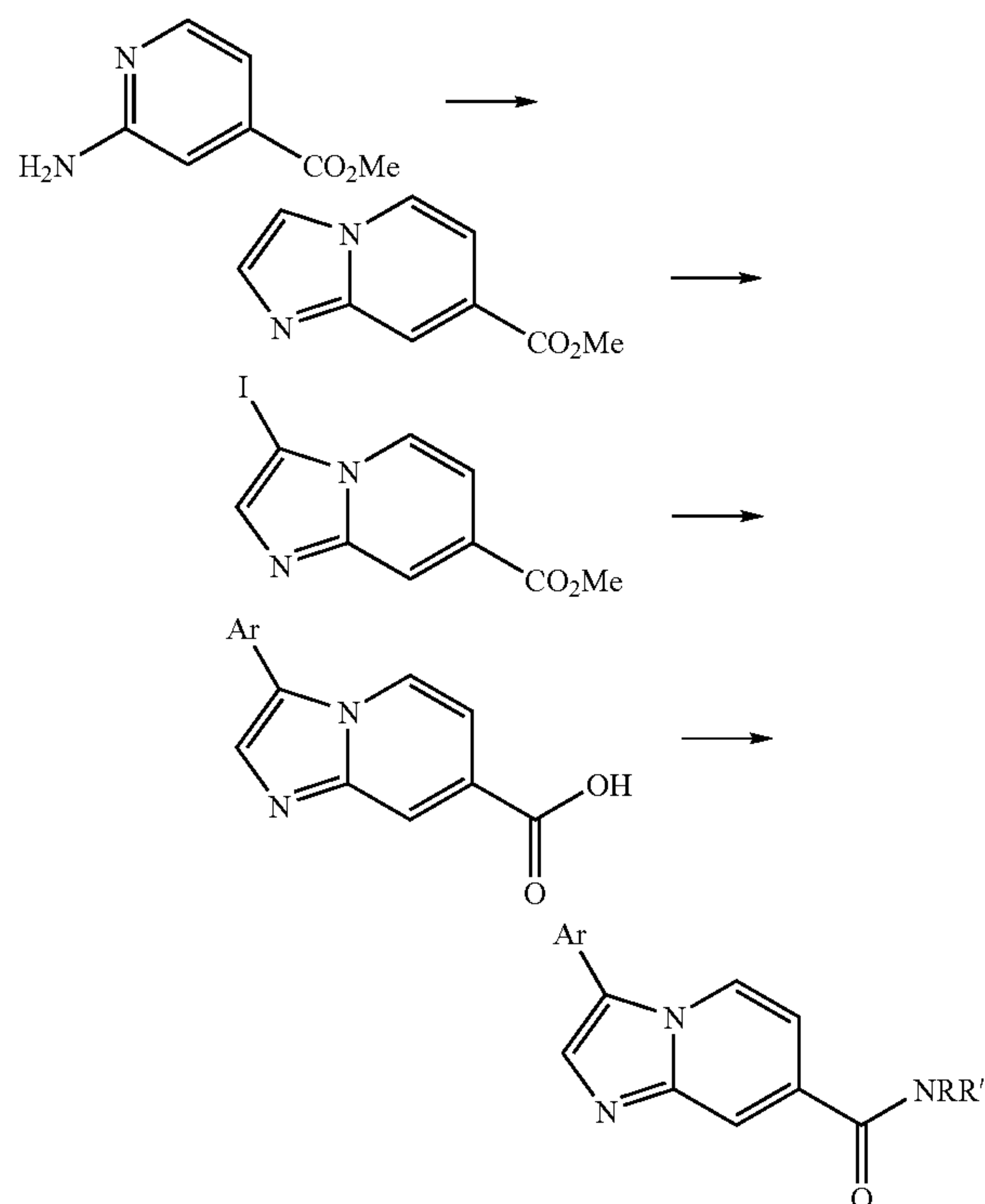
Scheme 1B
