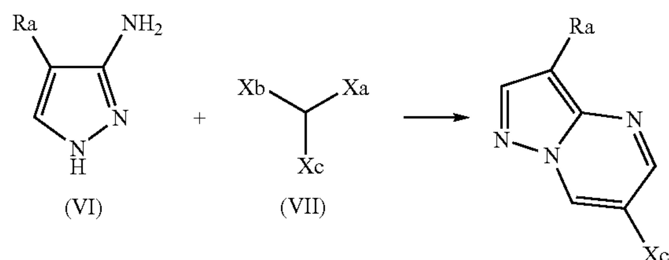
Scheme 5A
