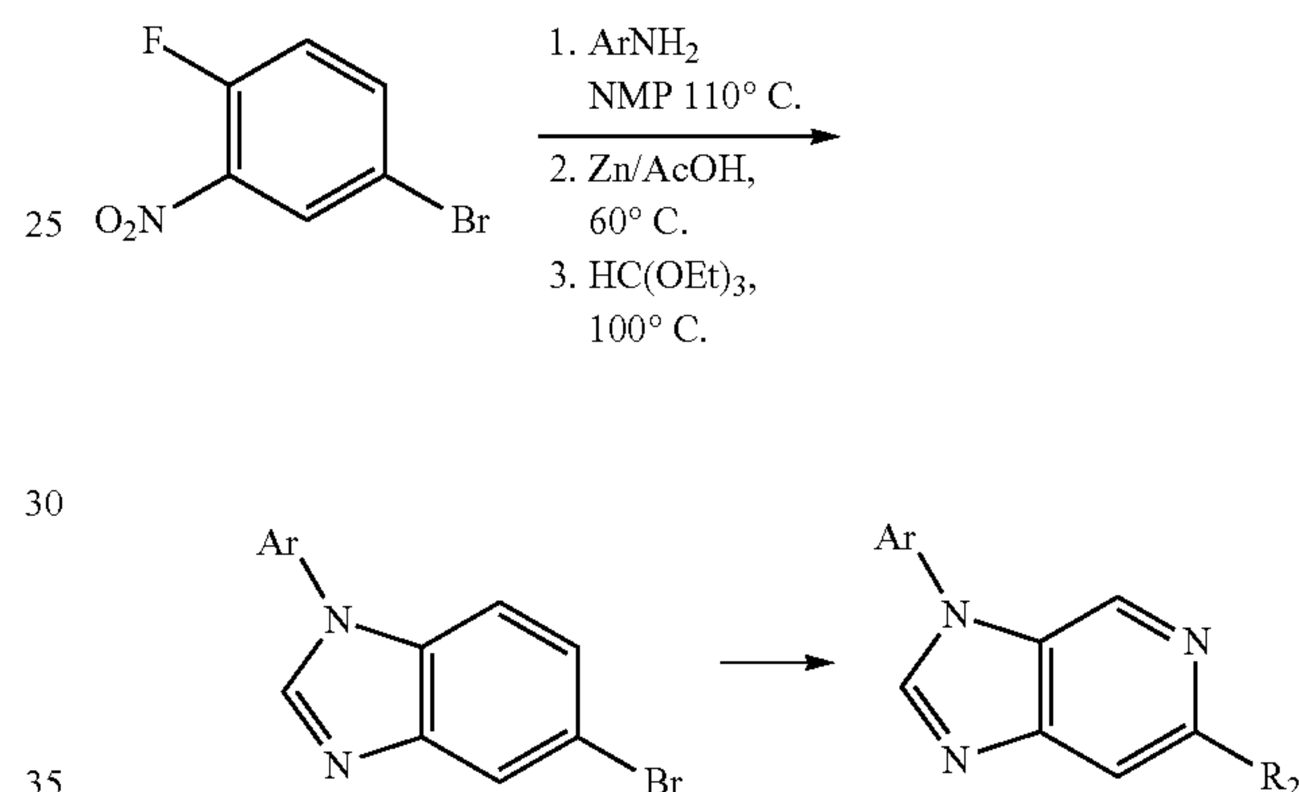
Scheme 13
