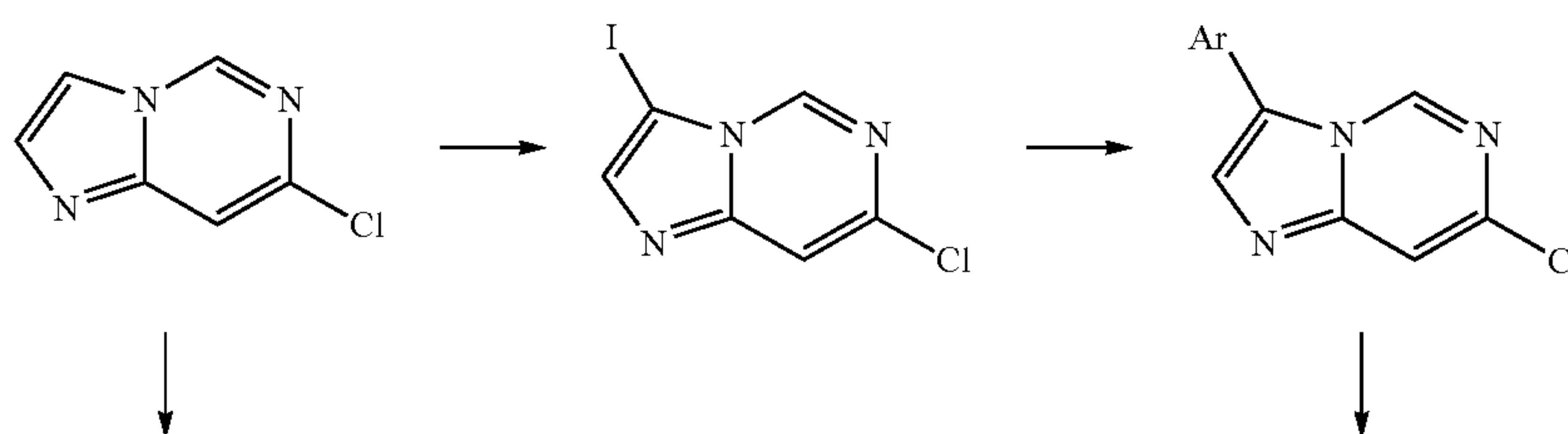
Scheme 14
