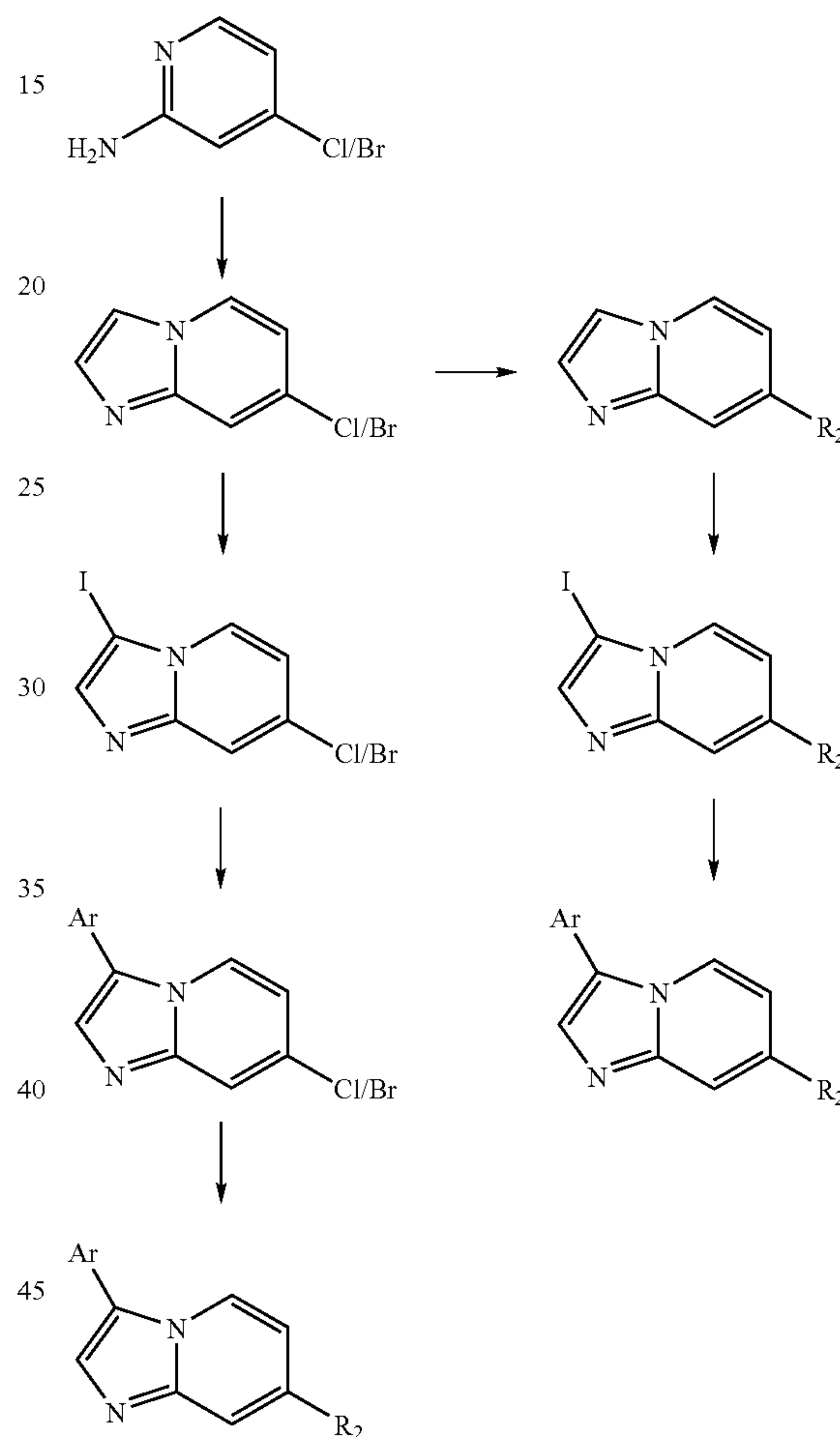
Scheme 2
