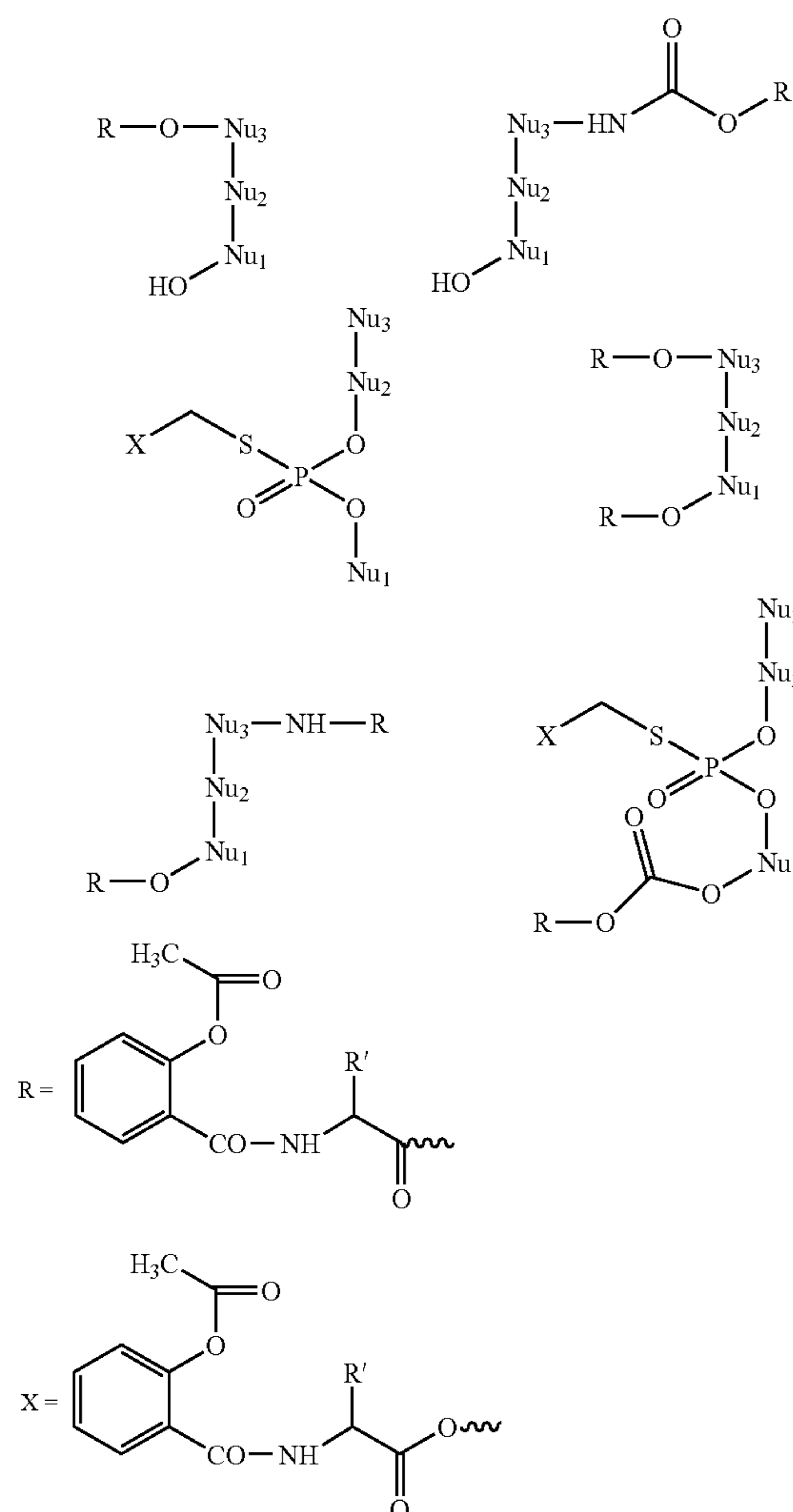
Scheme 3
