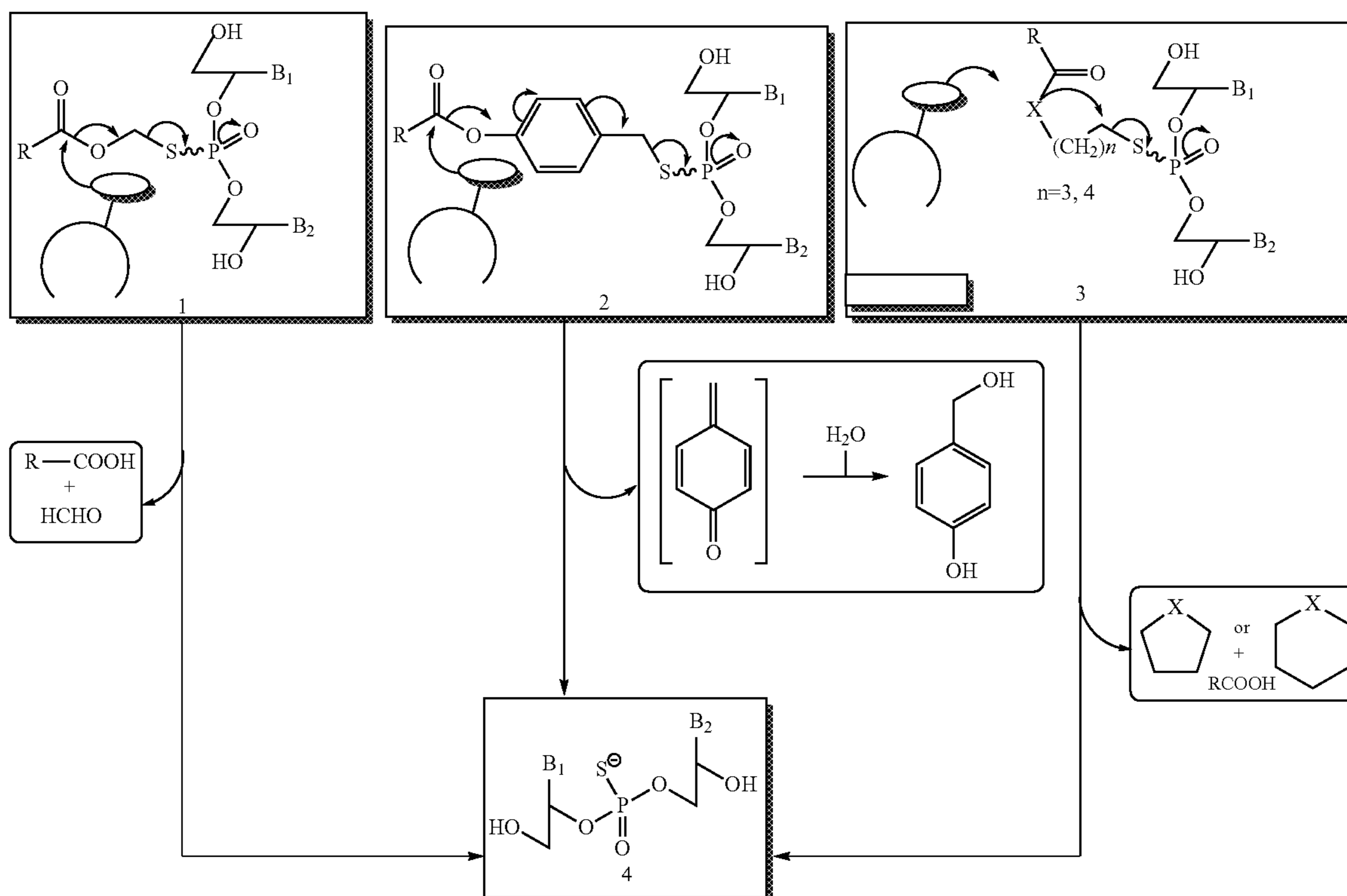
Scheme 1
