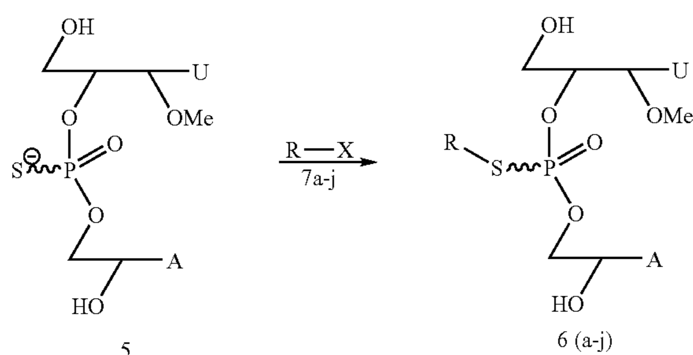
Scheme 4
