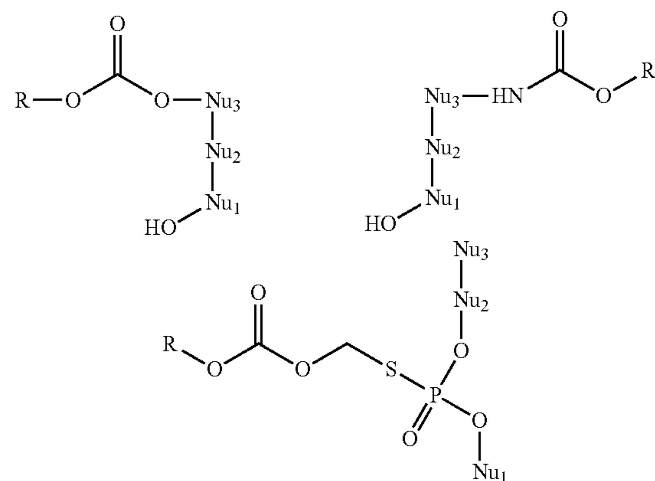
Scheme 2
