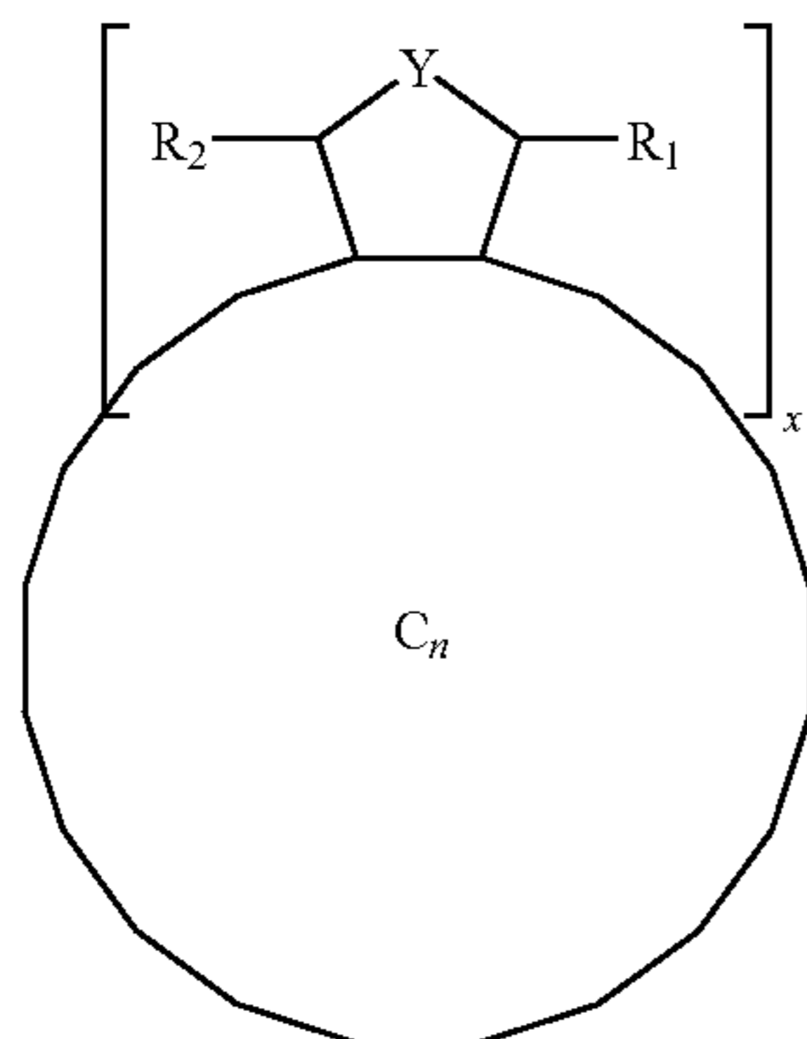
Diels Alder Derivative
