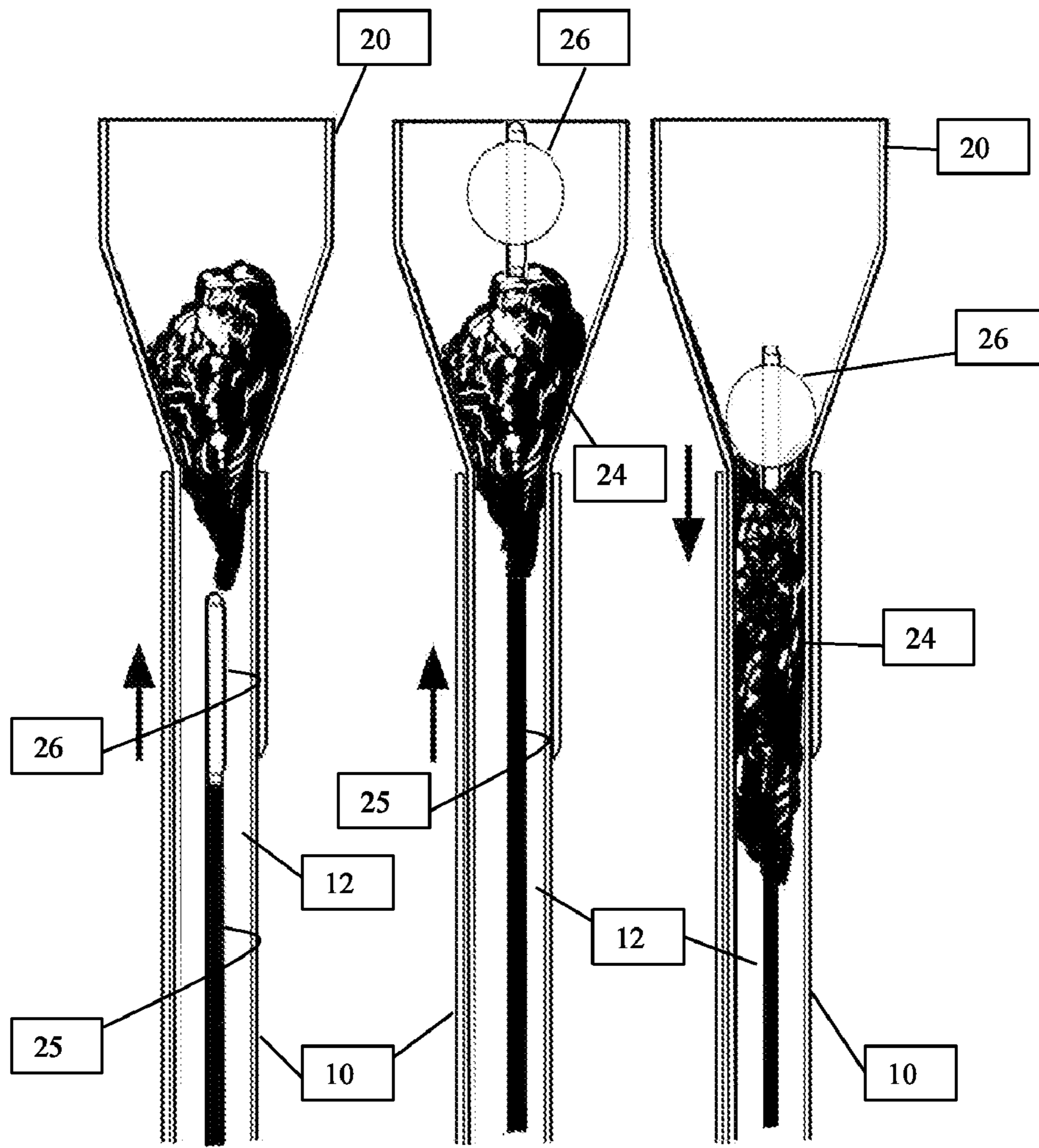
Cross section of catheter with eccentric balloon
