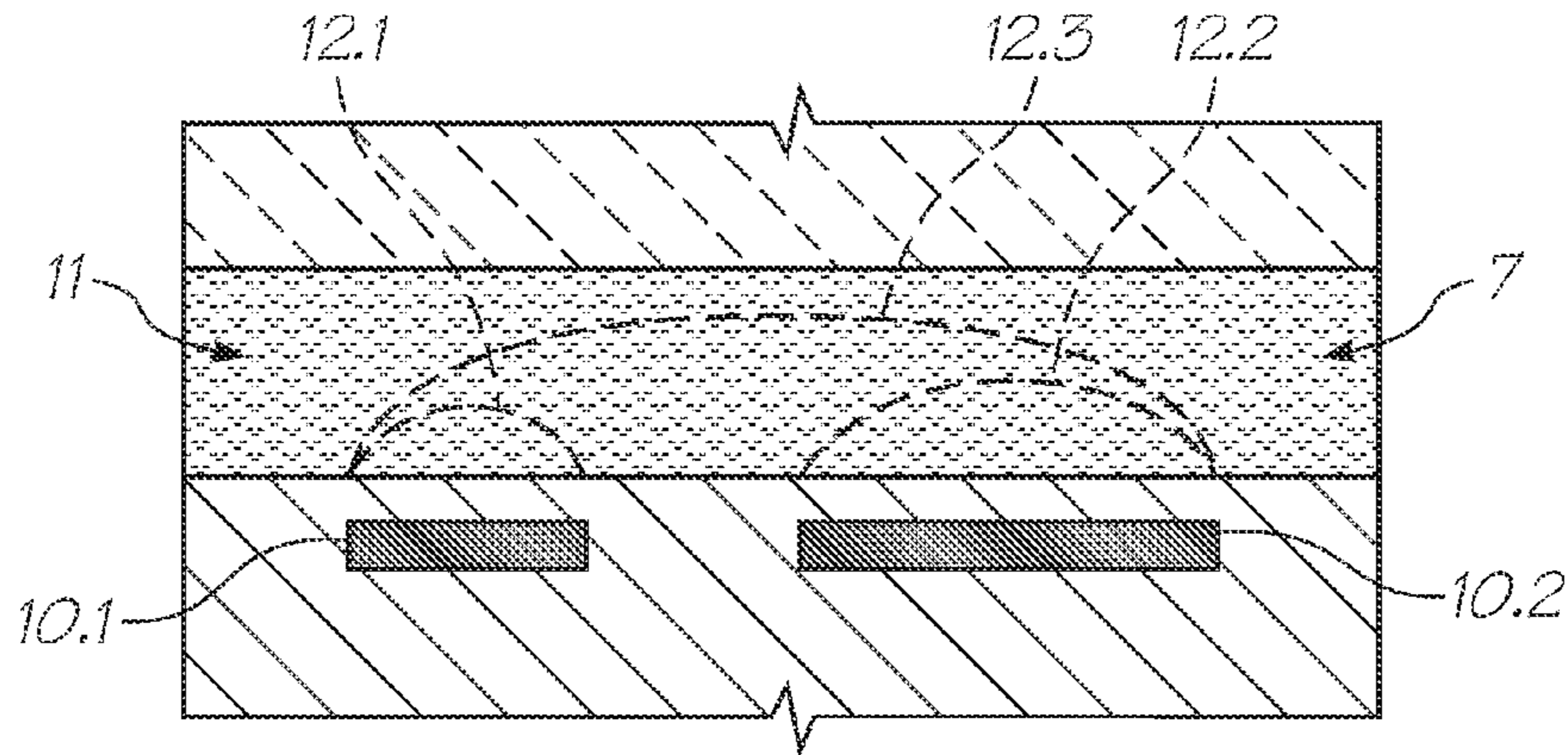
FIG. 52 (PRIOR ART)
