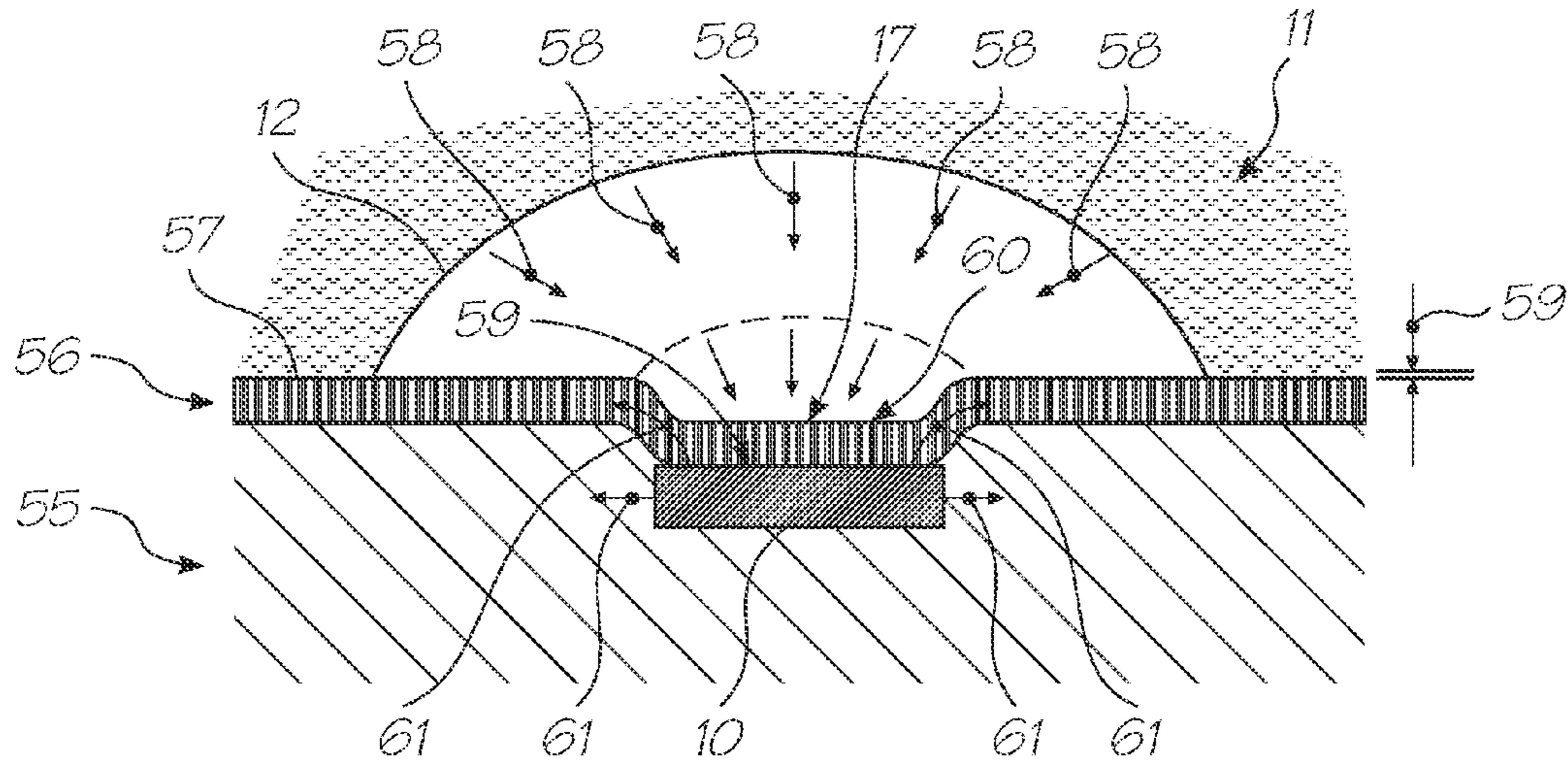
FIG. 47 (PRIOR ART)
