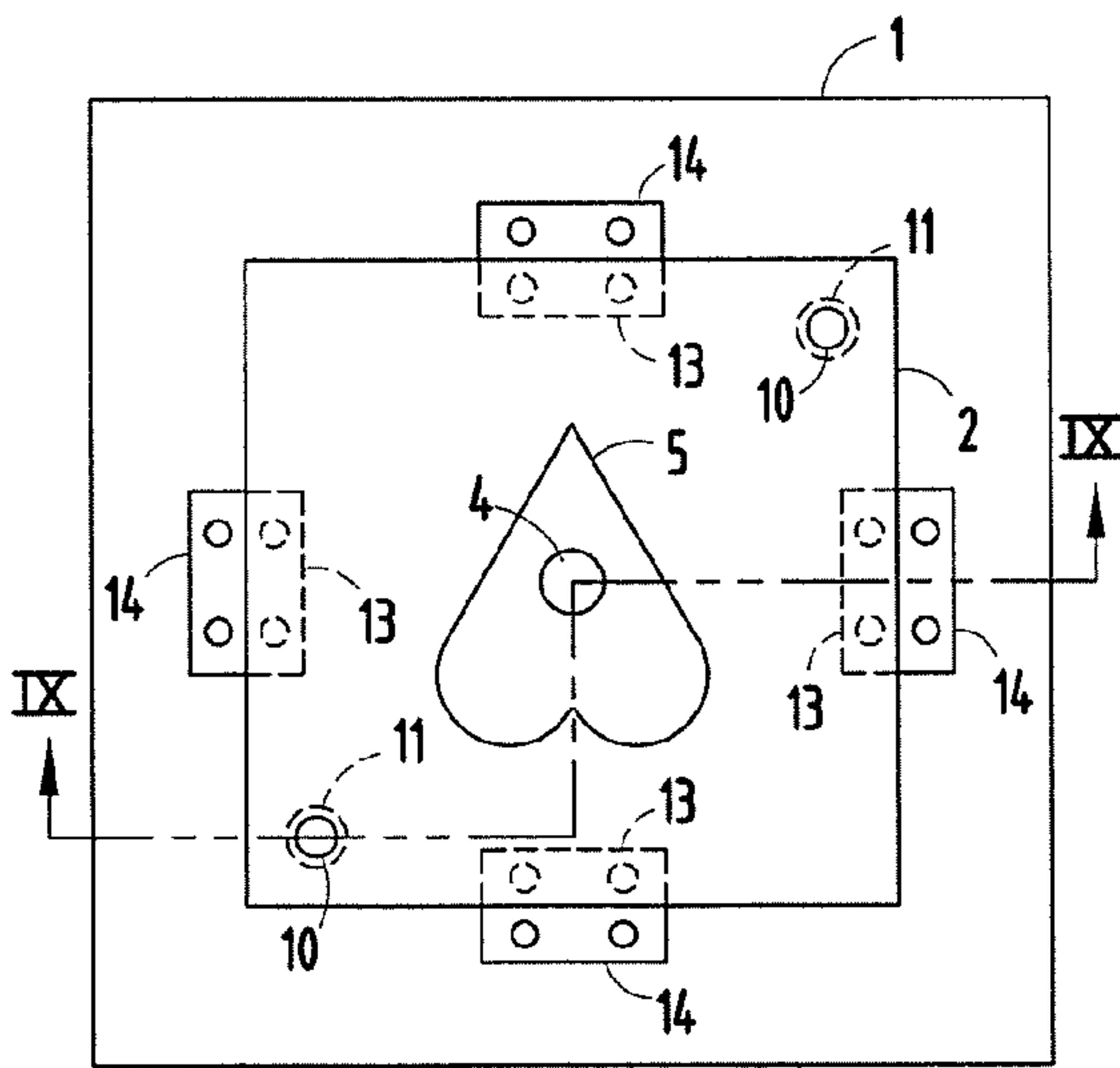
FIG. 8 PRIOR ART
