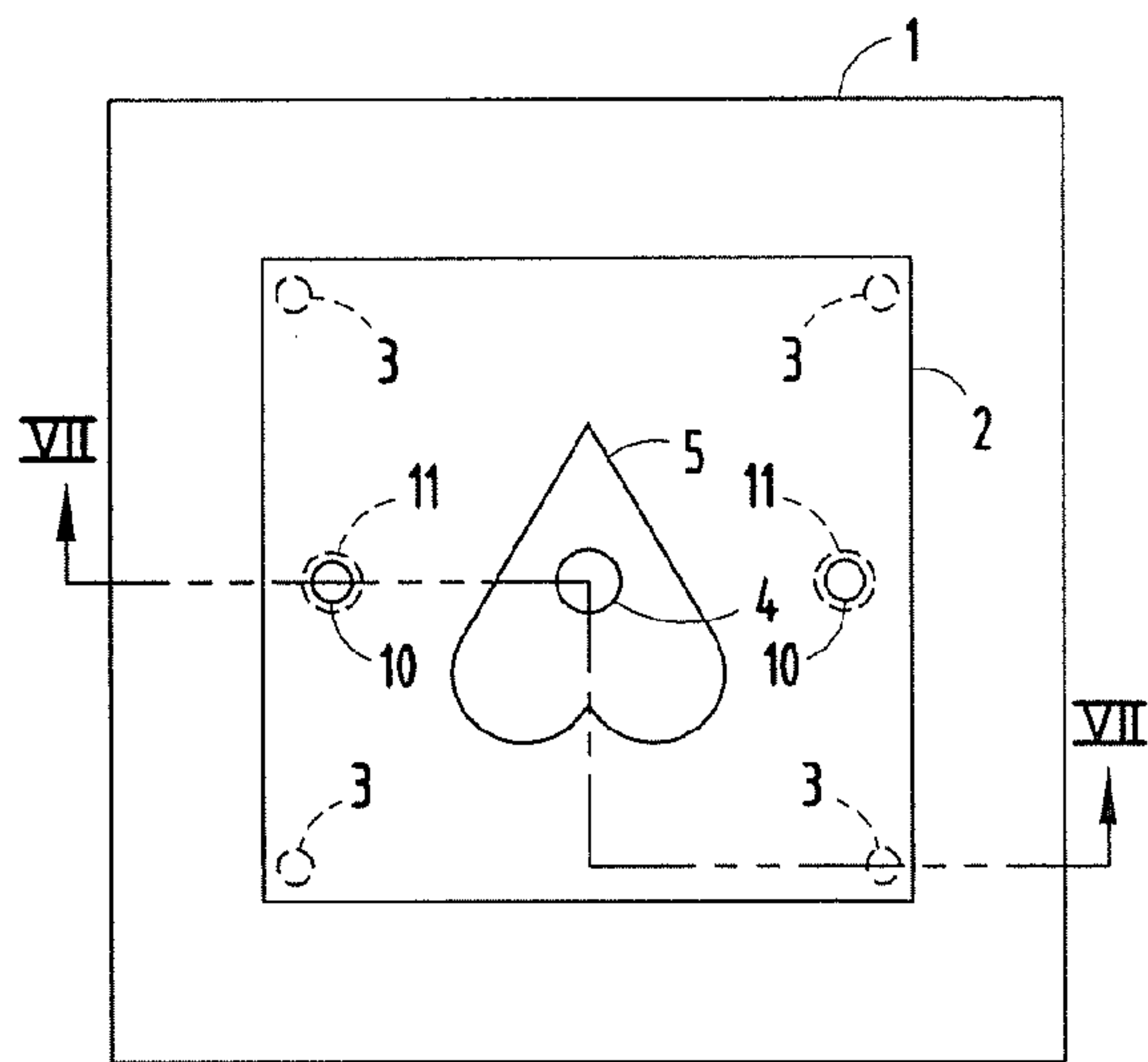
FIG. 6 PRIOR ART
