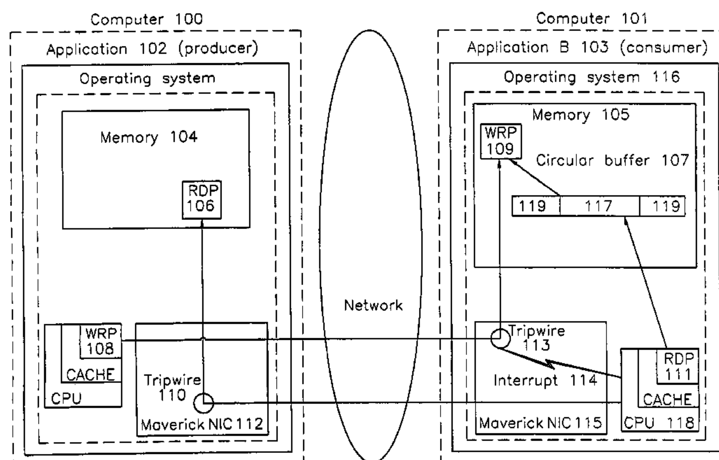
Circular buffer support using the NIC of FIG.6.
