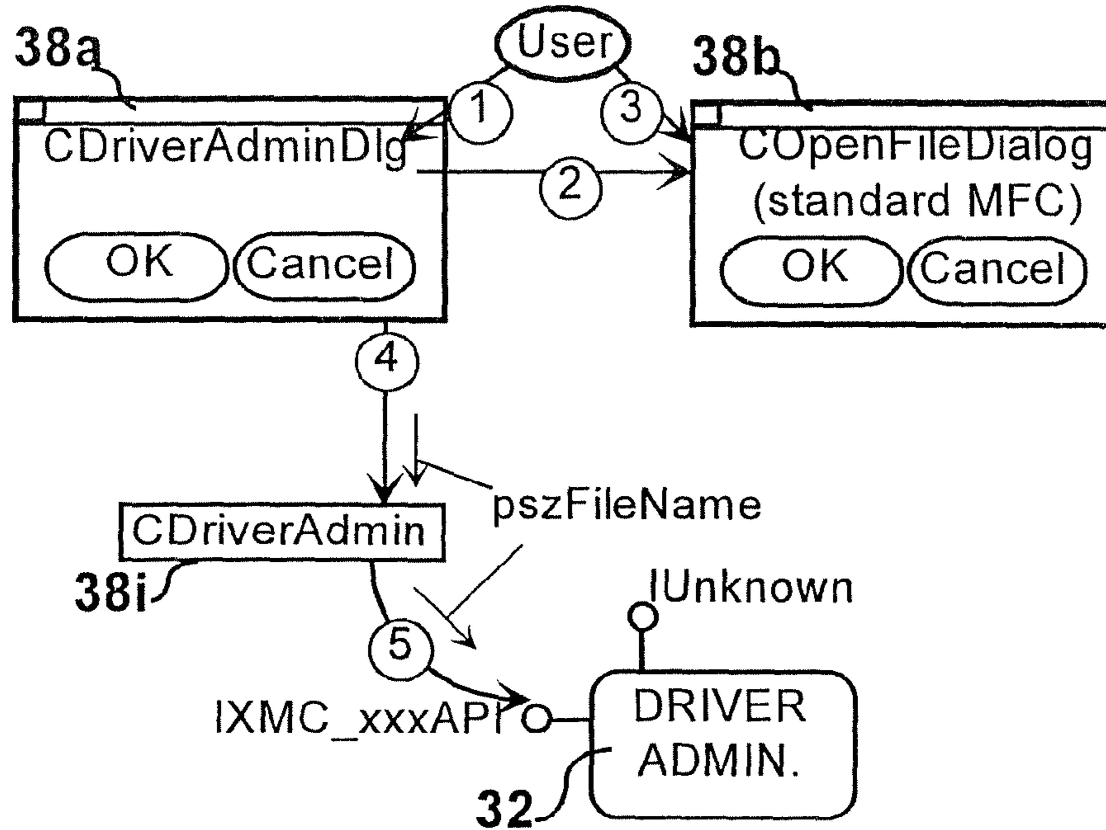
FIG. 55 Scenario-Map - Adding a Driver
