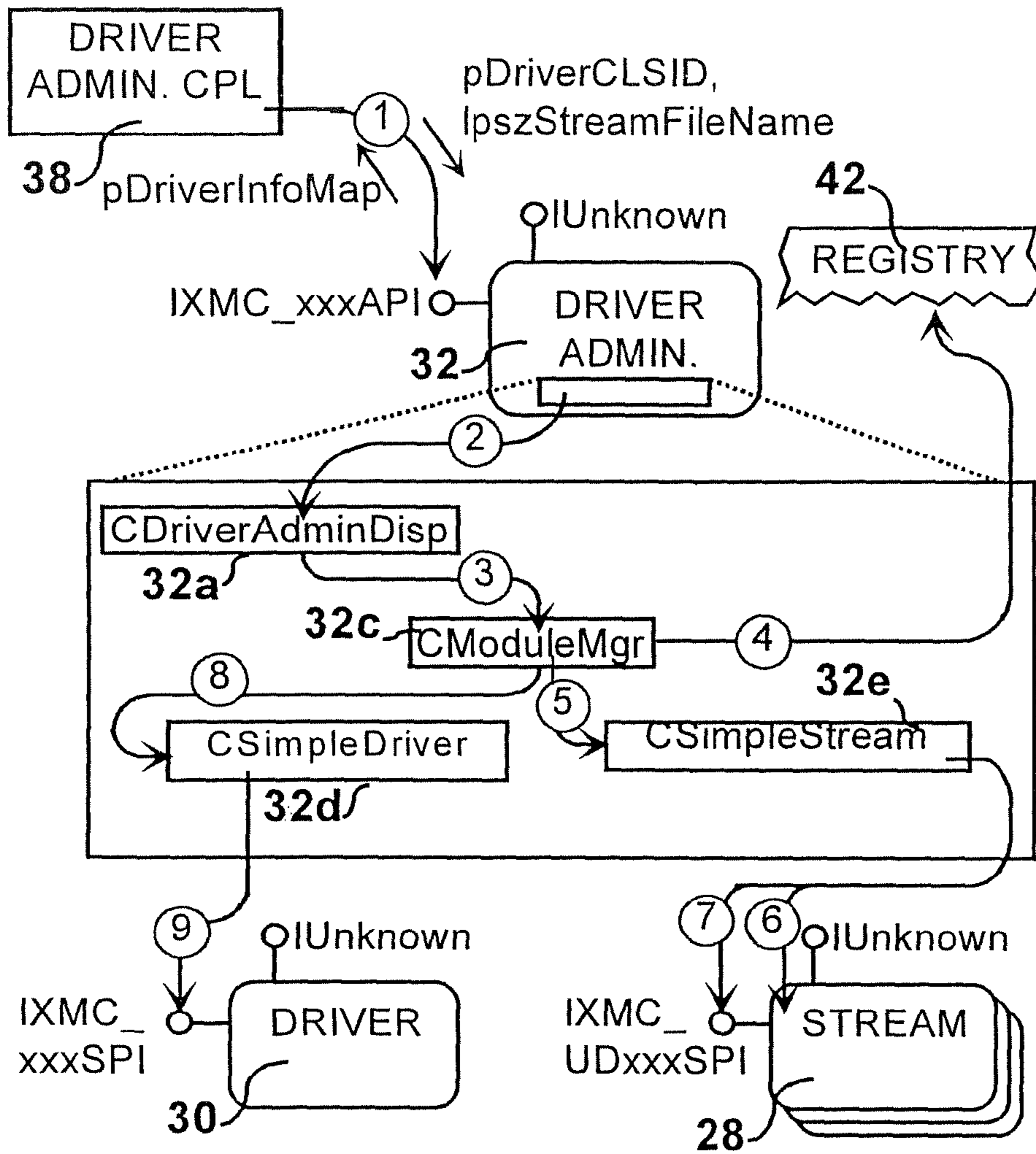
FIG. 44 Scenario-Map - Registering a Stream
