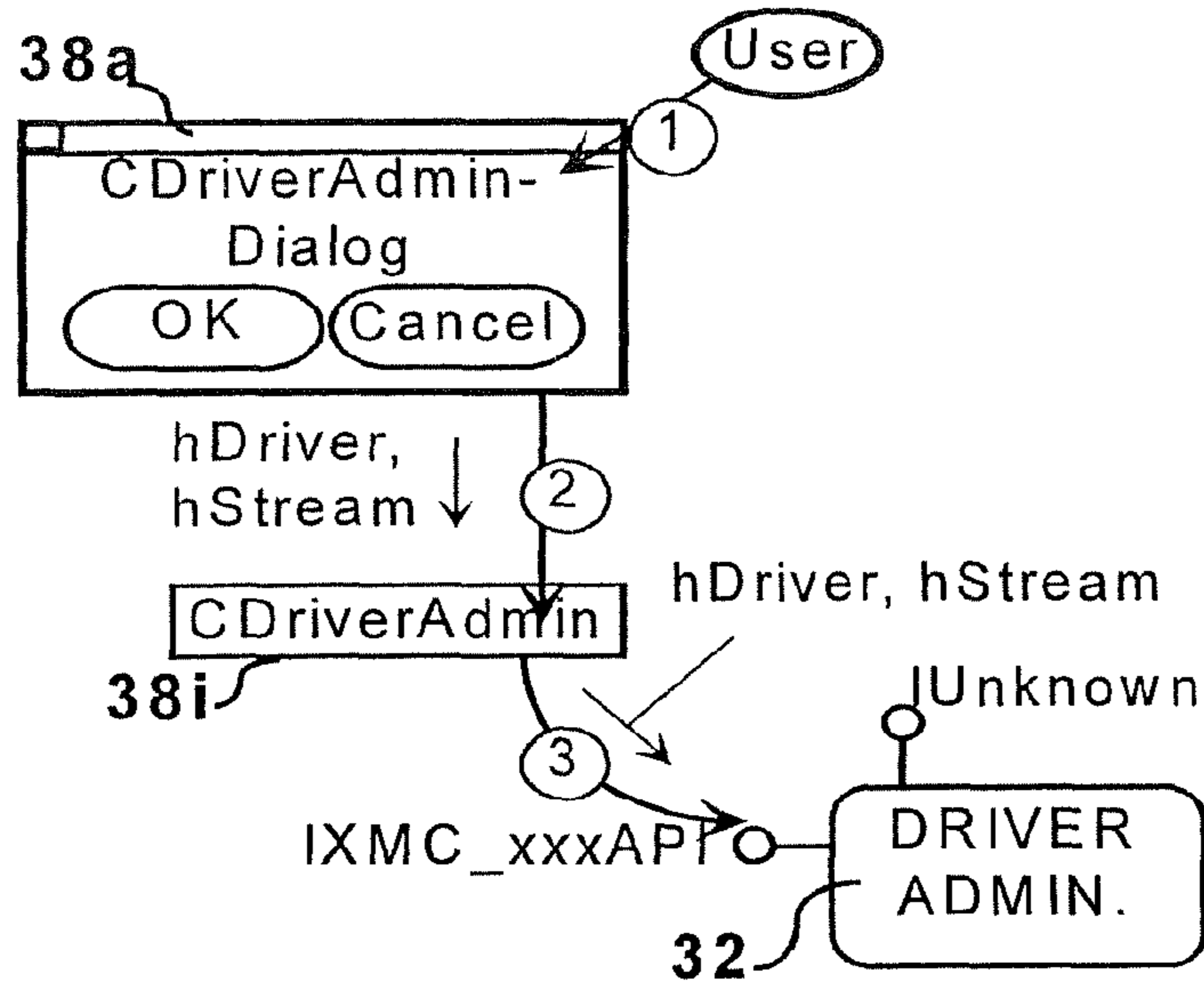
FIG. 56 Scenario-Map - Removing a Driver
