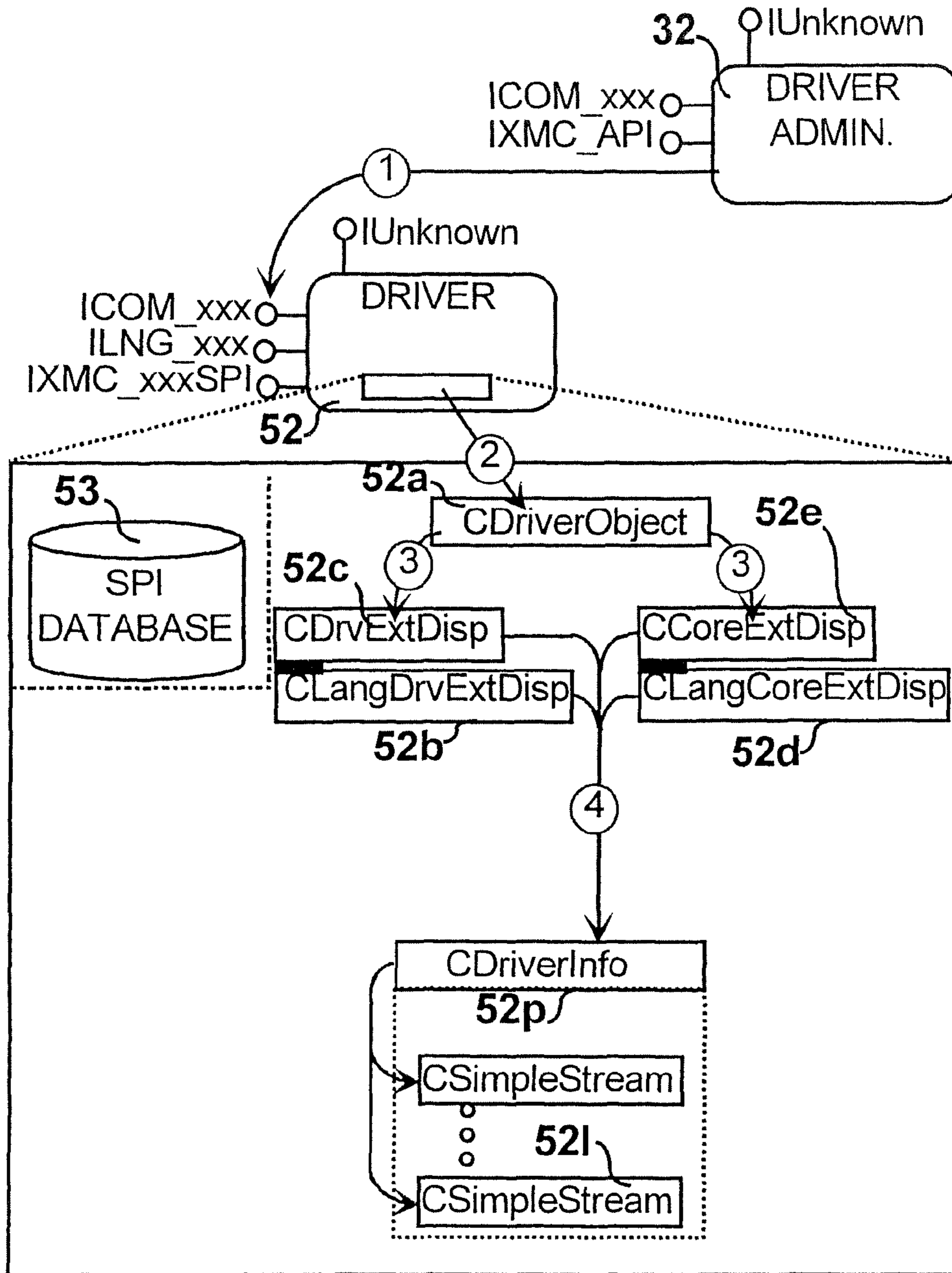
FIG. 62 Scenario-Map - Query Operation
