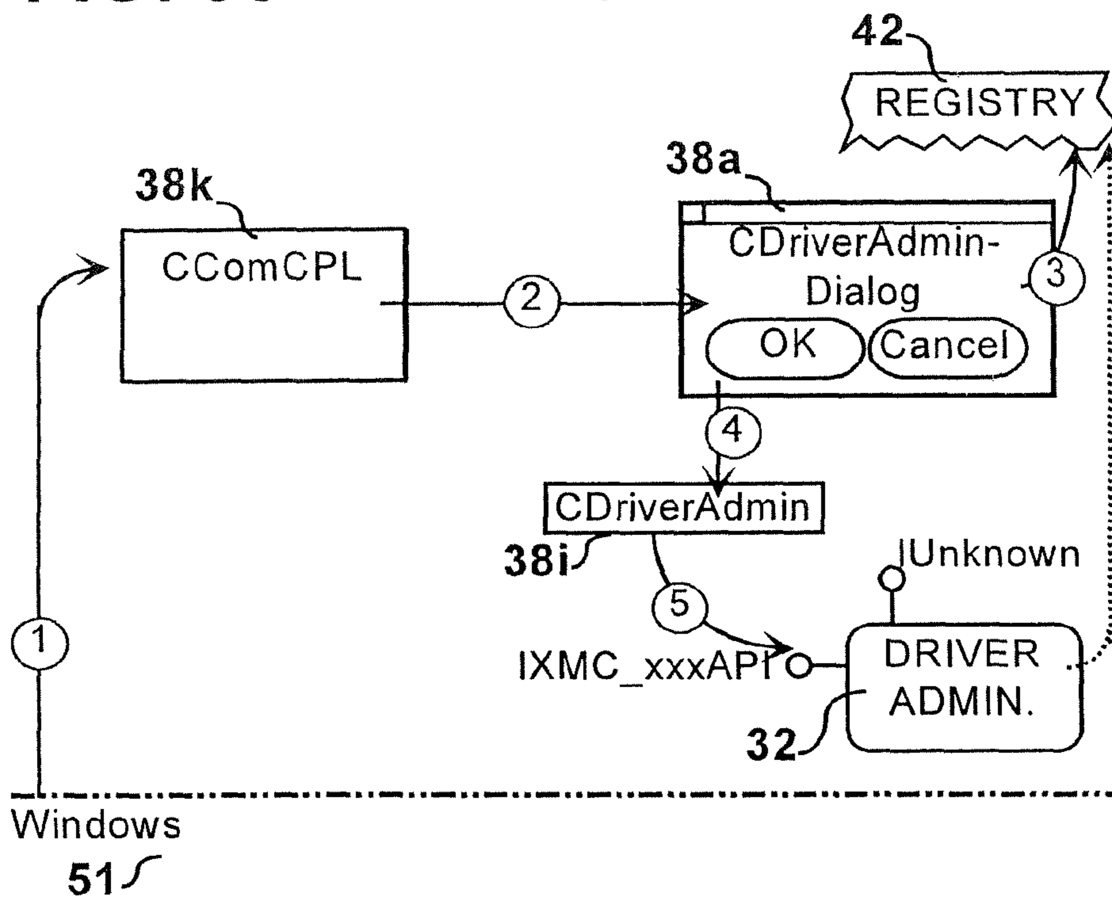
FIG. 53 Scenario-Map - Initializing the App.
