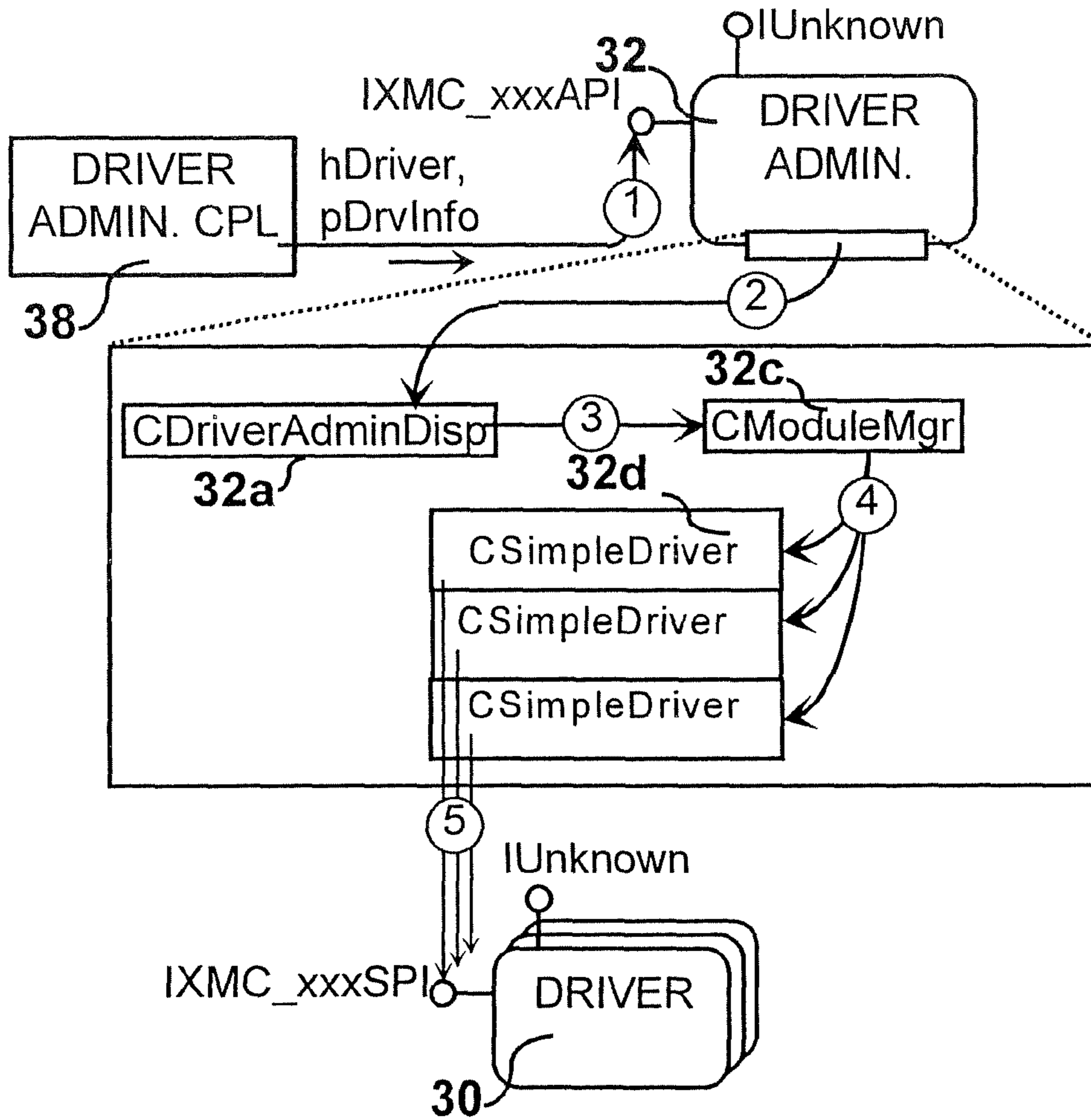
FIG. 45 Scenario-Map - Setting Driver Info.
