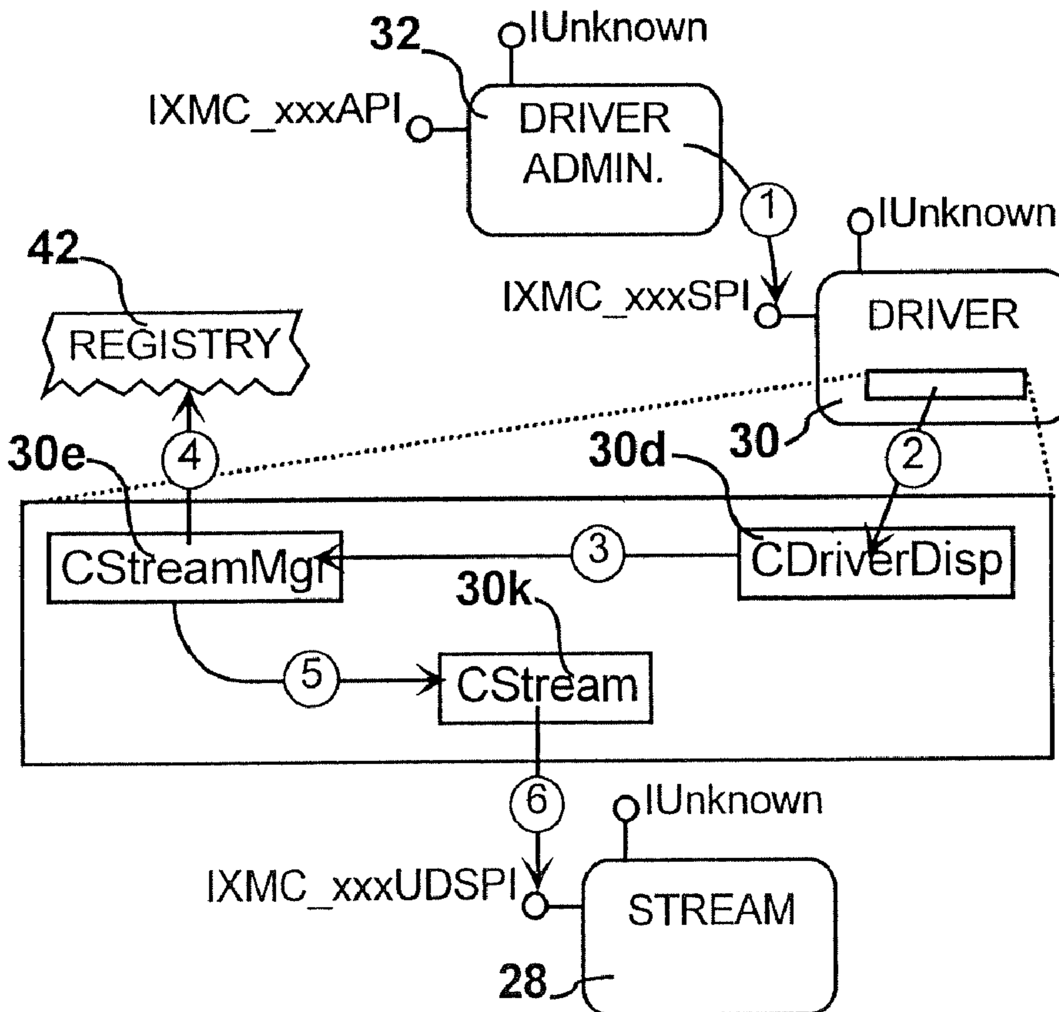
FIG. 16 Scenario-Map - Query Operation
