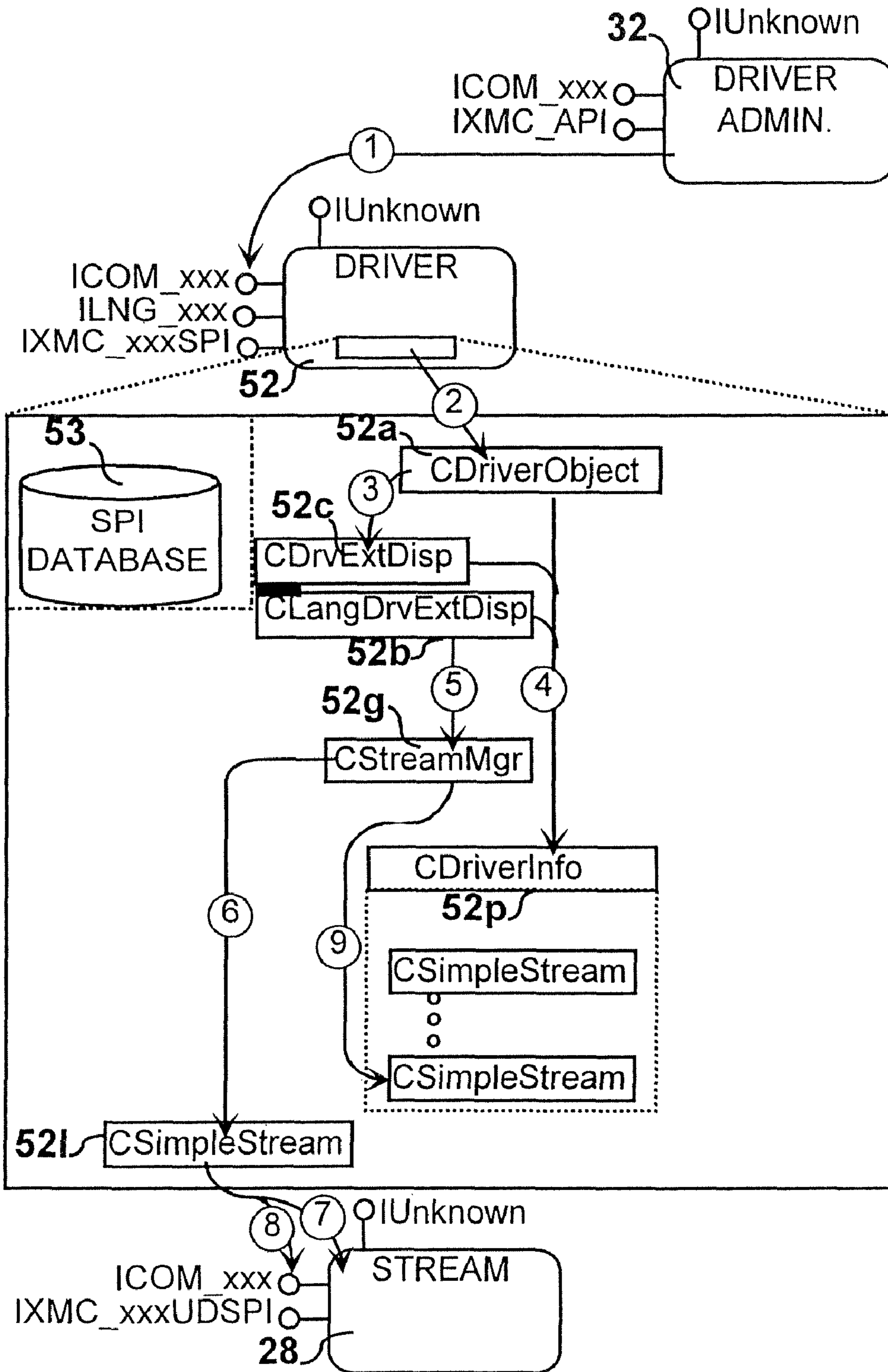
FIG. 61 Scenario-Map - Adding a Stream
