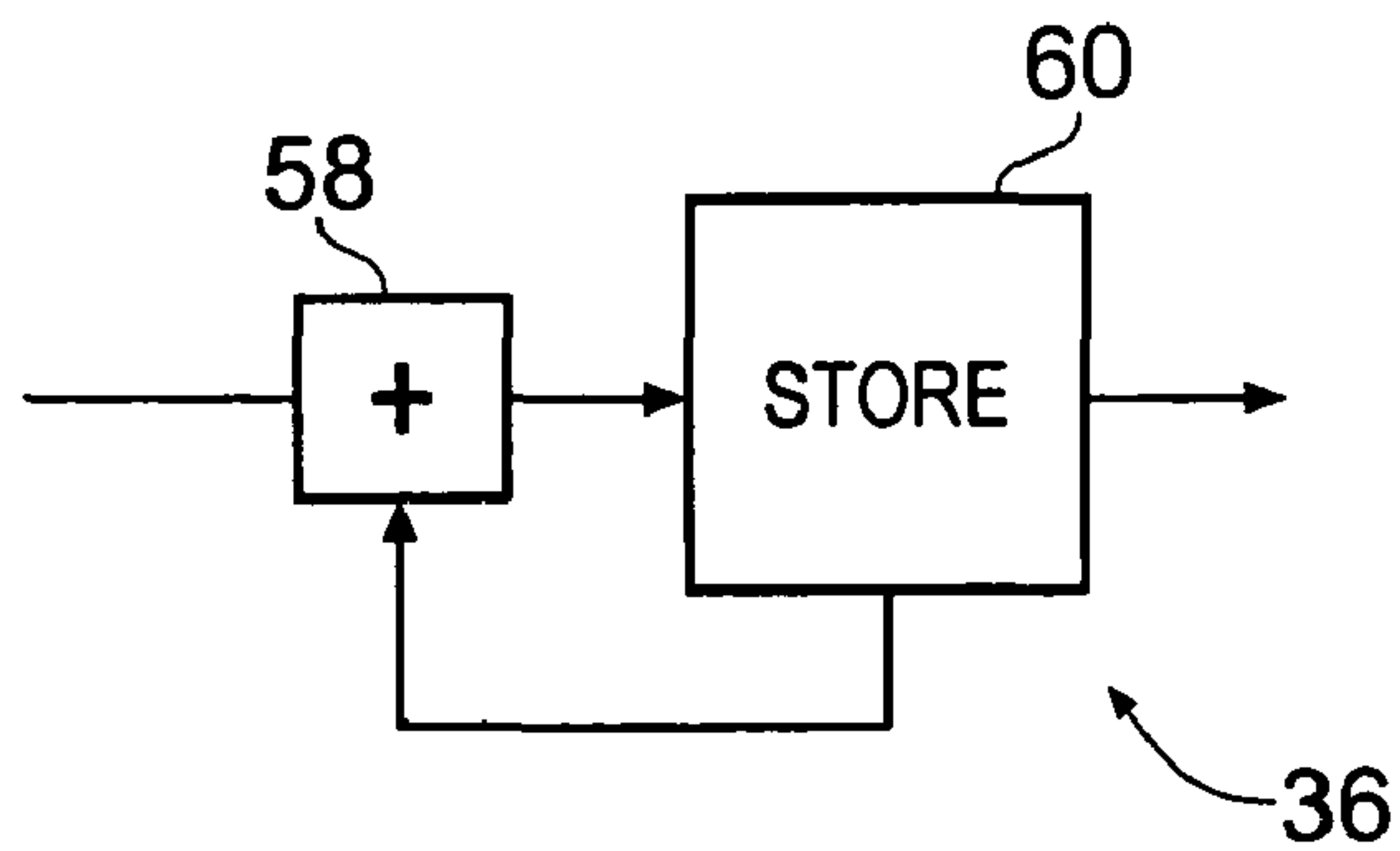
Fig. 6: Accumulator
