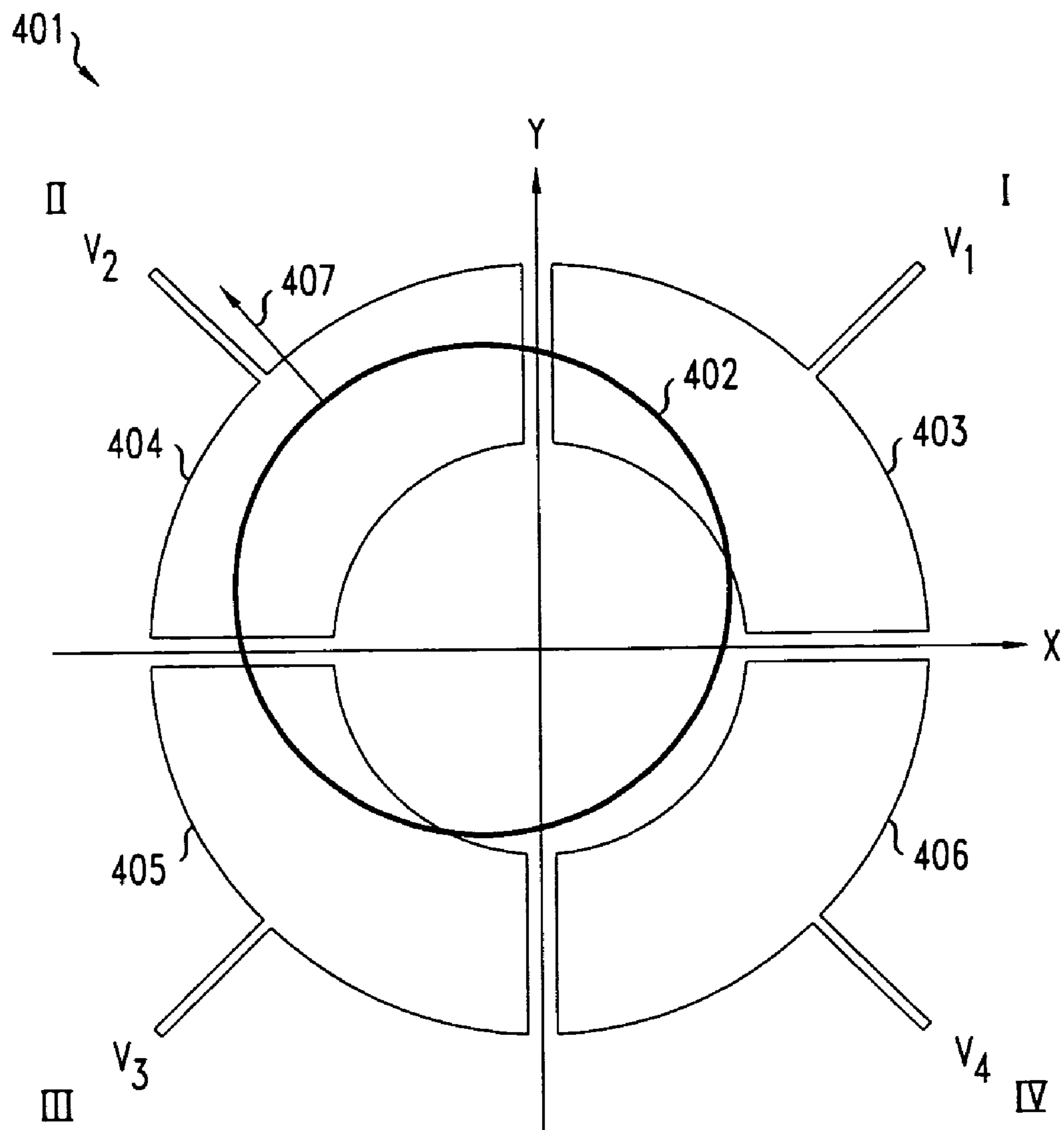
FIG. 4 (PRIOR ART)
