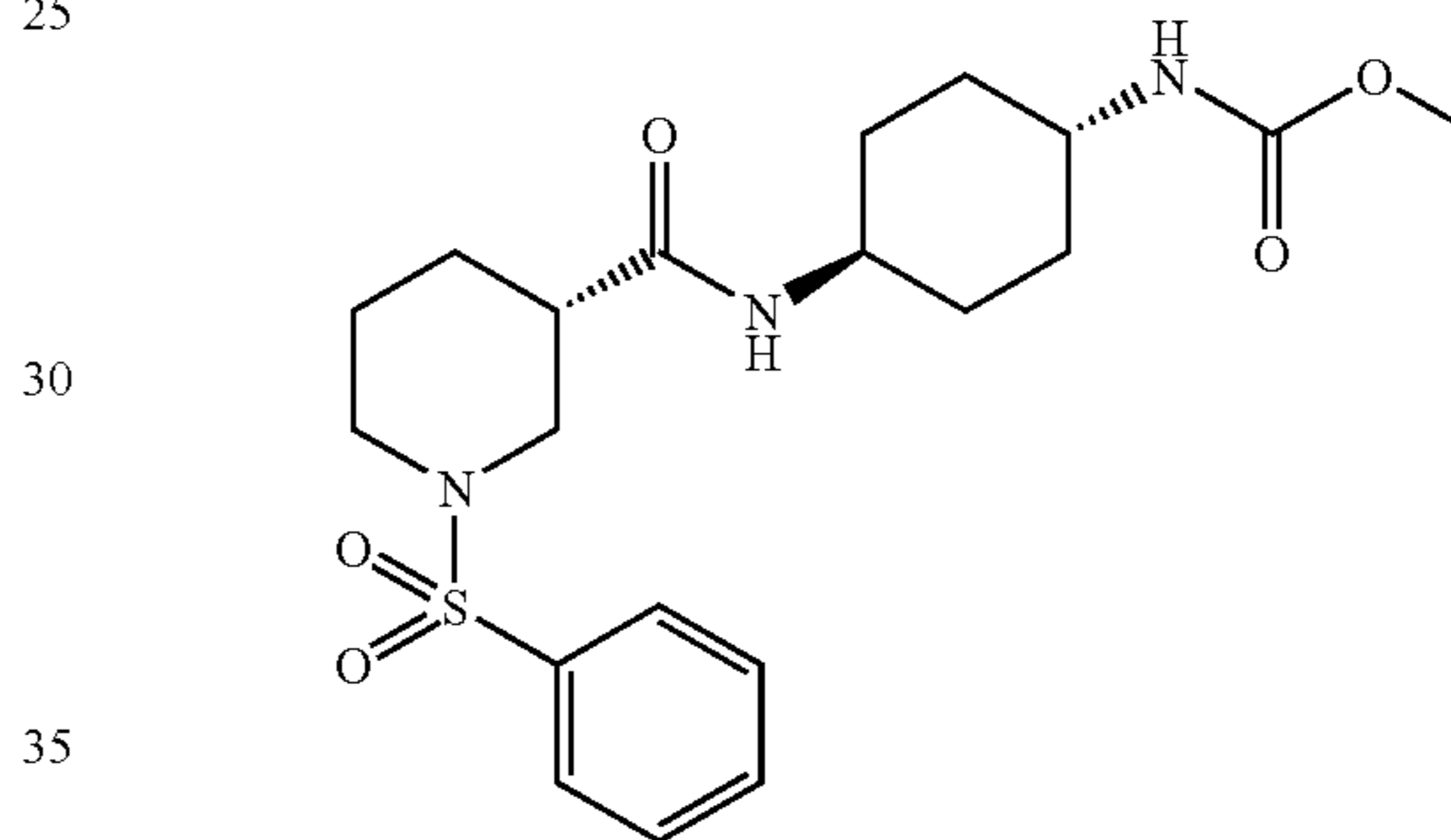
Methyl [trans-4-({[(3S)-1-(phenylsulfonyl)piperidin-3-yl]carbonyl}amino)cyclohexyl]carbamate
