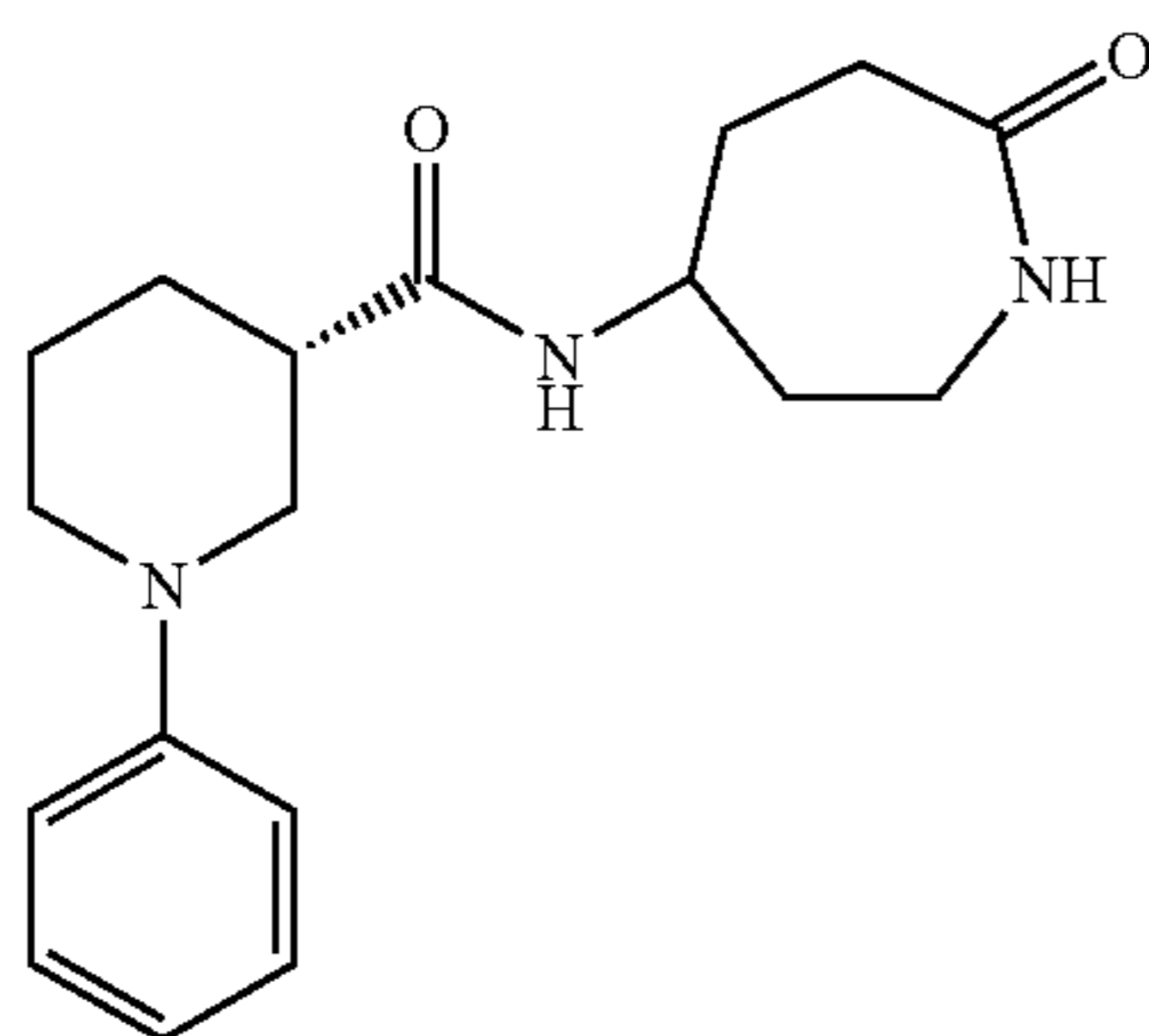
(3S)-N-(7-oxoazepan-4-yl)-1-phenylpiperidine-3-carboxamide
