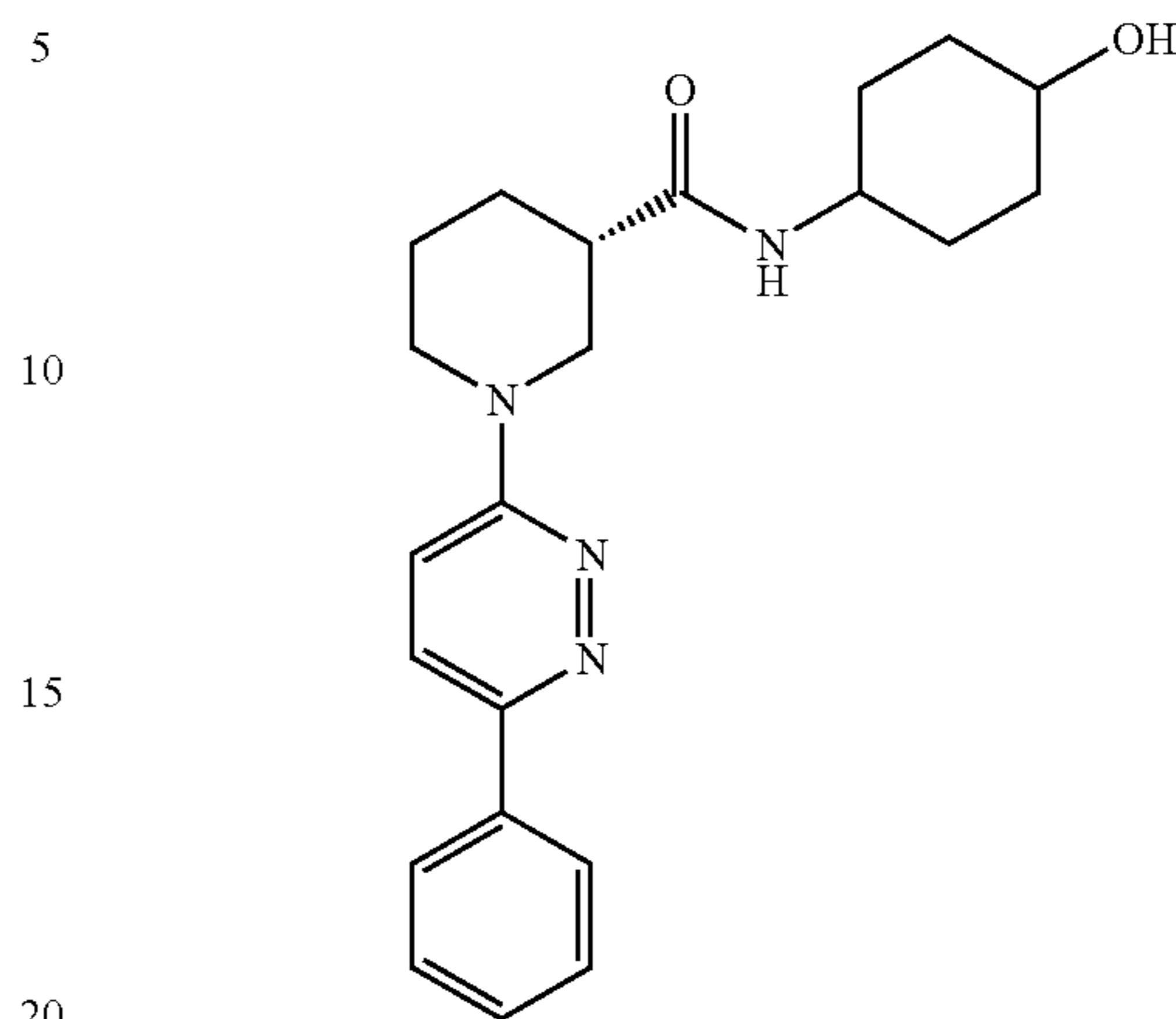
(3S)-N-(4-Hydroxycyclohexyl)-1-(2-methylquinolin-4-yl)piperidine-3-carboxamide
