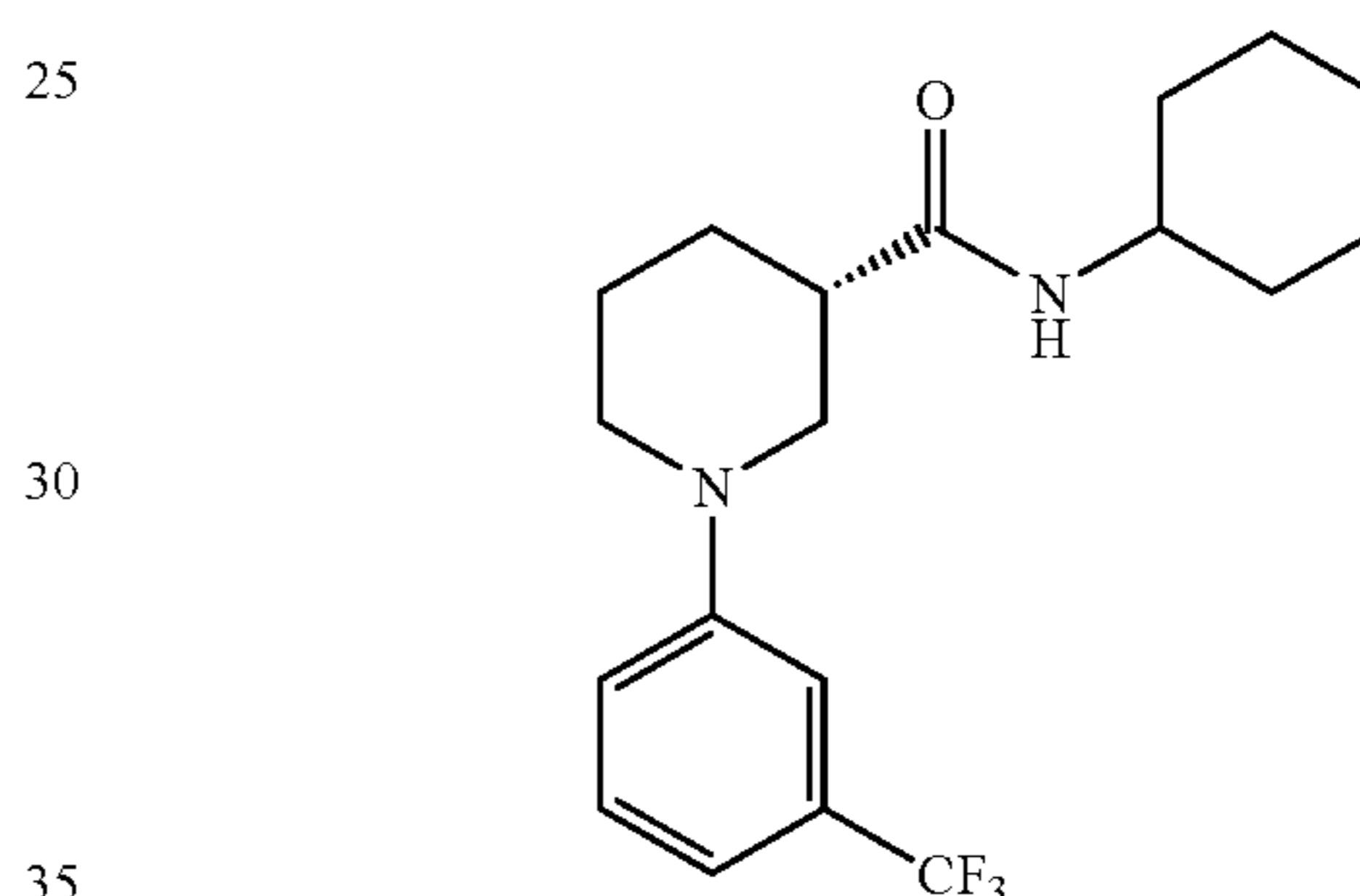
(3S)-N-Cyclohexyl-1-[3-(trifluoromethyl)phenyl]piperidine-3-carboxamide
