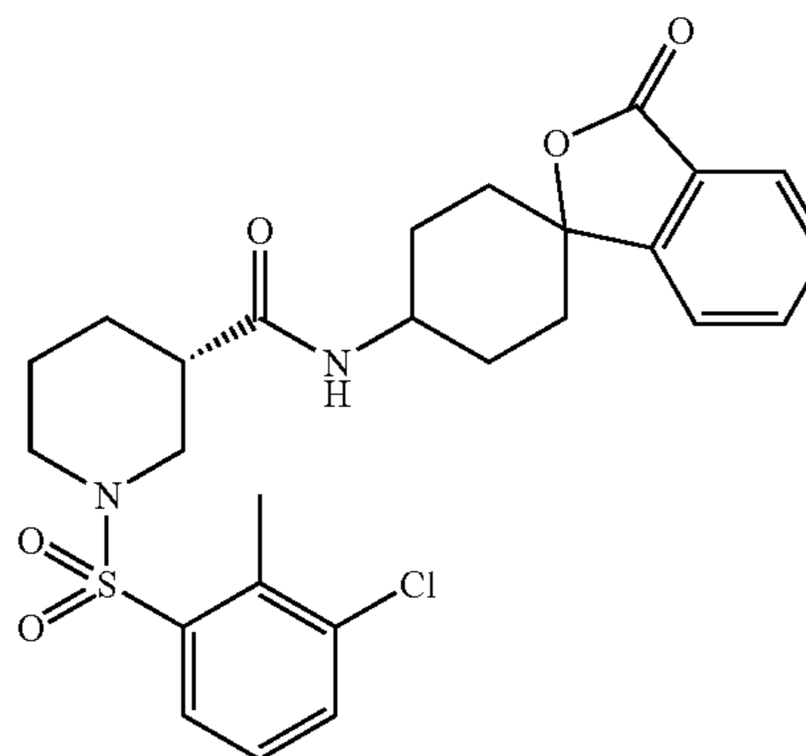
(3S)-1-[(3-Chloro-2-methylphenyl)sulfonyl]-N-(3-oxo-3H-spiro[2-benzofuran-1,1'-cyclohexan]-4'-yl)piperidine-3-carboxamide
