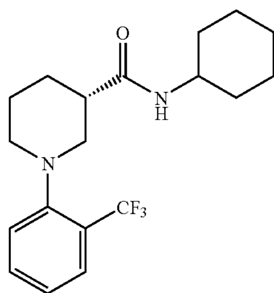
(3S)-N-Cyclohexyl-1-[2-(trifluoromethyl)phenyl]piperidine-3-carboxamide
