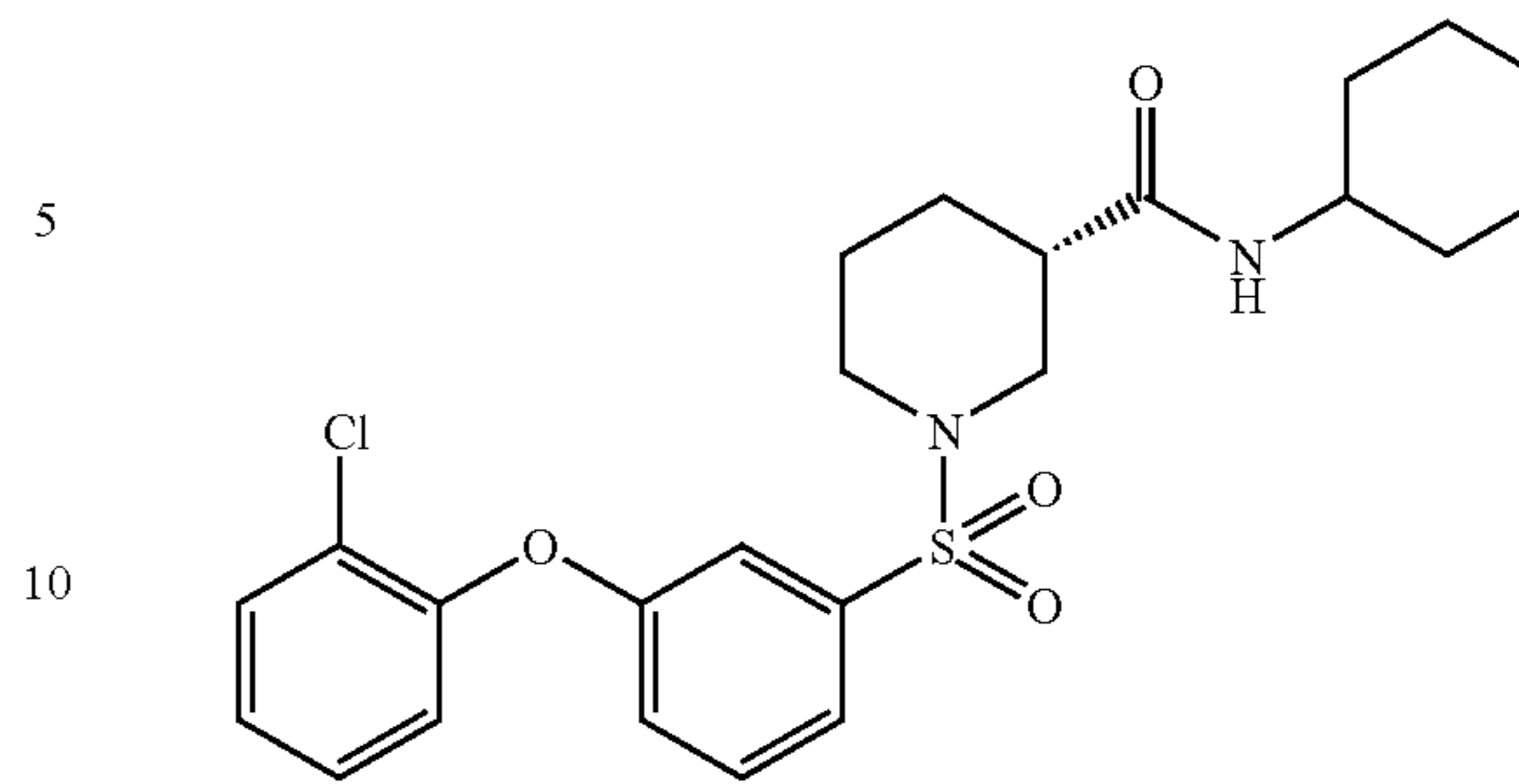
(3S)-1-([3-(2-chlorophenoxy)phenyl]sulfonyl)-N-cyclohexylpiperidine-3-carboxamide
