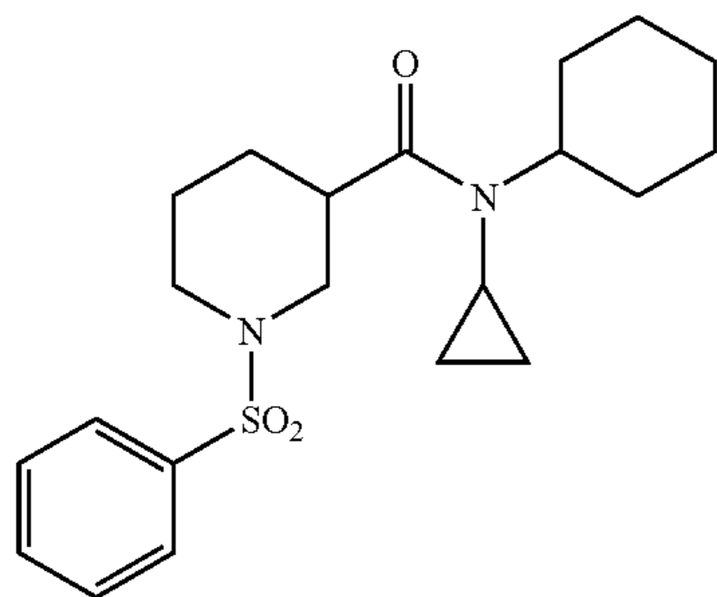
Example 3
