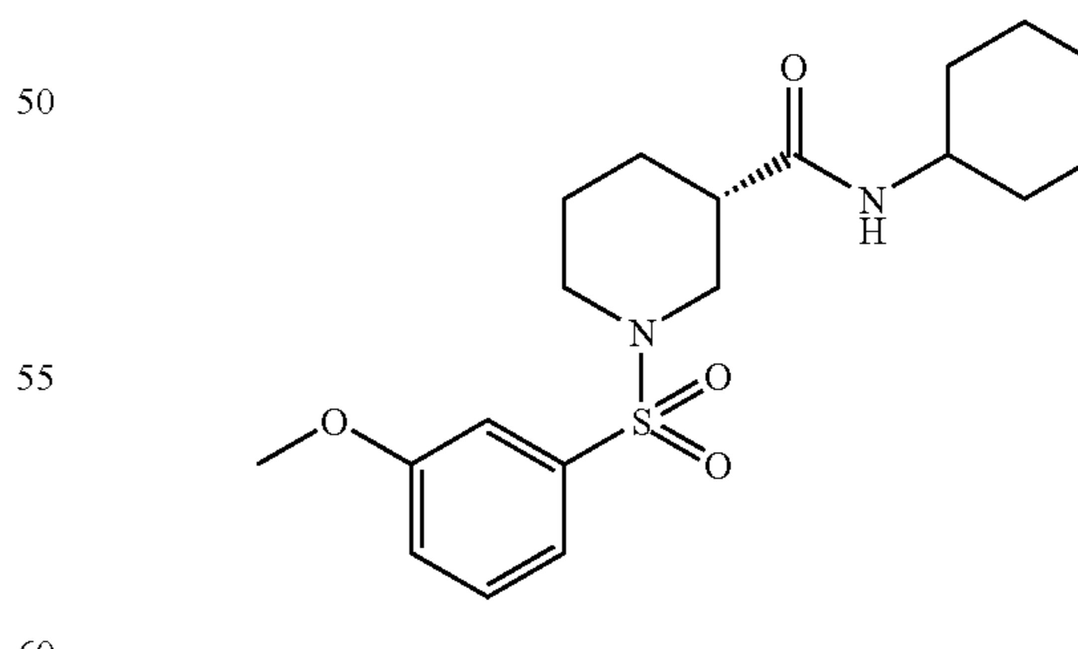
(3S)-N-Cyclohexyl-1-([3-methoxyphenyl]sulfonyl)piperidine-3-carboxamide
