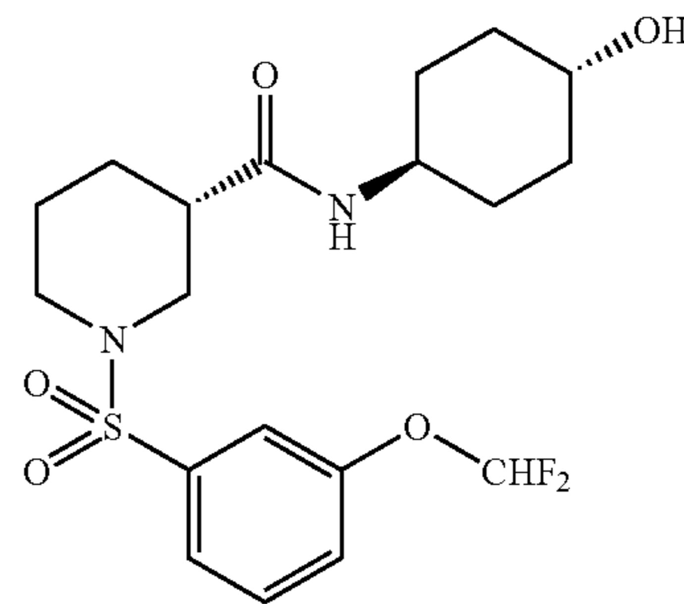
(3S)-1-[[3-(Difluoromethoxy)phenyl]sulfonyl]-N-(trans-4-hydroxycyclohexyl)piperidine-3-carboxamide
