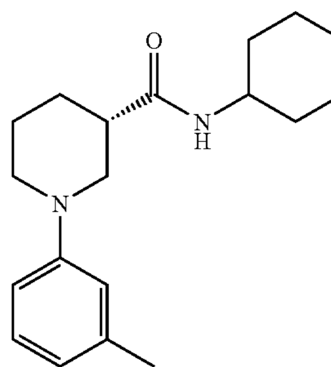
Example 132
