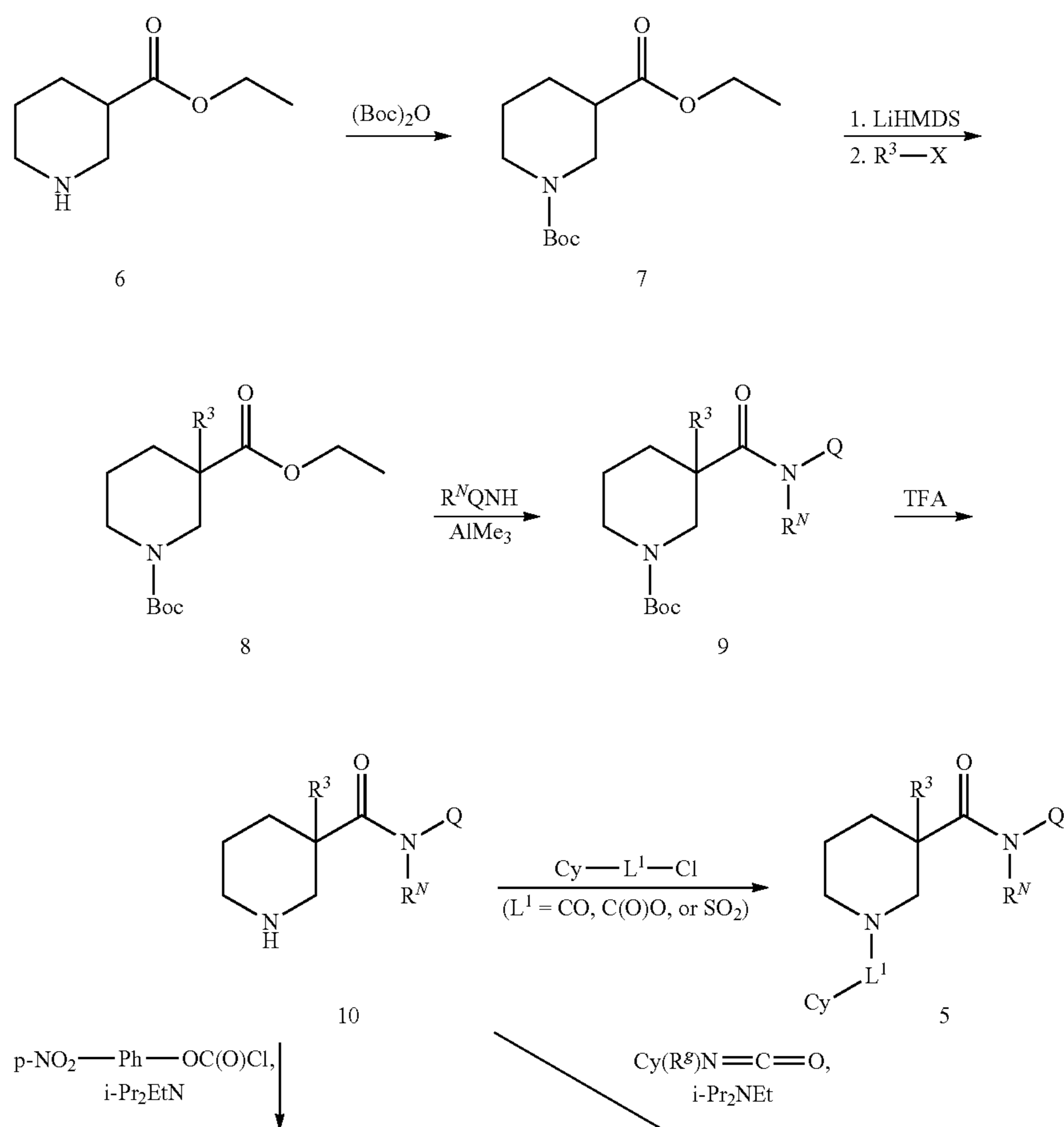
Scheme 2
