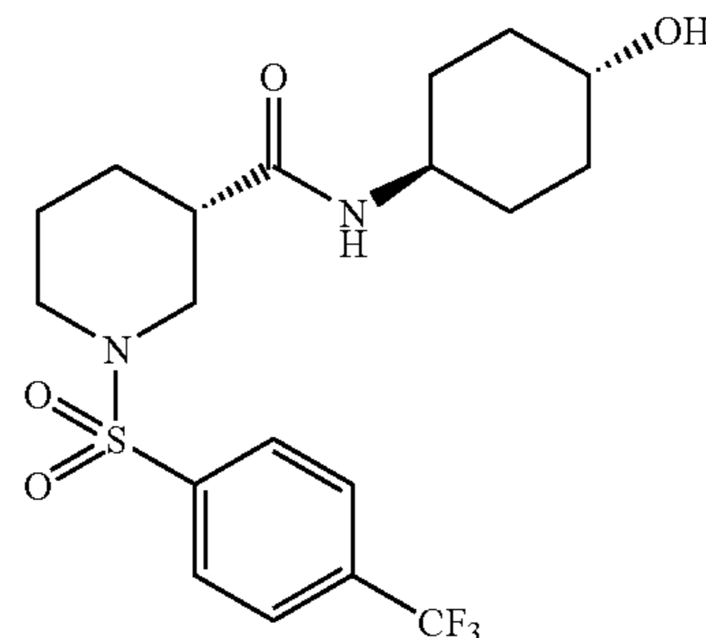
(3S)-N-(trans-4-Hydroxycyclohexyl)-1-[[4-(trifluoromethyl)phenyl]sulfonyl]piperidine-3-carboxamide
