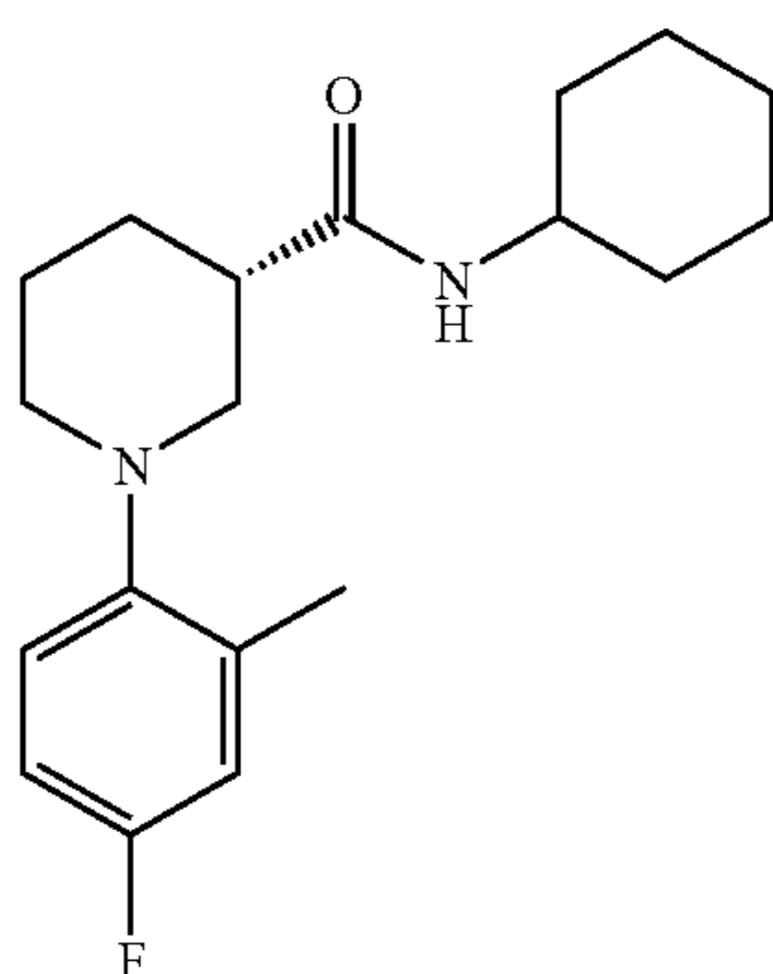
(3S)-N-Cyclohexyl-1-(4-fluoro-2-methylphenyl)piperidine-3-carboxamide
