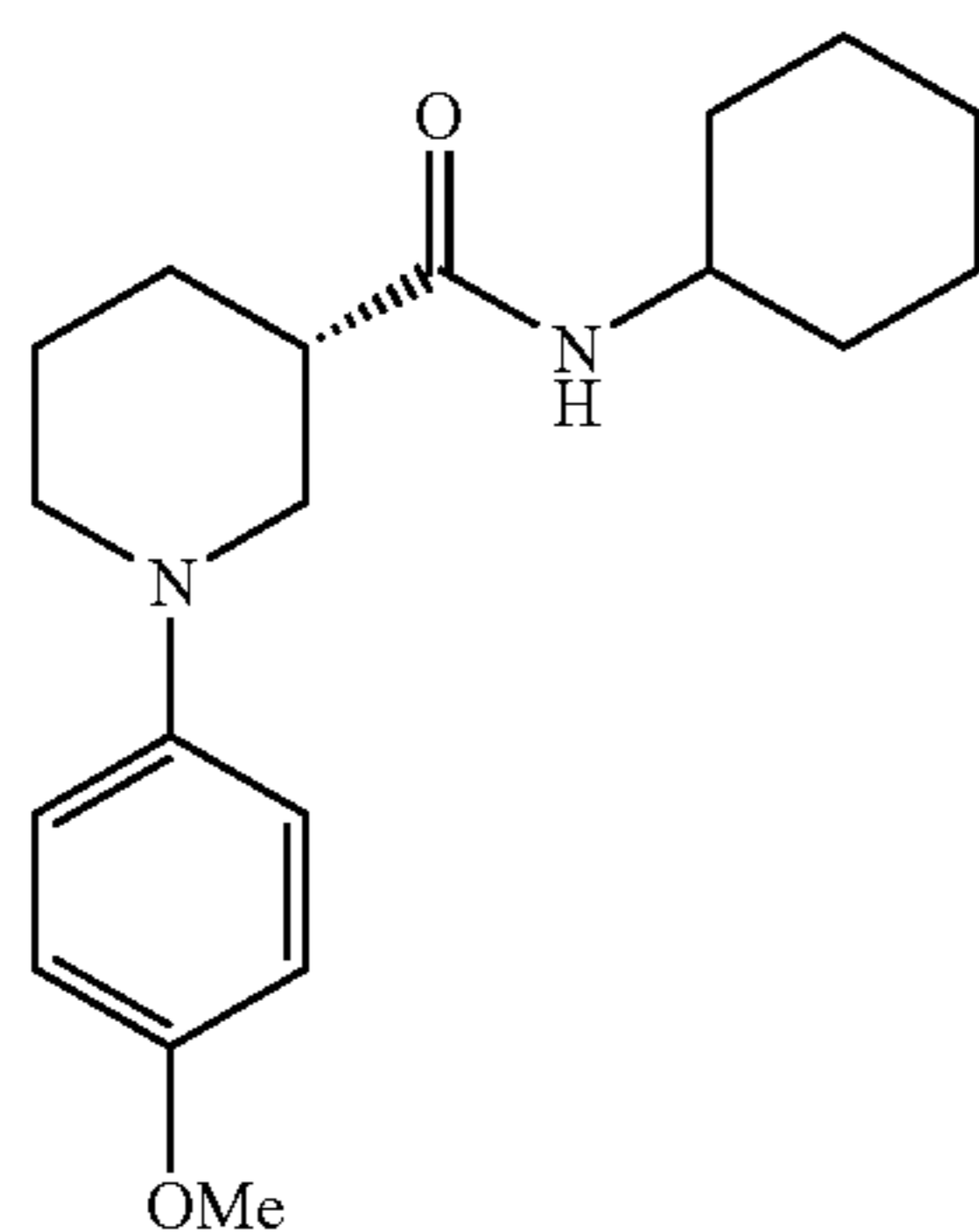
(3S)-N-Cyclohexyl-1-(4-methoxyphenyl)piperidine-3-carboxamide
