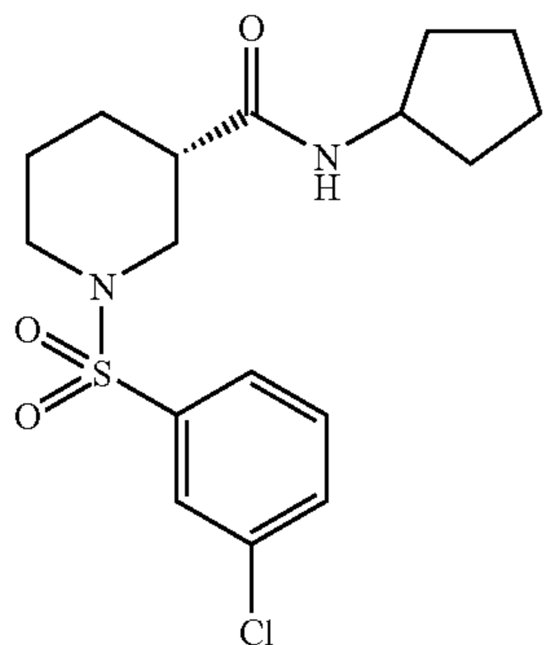
(3S)-1-[(3-Chlorophenyl)sulfonyl]-N-cyclopentylpiperidine-3-carboxamide
