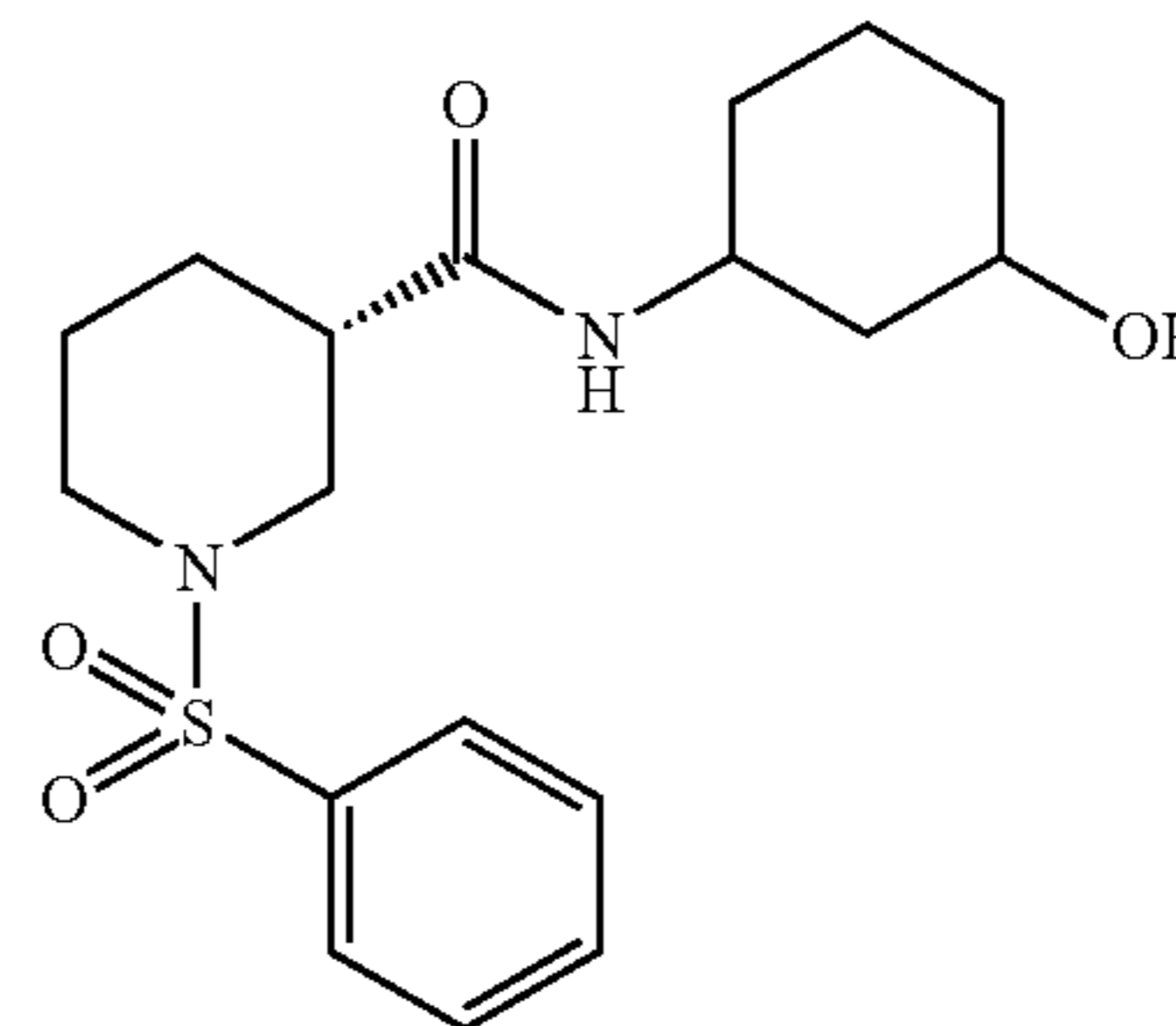
(3S)-N-(3-Hydroxycyclohexyl)-1-(phenylsulfonyl)piperidine-3-carboxamide
