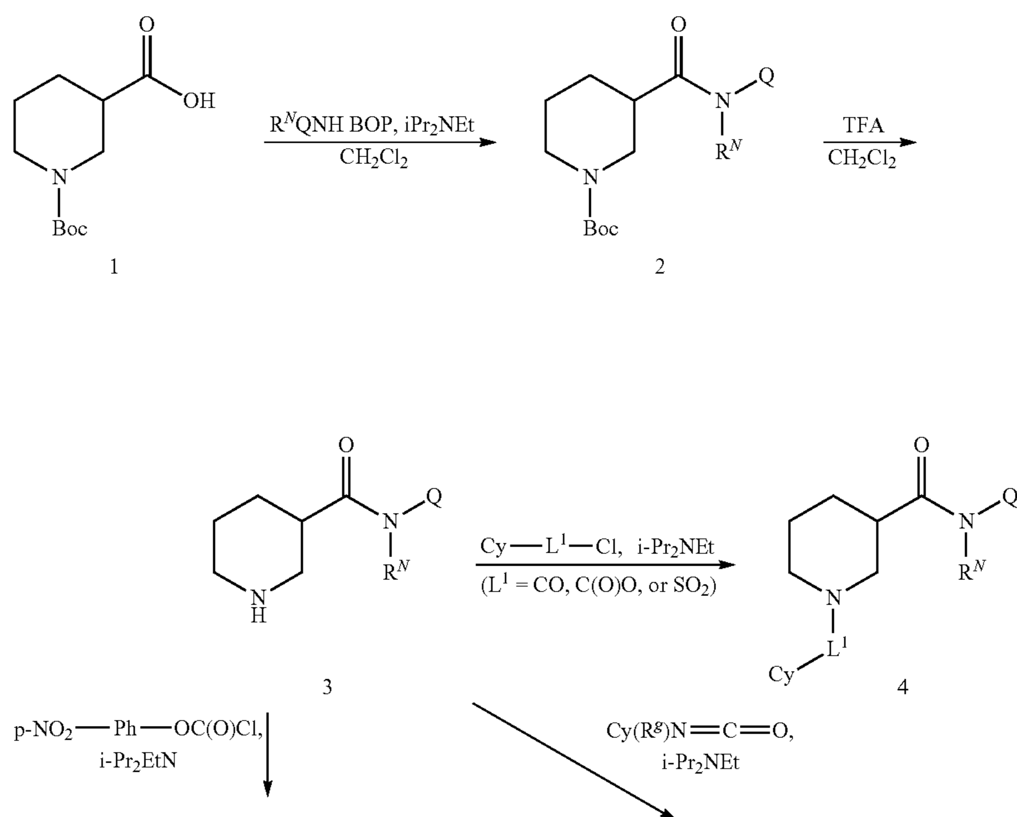
Scheme 1
