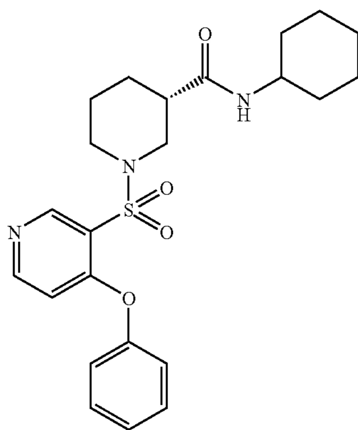
(3S)-N-Cyclohexyl-1-([4-phenoxy-pyridin-3-yl]sulfonyl)piperidine-3-carboxamide trifluoroacetate
