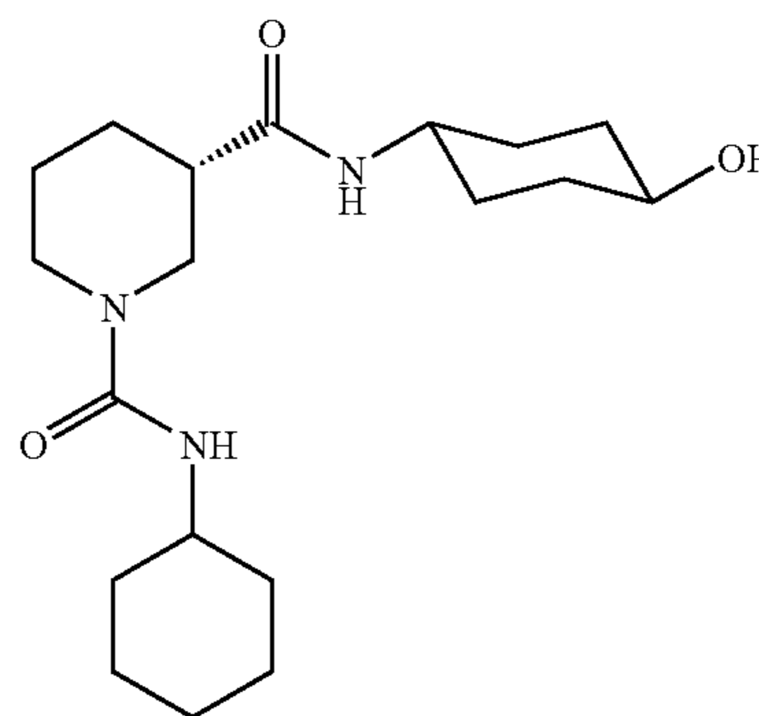
Example 177
