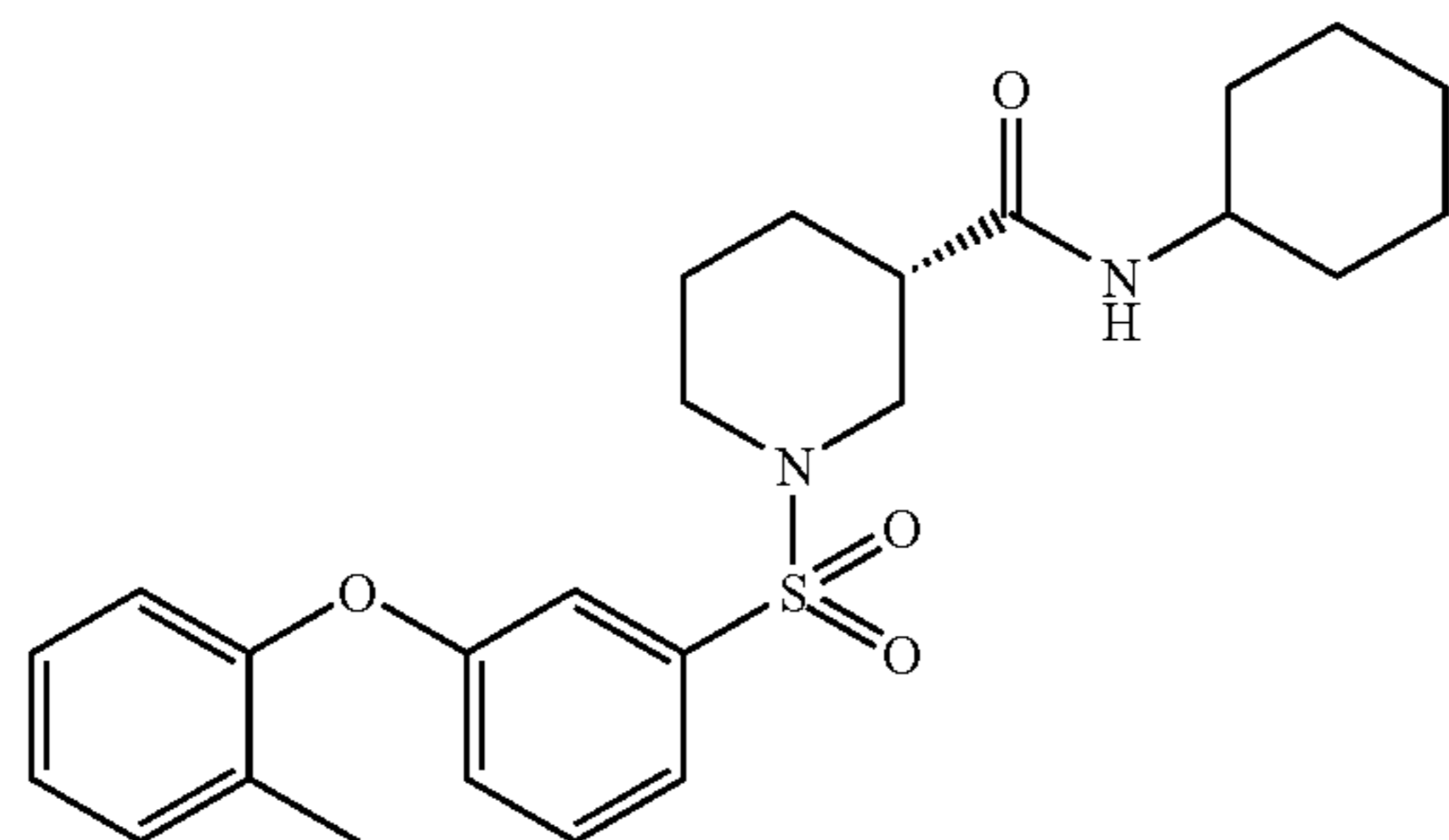
(3S)-N-Cyclohexyl-1-([3-(2-methylphenoxy)phenyl]sulfonyl)piperidine-3-carboxamide
