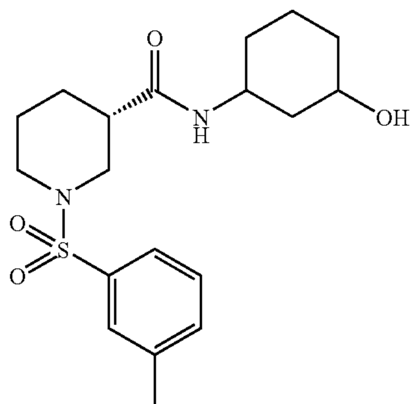
(3S)-N-(3-Hydroxycyclohexyl)-1-[(3-methylphenyl)sulfonyl]piperidine-3-carboxamide
