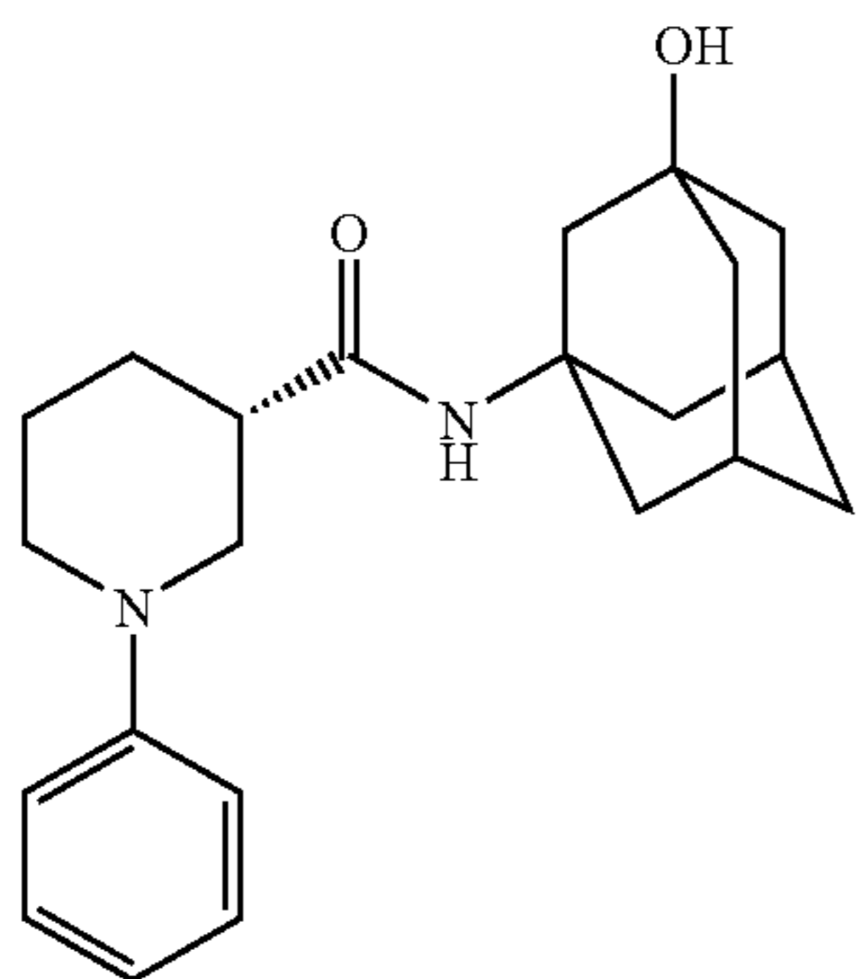
Example 130
