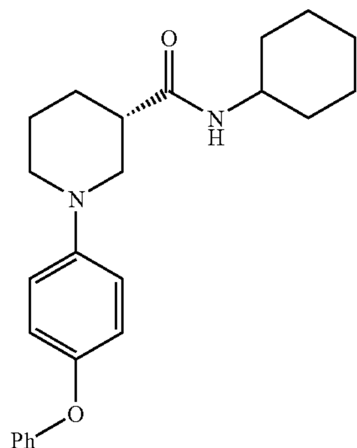
(3S)-N-Cyclohexyl-1-(4-phenoxyphenyl)piperidine-3-carboxamide
