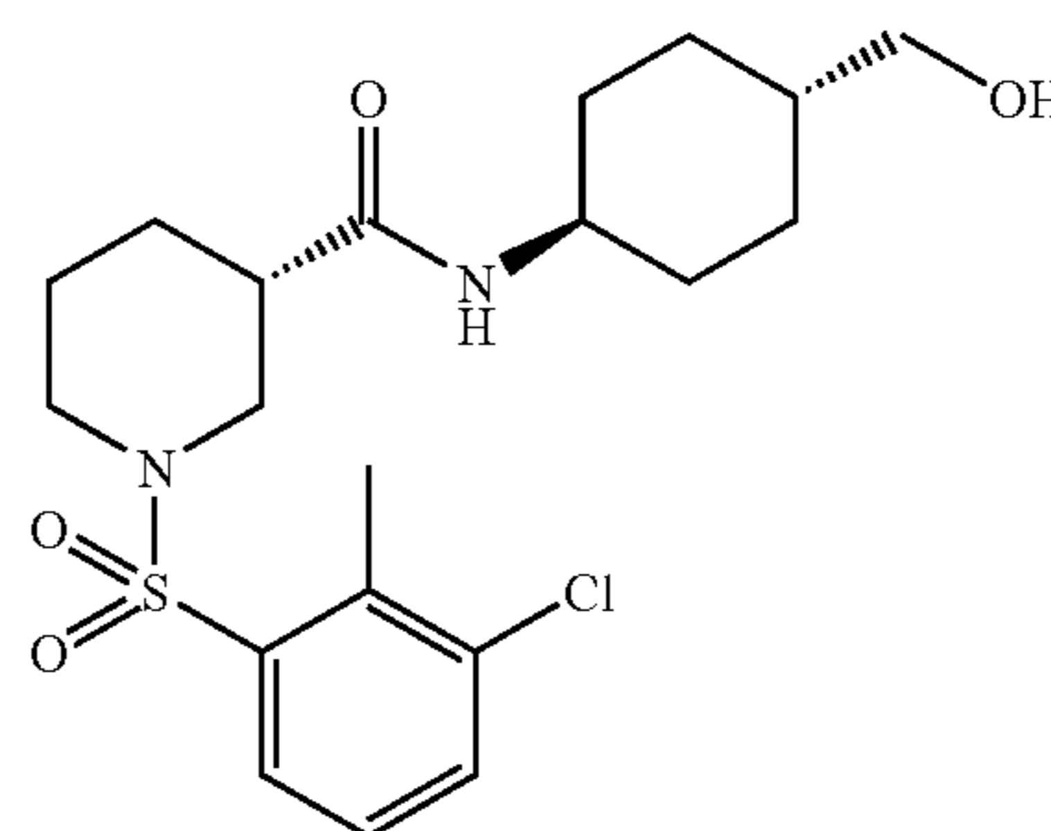
Example 109
