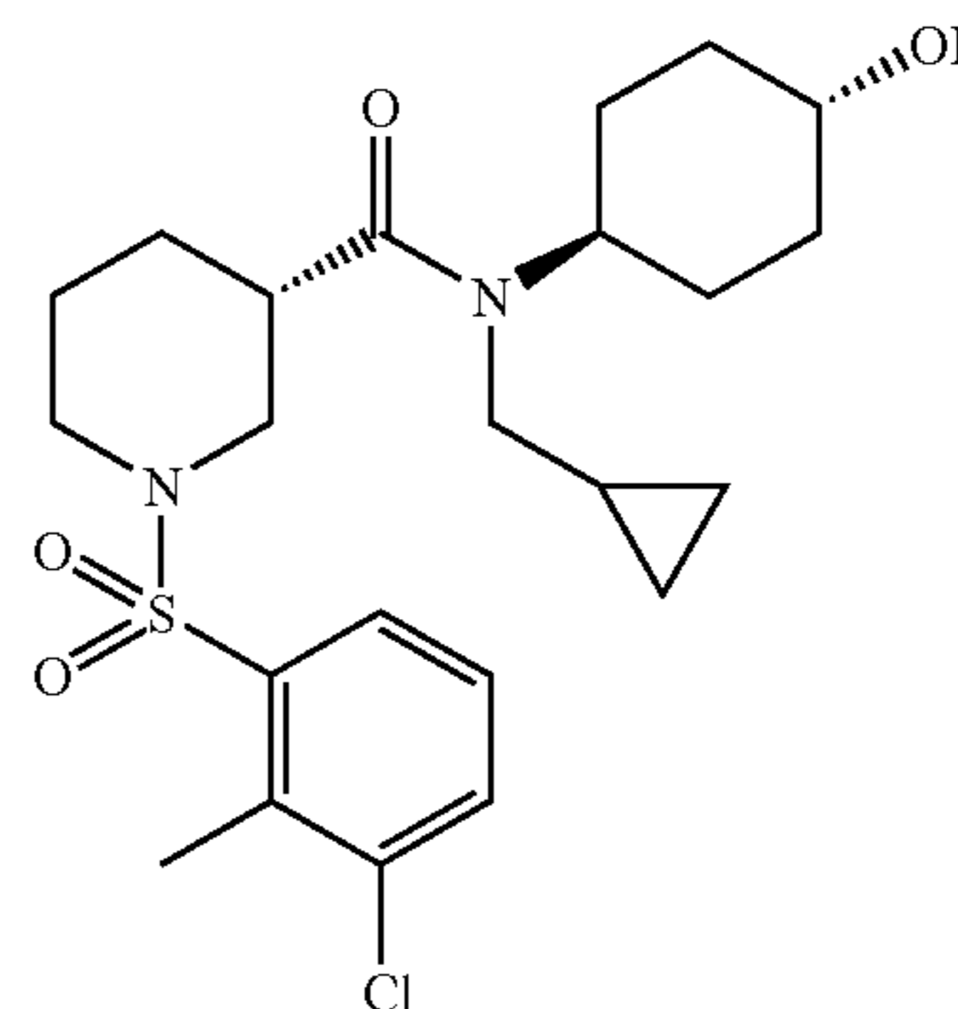
(3S)-1-[(3-Chloro-2-methylphenyl)sulfonyl]-N-(cyclopropylmethyl)-N-(trans-4-hydroxycyclohexyl)piperidine-3-carboxamide
