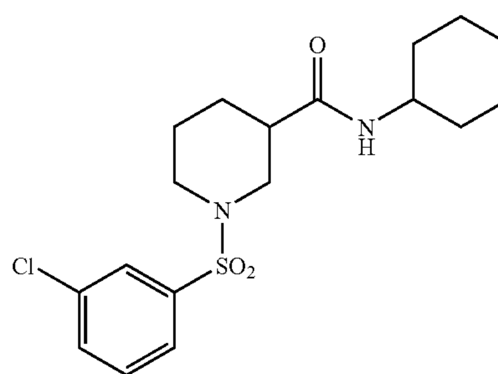
1-[(3-Chlorophenyl)sulfonyl]-N-cyclohexylpiperi- dine-3-carboxamide
