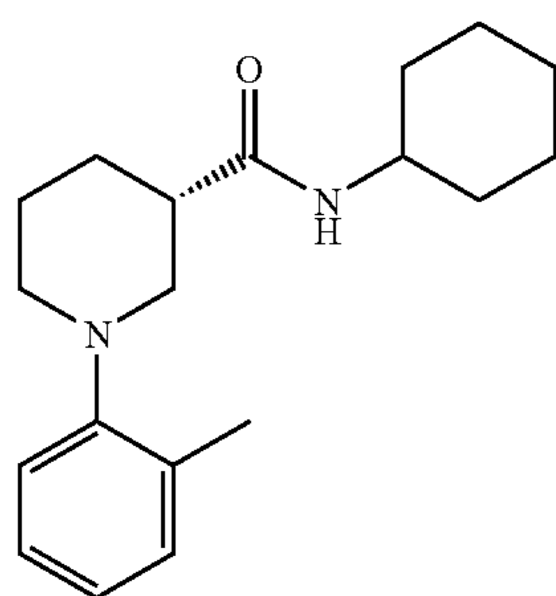
(3S)-N-Cyclohexyl-1-(2-methylphenyl)piperidine-3-carboxamide
