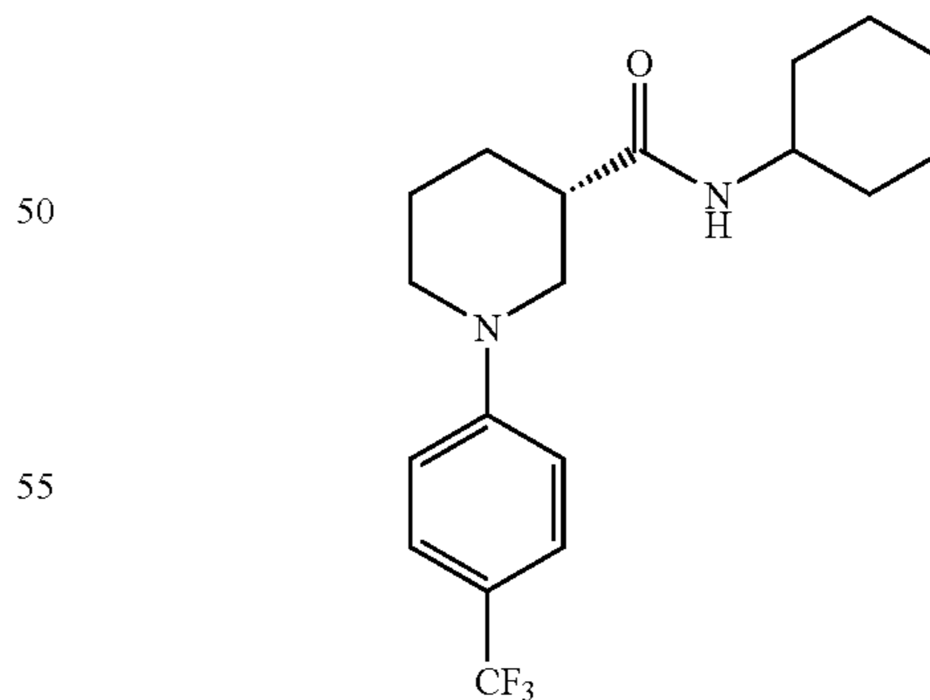
(3S)-N-Cyclohexyl-1-[4-(trifluoromethyl)phenyl]piperidine-3-carboxamide
