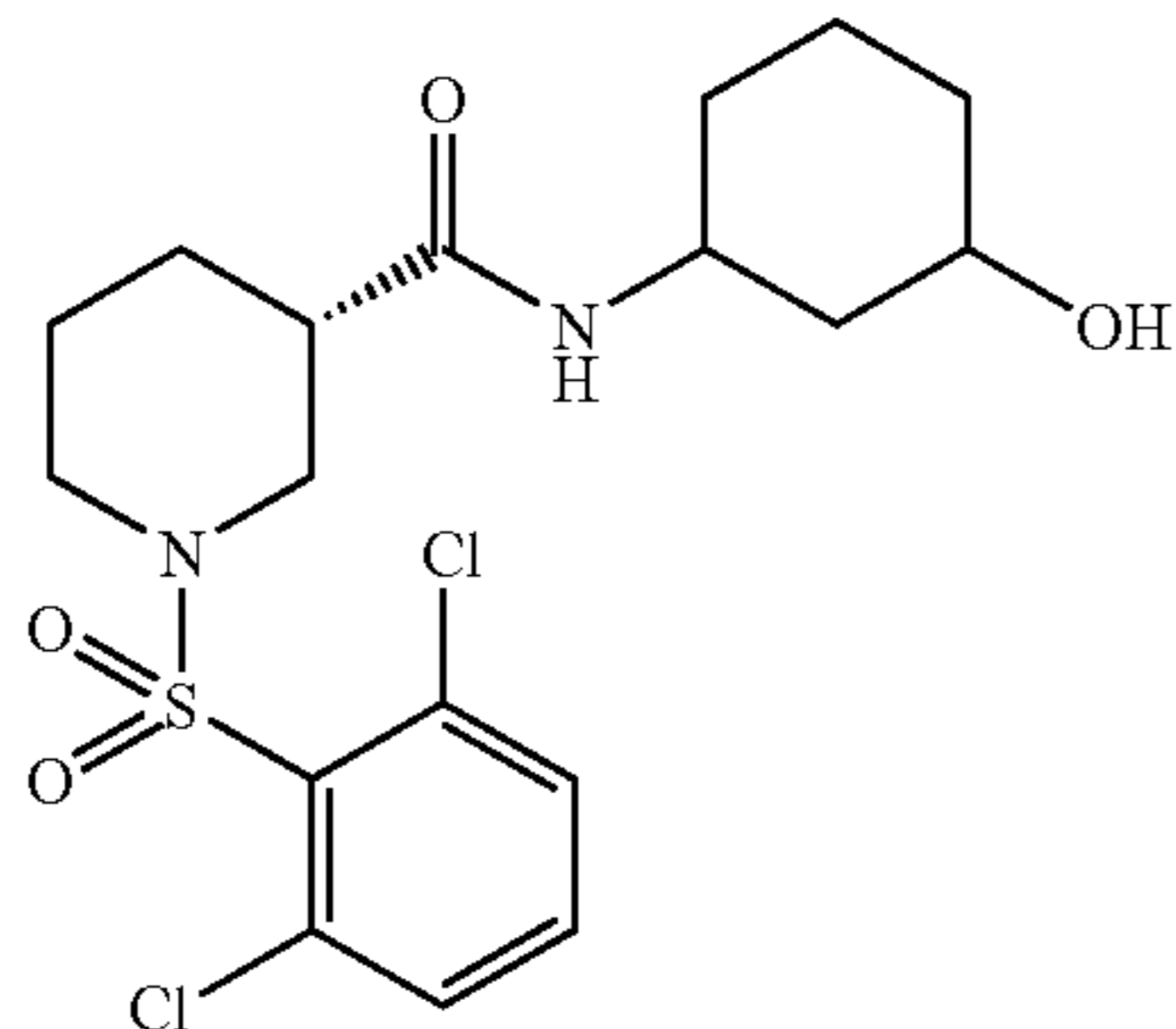
(3S)-1-[(2,6-Dichlorophenyl)sulfonyl]-N-(3-hydroxycyclohexyl)piperidine-3-carboxamide
