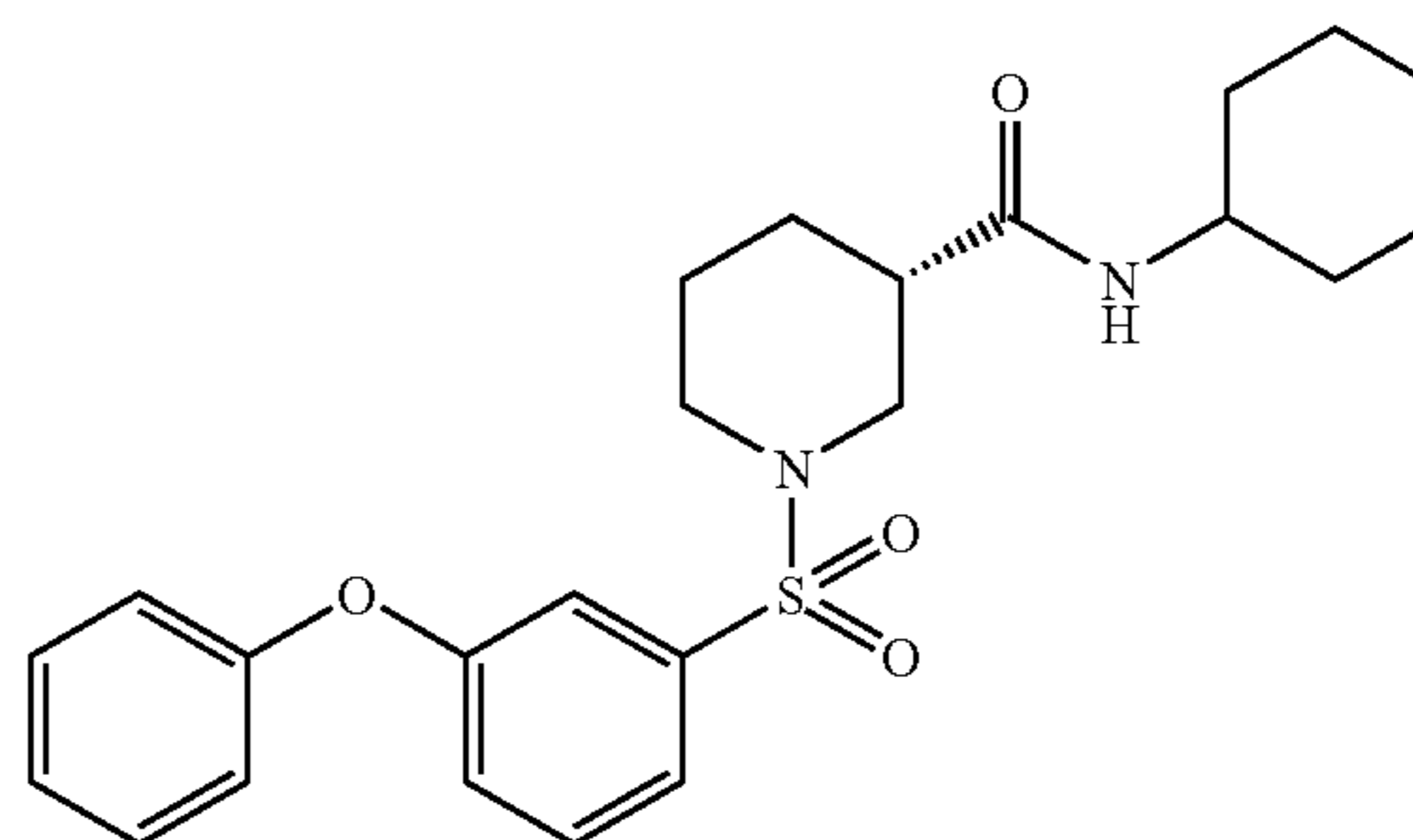
(3S)-N-Cyclohexyl-1-[(3-phenoxyphenyl)sulfonyl]piperidine-3-carboxamide
