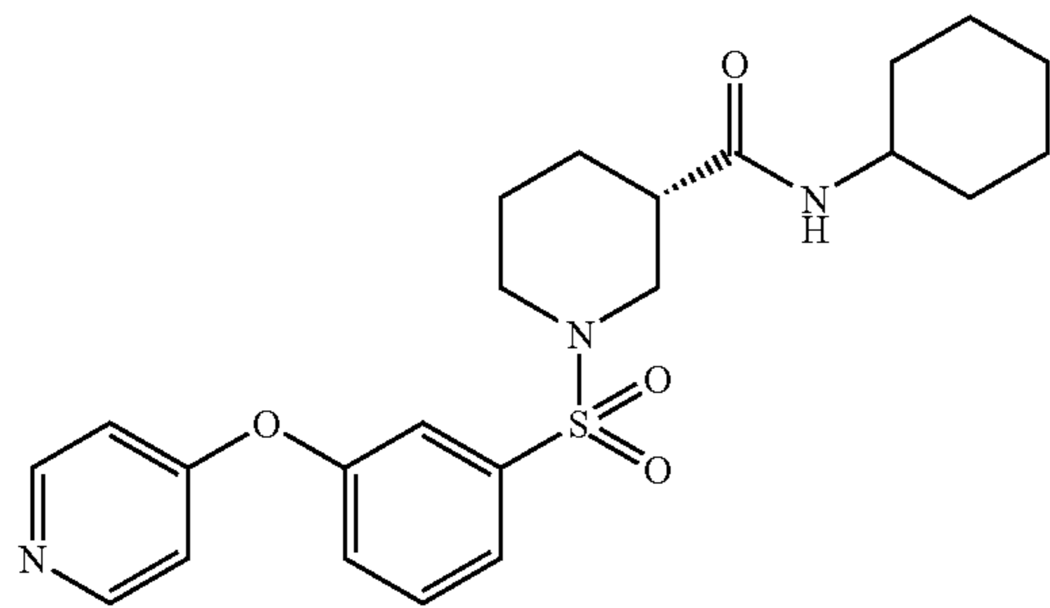
(3S)-N-Cyclohexyl-1-([3-(pyridin-4-yloxy)phenyl]sulfonyl)piperidine-3-carboxamide trifluoroacetate
