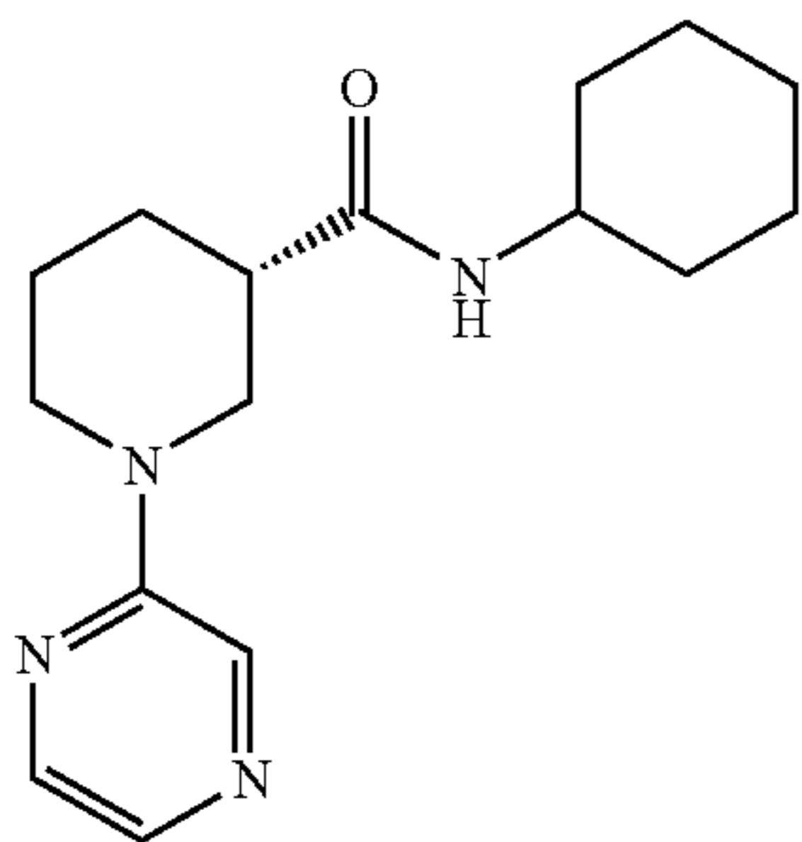
(3S)-N-Cyclohexyl-1-pyrazin-2-ylpiperidine-3-carboxamide
