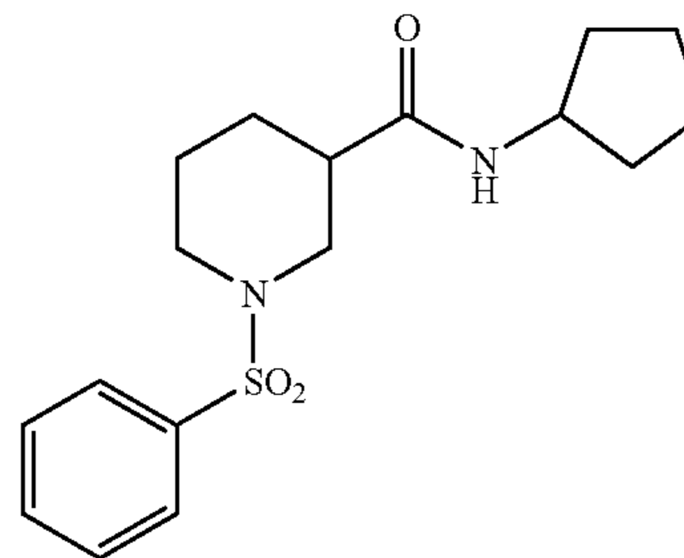
Example 4
