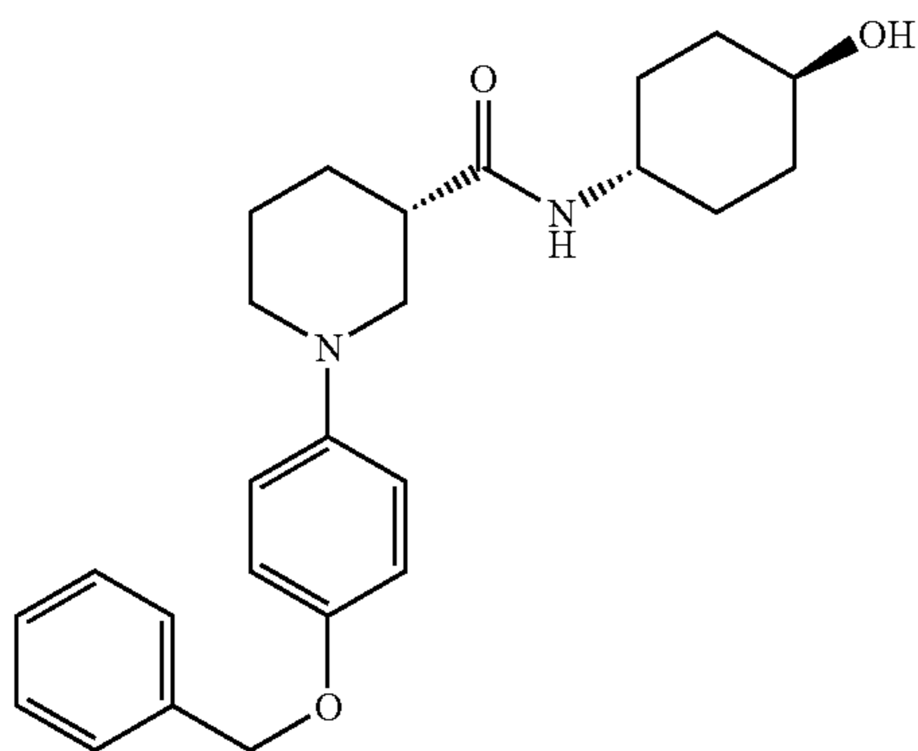
(3S)-1-[4-(Benzyloxy)phenyl]-N-(4-hydroxycyclohexyl)piperidine-3-carboxamide
