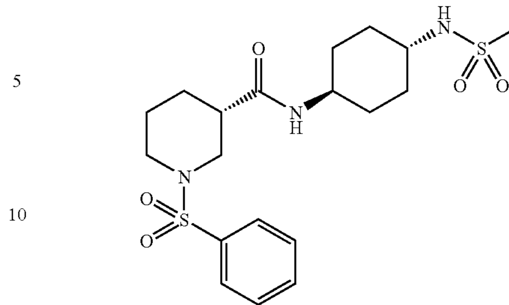
(3S)-N-{trans-4-[(Methylsulfonyl)amino]cyclohexyl}-1-(phenylsulfonyl)piperidine-3-carboxamide
