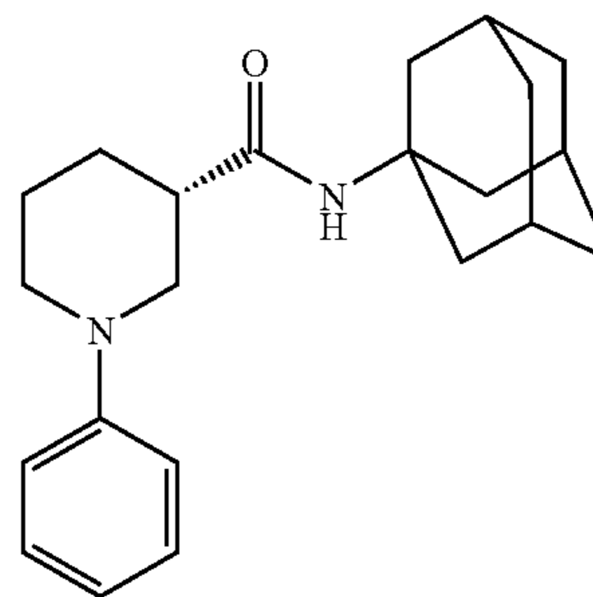
(3S)-N-1-Adamantyl-1-phenylpiperidine-3-carboxamide
