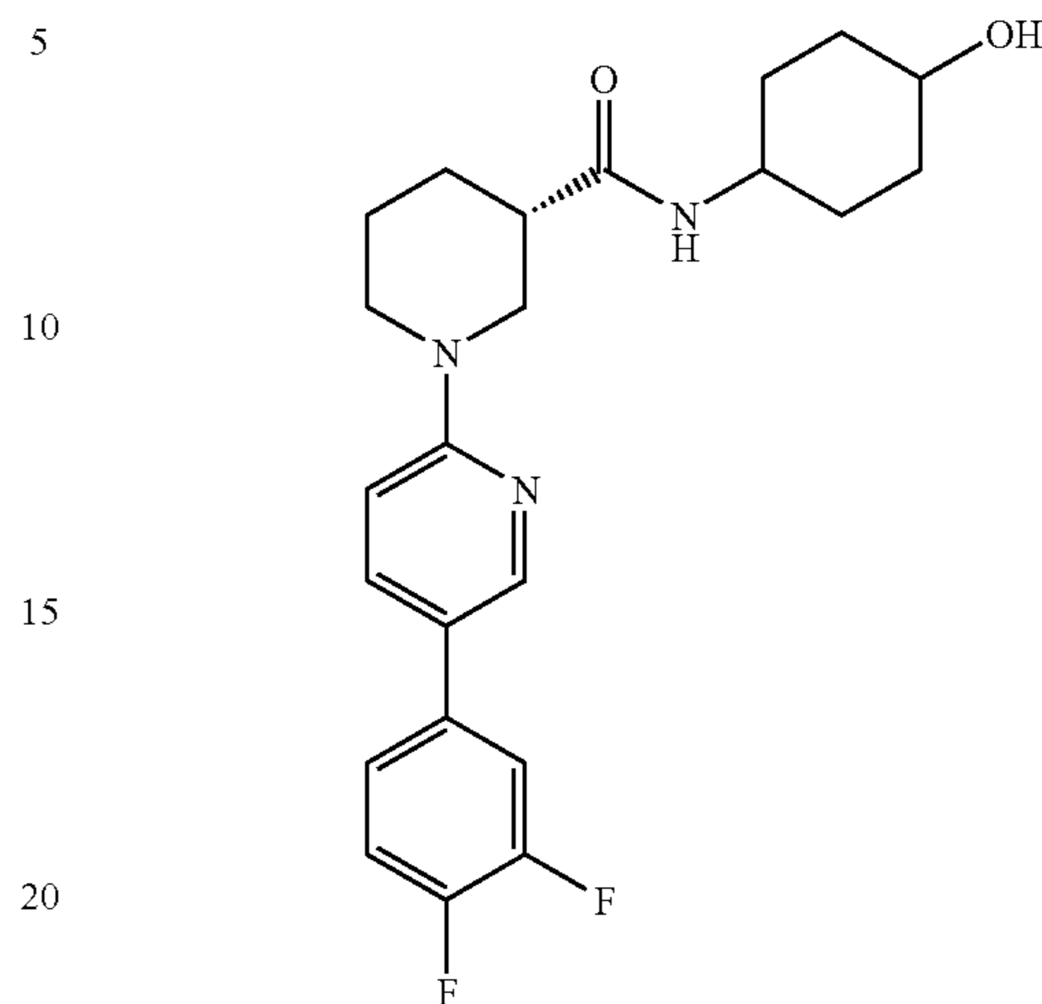
(3S)-N-(4-Hydroxycyclohexyl)-1-(5-phenylpyridin-2-yl)piperidine-3-carboxamide
