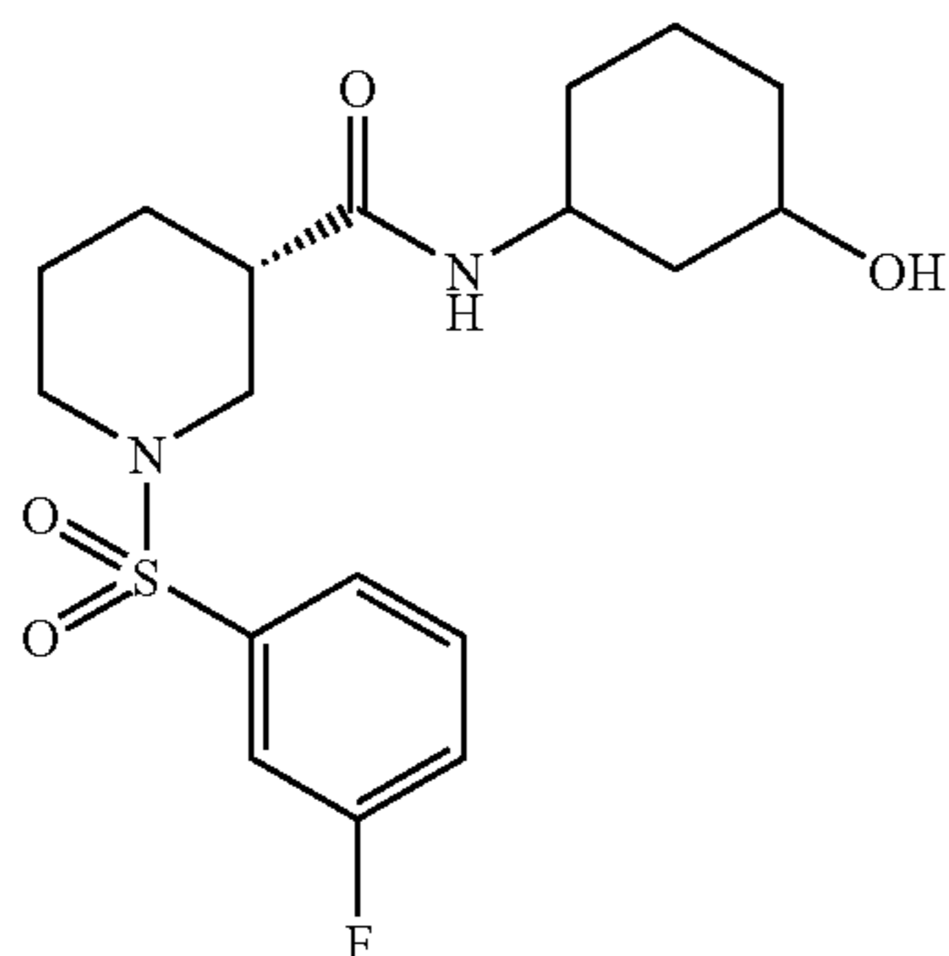
(3S)-1-[(3-Fluorophenyl)sulfonyl]-N-(3-hydroxycyclohexyl)piperidine-3-carboxamide
