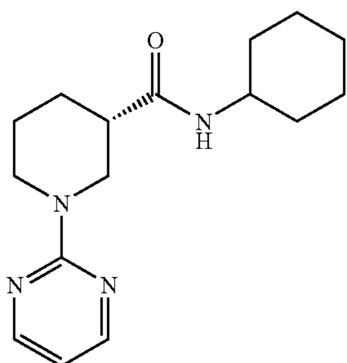
(3S)-N-Cyclohexyl-1-pyrimidin-2-ylpiperidine-3-carboxamide
