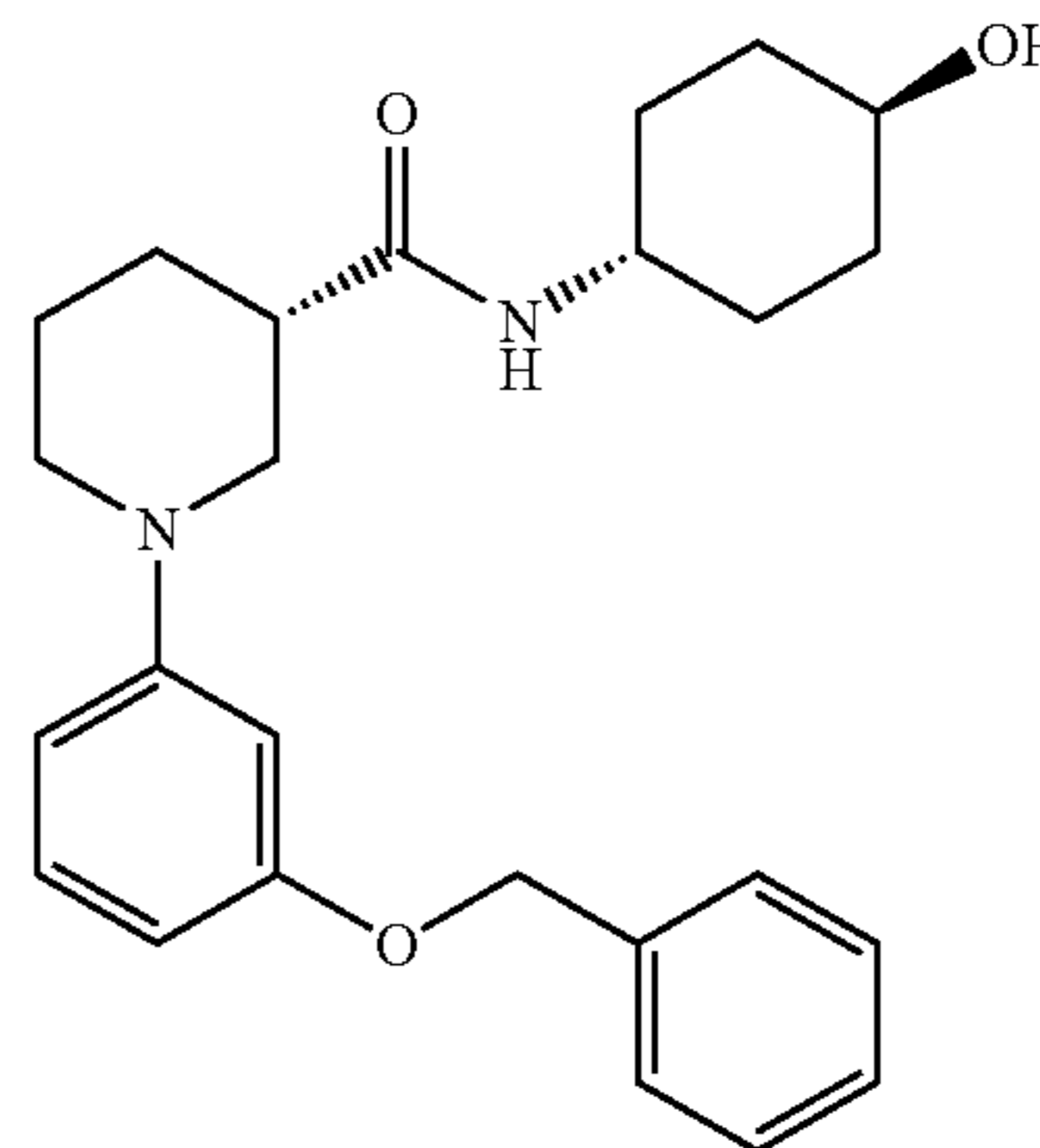
Example 172
