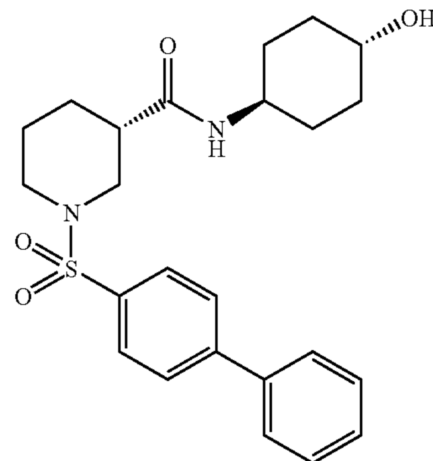
(3S)-1-(Biphenyl-4-ylsulfonyl)-N-(trans-4-hydroxycyclohexyl)piperidine-3-carboxamide
