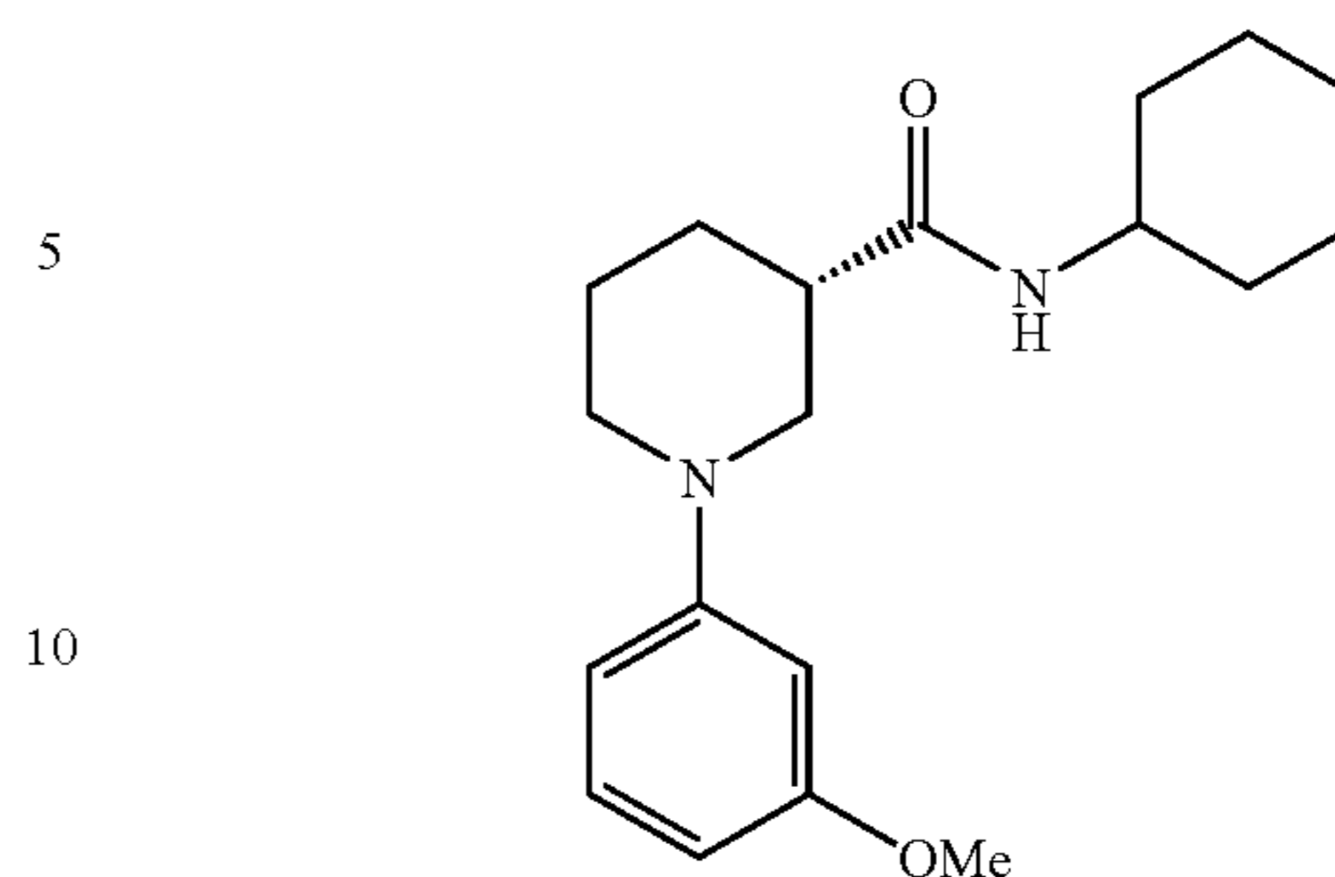
(3S)-N-Cyclohexyl-1-(3-methoxyphenyl)piperidine-3-carboxamide
