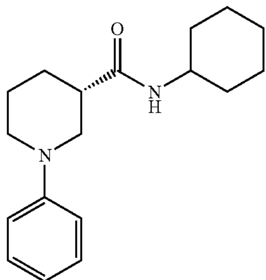
(3S)-N-Cyclohexyl-1-phenylpiperidine-3-carboxamide
