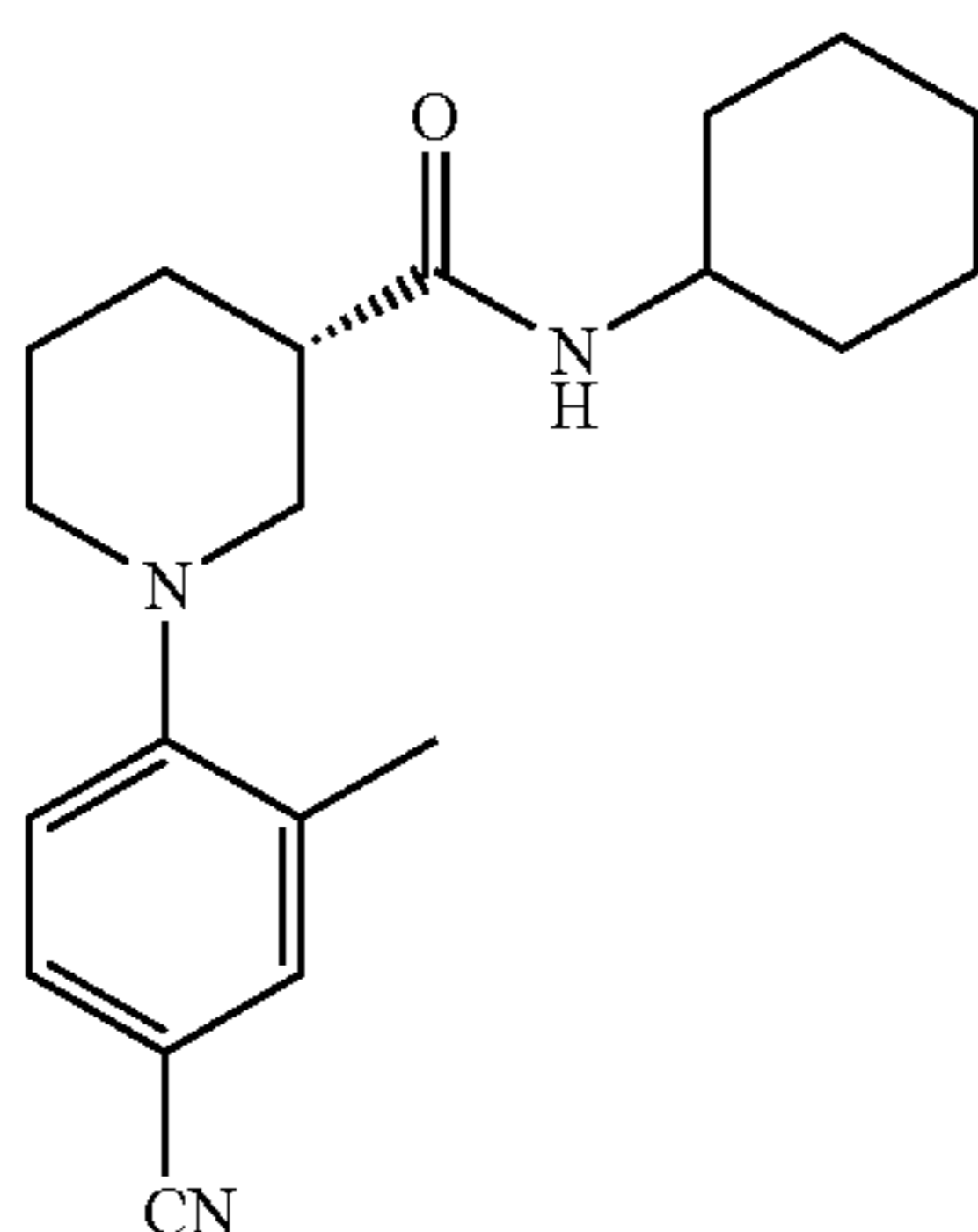
(3S)-1-(4-Cyano-2-methylphenyl)-N-cyclohexylpiperidine-3-carboxamide
