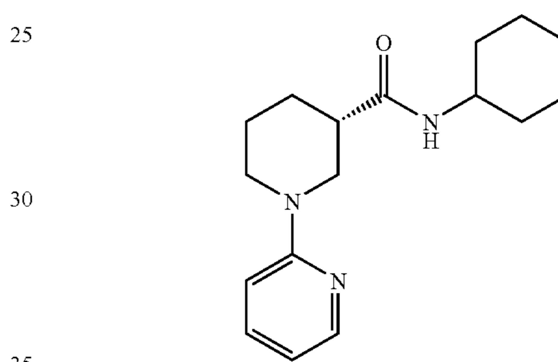
(3S)-N-Cyclohexyl-1-pyridin-2-ylpiperidine-3-carboxamide
