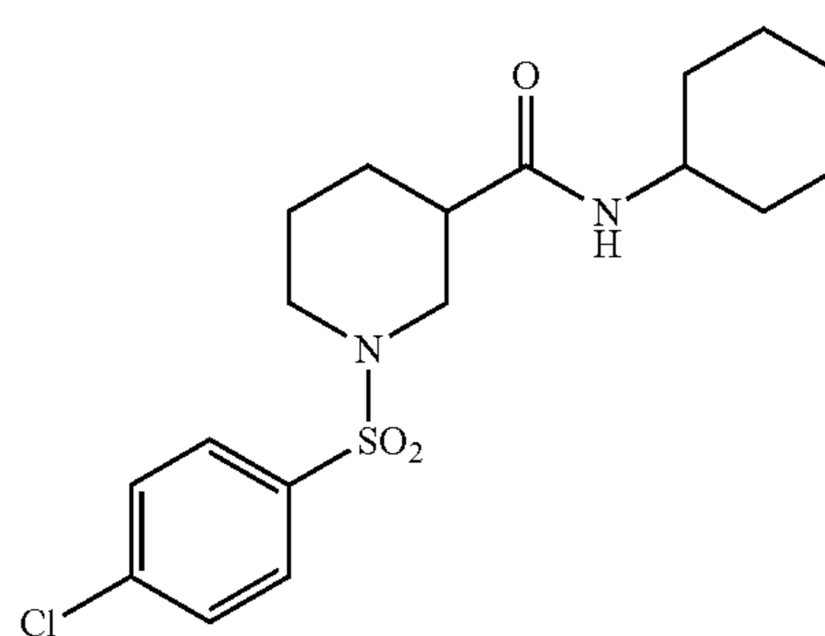
1-[(4-Chlorophenyl)sulfonyl]-N-cyclohexylpiperi- dine-3-carboxamide
