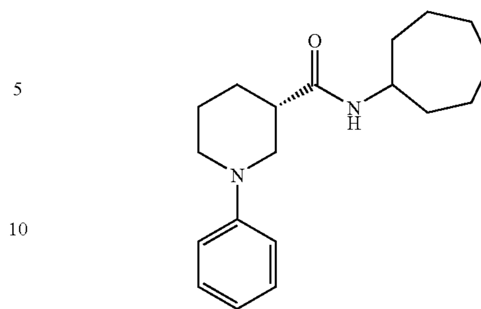
(3S)-N-Cycloheptyl-1-phenylpiperidine-3-carboxamide
