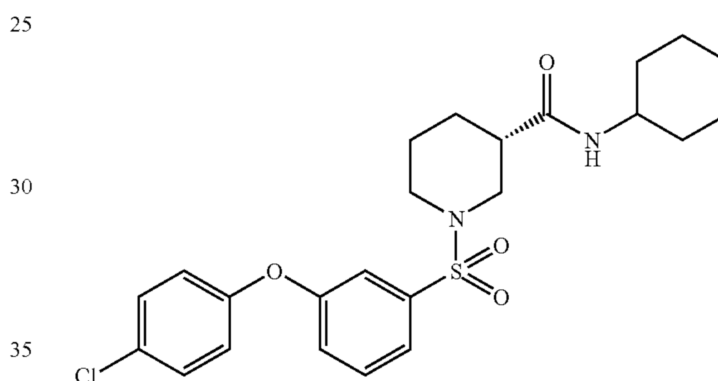
(3S)-1-([3-(4-chlorophenoxy)phenyl]sulfonyl)-N-cyclohexylpiperidine-3-carboxamide
