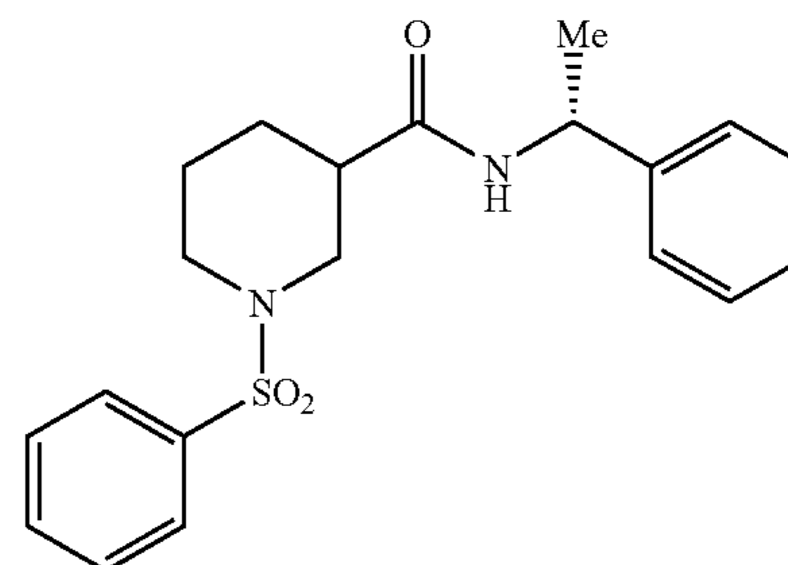
Example 5
