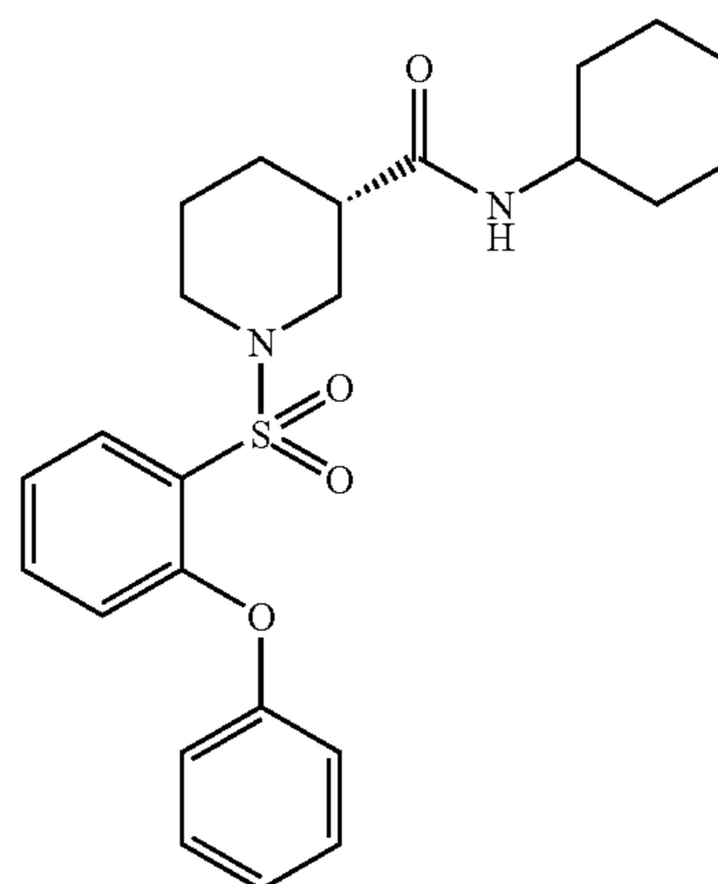
(3S)-N-Cyclohexyl-1-[(2-phenoxyphenyl)sulfonyl]piperidine-3-carboxamide
