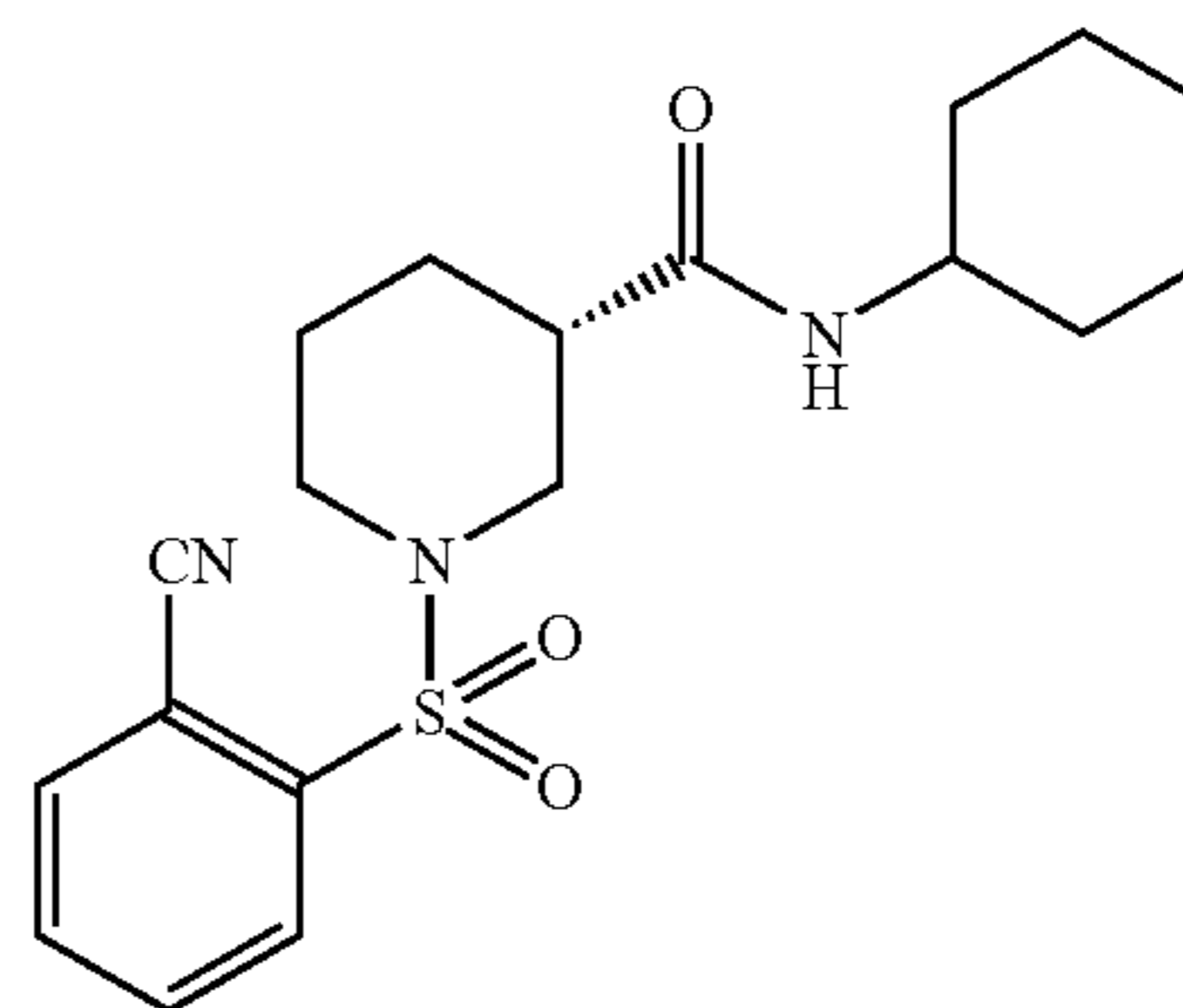
(3S)-1-[(2-Cyanophenyl)sulfonyl]-N-cyclohexylpiperidine-3-carboxamide
