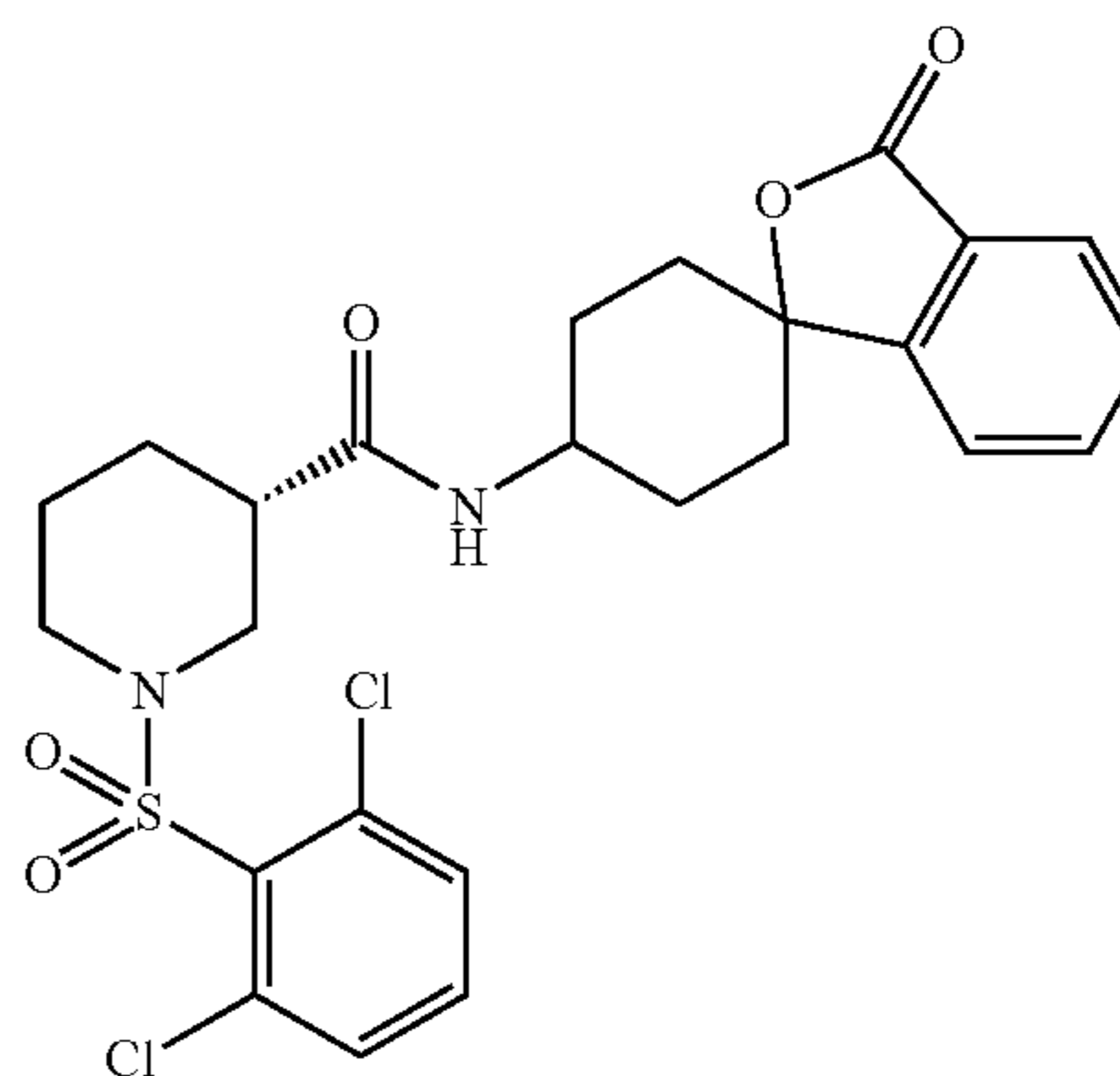
(3S)-1-[(2,6-Dichlorophenyl)sulfonyl]-N-(3-oxo-3H-spiro[2-benzofuran-1,1'-cyclohexan]-4'-yl)piperidine-3-carboxamide
