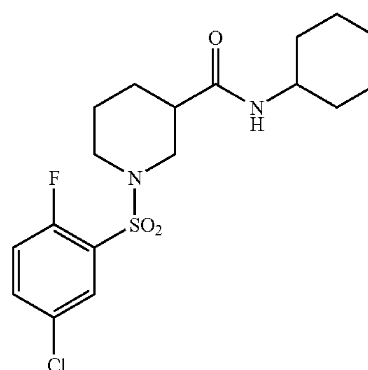
1-[(5-Chloro-2-fluorophenyl)sulfonyl]-N-cyclohexy- lpiperidine-3-carboxamide
