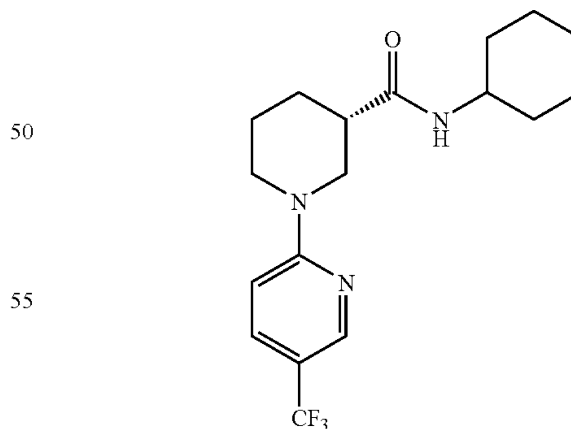
(3S)-N-Cyclohexyl-1-[5-(trifluoromethyl)pyridin-2-yl]piperidine-3-carboxamide
