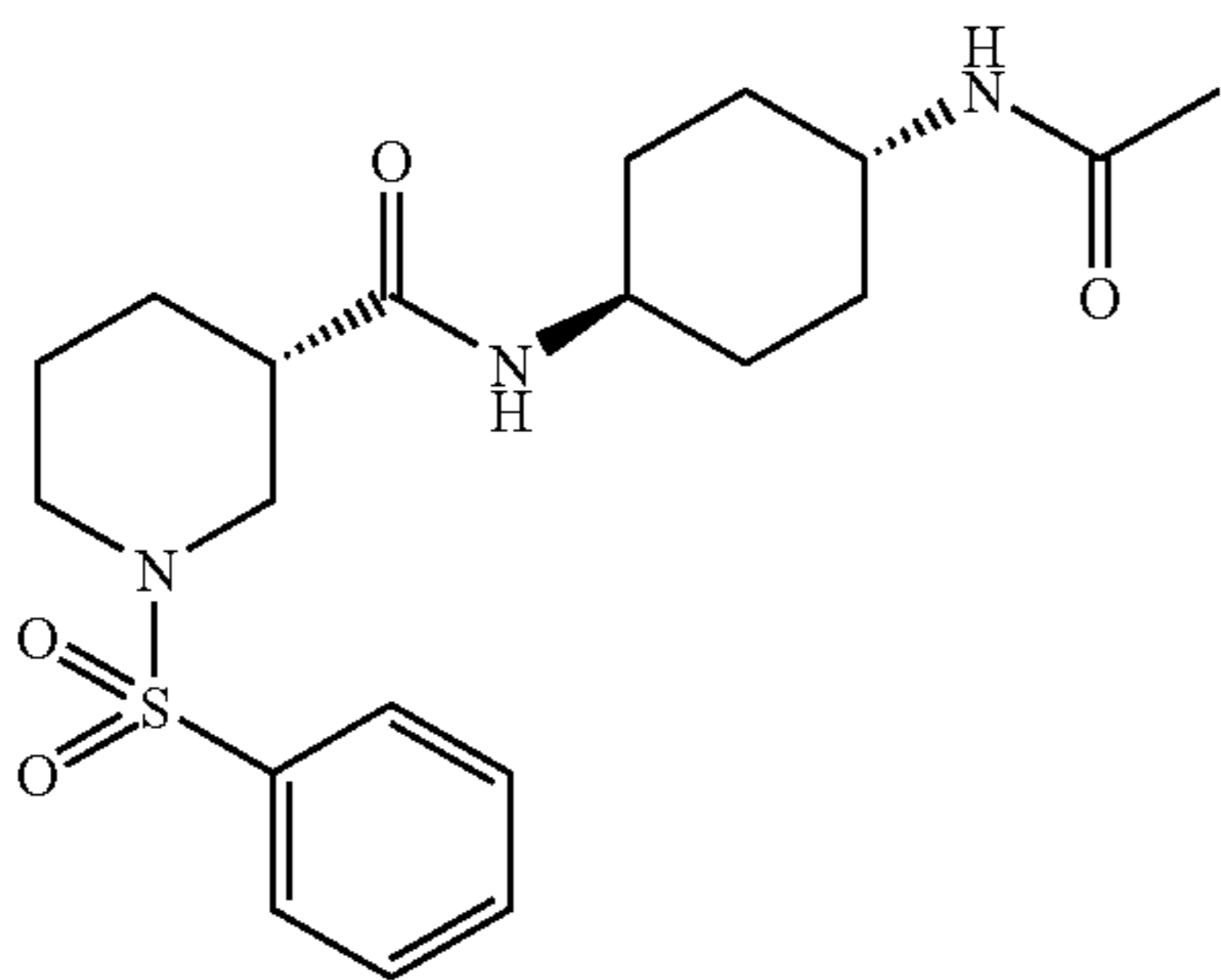
(3S)-N-[trans-4-(Acetylamino)cyclohexyl]-1-(phenylsulfonyl)piperidine-3-carboxamide
