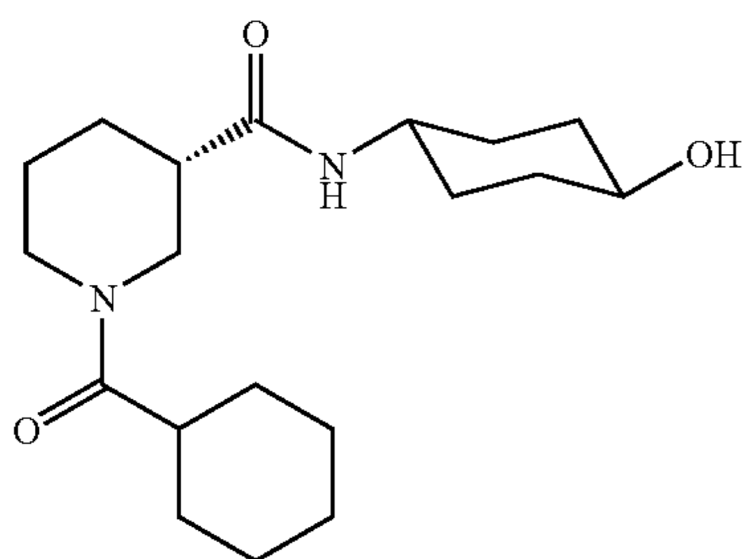
Example 175
