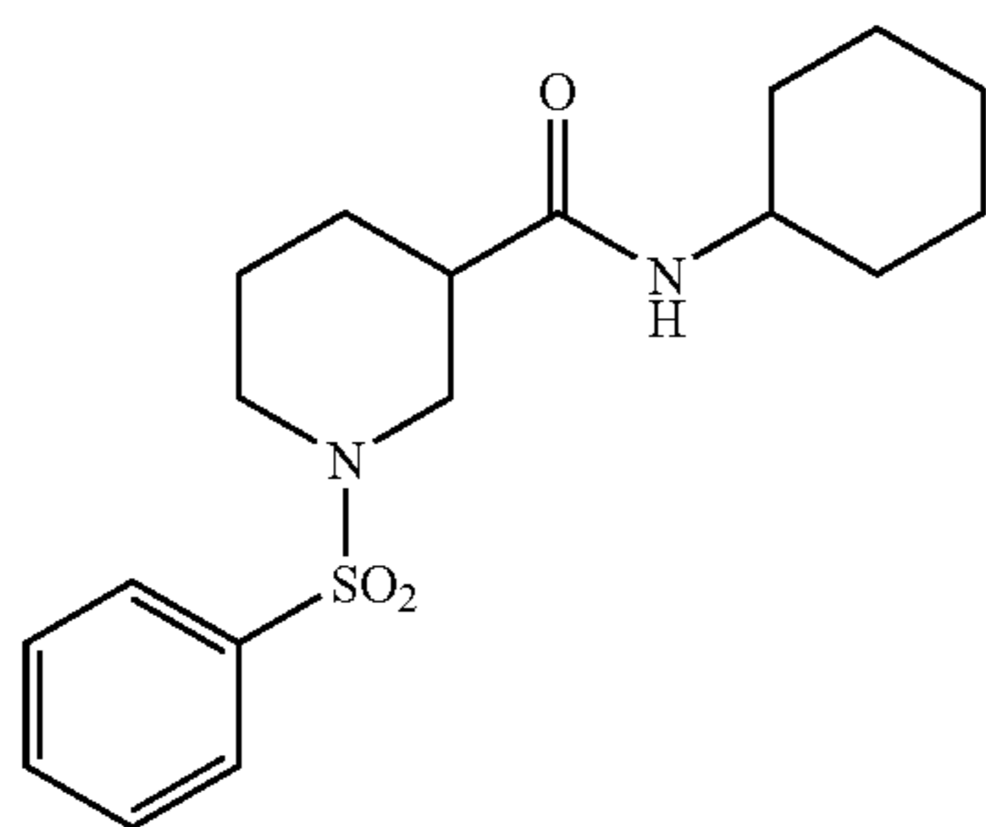
Example 2
