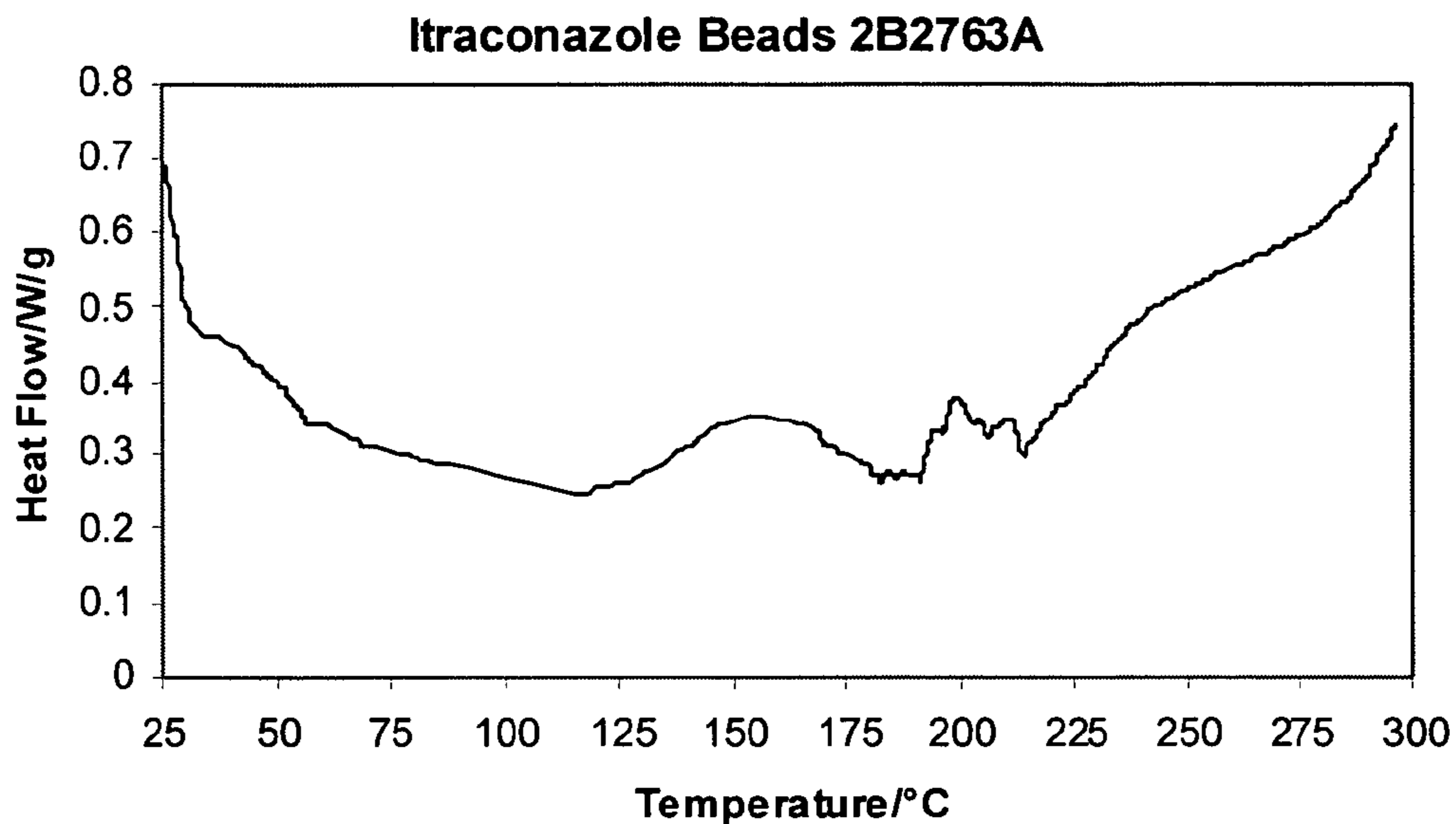
Figure 3: Normalized DSC thermogram from Itraconazole loaded beads
